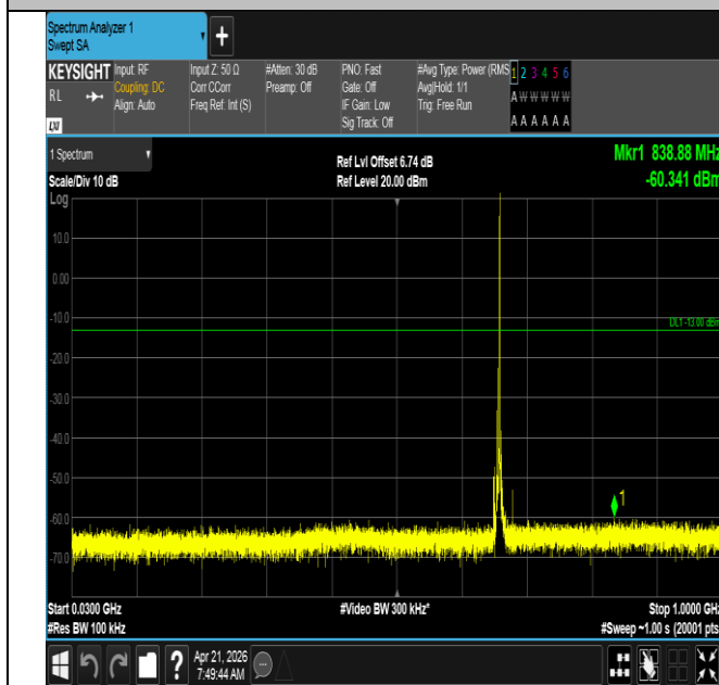
Band71-5MHz-16QAM-133147-1RB#24-30~1000-PASS
