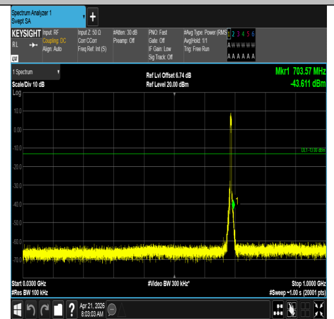
Band71-5MHz-16QAM-133447-25RB#0-30~1000-PASS
