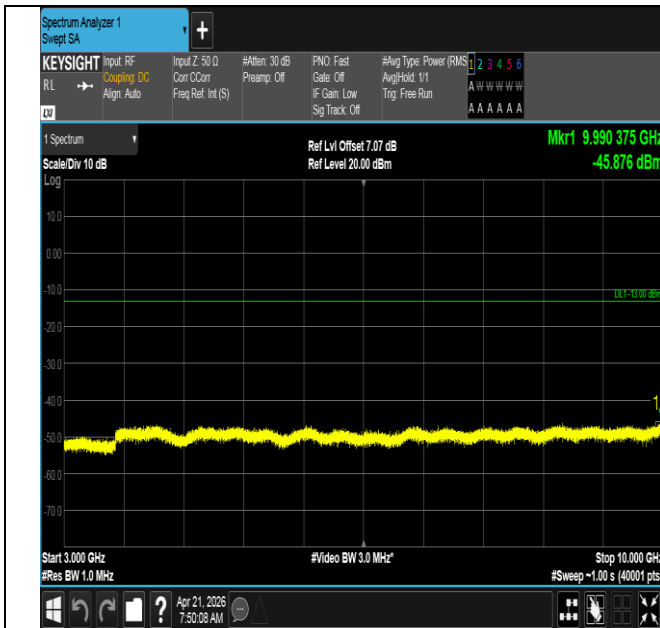
Band71-5MHz-16QAM-133147-1RB#24-3000~10000-PASS
