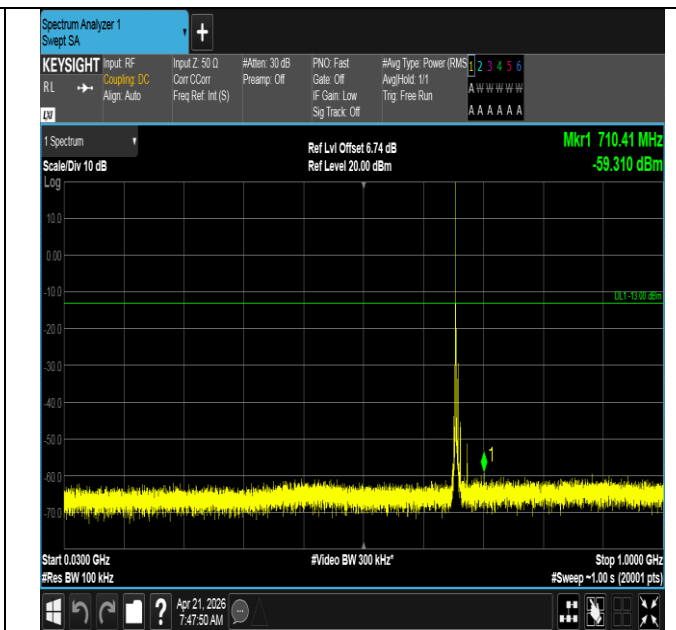
Band71-5MHz-16QAM-133147-1RB#0-30~1000-PASS
