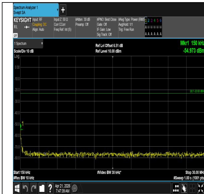
Band71-5MHz-16QAM-133147-1RB#0-0.15~30-PASS
