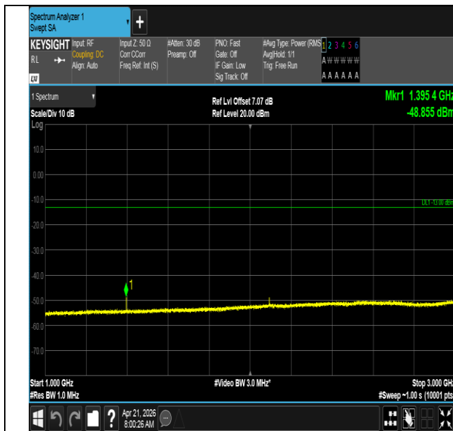
Band71-5MHz-QPSK-133447-1RB#24-1000~3000-PASS
