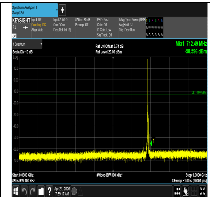
Band71-5MHz-16QAM-133447-1RB#0-30~1000-PASS
