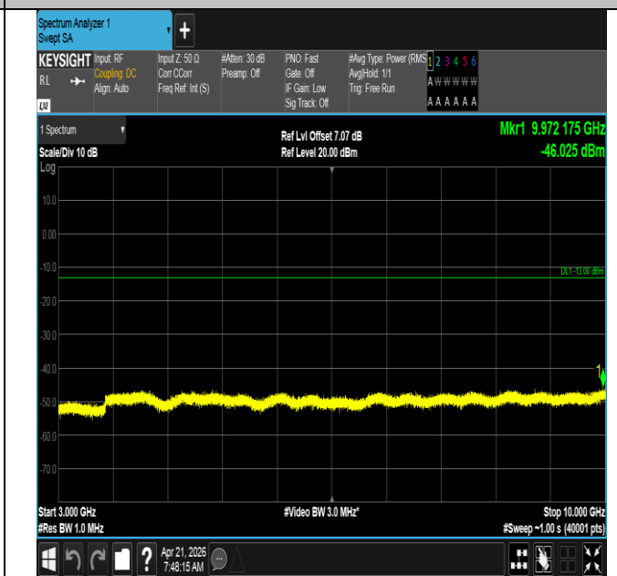
Band71-5MHz-16QAM-133147-1RB#0-3000~10000-PASS
