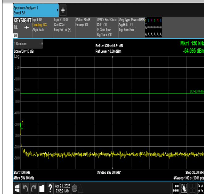
Band71-5MHz-16QAM-133297-1RB#0-0.15~30-PASS
