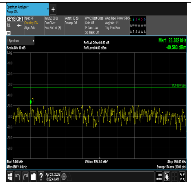
Band71-5MHz-16QAM-133447-25RB#0-0.009~0.15-PASS
