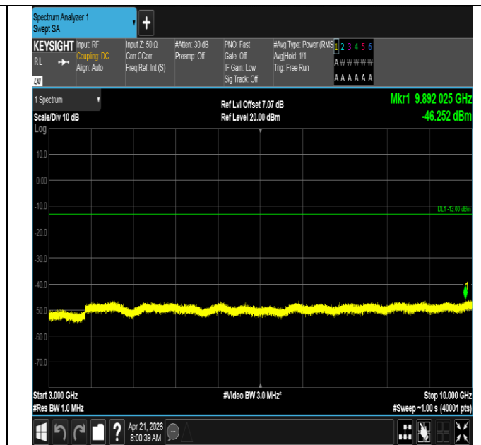
Band71-5MHz-QPSK-133447-1RB#24-3000~10000-PASS
