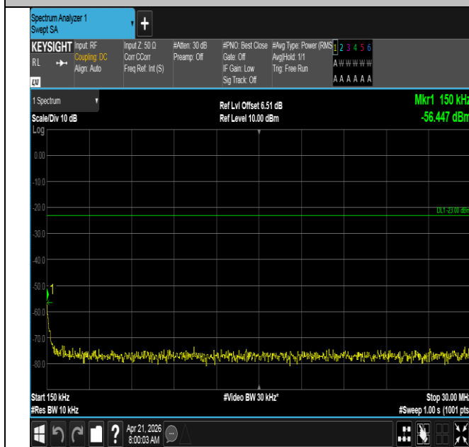
Band71-5MHz-QPSK-133447-1RB#24-0.15~30-PASS
