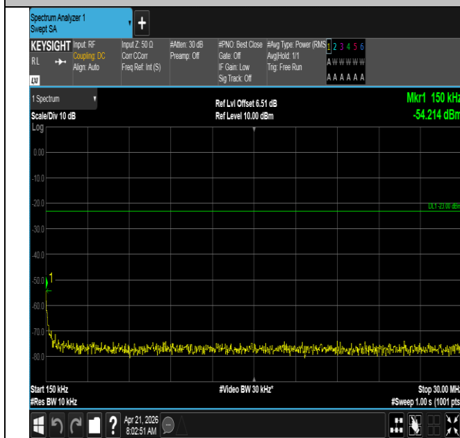
Band71-5MHz-16QAM-133447-25RB#0-0.15~30-PASS
