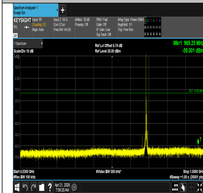
Band71-5MHz-QPSK-133447-1RB#0-30~1000-PASS
