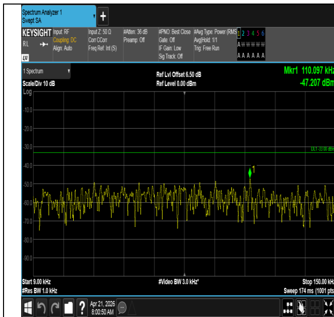
Band71-5MHz-16QAM-133447-1RB#24-0.009~0.15-PASS
