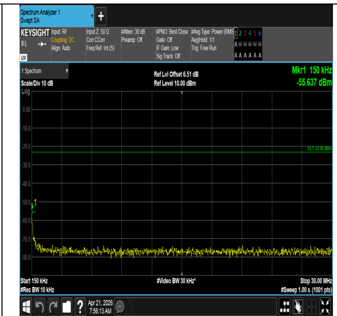
Band71-5MHz-QPSK-133297-25RB#0-0.15~30-PASS
