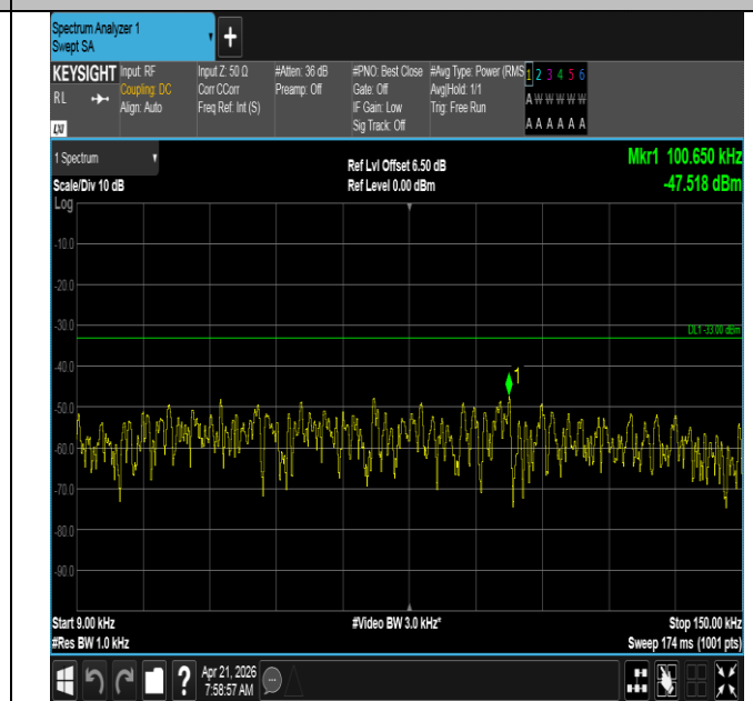
Band71-5MHz-16QAM-133447-1RB#0-0.009~0.15-PASS
