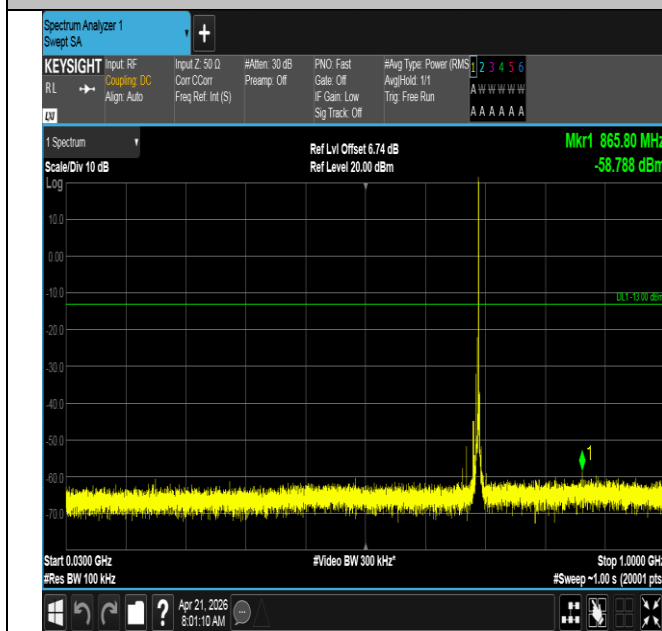
Band71-5MHz-16QAM-133447-1RB#24-30~1000-PASS
