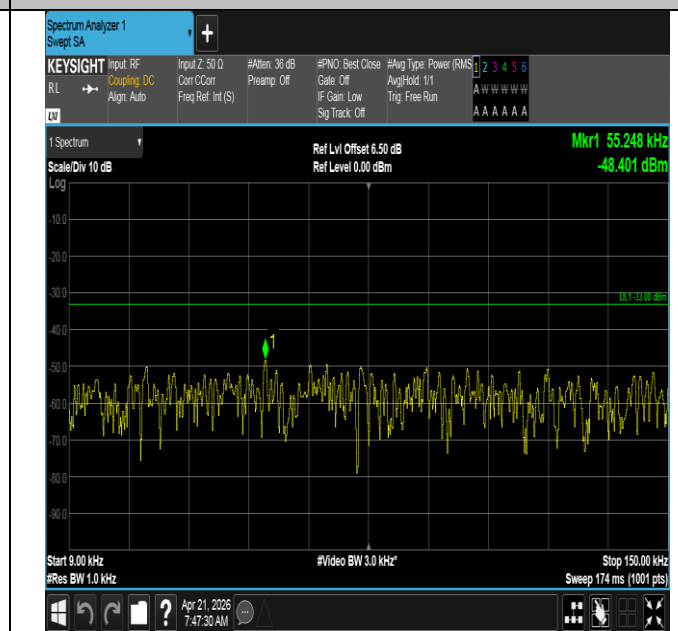
Band71-5MHz-16QAM-133147-1RB#0-0.009~0.15-PASS
