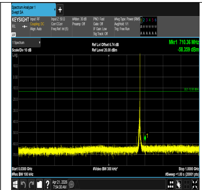
Band71-5MHz-QPSK-133297-1RB#24-30~1000-PASS
