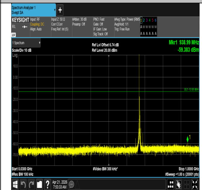
Band71-5MHz-16QAM-133297-1RB#0-30~1000-PASS
