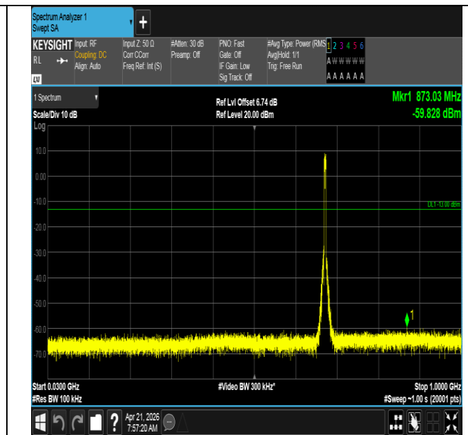
Band71-5MHz-16QAM-133297-25RB#0-30~1000-PASS
