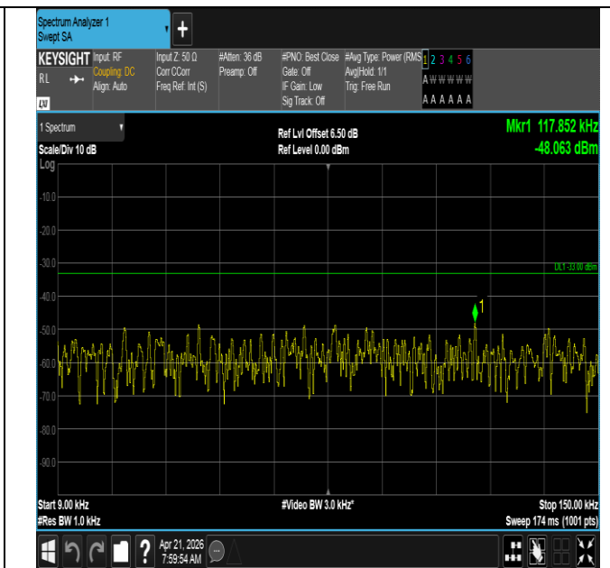
Band71-5MHz-QPSK-133447-1RB#24-0.009~0.15-PASS
