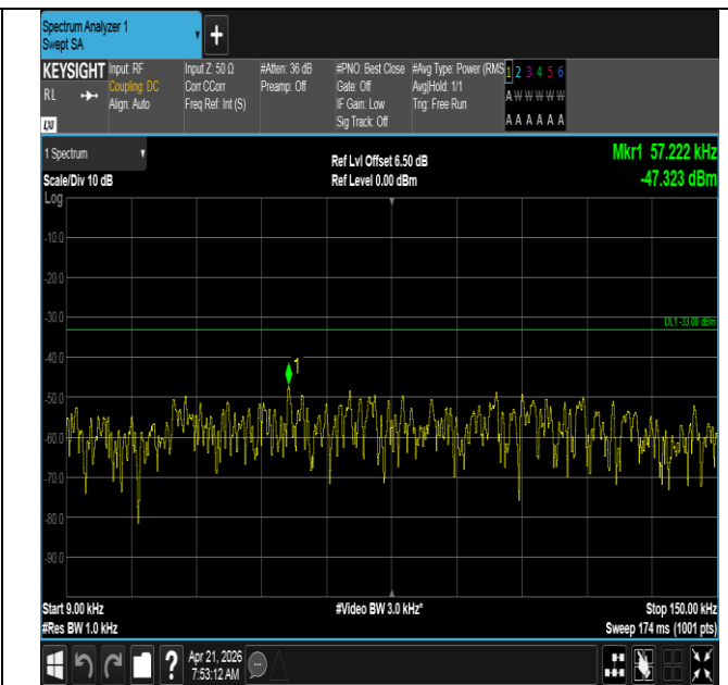
Band71-5MHz-16QAM-133297-1RB#0-0.009~0.15-PASS
