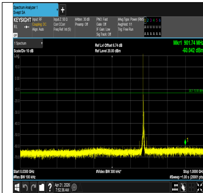
Band71-5MHz-QPSK-133297-1RB#0-30~1000-PASS
