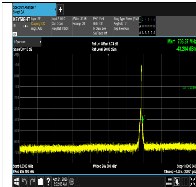
Band71-5MHz-QPSK-133447-25RB#0-30~1000-PASS
