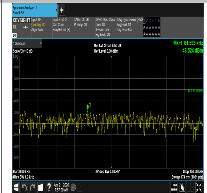
Band71-5MHz-16QAM-133297-25RB#0-0.009~0.15-PASS
