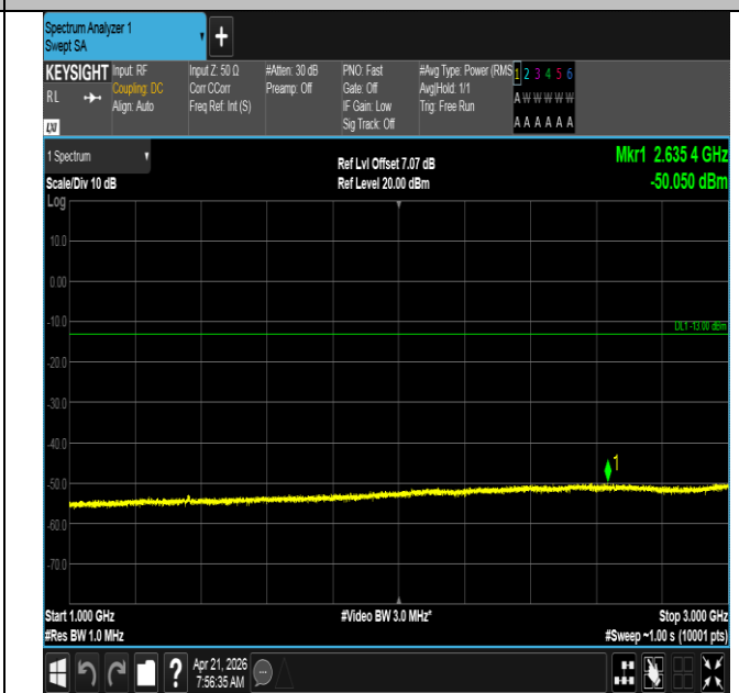
Band71-5MHz-QPSK-133297-25RB#0-1000~3000-PASS
