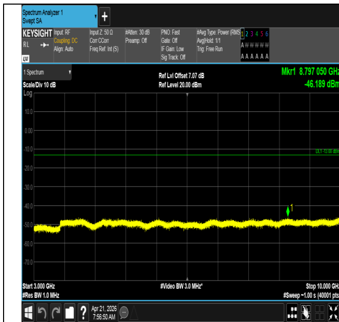
Band71-5MHz-QPSK-133297-25RB#0-3000~10000-PASS
