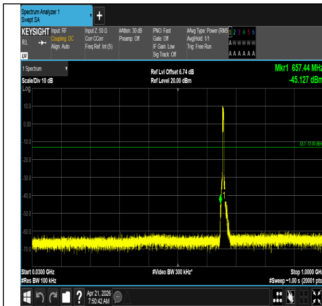
Band71-5MHz-QPSK-133147-25RB#0-30~1000-PASS
