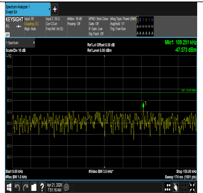
Band71-5MHz-16QAM-133147-25RB#0-0.009~0.15-PASS
