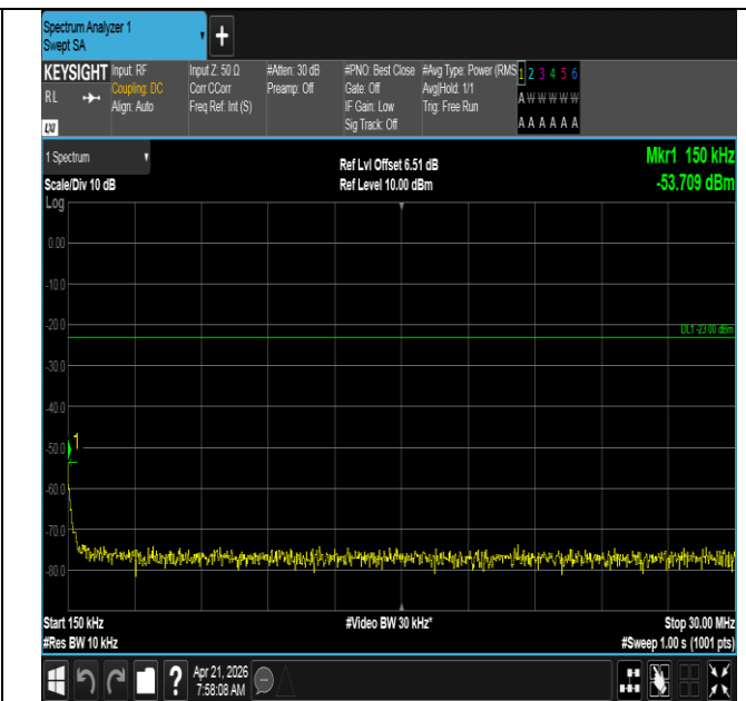
Band71-5MHz-QPSK-133447-1RB#0-0.15~30-PASS
