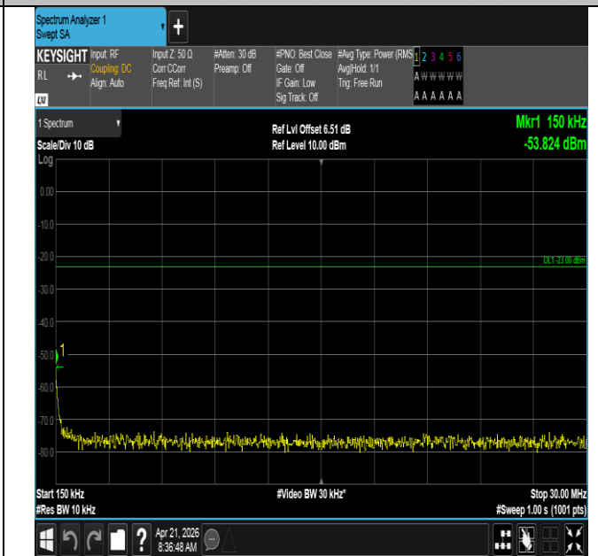
Band71-10MHz-QPSK-133172-1RB#0-0.15~30-PASS
