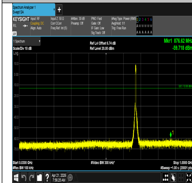
Band71-5MHz-QPSK-133297-25RB#0-30~1000-PASS
