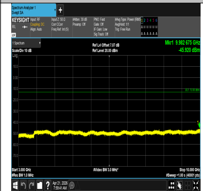
Band71-5MHz-16QAM-133447-1RB#0-3000~10000-PASS
