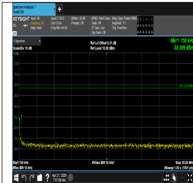
Band71-5MHz-16QAM-133297-25RB#0-0.15~30-PASS
