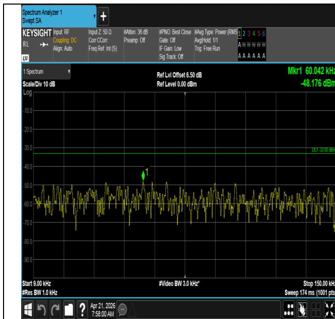
Band71-5MHz-QPSK-133447-1RB#0-0.009~0.15-PASS
