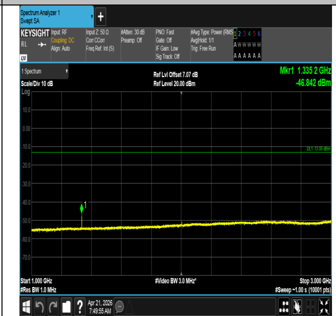
Band71-5MHz-16QAM-133147-1RB#24-1000~3000-PASS
