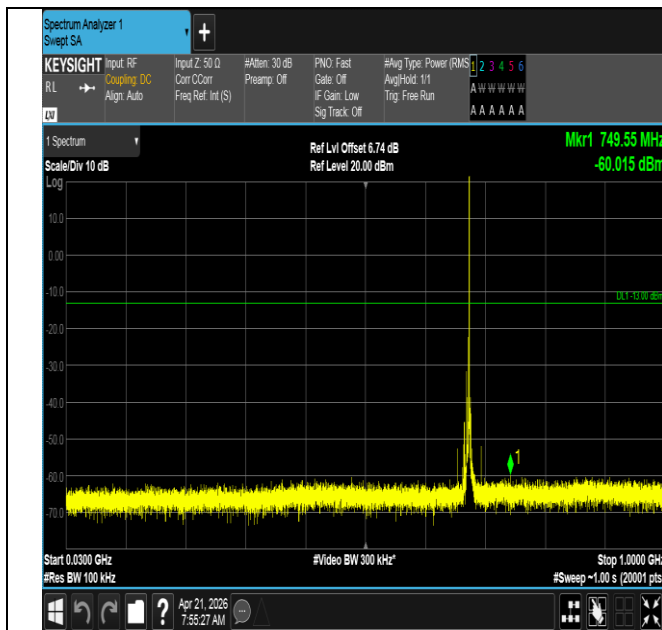
Band71-5MHz-16QAM-133297-1RB#24-30~1000-PASS
