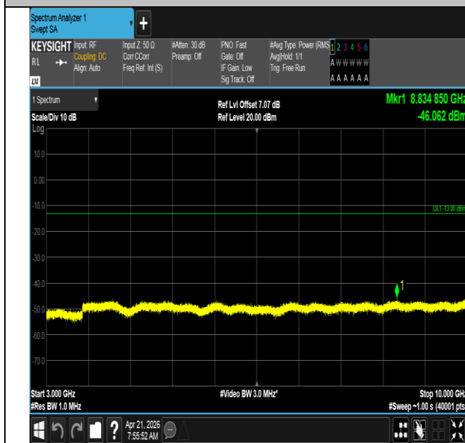
Band71-5MHz-16QAM-133297-1RB#24-3000~10000-PASS
