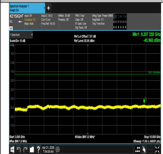
Band71-5MHz-QPSK-133297-1RB#24-3000~10000-PASS
