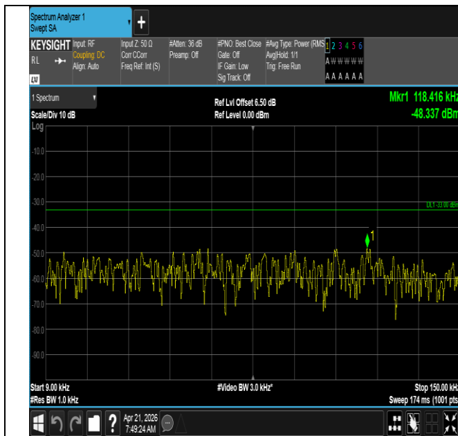
Band71-5MHz-16QAM-133147-1RB#24-0.009~0.15-PASS
