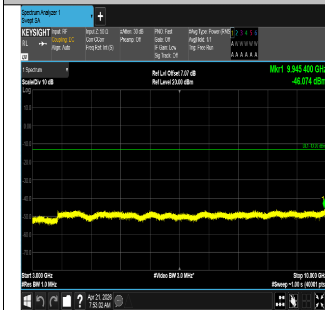
Band71-5MHz-QPSK-133297-1RB#0-3000~10000-PASS
