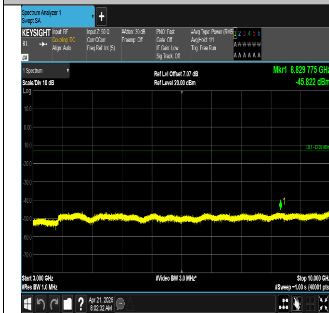
Band71-5MHz-QPSK-133447-25RB#0-3000~10000-PASS
