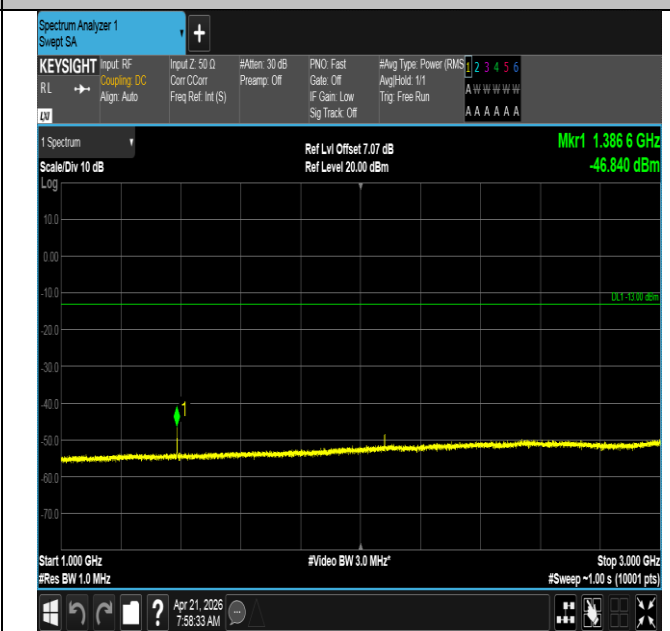
Band71-5MHz-QPSK-133447-1RB#0-1000~3000-PASS
