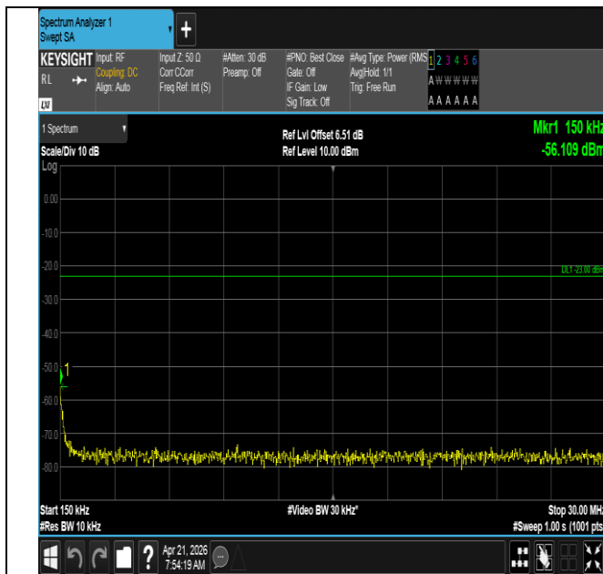
Band71-5MHz-QPSK-133297-1RB#24-0.15~30-PASS
