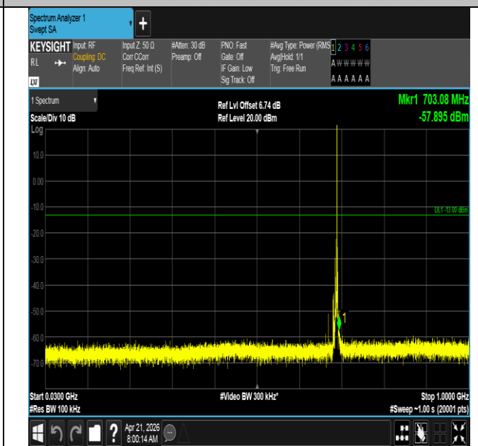
Band71-5MHz-QPSK-133447-1RB#24-30~1000-PASS
