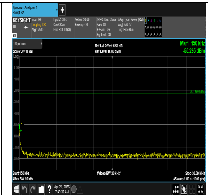
Band71-5MHz-16QAM-133147-1RB#24-0.15~30-PASS
