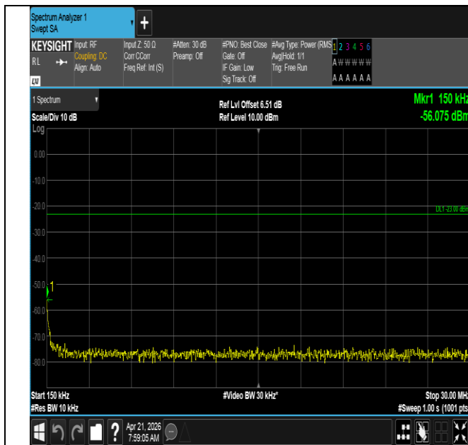
Band71-5MHz-16QAM-133447-1RB#0-0.15~30-PASS
