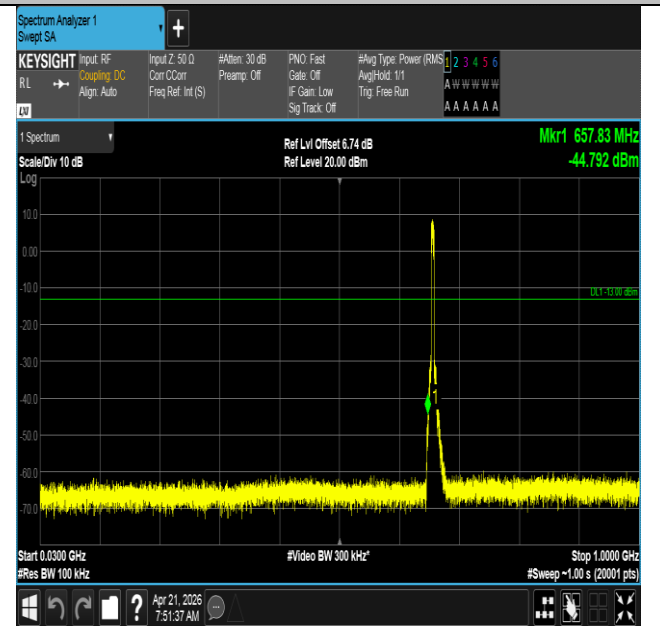
Band71-5MHz-16QAM-133147-25RB#0-30~1000-PASS
