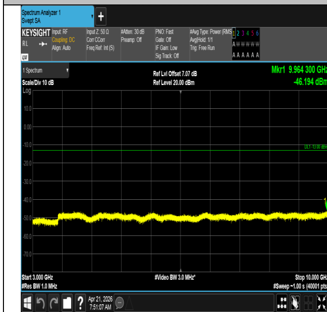
Band71-5MHz-QPSK-133147-25RB#0-3000~10000-PASS
