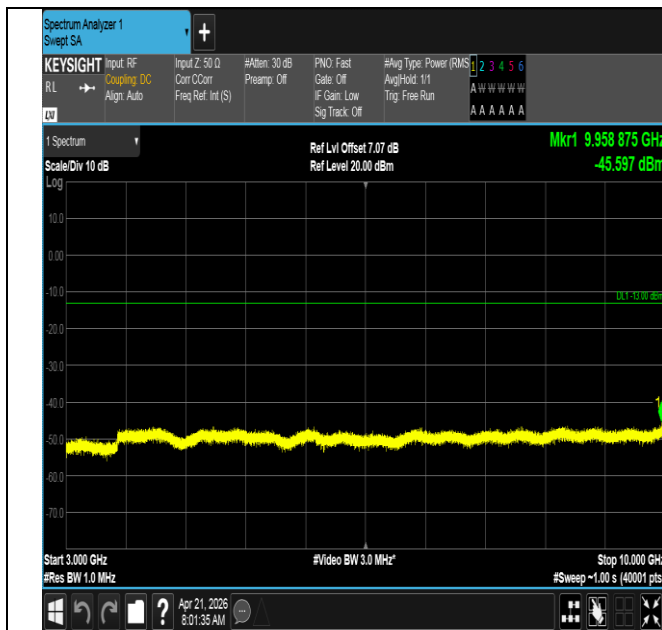
Band71-5MHz-16QAM-133447-1RB#24-3000~10000-PASS
