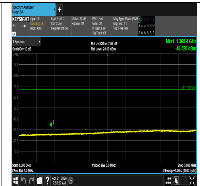
Band71-5MHz-16QAM-133297-1RB#24-1000~3000-PASS
