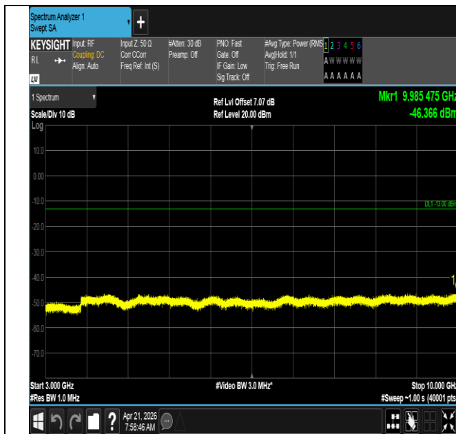
Band71-5MHz-QPSK-133447-1RB#0-3000~10000-PASS
