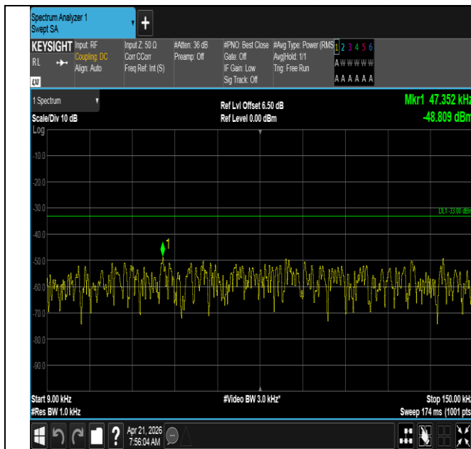
Band71-5MHz-QPSK-133297-25RB#0-0.009~0.15-PASS
