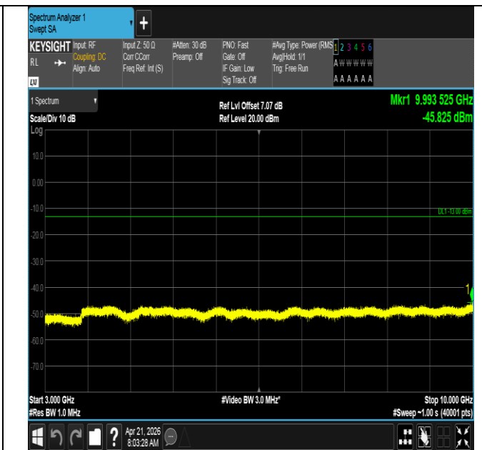
Band71-5MHz-16QAM-133447-25RB#0-3000~10000-PASS
