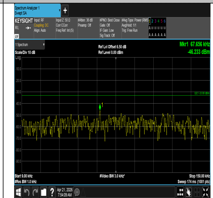
Band71-5MHz-QPSK-133297-1RB#24-0.009~0.15-PASS
