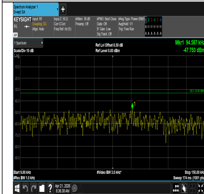
Band71-10MHz-QPSK-133172-1RB#0-0.009~0.15-PASS
