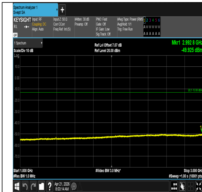
Band71-5MHz-16QAM-133447-25RB#0-1000~3000-PASS
