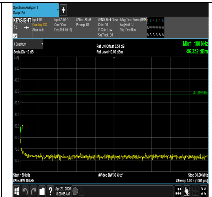
Band71-5MHz-16QAM-133447-1RB#24-0.15~30-PASS
