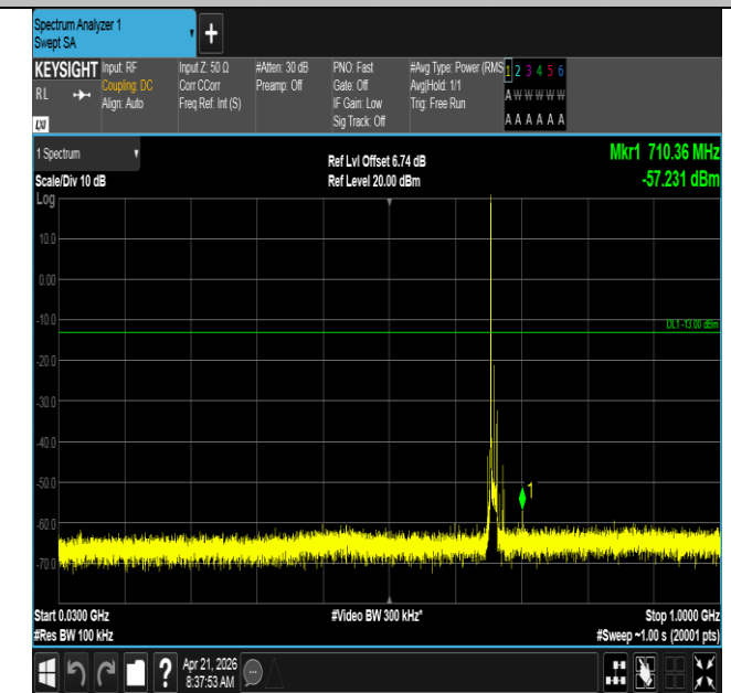
Band71-10MHz-16QAM-133172-1RB#0-30~1000-PASS
