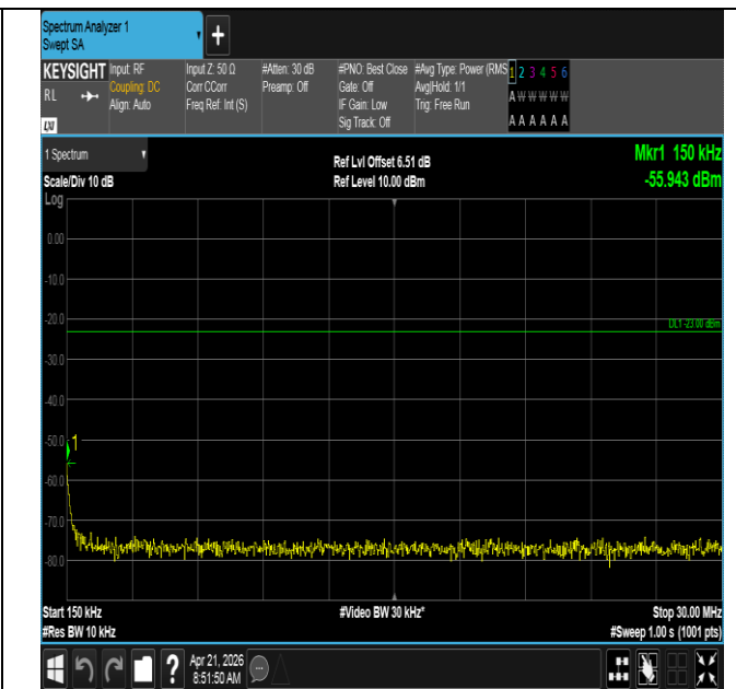
Band71-10MHz-QPSK-133422-50RB#0-0.15~30-PASS
