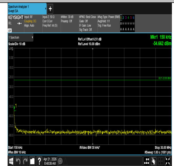
Band71-10MHz-QPSK-133422-1RB#0-0.15~30-PASS
