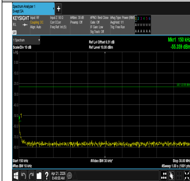
Band71-10MHz-16QAM-133422-1RB#0-0.15~30-PASS
