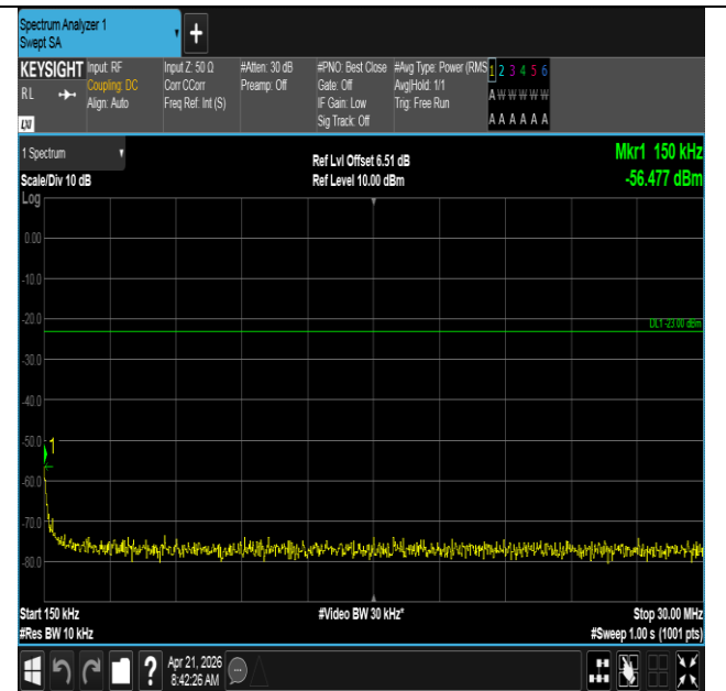
Band71-10MHz-QPSK-133297-1RB#0-0.15~30-PASS
