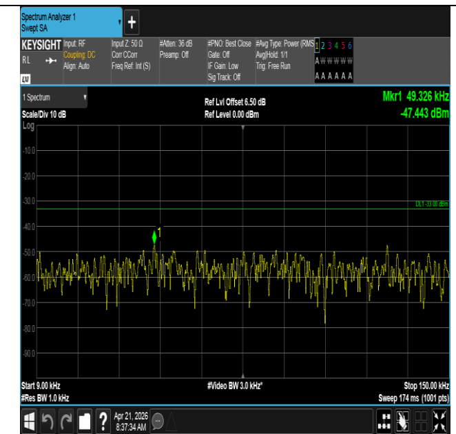
Band71-10MHz-16QAM-133172-1RB#0-0.009~0.15-PASS
