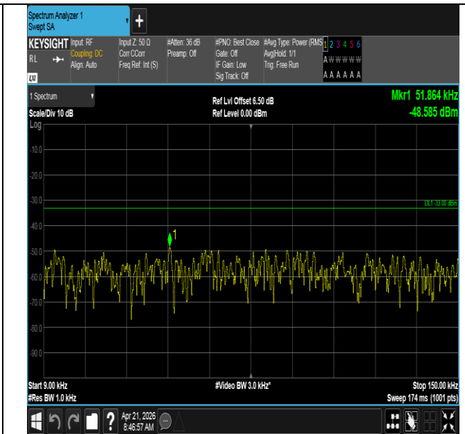
Band71-10MHz-16QAM-133297-50RB#0-0.009~0.15-PASS
