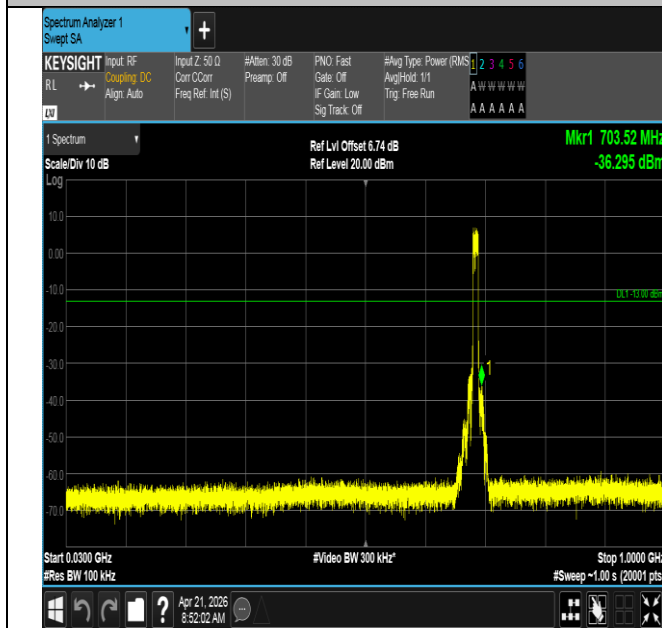
Band71-10MHz-QPSK-133422-50RB#0-30~1000-PASS
