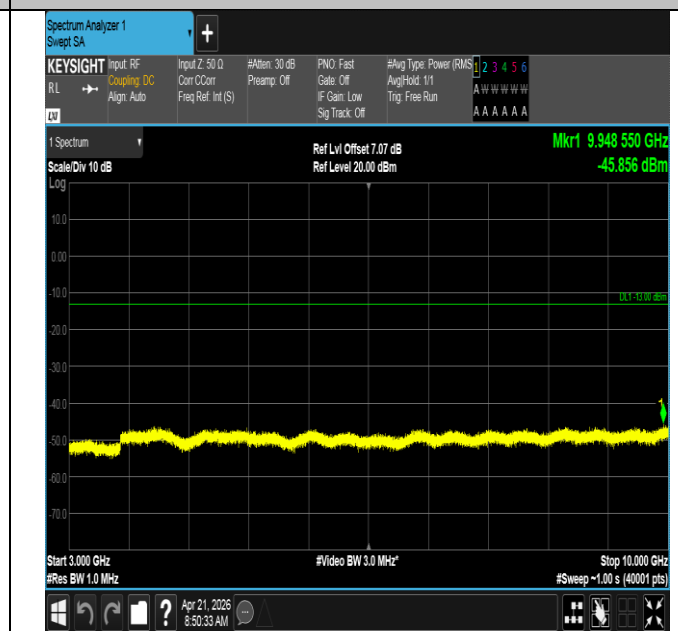
Band71-10MHz-QPSK-133422-1RB#49-3000~10000-PASS
