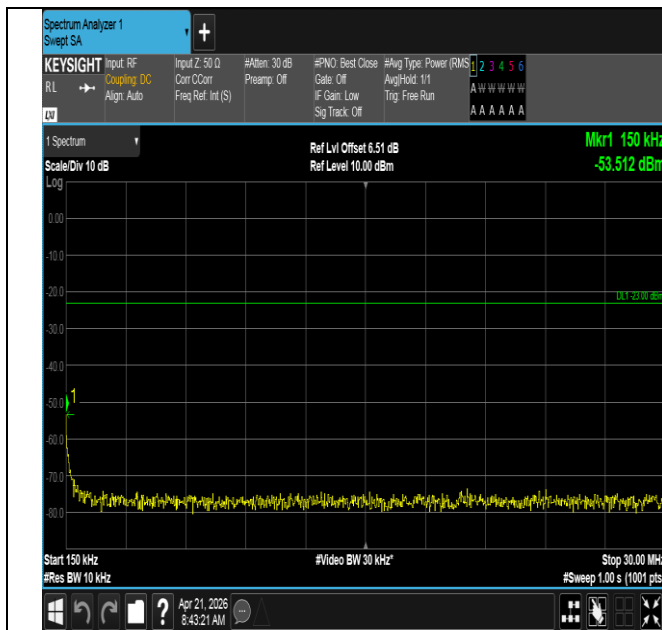
Band71-10MHz-16QAM-133297-1RB#0-0.15~30-PASS
