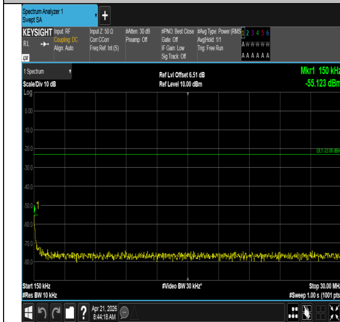
Band71-10MHz-QPSK-133297-1RB#49-0.15~30-PASS
