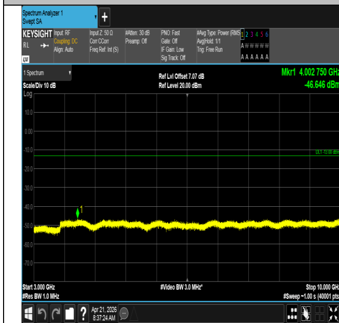
Band71-10MHz-QPSK-133172-1RB#0-3000~10000-PASS
