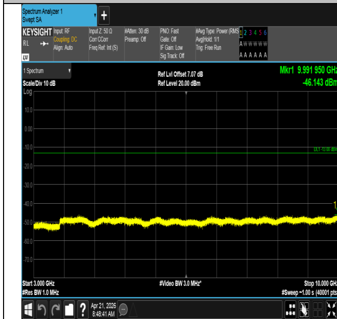
Band71-10MHz-QPSK-133422-1RB#0-3000~10000-PASS
