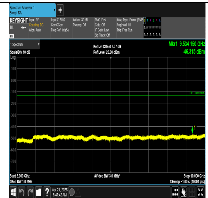
Band71-10MHz-16QAM-133297-50RB#0-3000~10000-PASS
