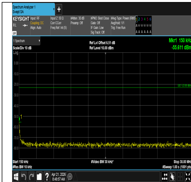
Band71-10MHz-QPSK-133422-1RB#49-0.15~30-PASS
