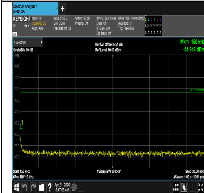
Band71-10MHz-16QAM-133297-50RB#0-0.15~30-PASS
