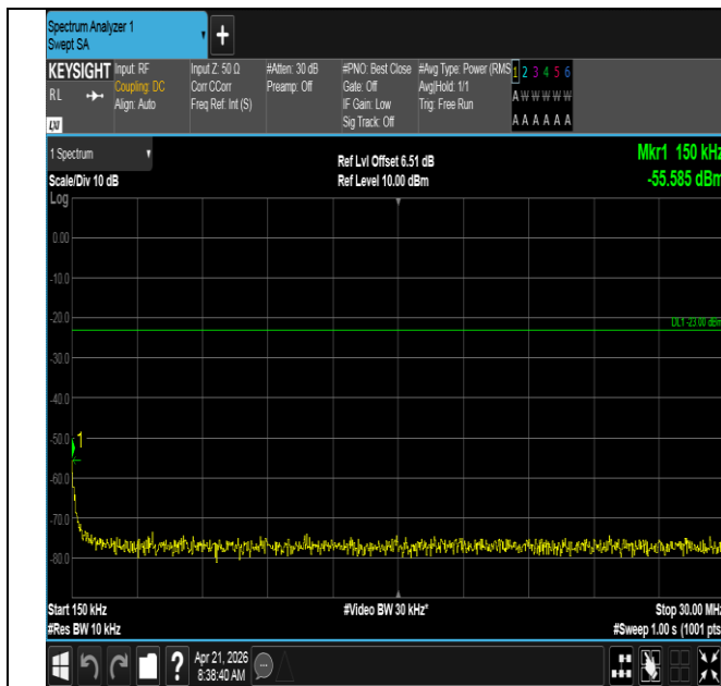
Band71-10MHz-QPSK-133172-1RB#49-0.15~30-PASS
