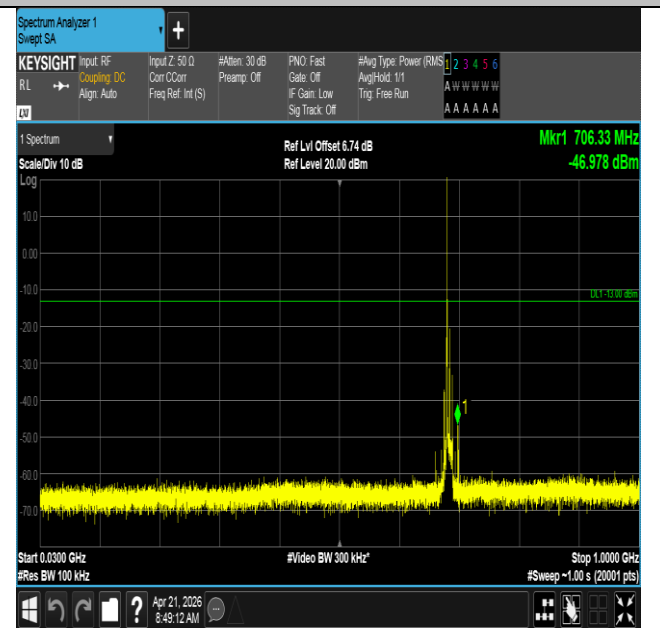
Band71-10MHz-16QAM-133422-1RB#0-30~1000-PASS
