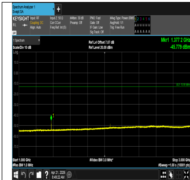
Band71-10MHz-16QAM-133422-1RB#0-1000~3000-PASS
