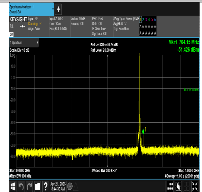
Band71-10MHz-QPSK-133297-1RB#49-30~1000-PASS
