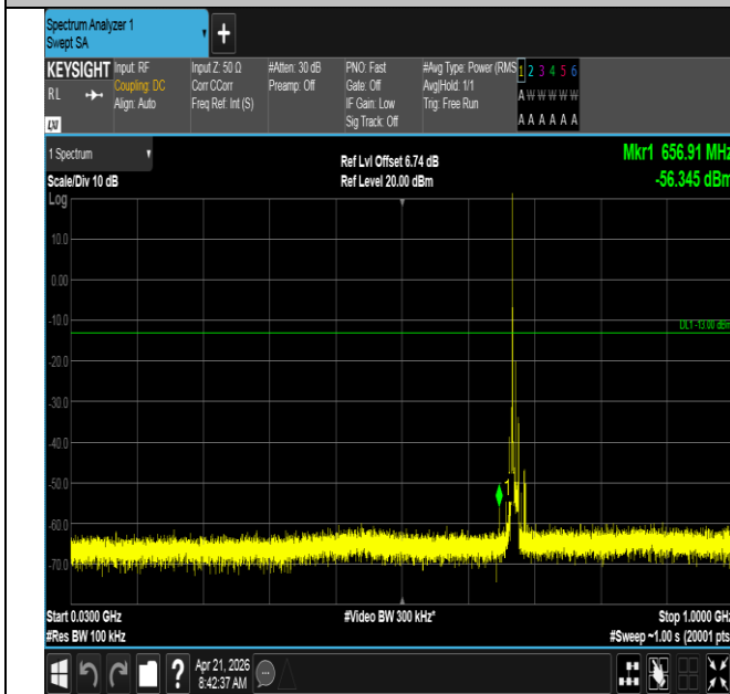
Band71-10MHz-QPSK-133297-1RB#0-30~1000-PASS
