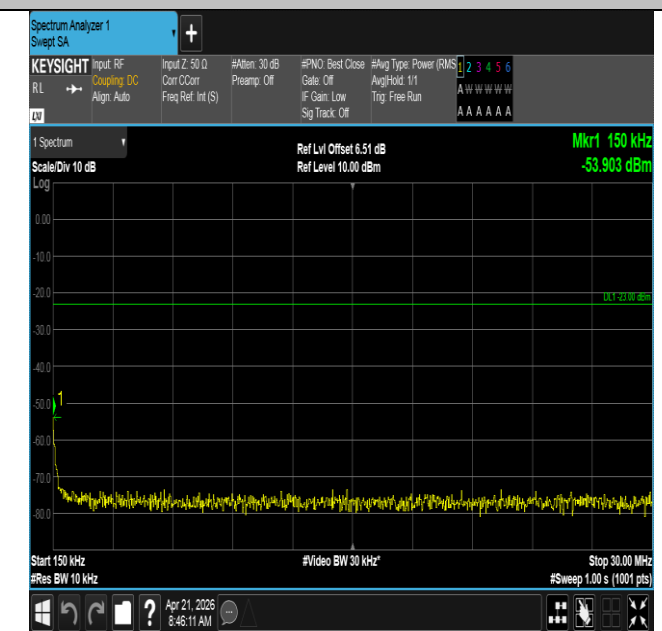
Band71-10MHz-QPSK-133297-50RB#0-0.15~30-PASS
