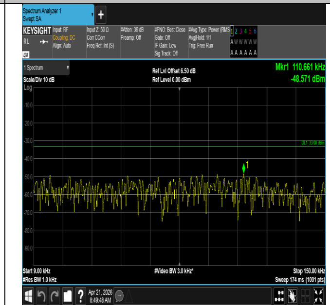
Band71-10MHz-QPSK-133422-1RB#49-0.009~0.15-PASS
