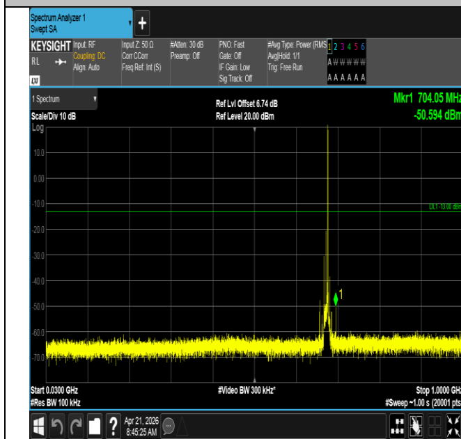
Band71-10MHz-16QAM-133297-1RB#49-30~1000-PASS
