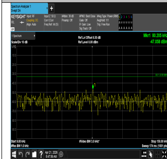
Band71-10MHz-QPSK-133422-1RB#0-0.009~0.15-PASS
