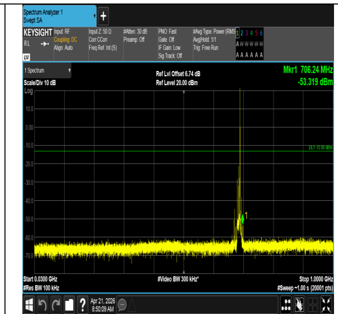
Band71-10MHz-QPSK-133422-1RB#49-30~1000-PASS
