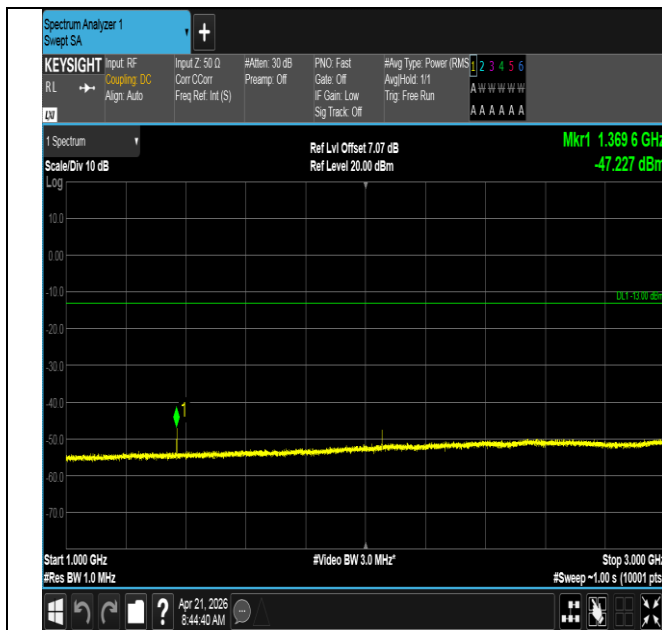
Band71-10MHz-QPSK-133297-1RB#49-1000~3000-PASS
