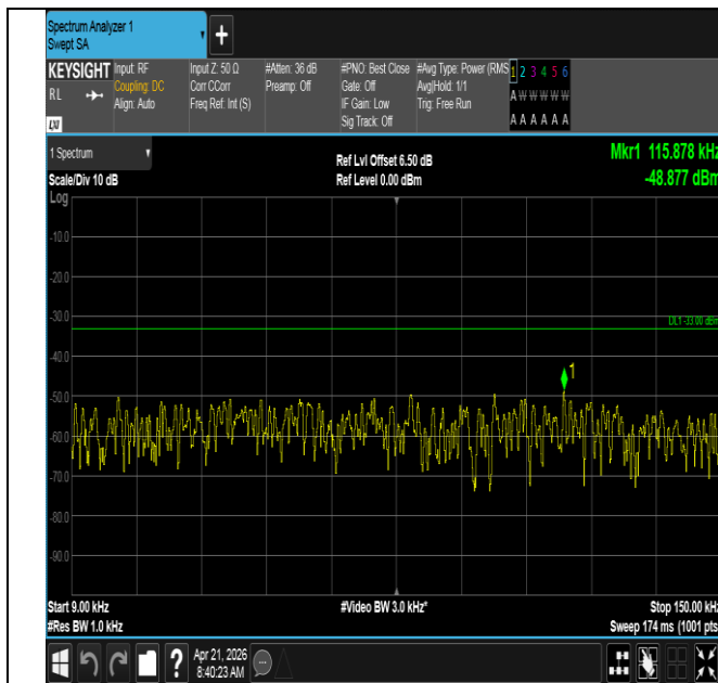
Band71-10MHz-QPSK-133172-50RB#0-0.009~0.15-PASS
