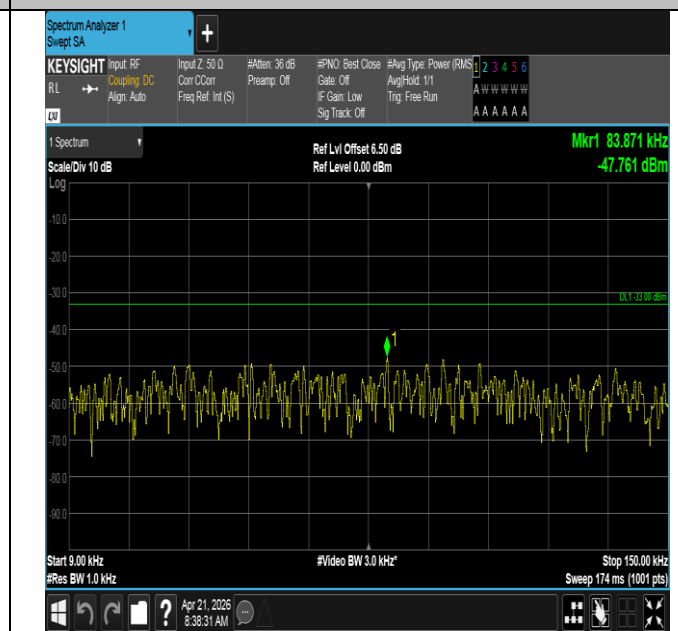
Band71-10MHz-QPSK-133172-1RB#49-0.009~0.15-PASS
