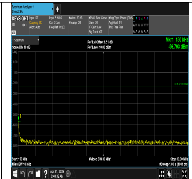
Band71-10MHz-QPSK-133172-50RB#0-0.15~30-PASS
