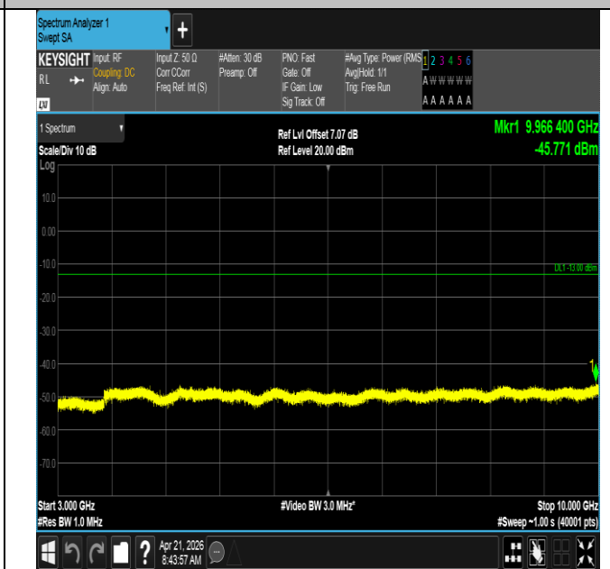
Band71-10MHz-16QAM-133297-1RB#0-3000~10000-PASS
