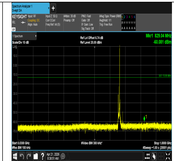
Band71-10MHz-QPSK-133172-1RB#49-30~1000-PASS
