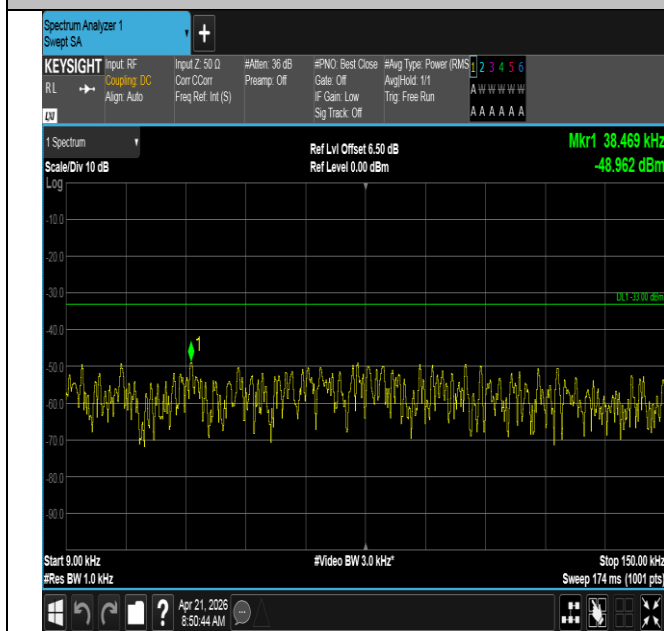
Band71-10MHz-16QAM-133422-1RB#49-0.009~0.15-PASS
