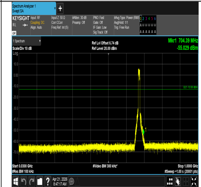
Band71-10MHz-16QAM-133297-50RB#0-30~1000-PASS
