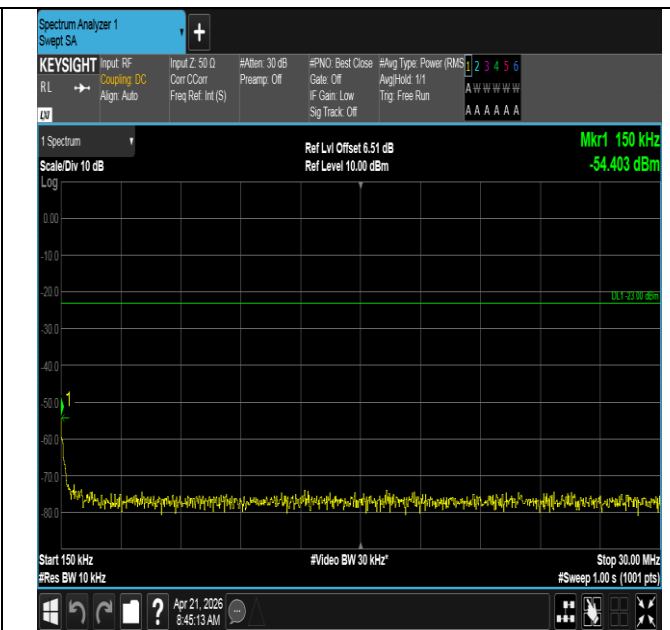
Band71-10MHz-16QAM-133297-1RB#49-0.15~30-PASS
