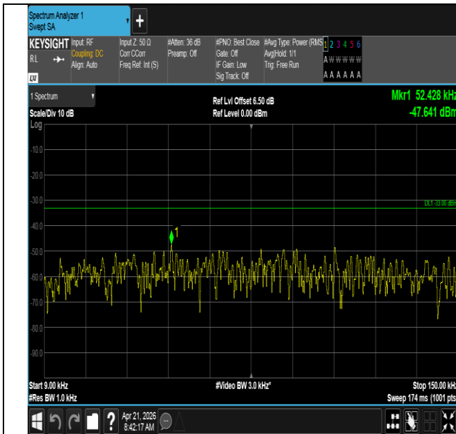
Band71-10MHz-QPSK-133297-1RB#0-0.009~0.15-PASS
