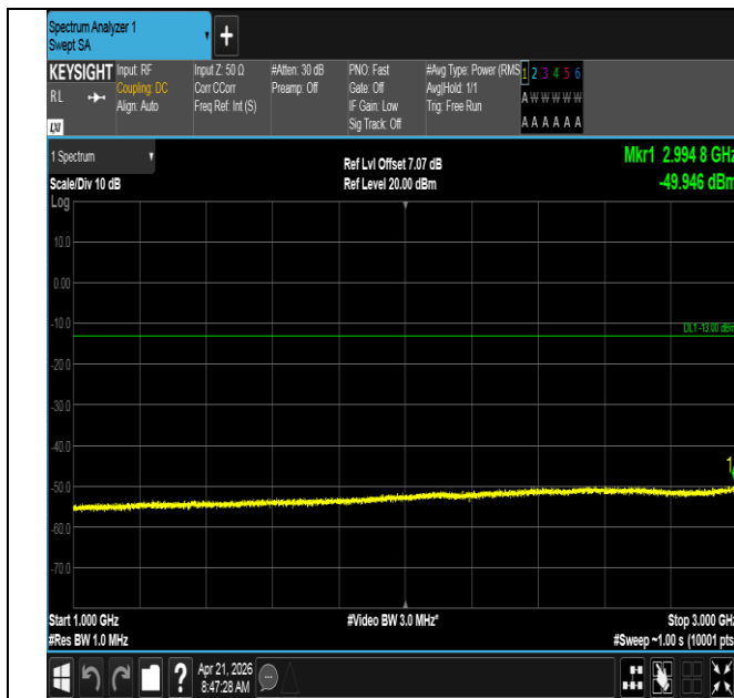
Band71-10MHz-16QAM-133297-50RB#0-1000~3000-PASS
