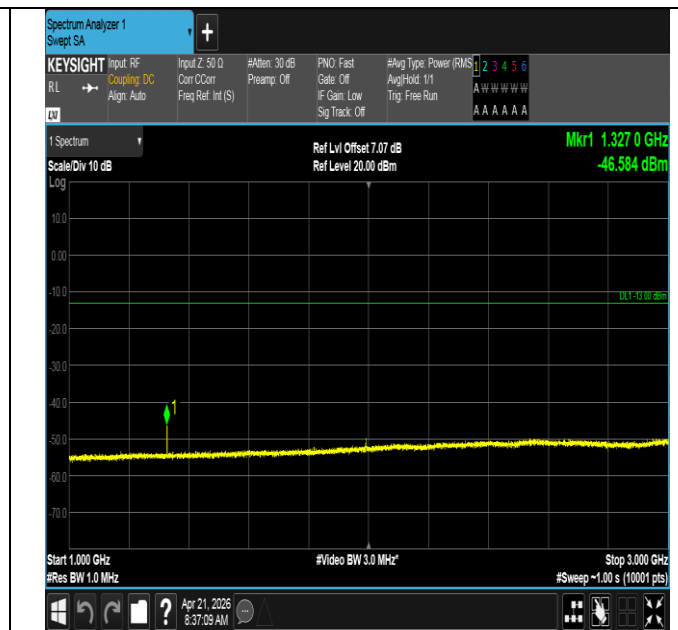
Band71-10MHz-QPSK-133172-1RB#0-1000~3000-PASS
