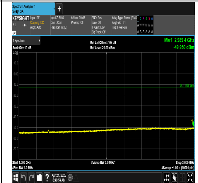
Band71-10MHz-QPSK-133172-50RB#0-1000~3000-PASS
