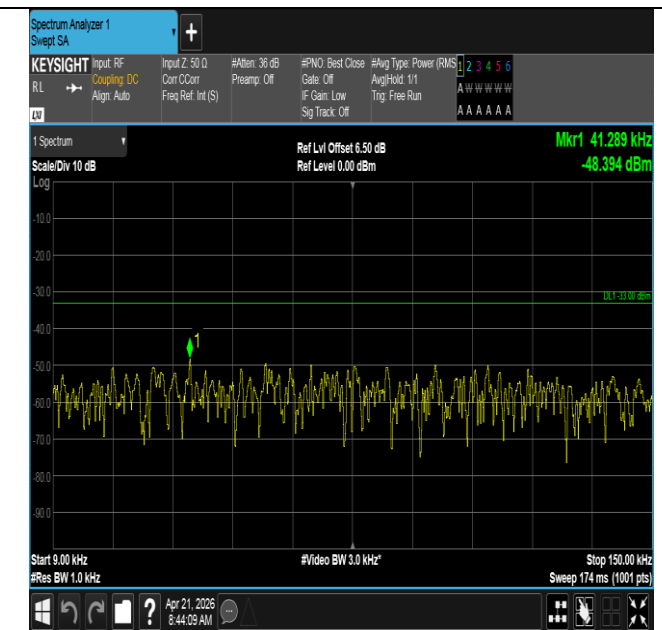
Band71-10MHz-QPSK-133297-1RB#49-0.009~0.15-PASS
