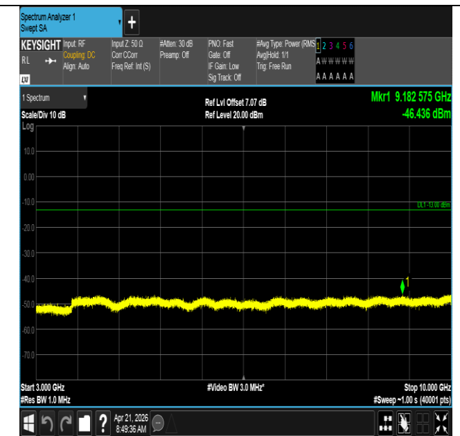
Band71-10MHz-16QAM-133422-1RB#0-3000~10000-PASS
