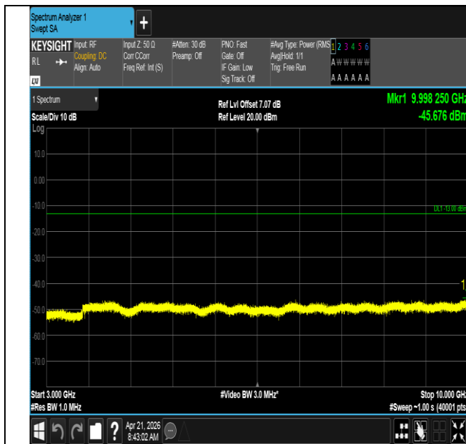
Band71-10MHz-QPSK-133297-1RB#0-3000~10000-PASS
