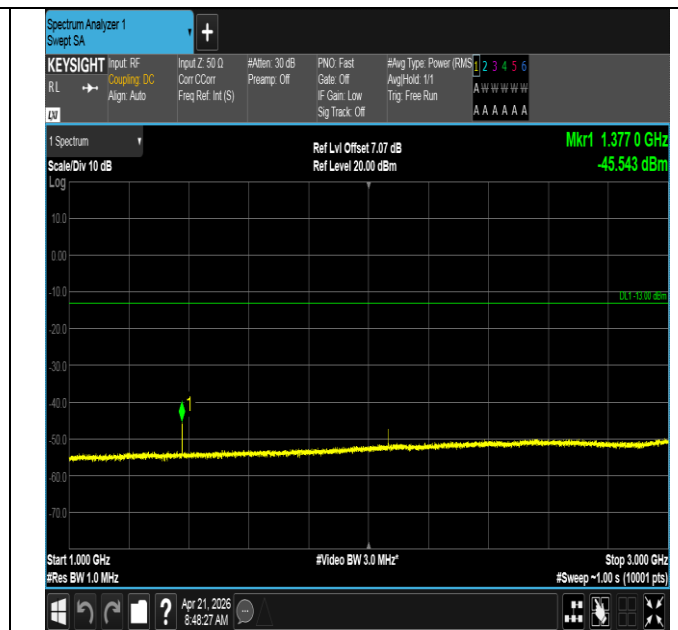
Band71-10MHz-QPSK-133422-1RB#0-1000~3000-PASS
