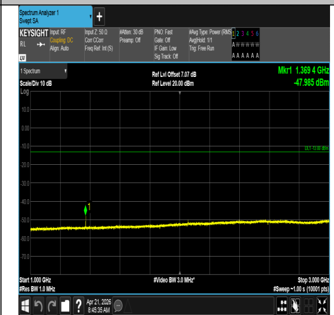
Band71-10MHz-16QAM-133297-1RB#49-1000~3000-PASS
