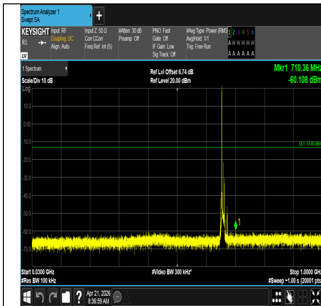
Band71-10MHz-QPSK-133172-1RB#0-30~1000-PASS
