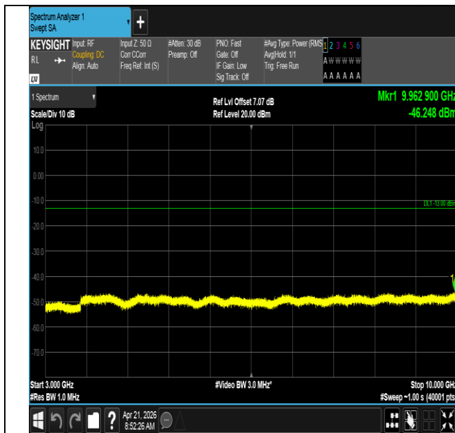
Band71-10MHz-QPSK-133422-50RB#0-3000~10000-PASS
