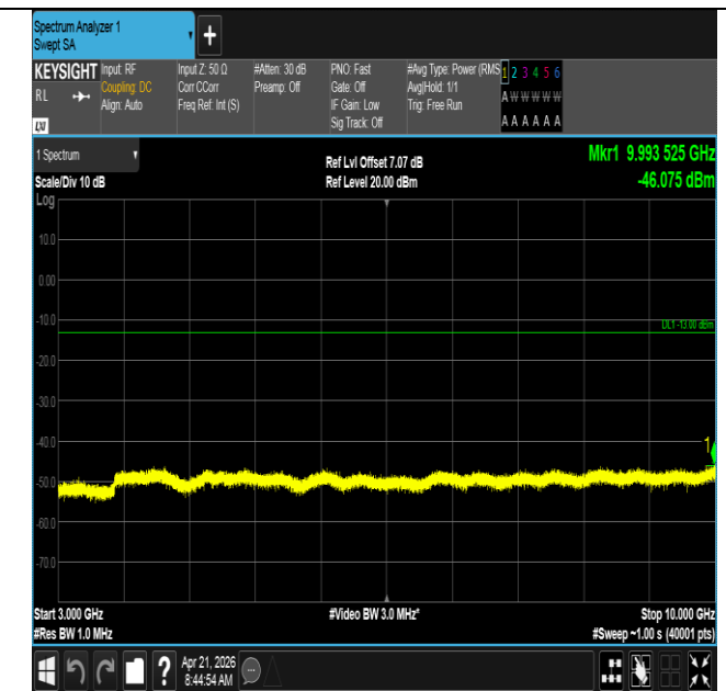
Band71-10MHz-QPSK-133297-1RB#49-3000~10000-PASS
