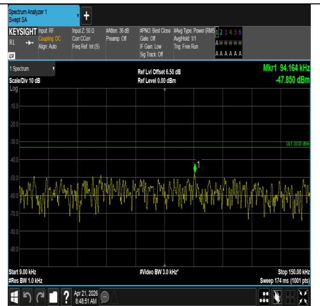
Band71-10MHz-16QAM-133422-1RB#0-0.009~0.15-PASS
