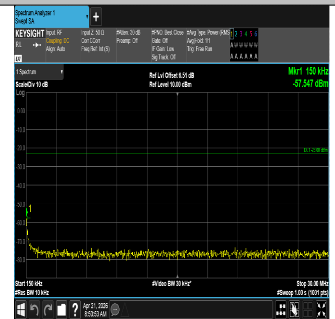
Band71-10MHz-16QAM-133422-1RB#49-0.15~30-PASS
