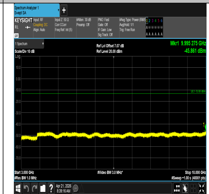
Band71-10MHz-QPSK-133172-1RB#49-3000~10000-PASS
