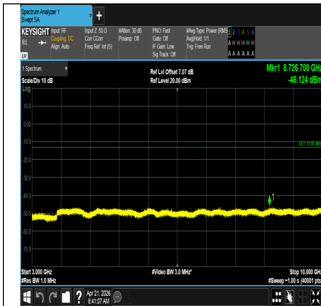
Band71-10MHz-QPSK-133172-50RB#0-3000~10000-PASS
