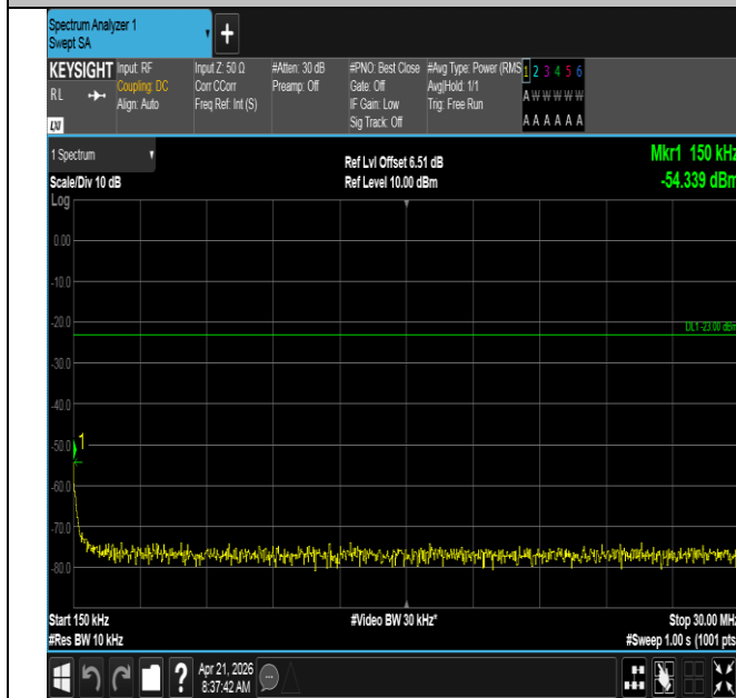
Band71-10MHz-16QAM-133172-1RB#0-0.15~30-PASS
