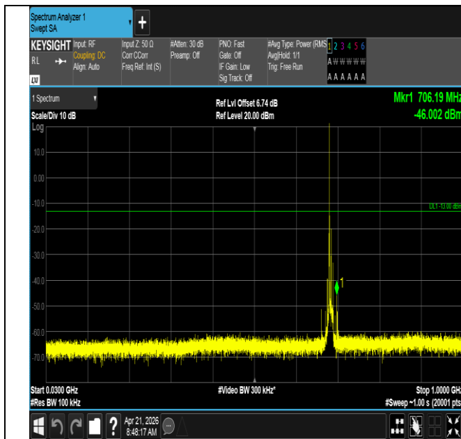
Band71-10MHz-QPSK-133422-1RB#0-30~1000-PASS
