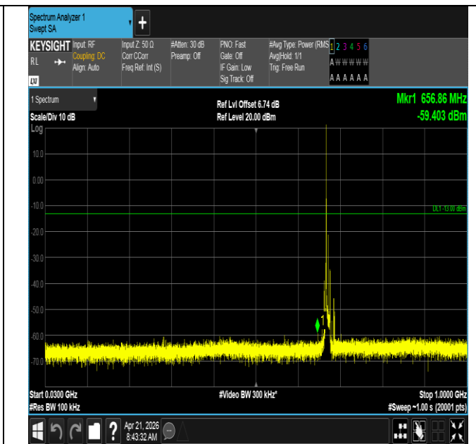
Band71-10MHz-16QAM-133297-1RB#0-30~1000-PASS
