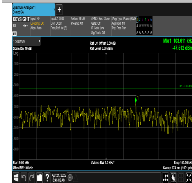
Band71-10MHz-QPSK-133297-50RB#0-0.009~0.15-PASS
