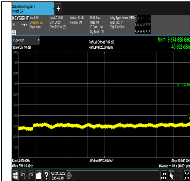
Band71-10MHz-16QAM-133297-1RB#49-3000~10000-PASS
