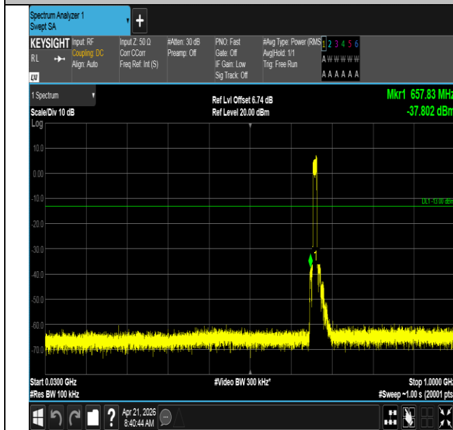
Band71-10MHz-QPSK-133172-50RB#0-30~1000-PASS
