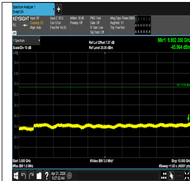
Band71-15MHz-QPSK-133197-1RB#0-3000~10000-PASS
