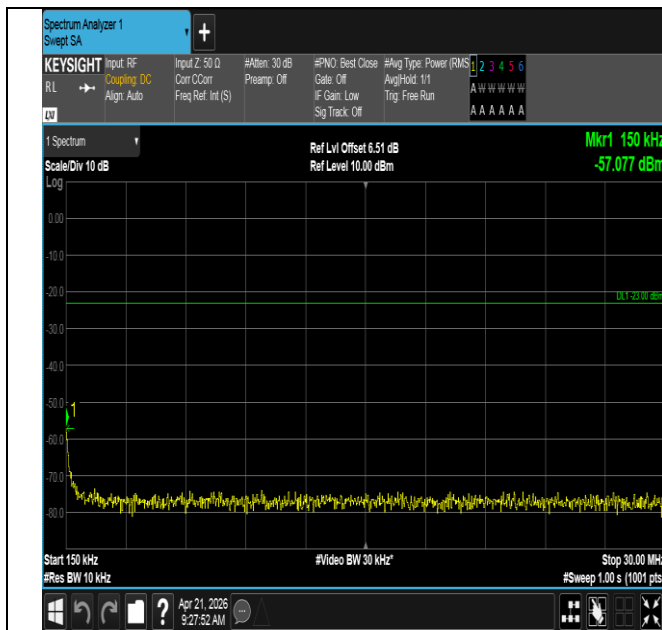
Band71-15MHz-16QAM-133197-1RB#0-0.15~30-PASS
