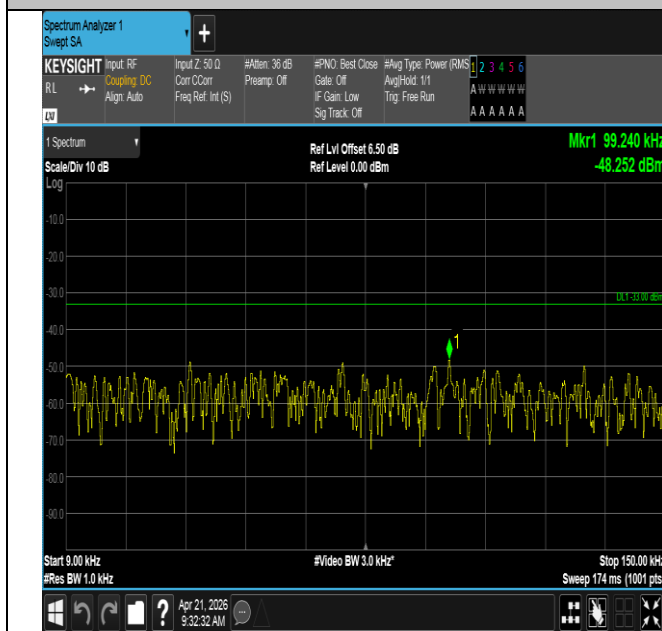
Band71-15MHz-QPSK-133297-1RB#0-0.009~0.15-PASS
