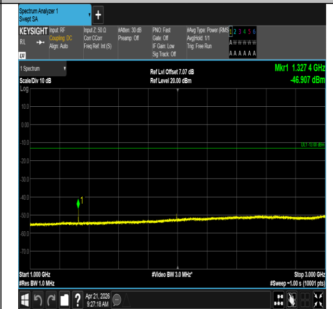
Band71-15MHz-QPSK-133197-1RB#0-1000~3000-PASS
