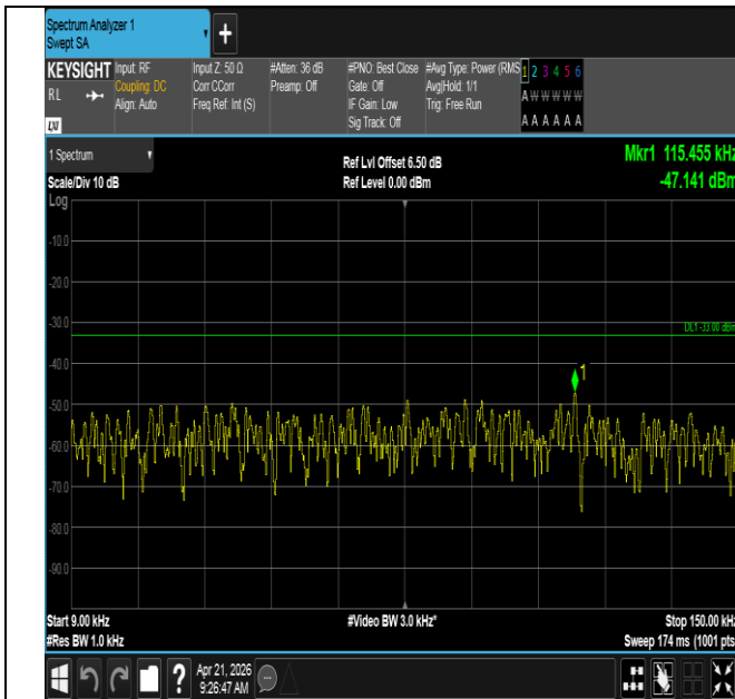
Band71-15MHz-QPSK-133197-1RB#0-0.009~0.15-PASS
