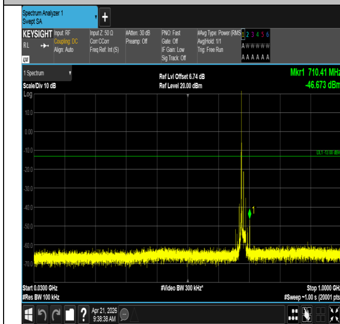
Band71-15MHz-QPSK-133397-1RB#0-30~1000-PASS
