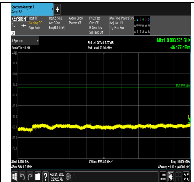
Band71-15MHz-QPSK-133197-1RB#74-3000~10000-PASS
