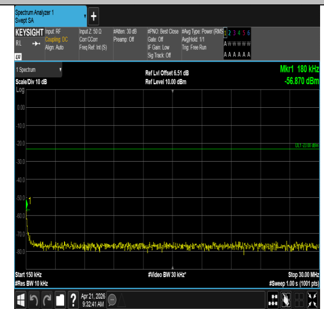
Band71-15MHz-QPSK-133297-1RB#0-0.15~30-PASS
