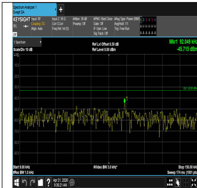
Band71-15MHz-QPSK-133297-75RB#0-0.009~0.15-PASS
