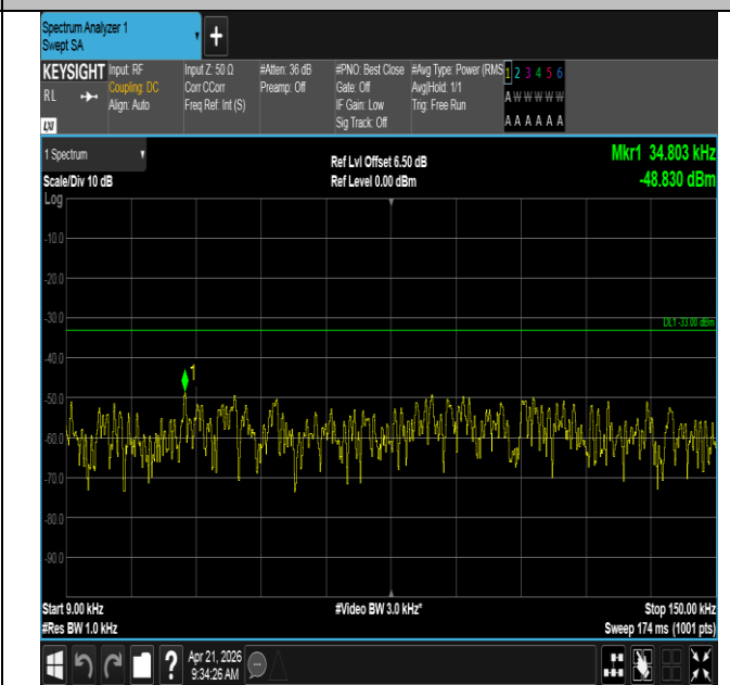
Band71-15MHz-QPSK-133297-1RB#74-0.009~0.15-PASS
