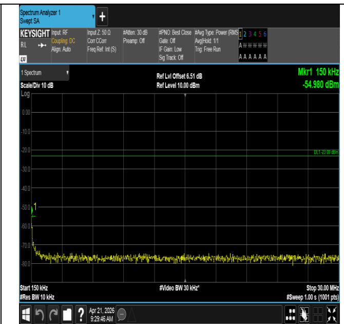
Band71-15MHz-16QAM-133197-1RB#74-0.15~30-PASS
