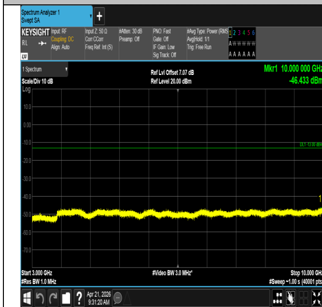
Band71-15MHz-QPSK-133197-75RB#0-3000~10000-PASS
