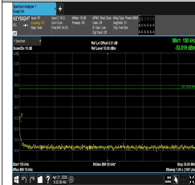
Band71-15MHz-16QAM-133297-1RB#0-0.15~30-PASS
