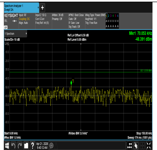
Band71-15MHz-QPSK-133397-1RB#74-0.009~0.15-PASS
