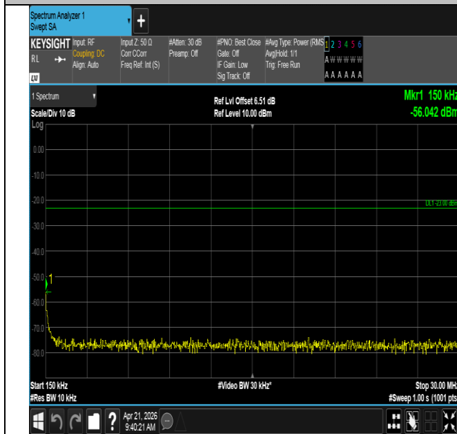
Band71-15MHz-QPSK-133397-1RB#74-0.15~30-PASS
