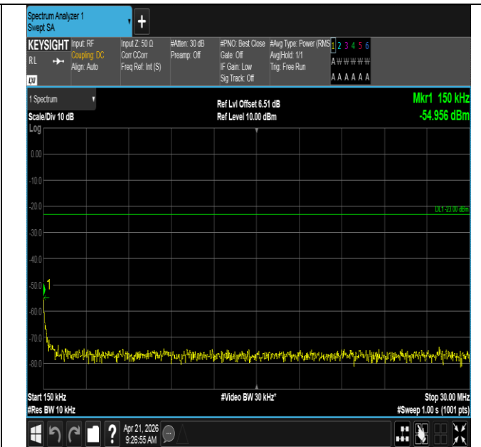
Band71-15MHz-QPSK-133197-1RB#0-0.15~30-PASS
