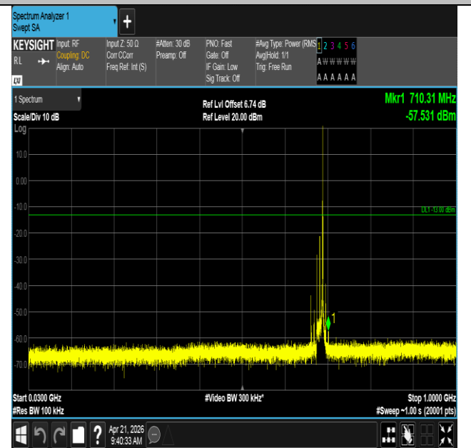
Band71-15MHz-QPSK-133397-1RB#74-30~1000-PASS
