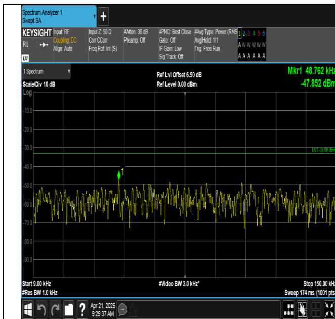
Band71-15MHz-16QAM-133197-1RB#74-0.009~0.15-PASS
