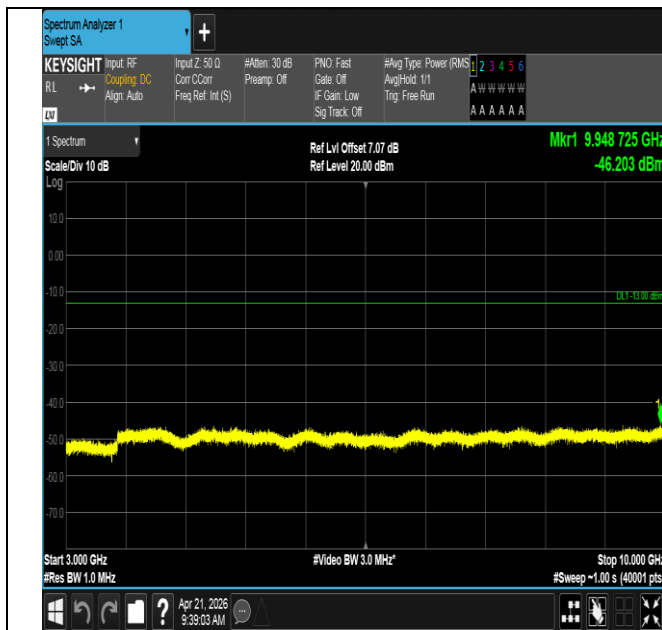
Band71-15MHz-QPSK-133397-1RB#0-3000~10000-PASS
