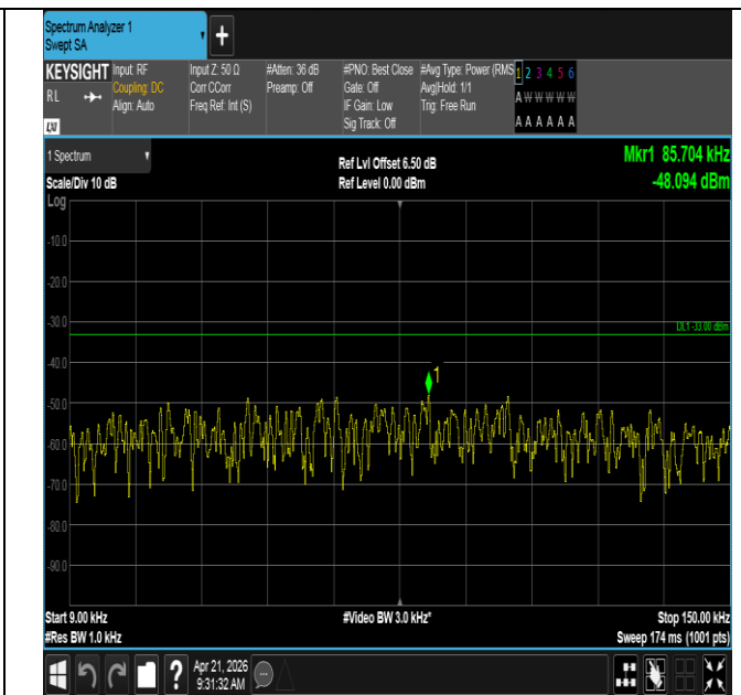
Band71-15MHz-16QAM-133197-75RB#0-0.009~0.15-PASS
