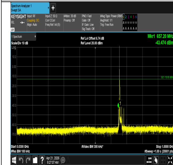
Band71-15MHz-QPSK-133197-1RB#0-30~1000-PASS
