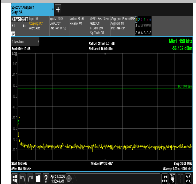
Band71-15MHz-QPSK-133197-75RB#0-0.15~30-PASS
