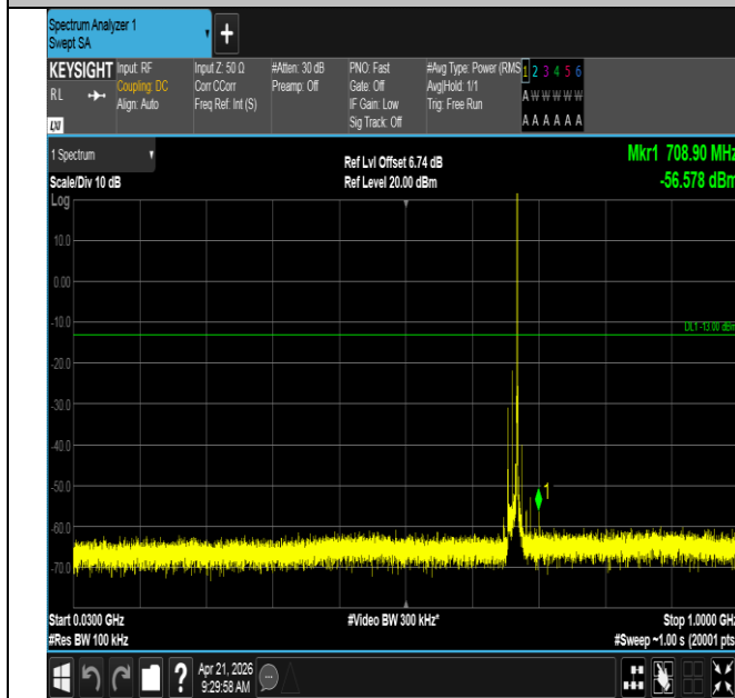
Band71-15MHz-16QAM-133197-1RB#74-30~1000-PASS
