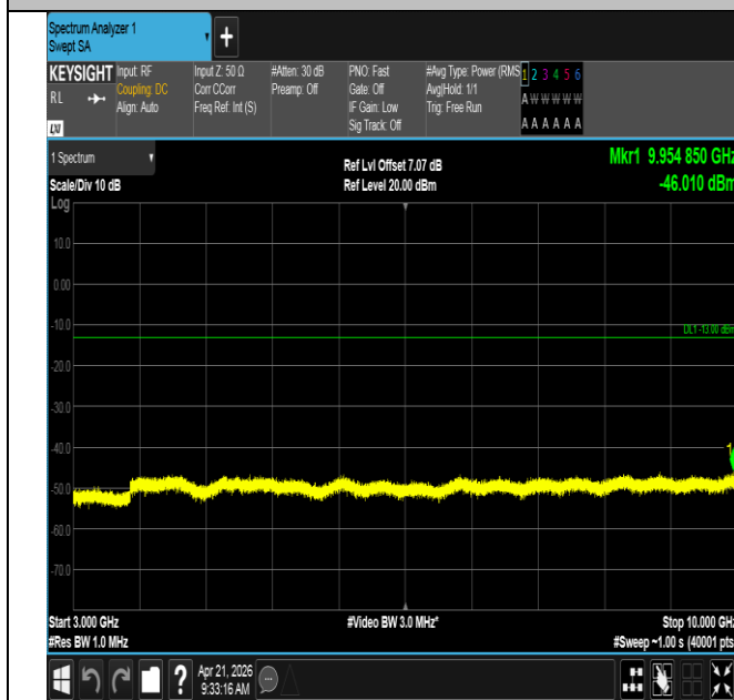
Band71-15MHz-QPSK-133297-1RB#0-3000~10000-PASS
