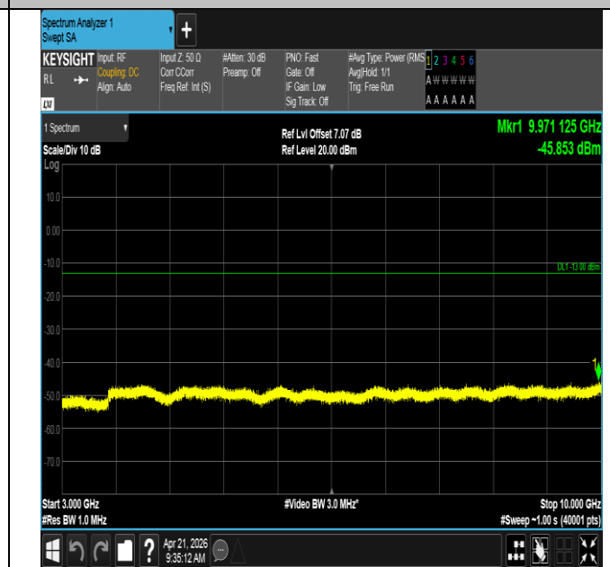
Band71-15MHz-QPSK-133297-1RB#74-3000~10000-PASS
