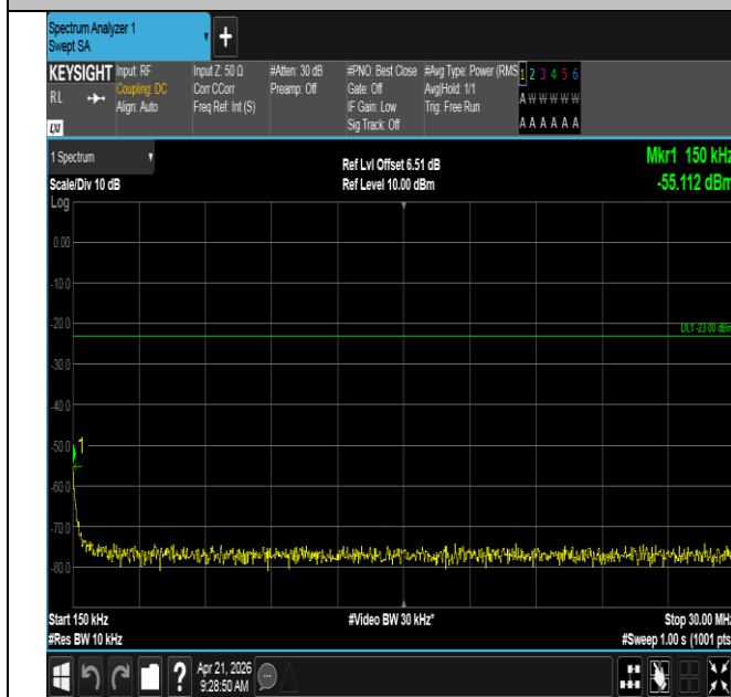
Band71-15MHz-QPSK-133197-1RB#74-0.15~30-PASS
