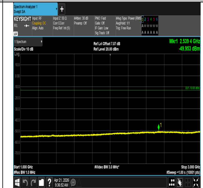
Band71-15MHz-QPSK-133297-75RB#0-1000~3000-PASS
