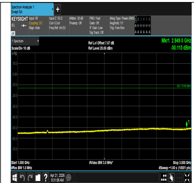
Band71-15MHz-QPSK-133197-75RB#0-1000~3000-PASS
