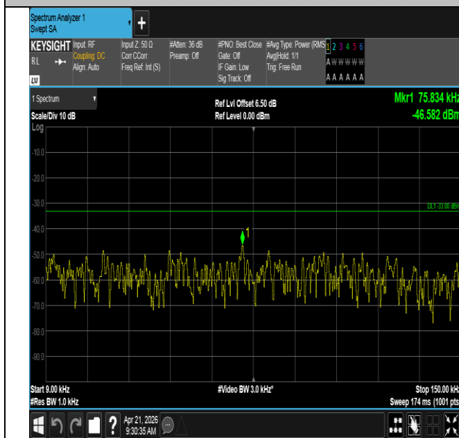
Band71-15MHz-QPSK-133197-75RB#0-0.009~0.15-PASS
