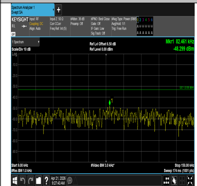
Band71-15MHz-16QAM-133197-1RB#0-0.009~0.15-PASS
