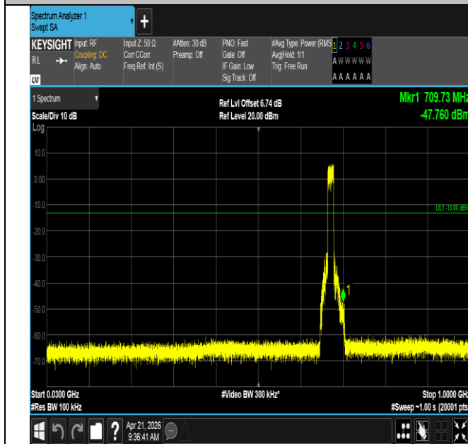
Band71-15MHz-QPSK-133297-75RB#0-30~1000-PASS
