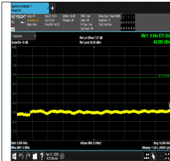
Band71-15MHz-QPSK-133297-75RB#0-3000~10000-PASS
