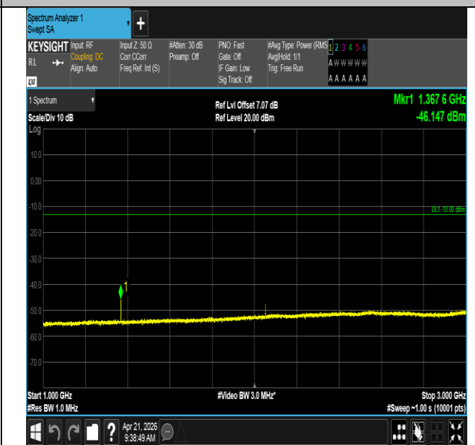
Band71-15MHz-QPSK-133397-1RB#0-1000~3000-PASS
