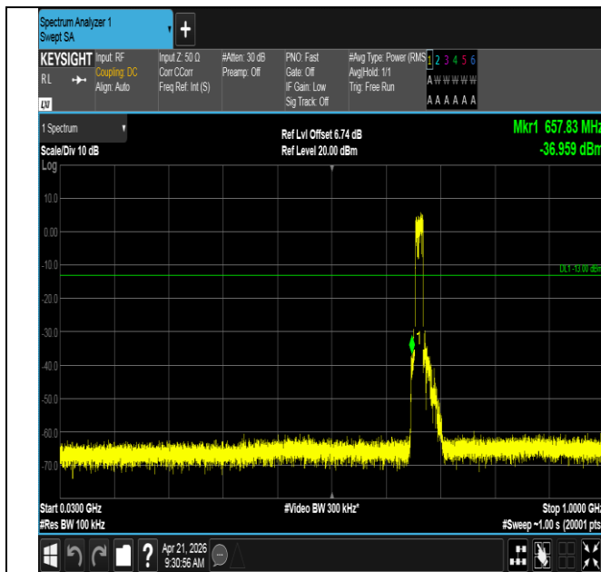
Band71-15MHz-QPSK-133197-75RB#0-30~1000-PASS
