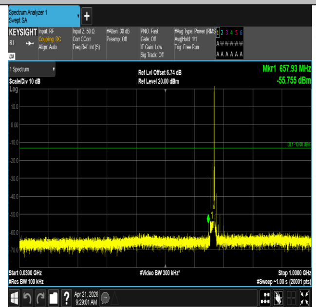
Band71-15MHz-QPSK-133197-1RB#74-30~1000-PASS
