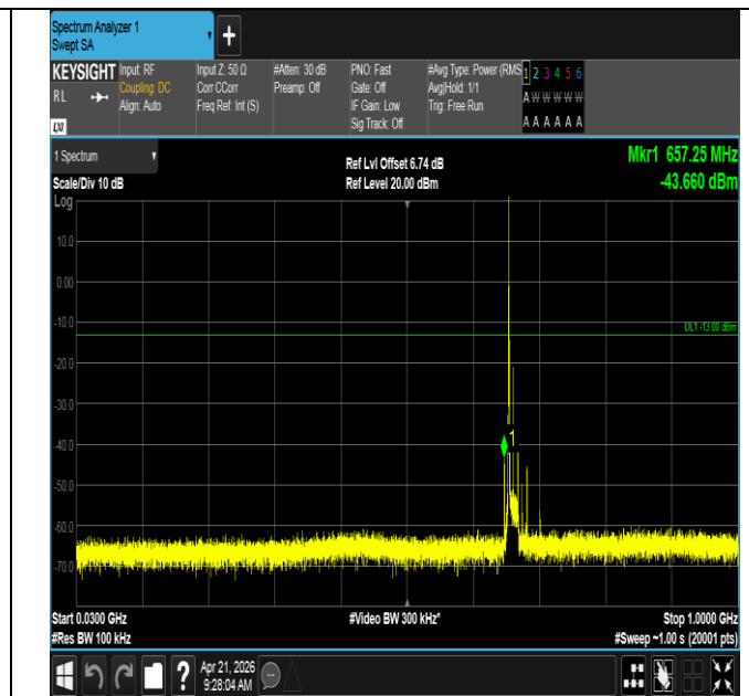
Band71-15MHz-16QAM-133197-1RB#0-30~1000-PASS
