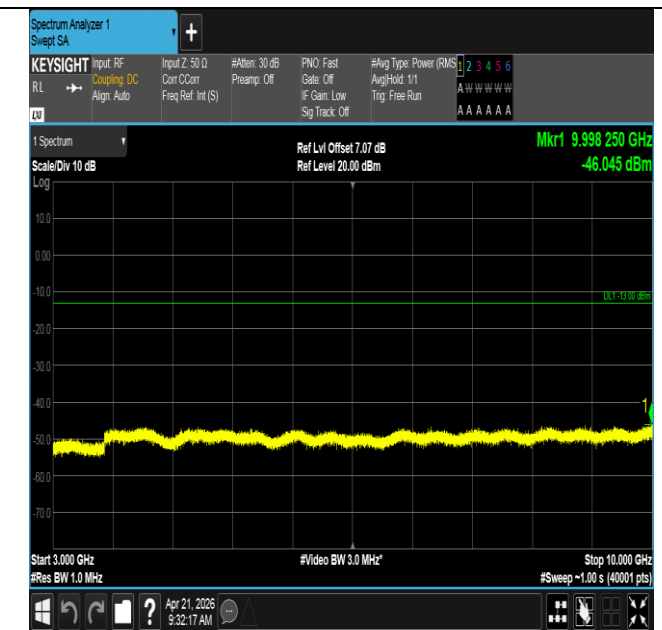
Band71-15MHz-16QAM-133197-75RB#0-3000~10000-PASS
