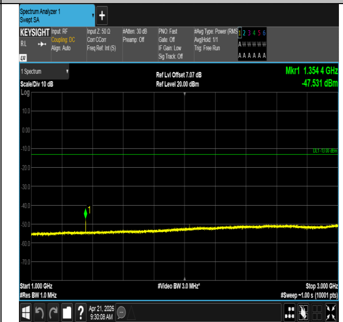
Band71-15MHz-16QAM-133197-1RB#74-1000~3000-PASS
