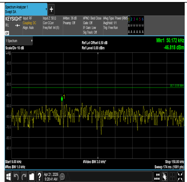
Band71-15MHz-QPSK-133197-1RB#74-0.009~0.15-PASS
