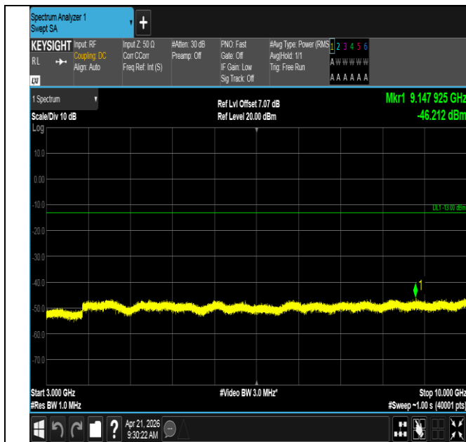
Band71-15MHz-16QAM-133197-1RB#74-3000~10000-PASS
