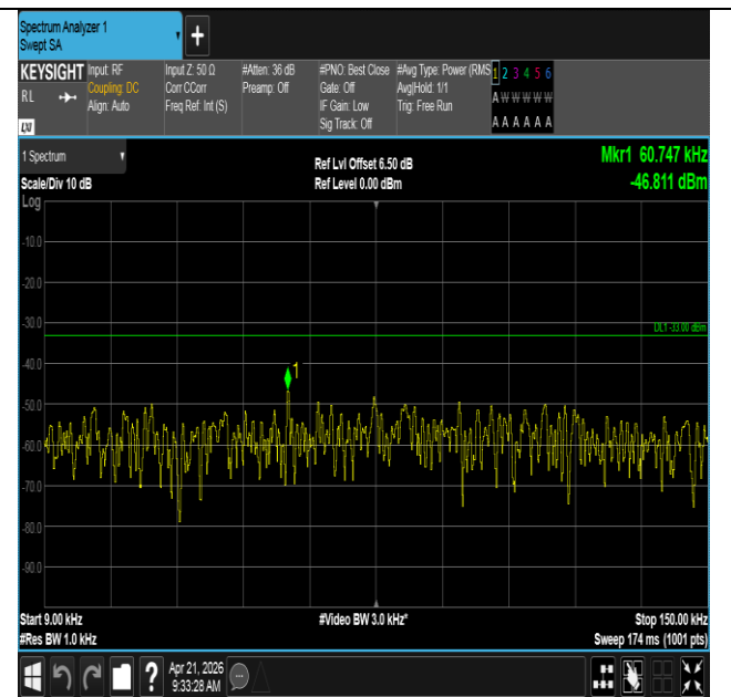
Band71-15MHz-16QAM-133297-1RB#0-0.009~0.15-PASS
