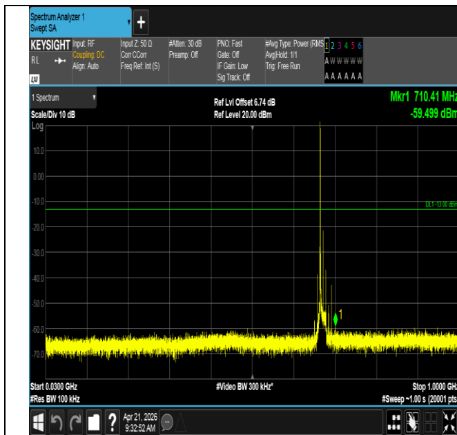
Band71-15MHz-QPSK-133297-1RB#0-30~1000-PASS
