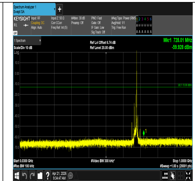
Band71-15MHz-QPSK-133297-1RB#74-30~1000-PASS
