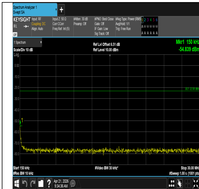
Band71-15MHz-QPSK-133297-1RB#74-0.15~30-PASS
