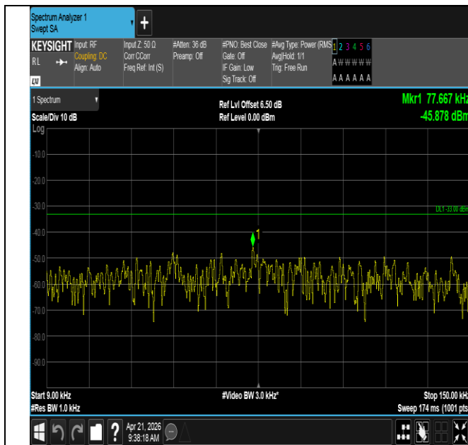
Band71-15MHz-QPSK-133397-1RB#0-0.009~0.15-PASS
