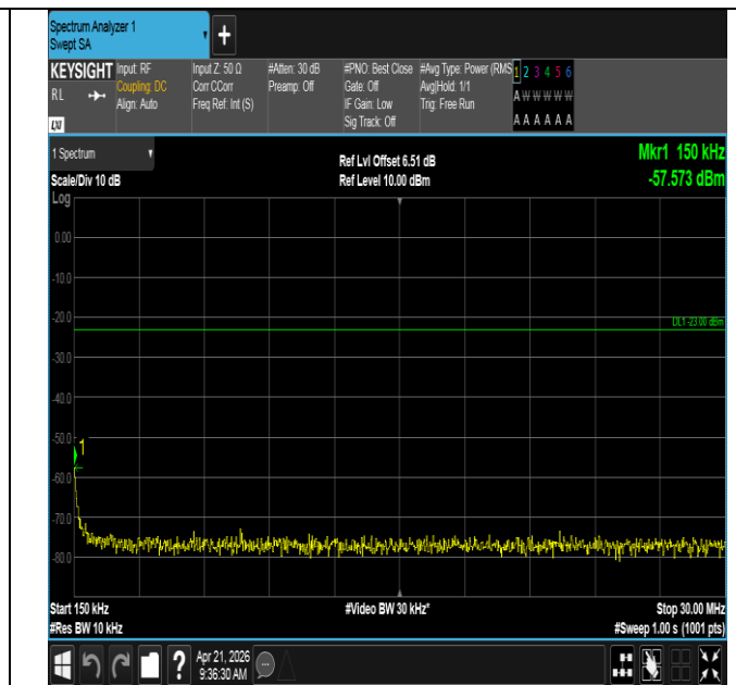
Band71-15MHz-QPSK-133297-75RB#0-0.15~30-PASS
