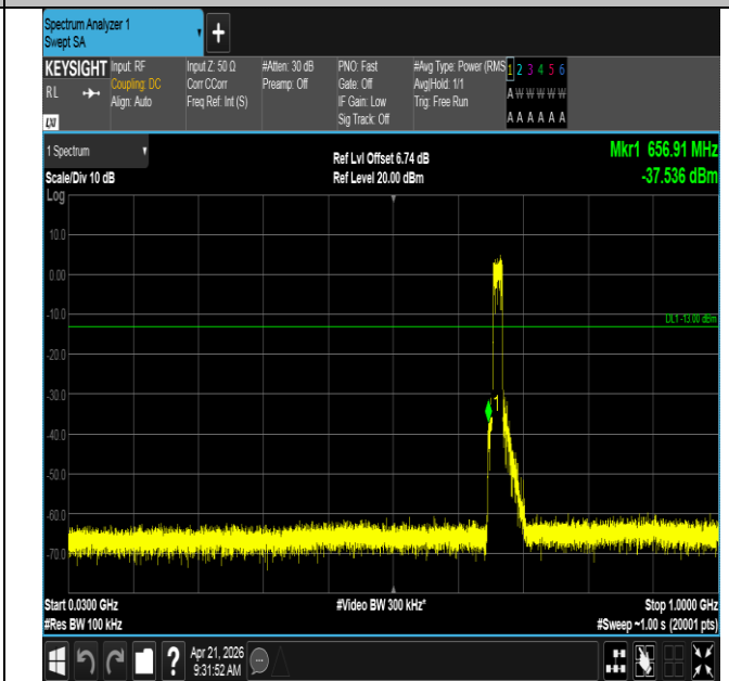
Band71-15MHz-16QAM-133197-75RB#0-30~1000-PASS
