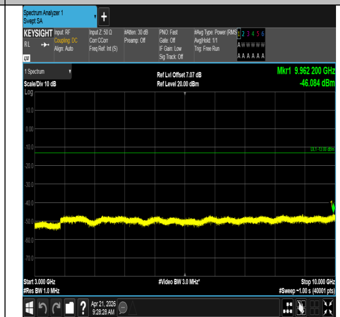
Band71-15MHz-16QAM-133197-1RB#0-3000~10000-PASS
