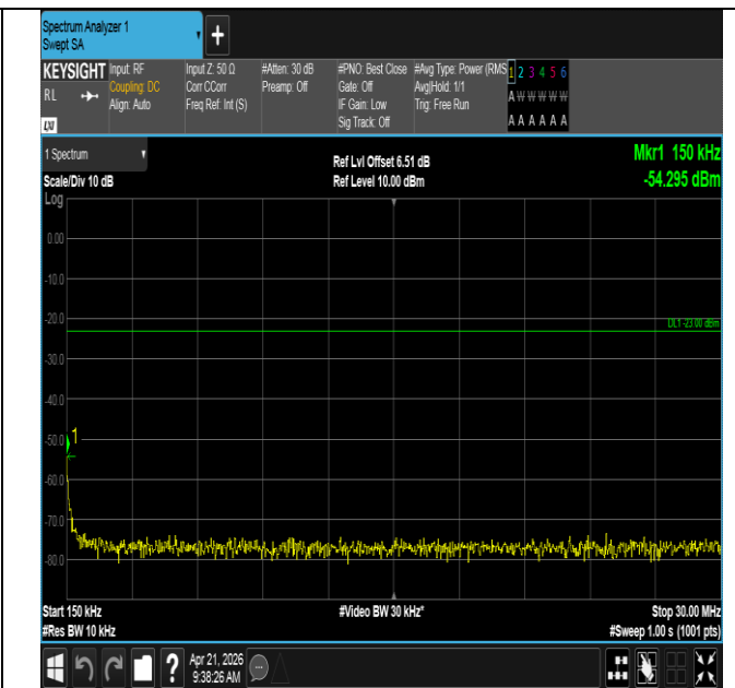
Band71-15MHz-QPSK-133397-1RB#0-0.15~30-PASS
