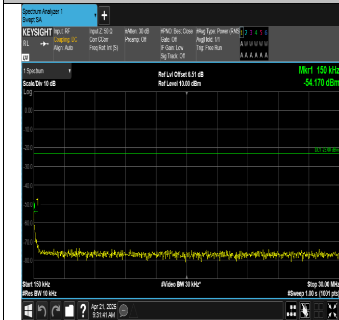
Band71-15MHz-16QAM-133197-75RB#0-0.15~30-PASS
