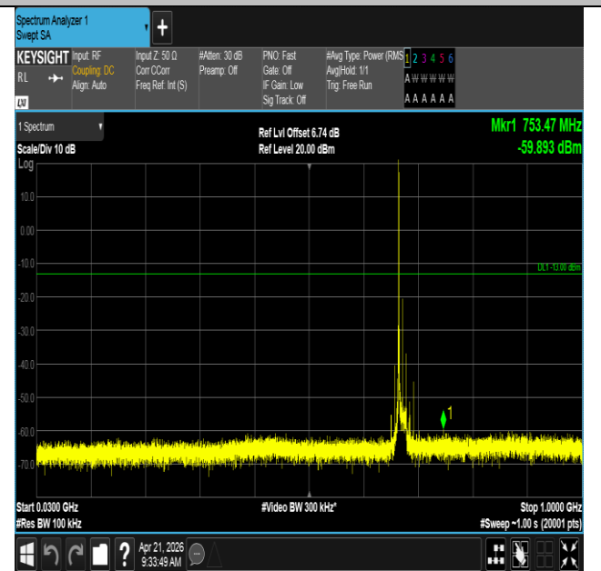
Band71-15MHz-16QAM-133297-1RB#0-30~1000-PASS
