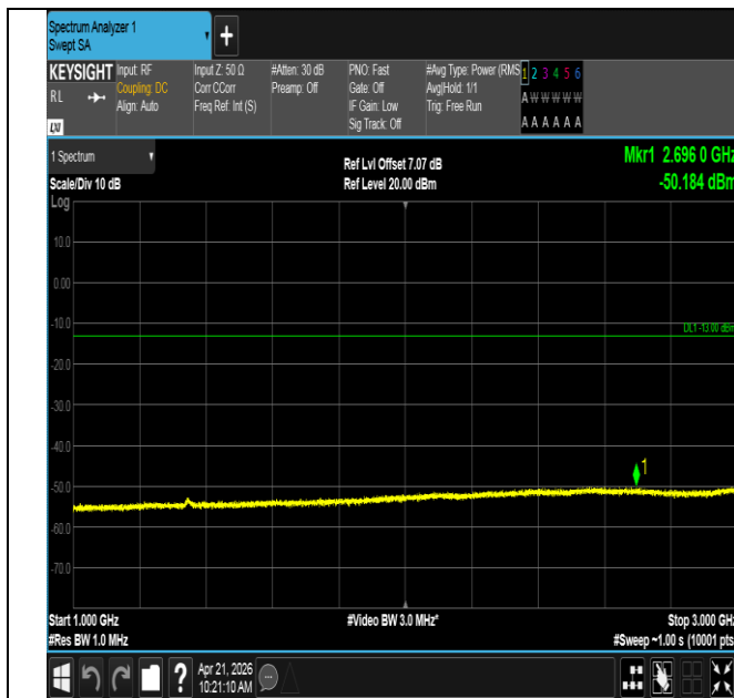
Band71-20MHz-16QAM-133222-100RB#0-1000~3000-PASS
