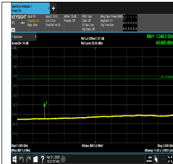
Band71-20MHz-QPSK-133322-1RB#0-1000~3000-PASS
