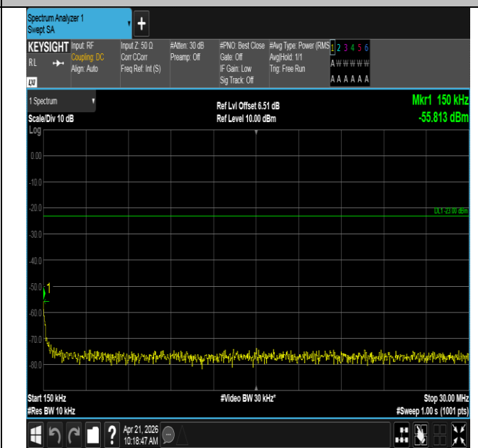
Band71-20MHz-QPSK-133222-1RB#99-0.15~30-PASS
