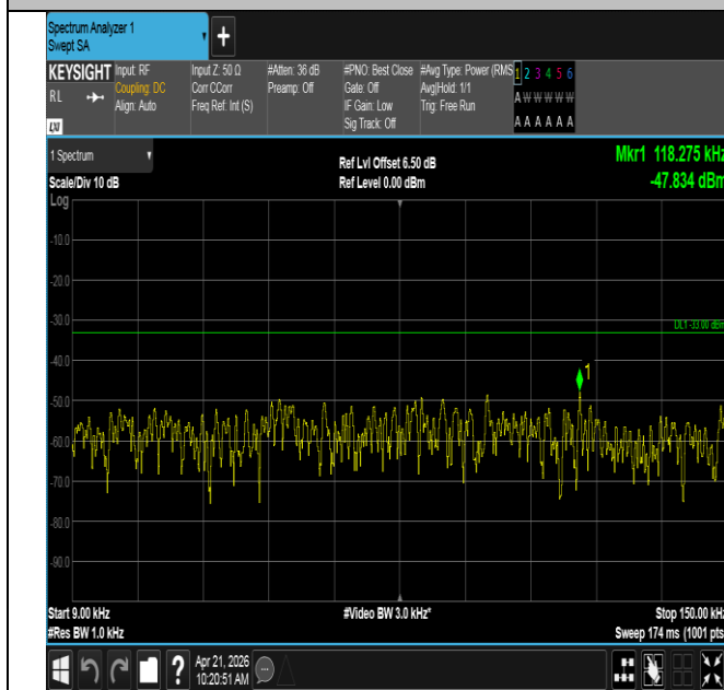
Band71-20MHz-16QAM-133222-100RB#0-0.009~0.15-PASS
