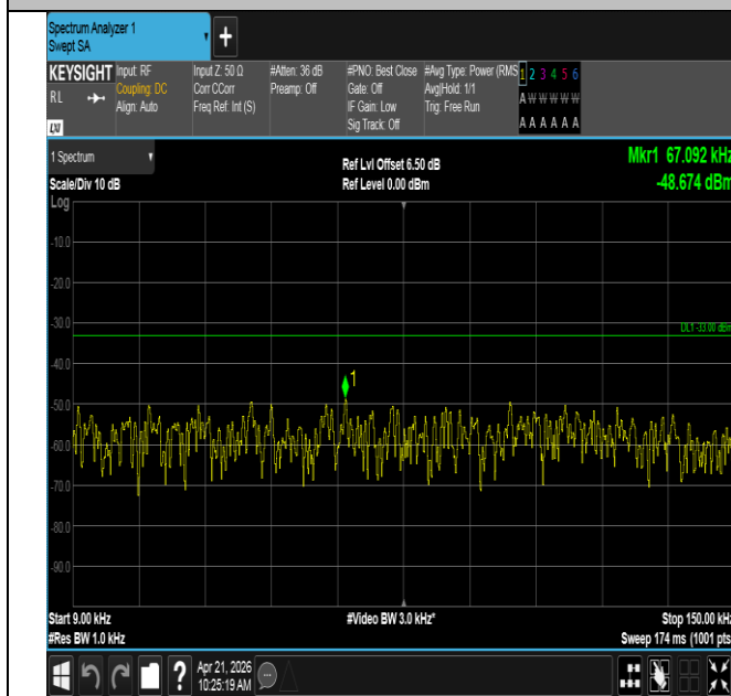
Band71-20MHz-16QAM-133322-100RB#0-0.009~0.15-PASS
