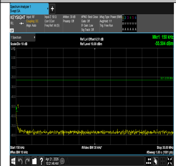
Band71-20MHz-QPSK-133322-1RB#0-0.15~30-PASS
