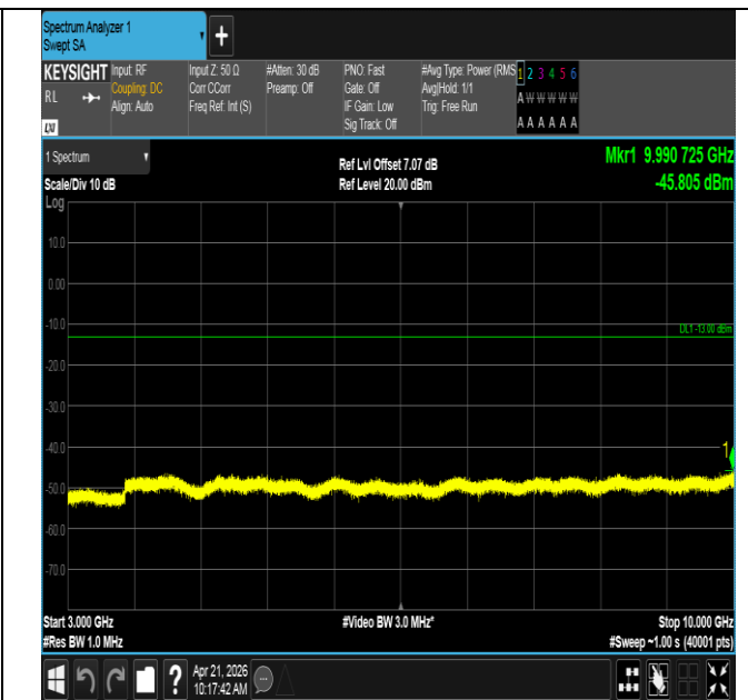
Band71-20MHz-QPSK-133222-1RB#0-3000~10000-PASS
