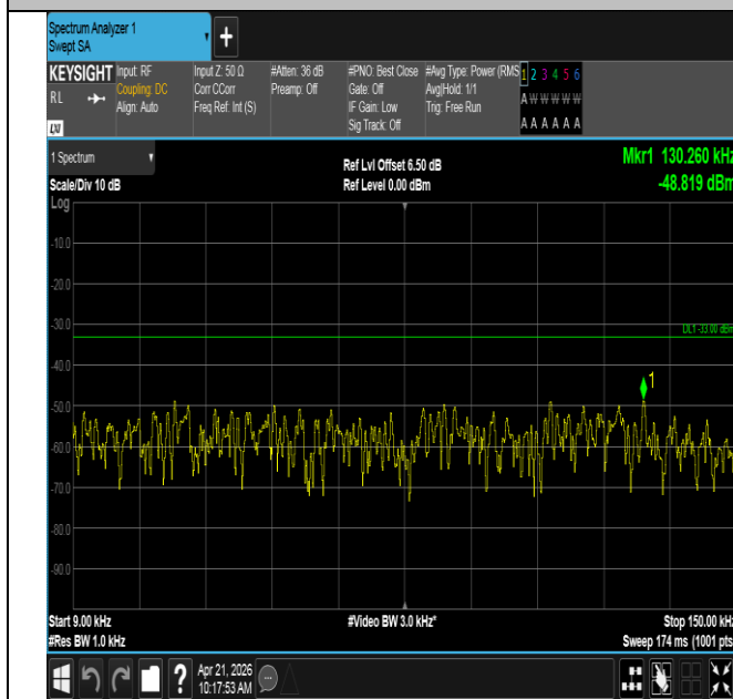
Band71-20MHz-16QAM-133222-1RB#0-0.009~0.15-PASS
