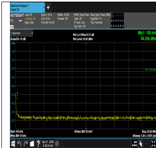
Band71-15MHz-16QAM-133397-1RB#0-0.15~30-PASS
