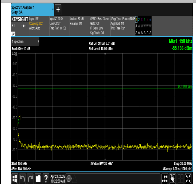
Band71-20MHz-16QAM-133322-1RB#0-0.15~30-PASS
