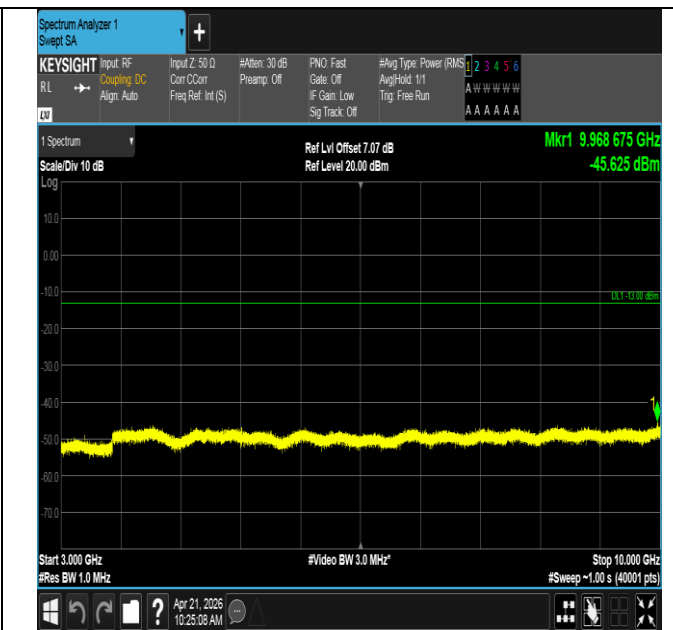
Band71-20MHz-QPSK-133322-100RB#0-3000~10000-PASS
