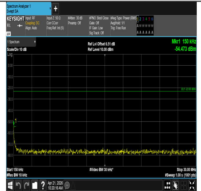
Band71-20MHz-QPSK-133222-100RB#0-0.15~30-PASS
