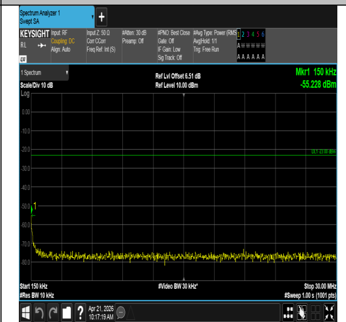
Band71-20MHz-QPSK-133222-1RB#0-0.15~30-PASS
