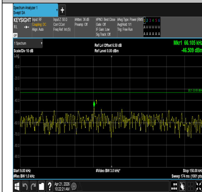
Band71-20MHz-16QAM-133322-1RB#0-0.009~0.15-PASS
