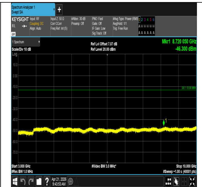
Band71-15MHz-16QAM-133397-75RB#0-3000~10000-PASS
