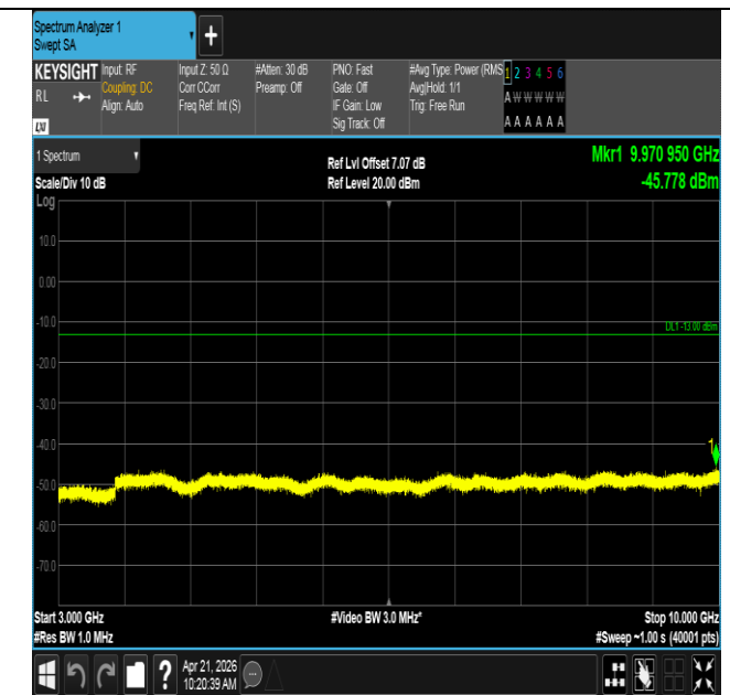
Band71-20MHz-QPSK-133222-100RB#0-3000~10000-PASS
