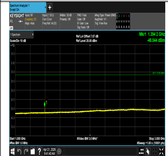
Band71-15MHz-16QAM-133397-1RB#74-1000~3000-PASS
