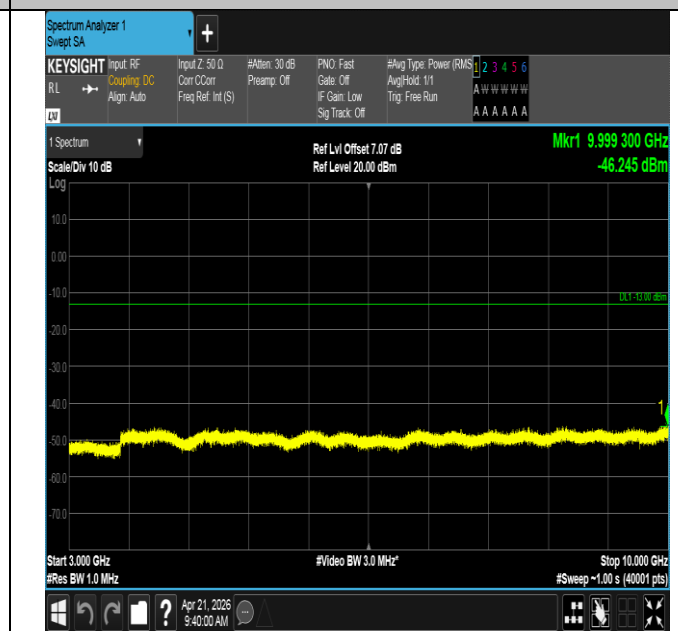
Band71-15MHz-16QAM-133397-1RB#0-3000~10000-PASS
