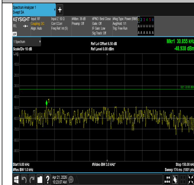
Band71-20MHz-QPSK-133322-1RB#99-0.009~0.15-PASS
