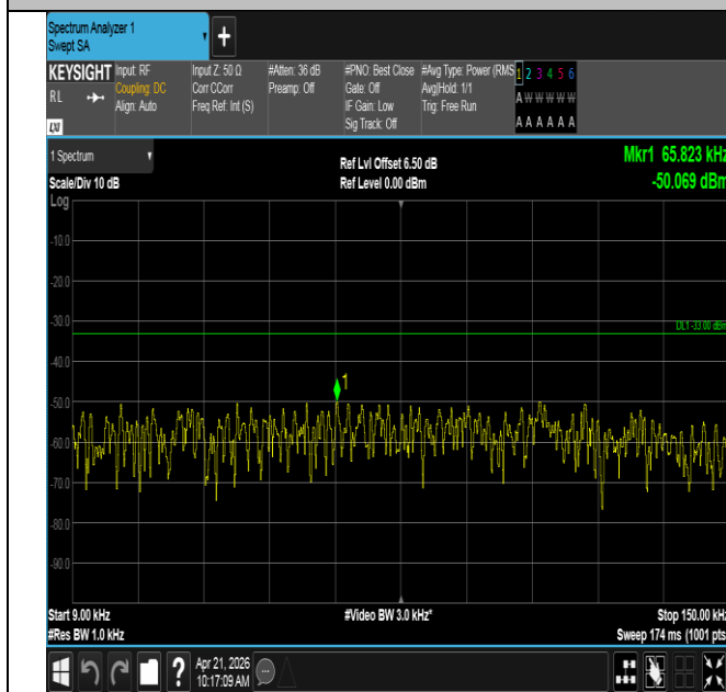
Band71-20MHz-QPSK-133222-1RB#0-0.009~0.15-PASS
