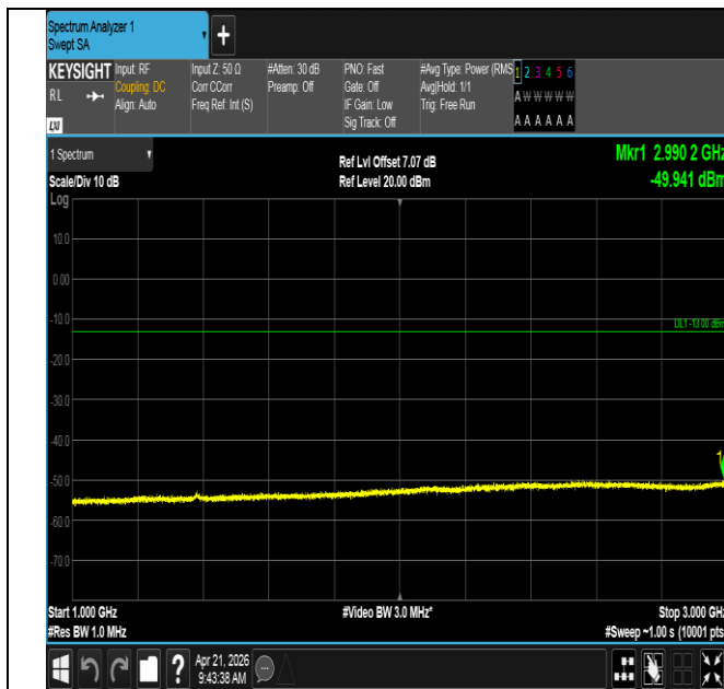
Band71-15MHz-16QAM-133397-75RB#0-1000~3000-PASS
