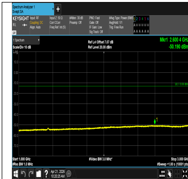
Band71-20MHz-QPSK-133222-100RB#0-1000~3000-PASS
