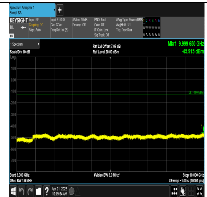
Band71-20MHz-16QAM-133222-1RB#99-3000~10000-PASS
