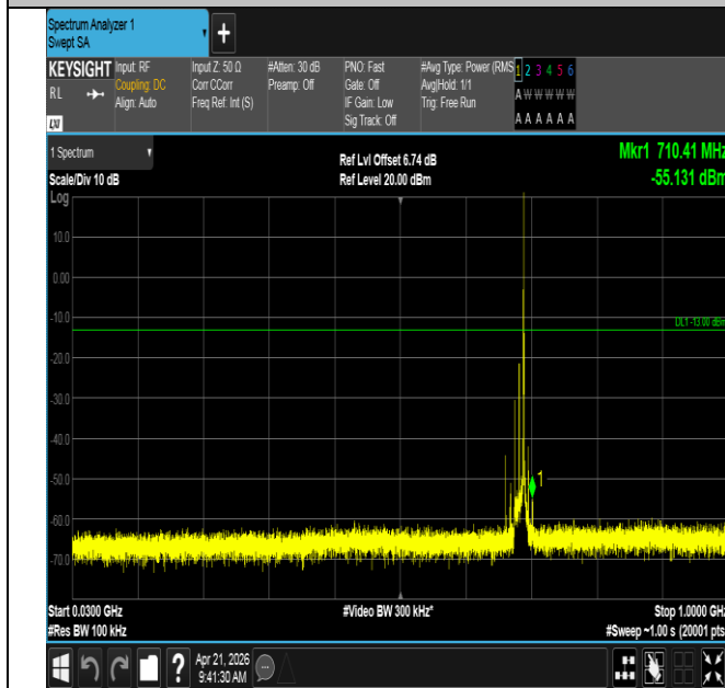
Band71-15MHz-16QAM-133397-1RB#74-30~1000-PASS
