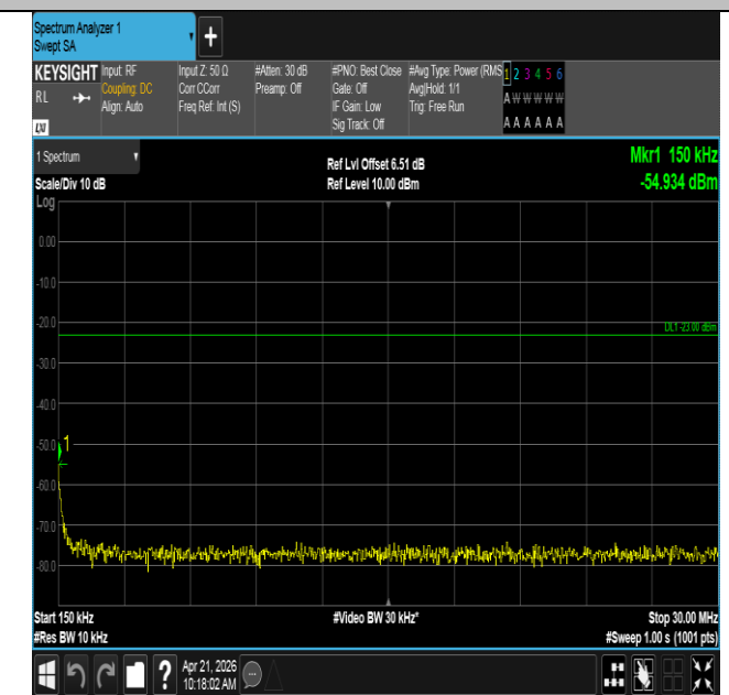
Band71-20MHz-16QAM-133222-1RB#0-0.15~30-PASS
