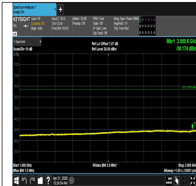
Band71-20MHz-QPSK-133322-100RB#0-1000~3000-PASS
