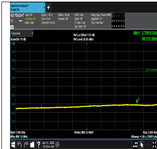
Band71-20MHz-16QAM-133222-1RB#99-1000~3000-PASS
