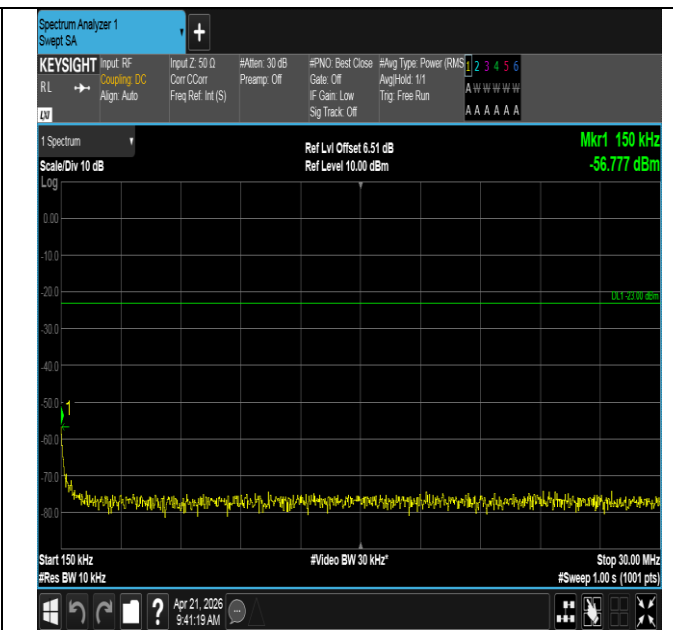
Band71-15MHz-16QAM-133397-1RB#74-0.15~30-PASS
