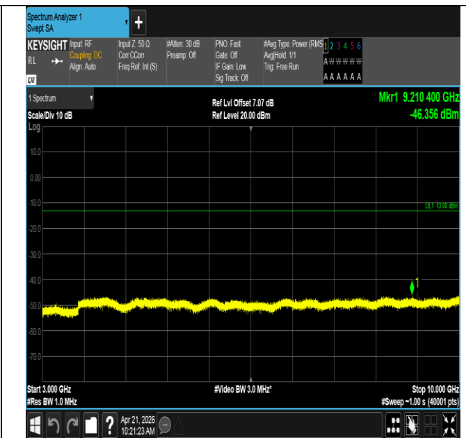
Band71-20MHz-16QAM-133222-100RB#0-3000~10000-PASS
