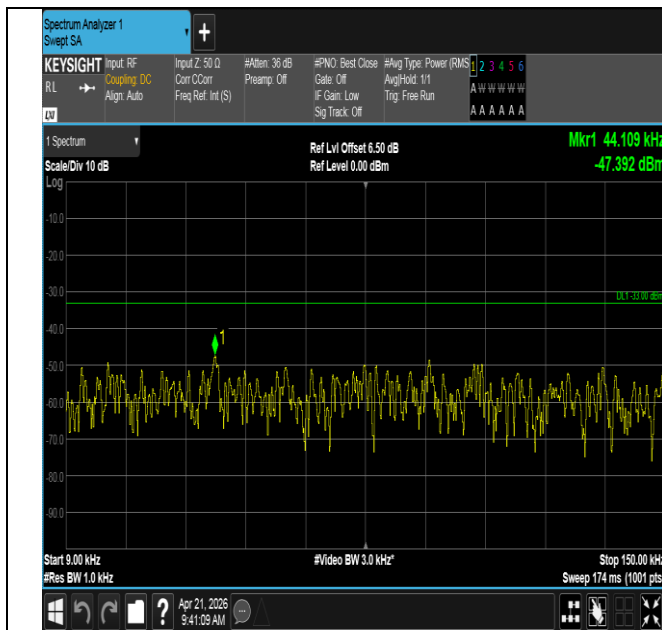
Band71-15MHz-16QAM-133397-1RB#74-0.009~0.15-PASS
