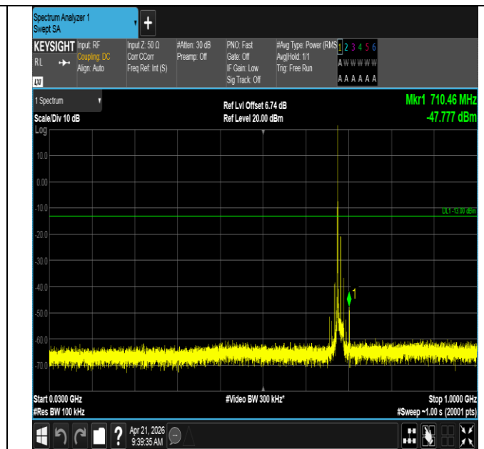
Band71-15MHz-16QAM-133397-1RB#0-30~1000-PASS
