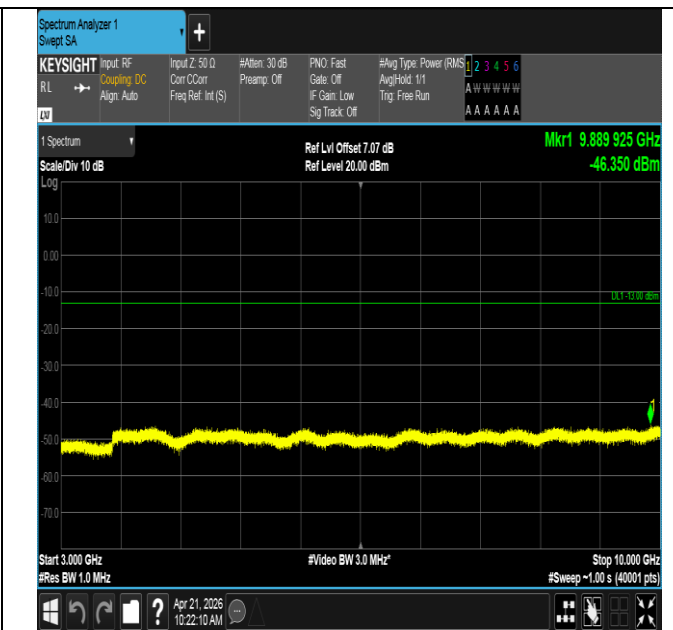
Band71-20MHz-QPSK-133322-1RB#0-3000~10000-PASS
