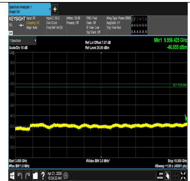
Band71-20MHz-16QAM-133322-1RB#99-3000~10000-PASS
