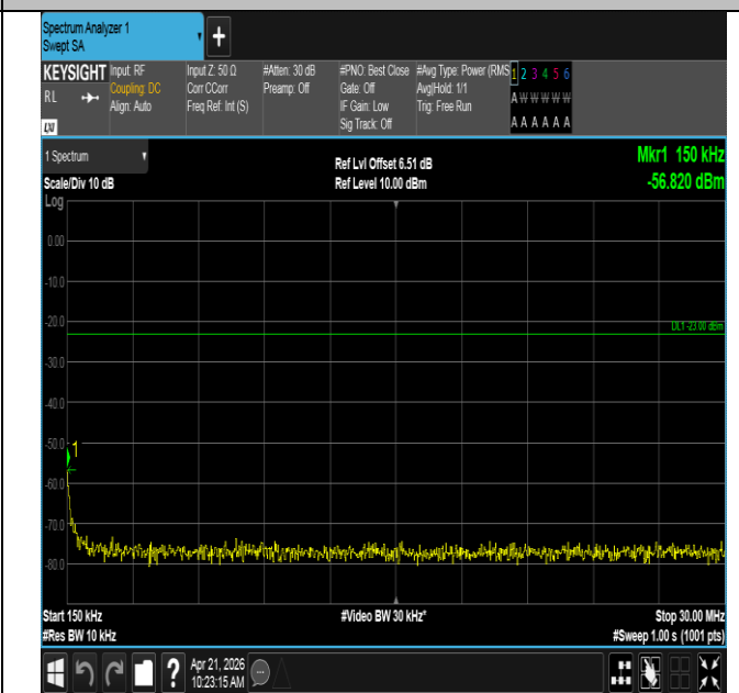
Band71-20MHz-QPSK-133322-1RB#99-0.15~30-PASS
