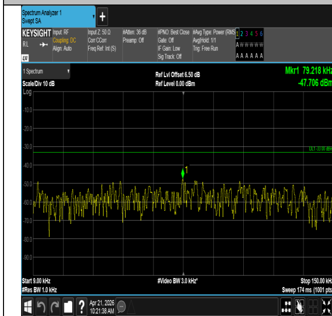
Band71-20MHz-QPSK-133322-1RB#0-0.009~0.15-PASS
