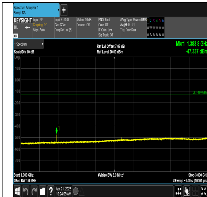
Band71-20MHz-16QAM-133322-1RB#99-1000~3000-PASS
