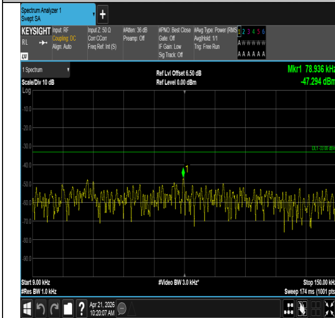
Band71-20MHz-QPSK-133222-100RB#0-0.009~0.15-PASS
