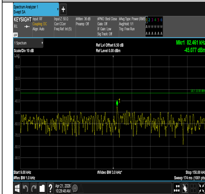
Band71-20MHz-16QAM-133372-100RB#0-0.009~0.15-PASS
