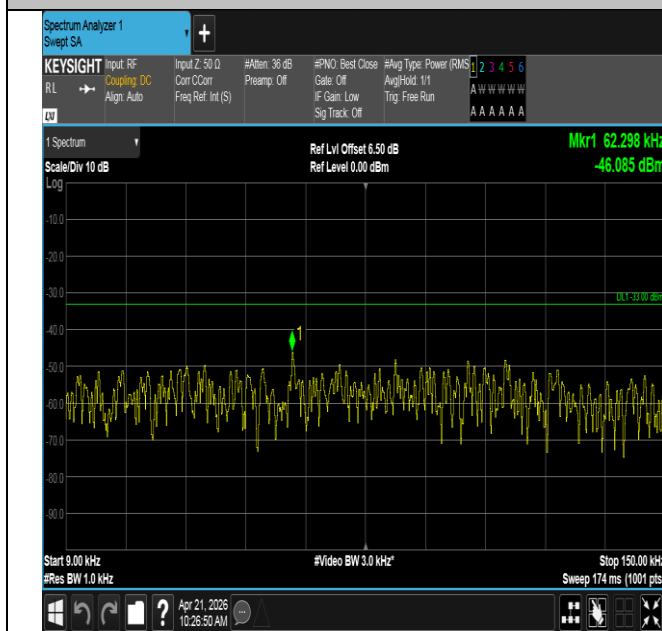
Band71-20MHz-16QAM-133372-1RB#0-0.009~0.15-PASS
