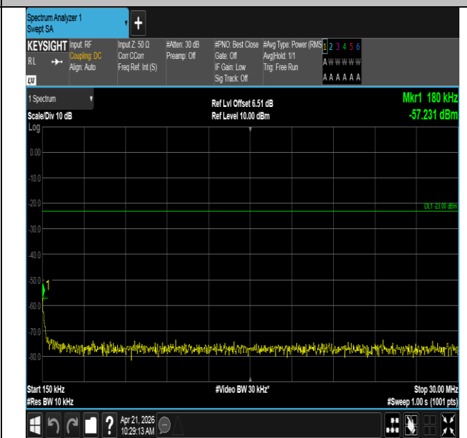
Band71-20MHz-QPSK-133372-100RB#0-0.15~30-PASS
