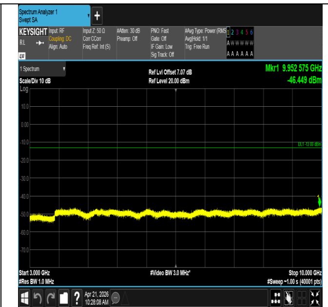
Band71-20MHz-QPSK-133372-1RB#99-3000~10000-PASS
