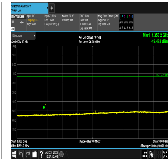
Band71-20MHz-16QAM-133372-1RB#0-1000~3000-PASS
