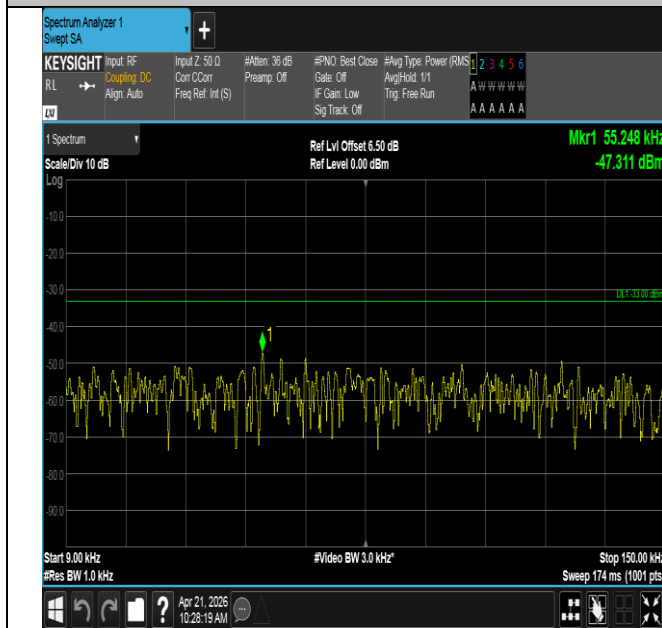
Band71-20MHz-16QAM-133372-1RB#99-0.009~0.15-PASS
