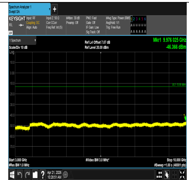
Band71-20MHz-16QAM-133372-1RB#99-3000~10000-PASS
