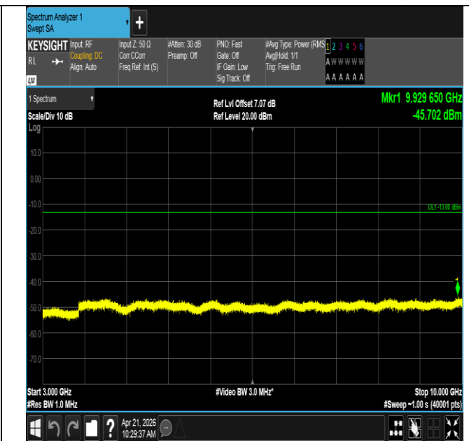
Band71-20MHz-QPSK-133372-100RB#0-3000~10000-PASS
