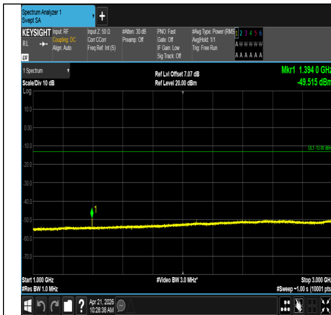
Band71-20MHz-16QAM-133372-1RB#99-1000~3000-PASS
