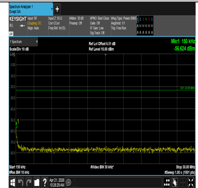
Band71-20MHz-16QAM-133372-1RB#99-0.15~30-PASS
