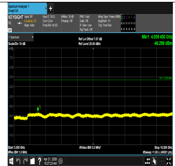
Band71-20MHz-16QAM-133372-1RB#0-3000~10000-PASS
