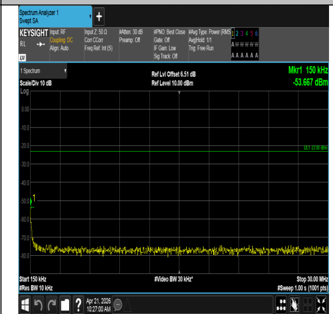
Band71-20MHz-16QAM-133372-1RB#0-0.15~30-PASS
