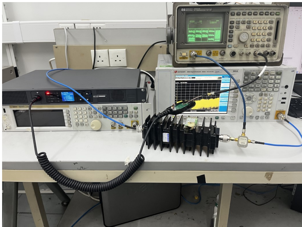
UHF Conducted Test Setup (Mobile)
