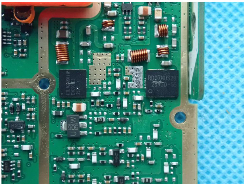
Internal Photo 14
