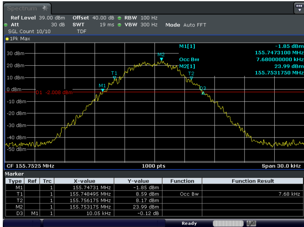
Test Graph 4FSK 1W 155.7525 12.5k OBW
