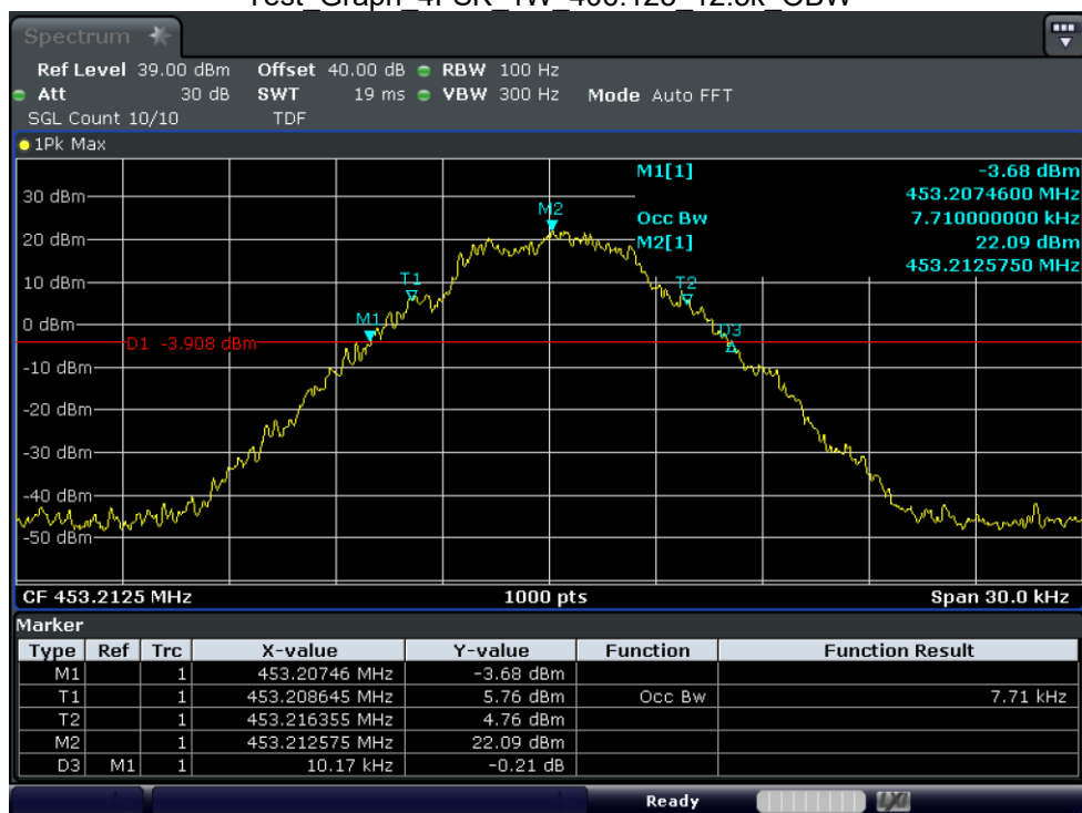
Test_Graph_4FSK_1W_453.2125_12.5k_OBW
