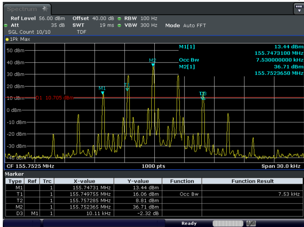
Test Graph FM 5W 155.7525 12.5k OBW
