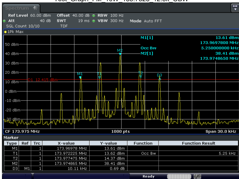
Test_Graph_FM_10W_173.975_12.5k_OBW
