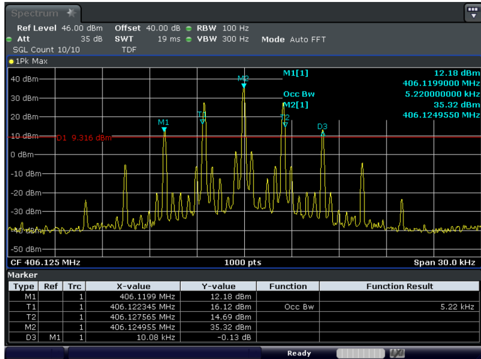
Test Graph FM 4W 406.125 12.5k OBW
