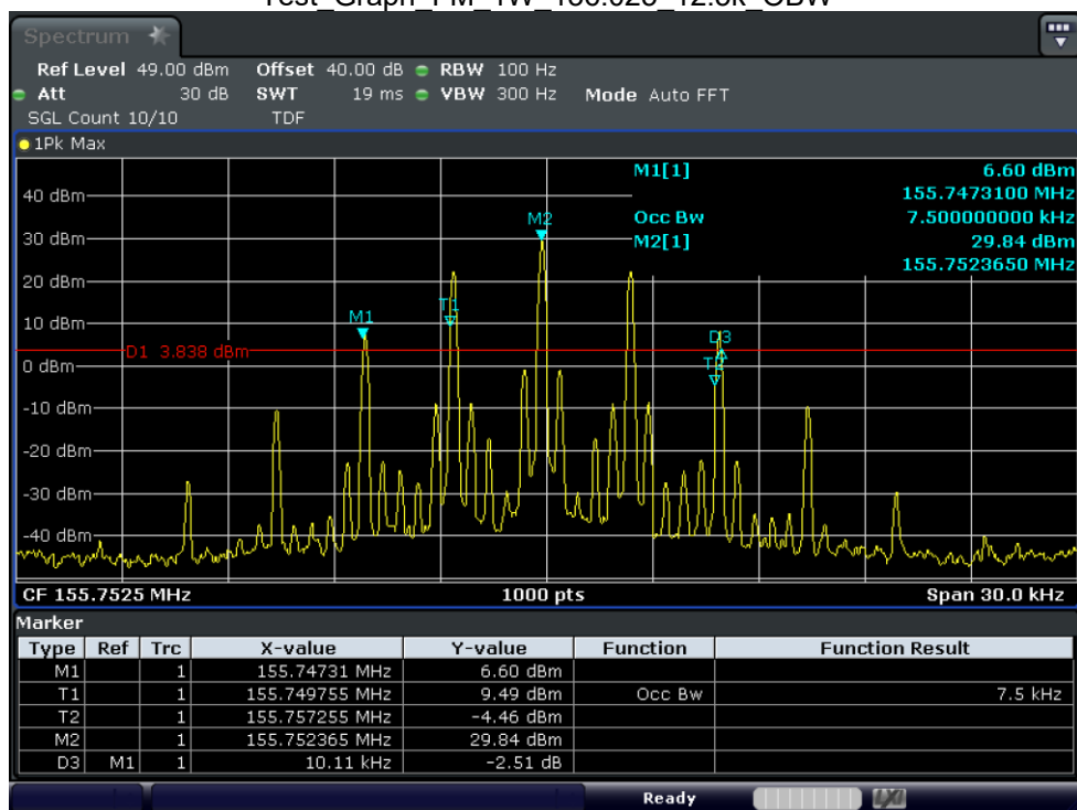
Test_Graph_FM_1W_155.7525_12.5k_OBW
