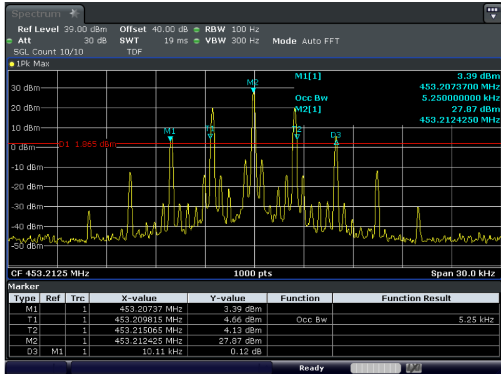
Test Graph FM 1W 453.2125 12.5k OBW
