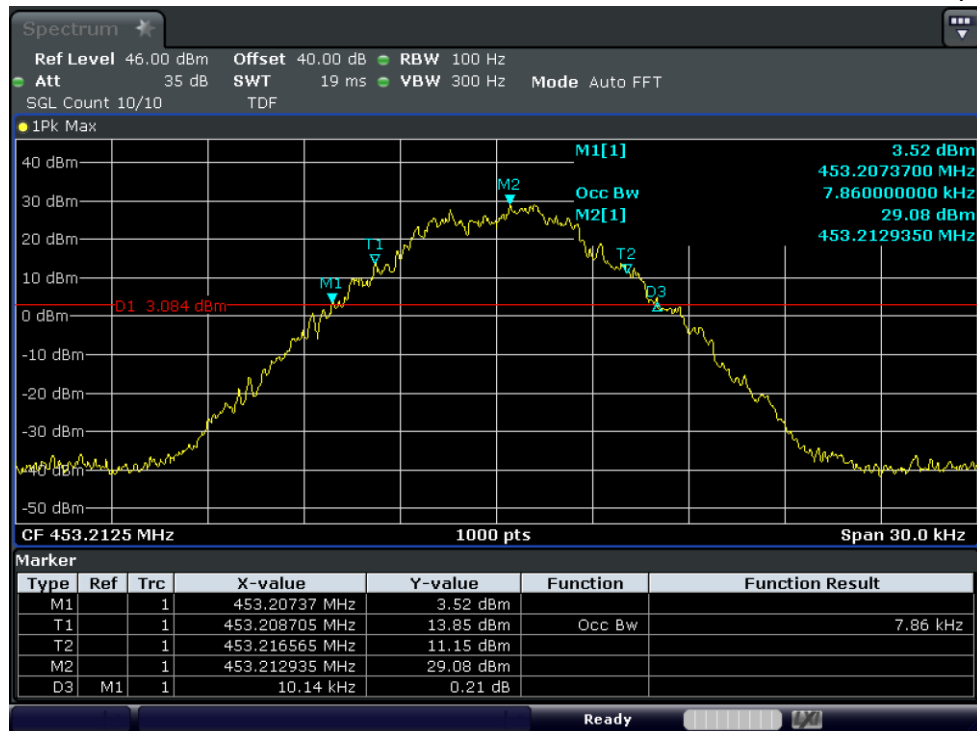
Test Graph 4FSK 4W 453.2125 12.5k OBW
