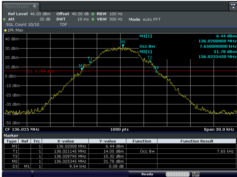
Test Graph 4FSK 5W 136.025 12.5k OBW
