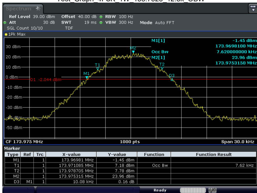
Test_Graph_4FSK_1W_173.975_12.5k_OBW
