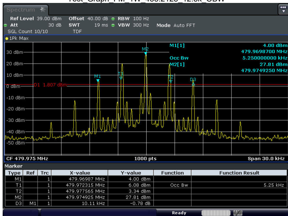
Test_Graph_FM_1W_479.975_12.5k_OBW
