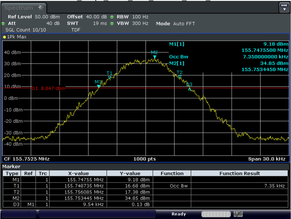
Test_Graph_4FSK_10W_155.7525_12.5k_OBW
