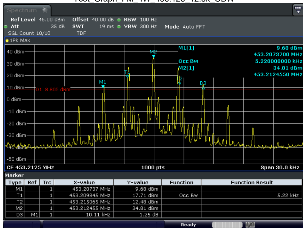
Test_Graph_FM_4W_453.2125_12.5k_OBW
