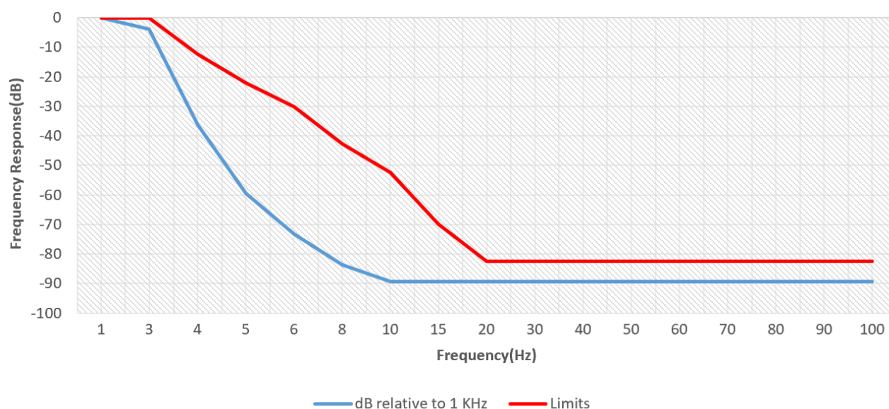
Audio Low Pass Filter Frequency Response
