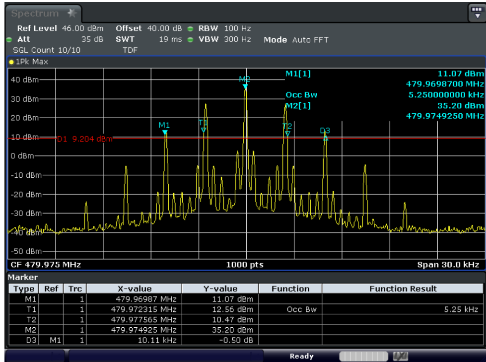
Test Graph FM 4W 479.975 12.5k OBW
