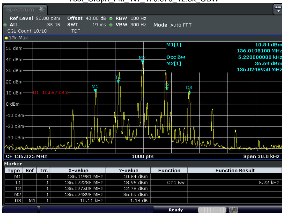
Test_Graph_FM_5W_136.025_12.5k_OBW
