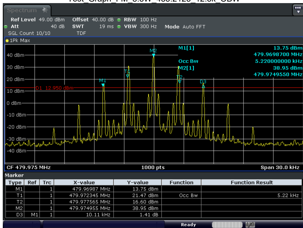
Test_Graph_FM_8.5W_479.975_12.5k_OBW
