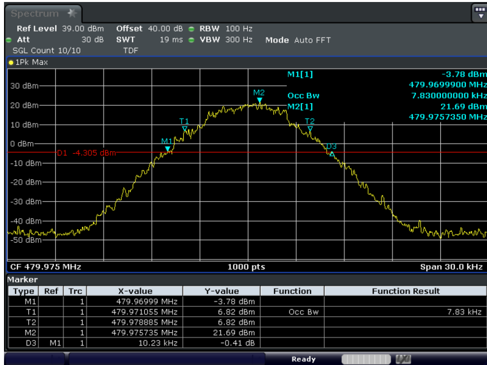
Test Graph 4FSK 1W 479.975 12.5k OBW
