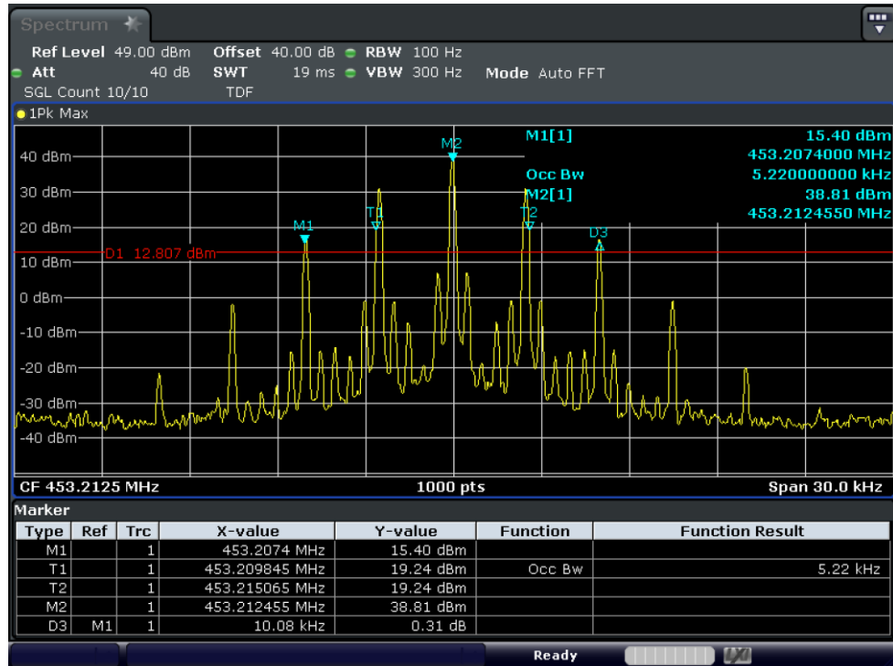
Test Graph FM 8.5W 453.2125 12.5k OBW
