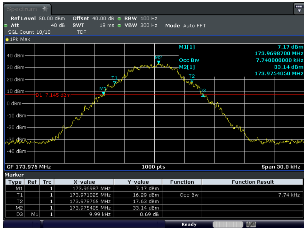
Test Graph 4FSK 10W 173.975 12.5k OBW
