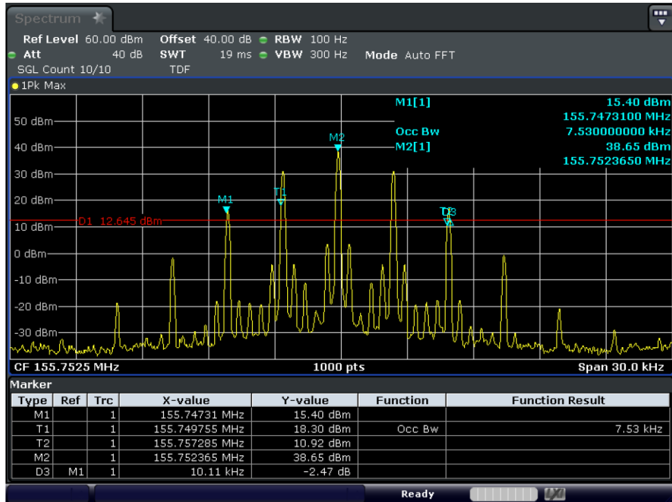
Test Graph FM 10W 155.7525 12.5k OBW
