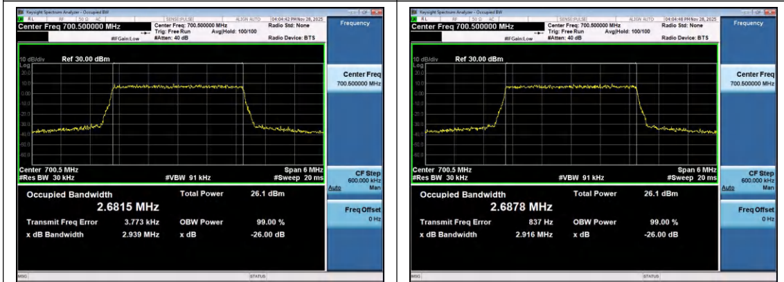
Band12-3MHz-QPSK-23025-15RB#0-PASS
