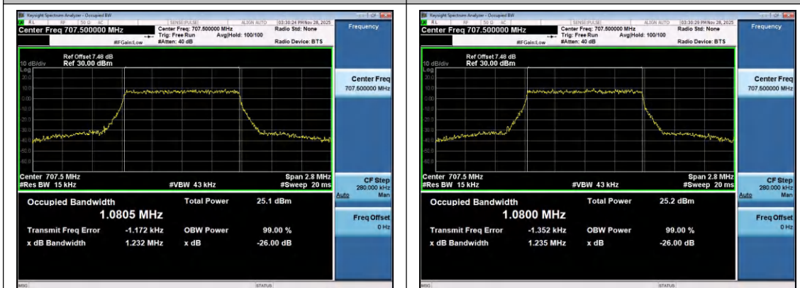
Band12-1.4MHz-16QAM-23095-6RB#0-PASS
