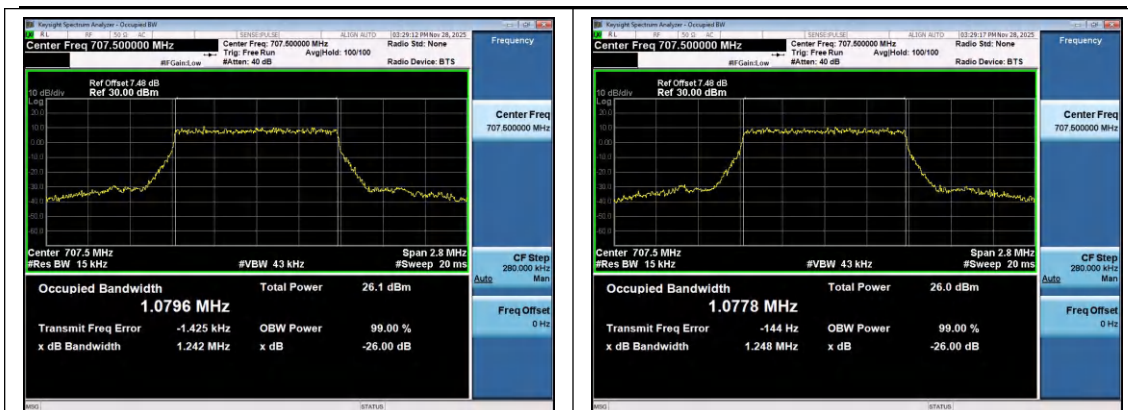
Band12-1.4MHz-QPSK-23095-6RB#0-PASS
