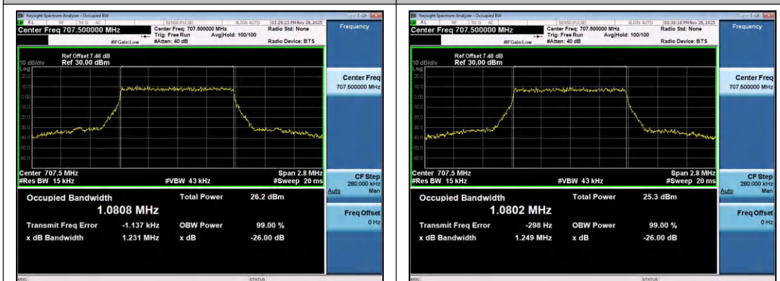
Band12-1.4MHz-QPSK-23095-6RB#0-PASS
