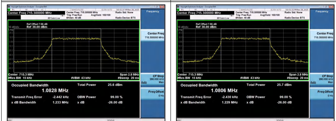
Band12-1.4MHz-QPSK-23173-6RB#0-PASS
