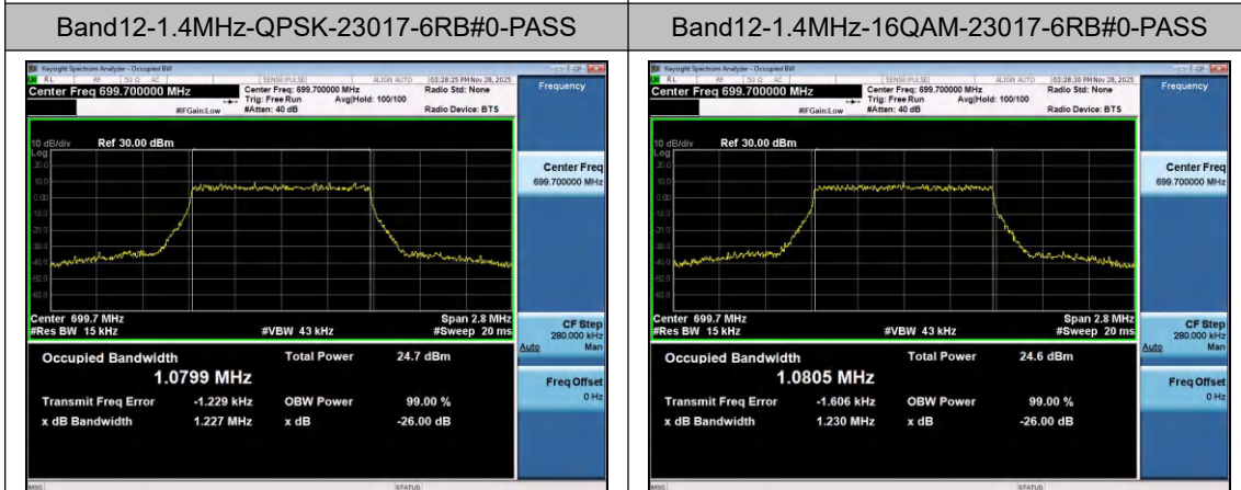
Band12-1.4MHz-16QAM-23017-6RB#0-PASS
