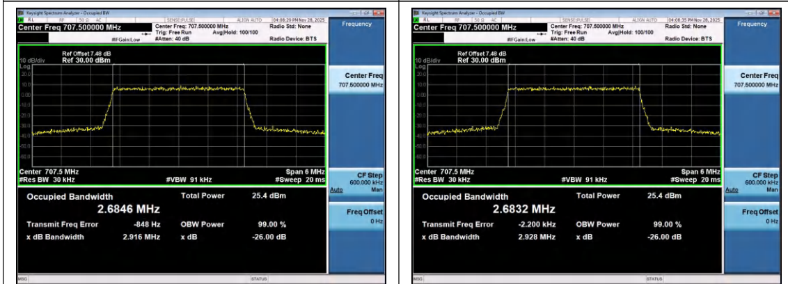
Band12-3MHz-16QAM-23095-15RB#0-PASS
