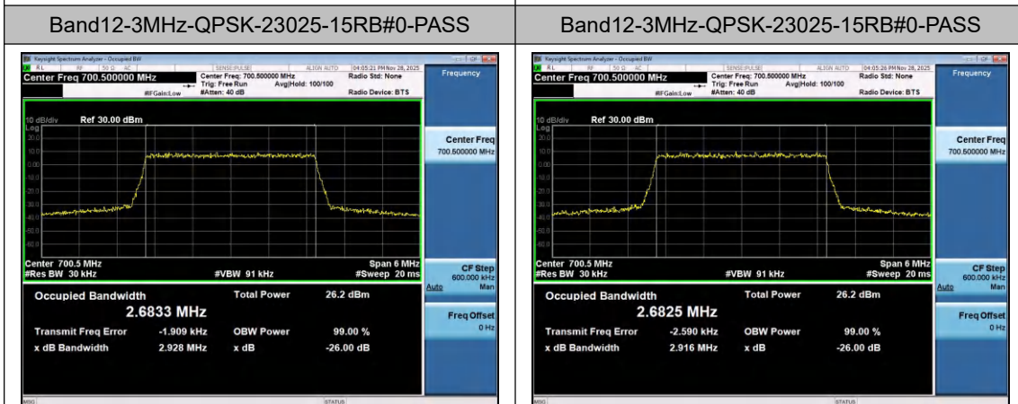
Band12-3MHz-QPSK-23025-15RB#0-PASS
