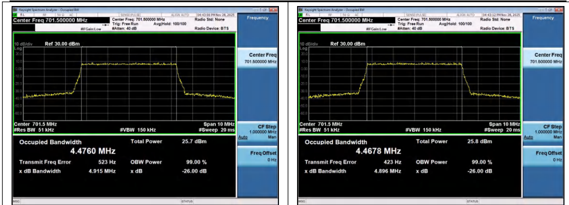
Band12-5MHz-16QAM-23035-25RB#0-PASS
