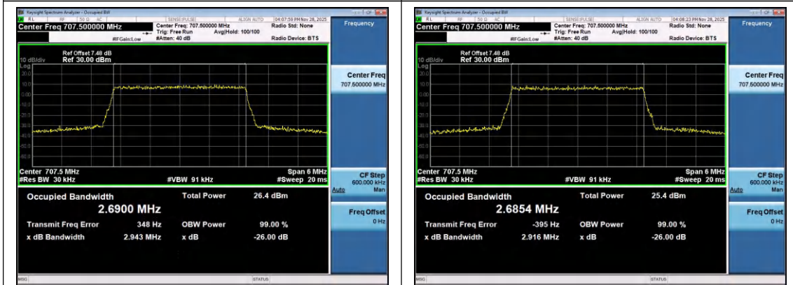
Band12-3MHz-QPSK-23095-15RB#0-PASS
