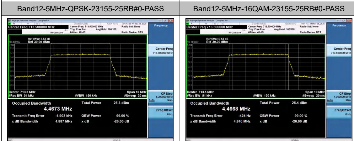
Band12-5MHz-16QAM-23155-25RB#0-PASS
