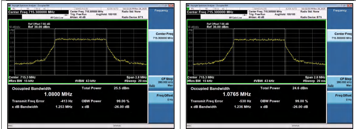
Band12-1.4MHz-QPSK-23173-6RB#0-PASS
