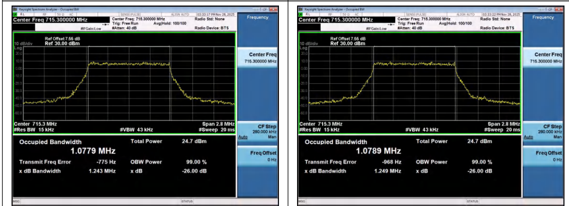
Band12-1.4MHz-16QAM-23173-6RB#0-PASS
