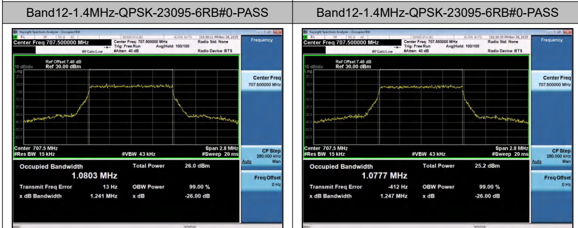
Band12-1.4MHz-QPSK-23095-6RB#0-PASS
