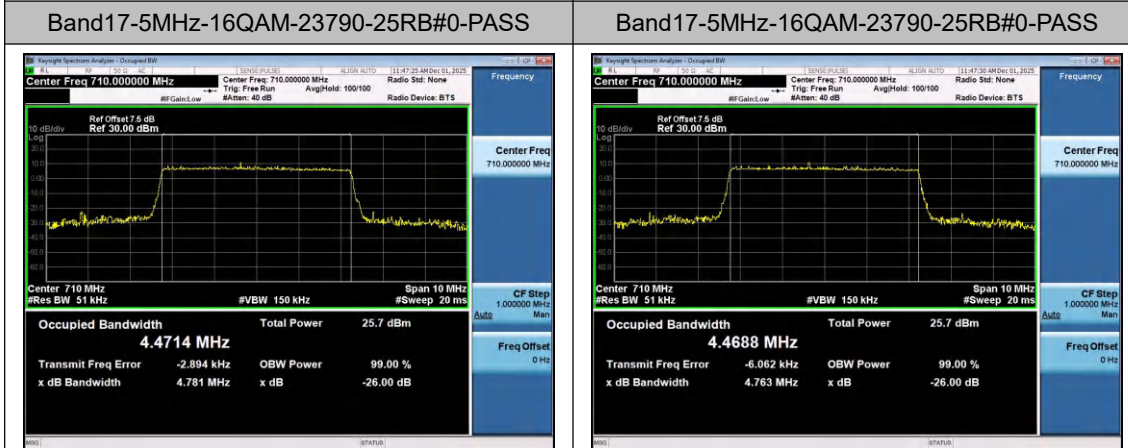
Band17-5MHz-16QAM-23790-25RB#0-PASS
