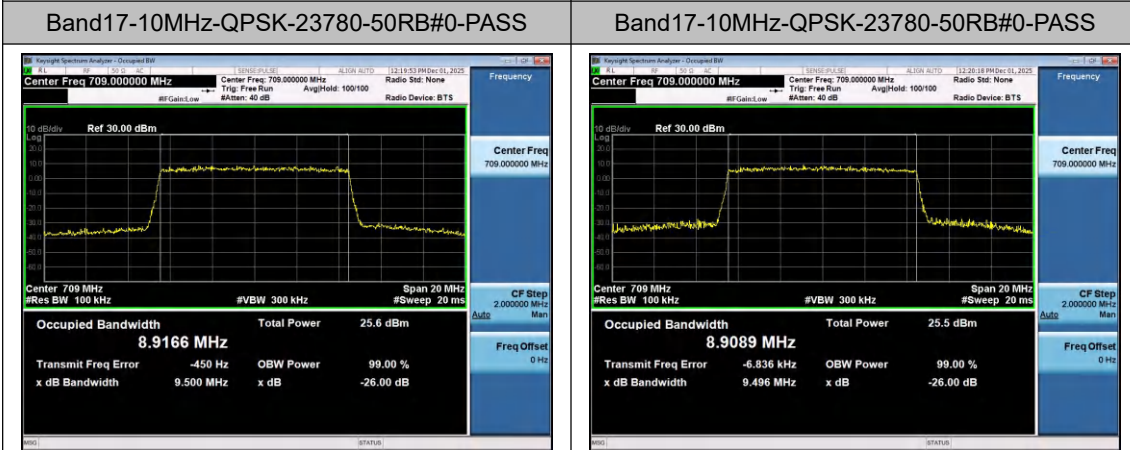
Band17-10MHz-QPSK-23780-50RB#0-PASS
