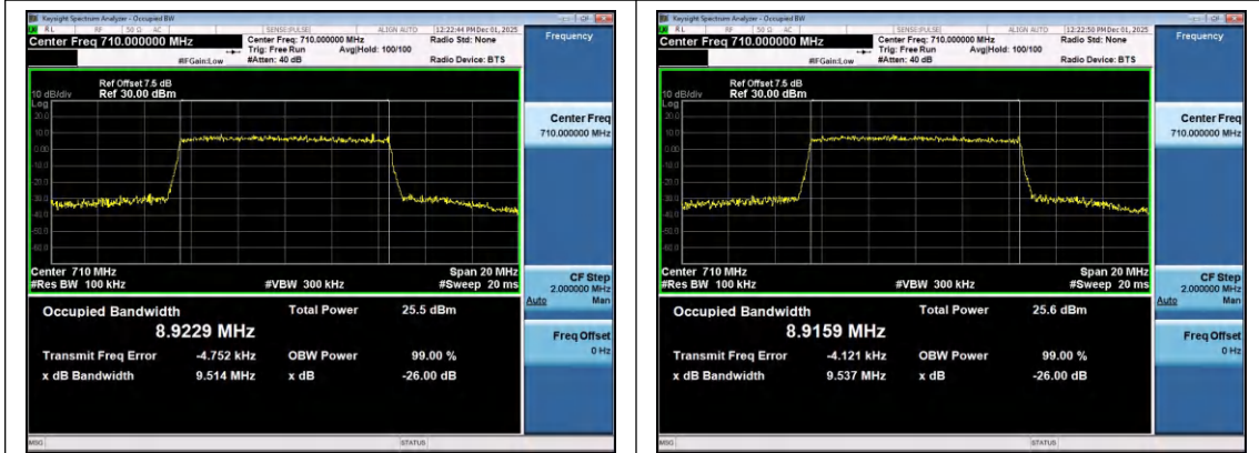
Band17-10MHz-16QAM-23790-50RB#0-PASS
