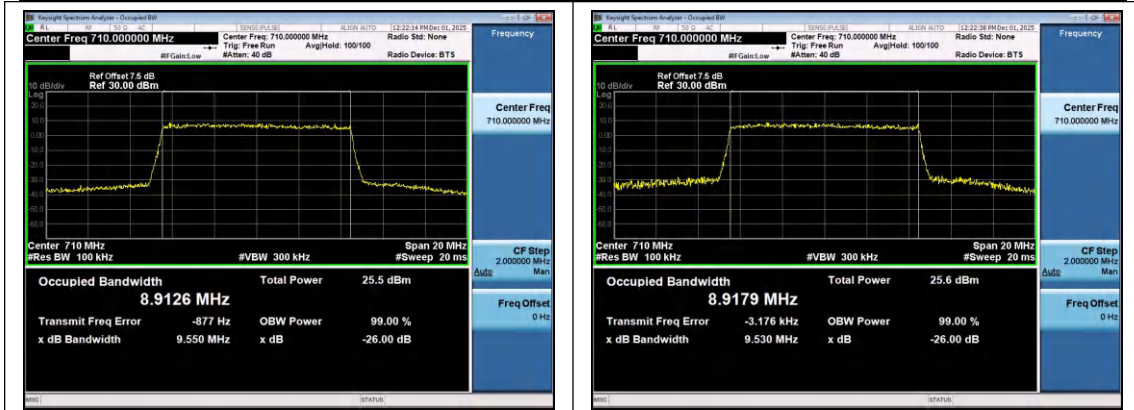
Band17-10MHz-QPSK-23790-50RB#0-PASS
