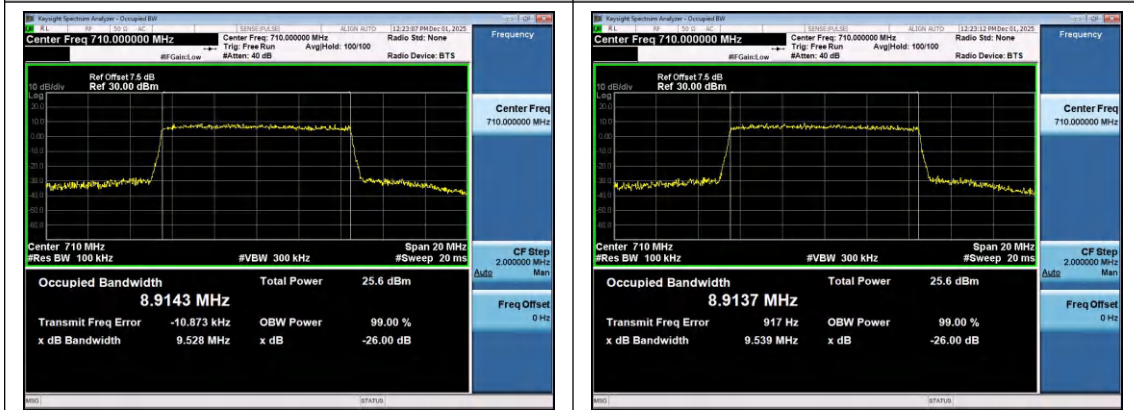
Band17-10MHz-16QAM-23790-50RB#0-PASS
