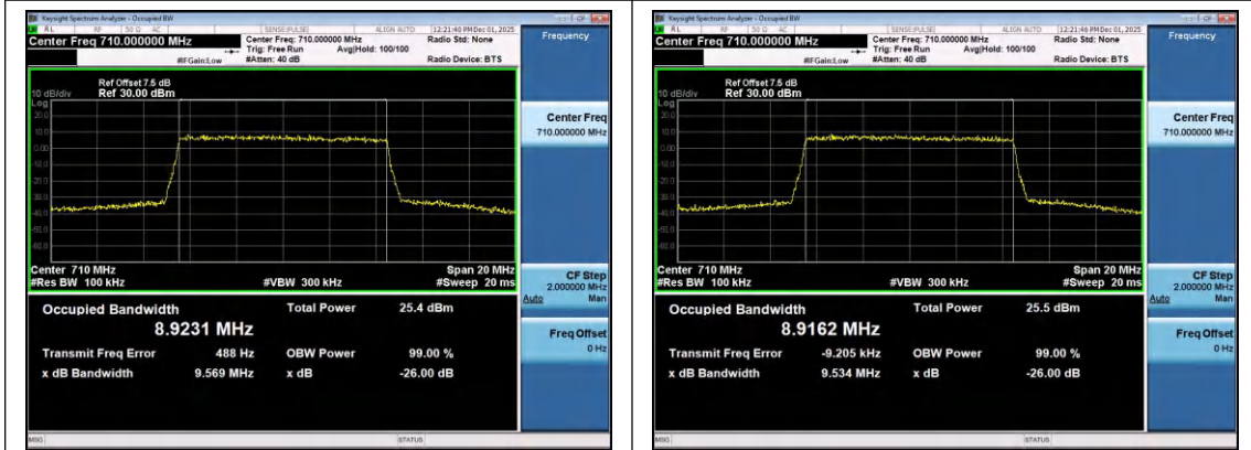
Band17-10MHz-QPSK-23790-50RB#0-PASS
