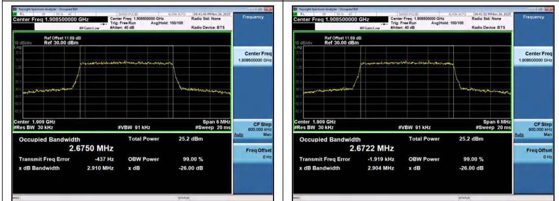
Band2-3MHz-16QAM-19185-15RB#0-PASS
