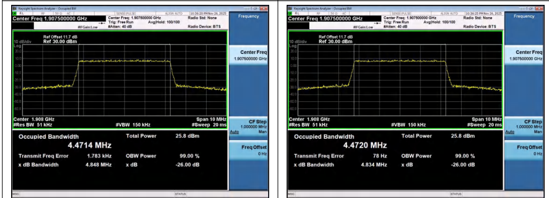
Band2-5MHz-16QAM-19175-25RB#0-PASS
