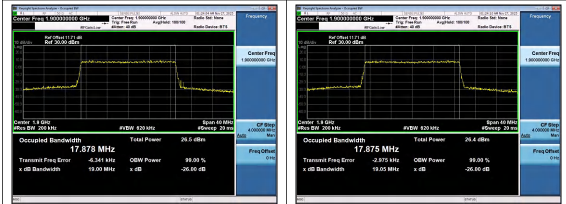
Band2-20MHz-16QAM-19100-100RB#0-PASS
