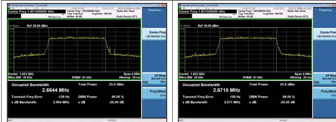
Band2-3MHz-16QAM-18615-15RB#0-PASS
