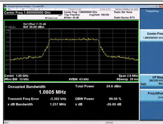
Band2-1.4MHz-16QAM-18900-6RB#0-PASS
