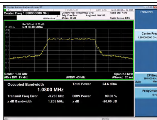
Band2-1.4MHz-16QAM-18900-6RB#0-PASS
