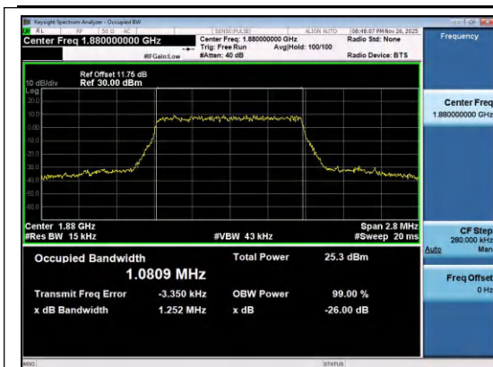
Band2-1.4MHz-QPSK-18900-6RB#0-PASS
