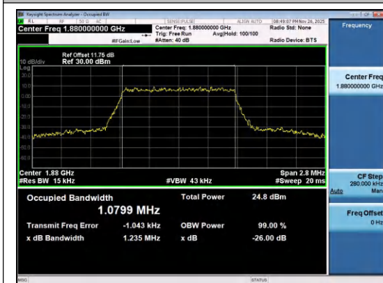
Band2-1.4MHz-16QAM-18900-6RB#0-PASS
