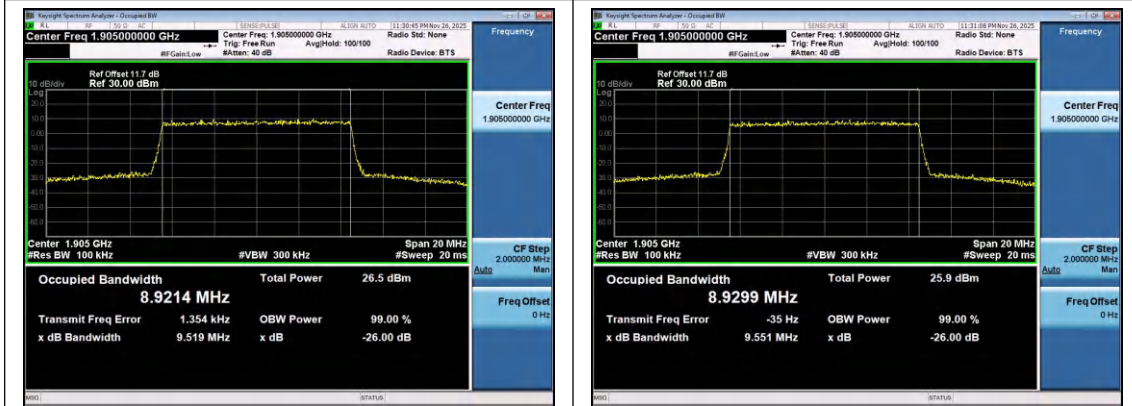
Band2-10MHz-QPSK-19150-50RB#0-PASS
