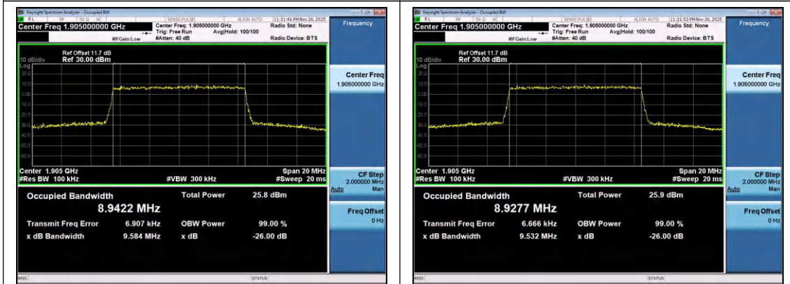
Band2-10MHz-16QAM-19150-50RB#0-PASS
