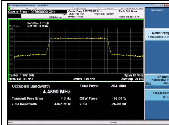
Band2-5MHz-16QAM-19175-25RB#0-PASS
