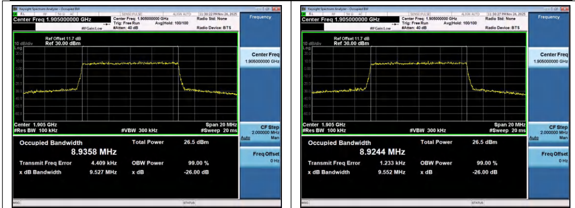
Band2-10MHz-QPSK-19150-50RB#0-PASS
