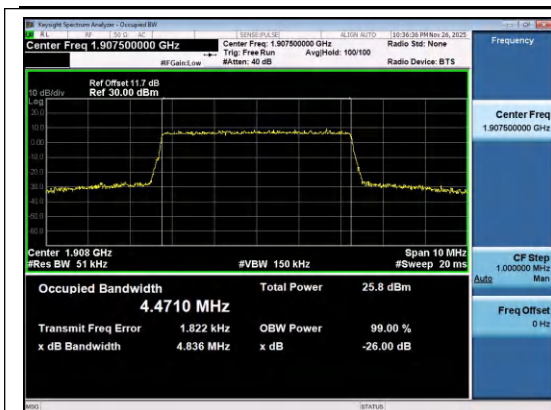
Band2-5MHz-16QAM-19175-25RB#0-PASS
