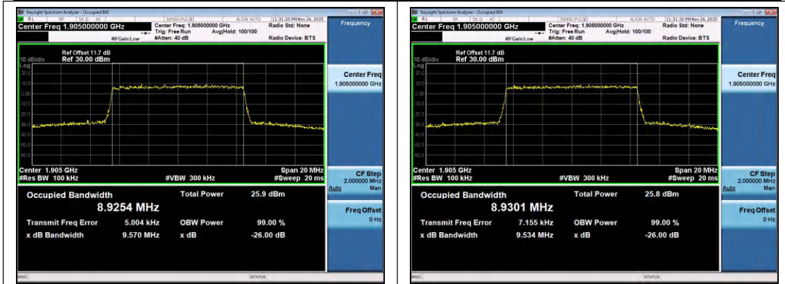
Band2-10MHz-16QAM-19150-50RB#0-PASS
