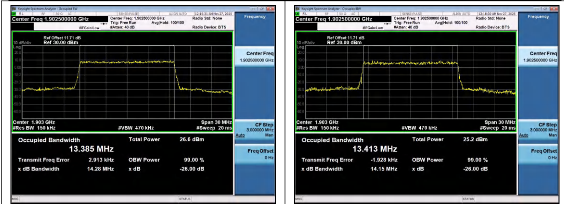
Band2-15MHz-QPSK-19125-75RB#0-PASS
