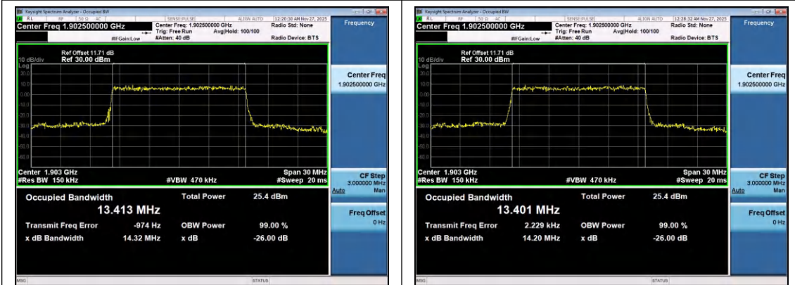
Band2-15MHz-QPSK-19125-75RB#0-PASS
