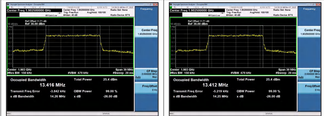
Band2-15MHz-16QAM-19125-75RB#0-PASS
