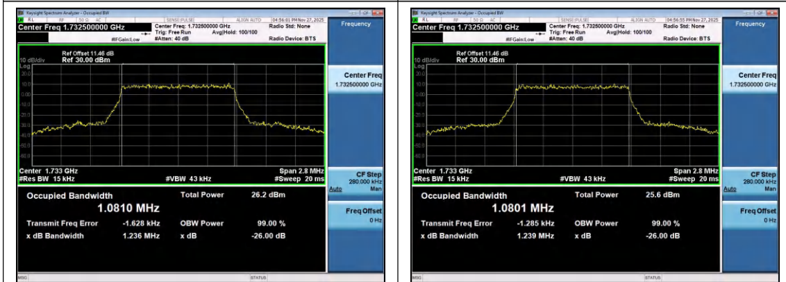
Band4-1.4MHz-QPSK-20175-6RB#0-PASS
