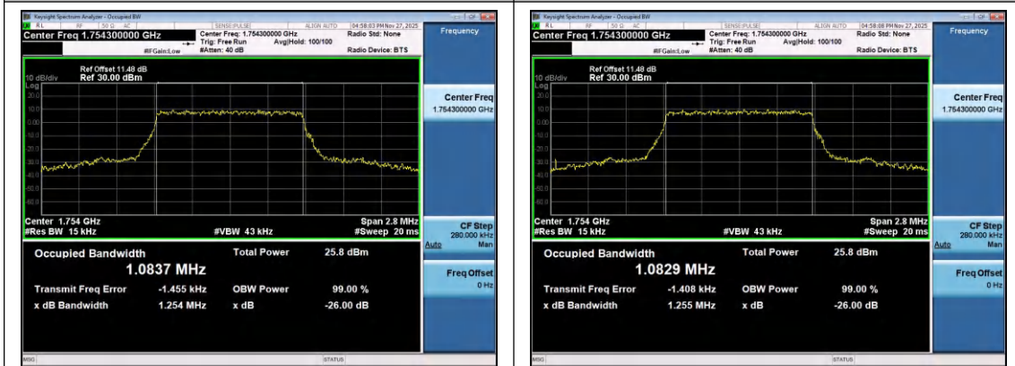
Band4-1.4MHz-QPSK-20393-6RB#0-PASS
