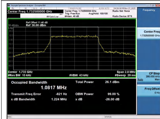
Band4-1.4MHz-QPSK-20175-6RB#0-PASS
