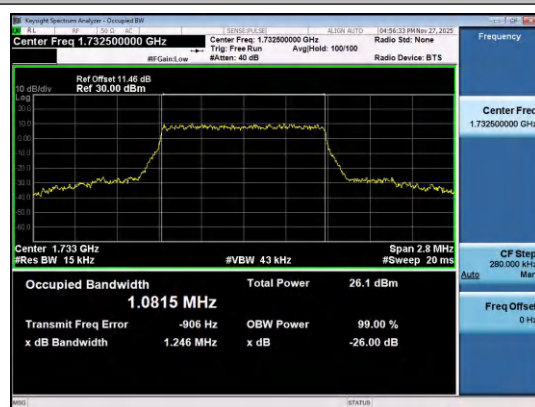
Band4-1.4MHz-QPSK-20175-6RB#0-PASS
