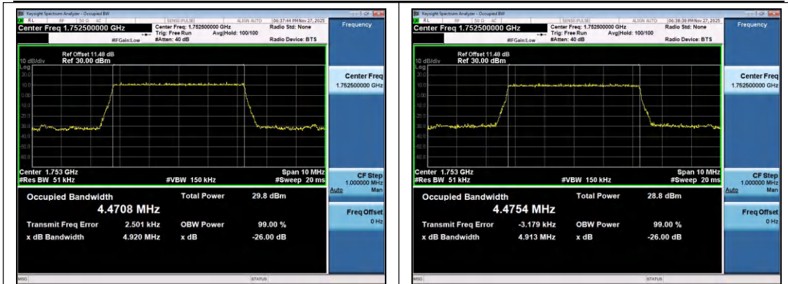
Band4-5MHz-QPSK-20375-25RB#0-PASS
