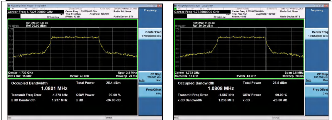
Band4-1.4MHz-16QAM-20175-6RB#0-PASS
