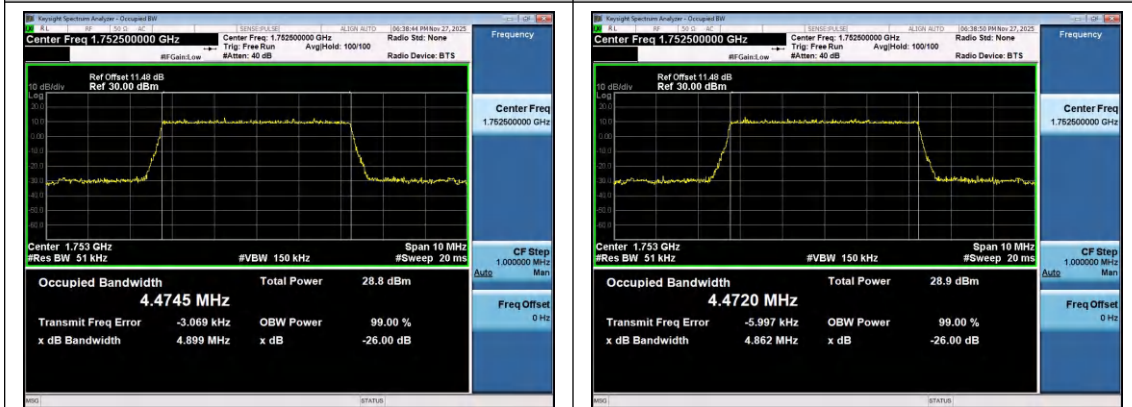
Band4-5MHz-16QAM-20375-25RB#0-PASS
