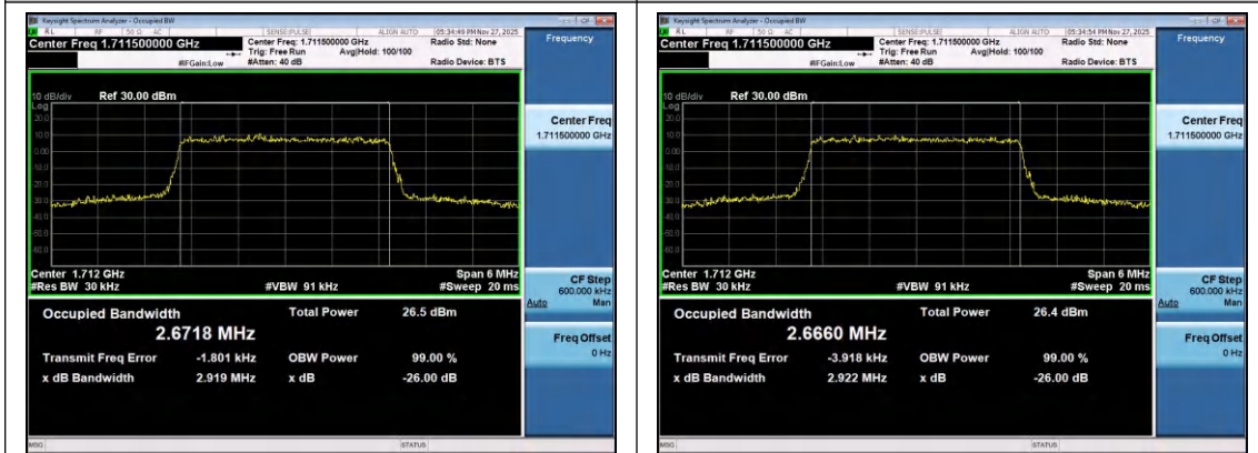
Band4-3MHz-16QAM-19965-15RB#0-PASS
