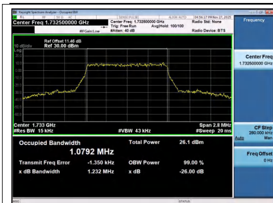
Band4-1.4MHz-QPSK-20175-6RB#0-PASS
