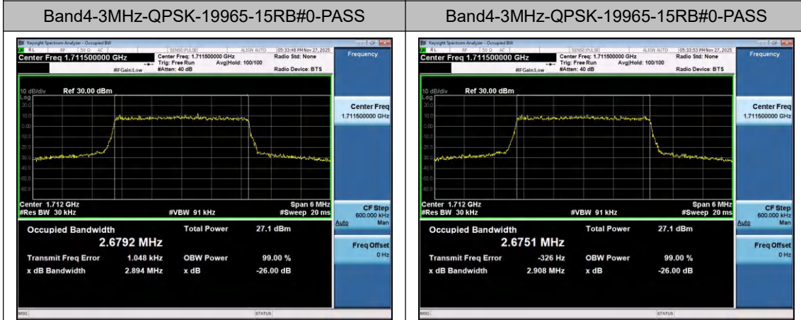
Band4-3MHz-QPSK-19965-15RB#0-PASS
