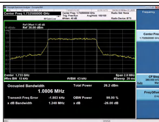
Band4-1.4MHz-QPSK-20175-6RB#0-PASS
