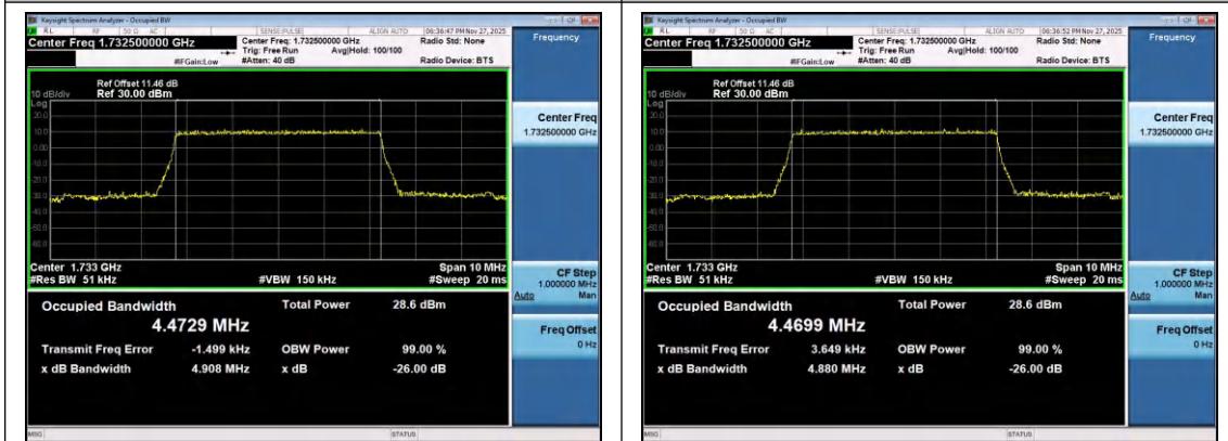
Band4-5MHz-16QAM-20175-25RB#0-PASS
