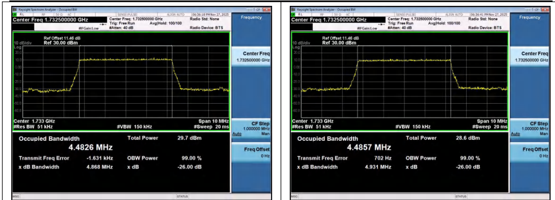
Band4-5MHz-QPSK-20175-25RB#0-PASS
