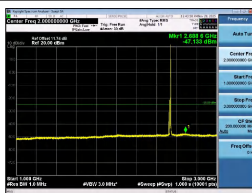
Band7-10MHz-16QAM-21100-1RB#49-1000~30 00-PASS
