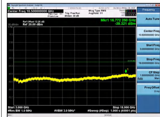
Band7-15MHz-16QAM-21375-1RB#74-3000~18000-PASS
