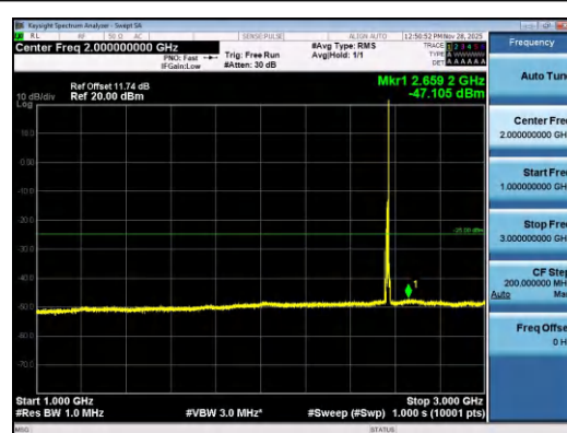
Band7-10MHz-16QAM-21400-1RB#49-1000~3000-PASS
