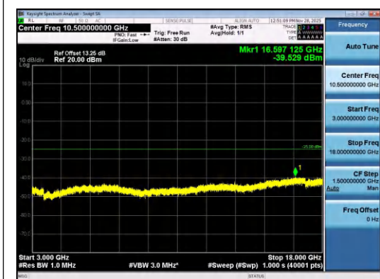
Band7-10MHz-16QAM-21400-1RB#49-3000~18000-PASS
