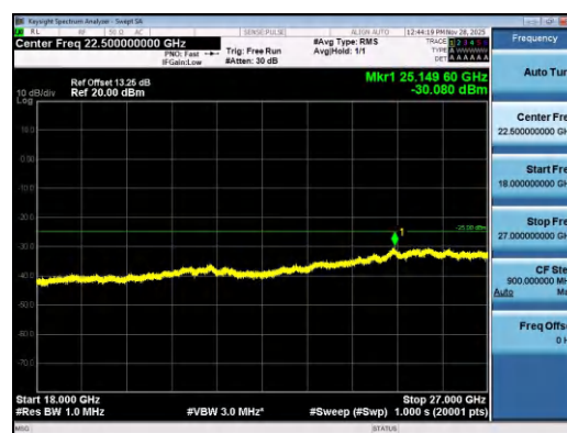
Band7-10MHz-16QAM-21100-1RB#49-18000~2 7000-PASS
