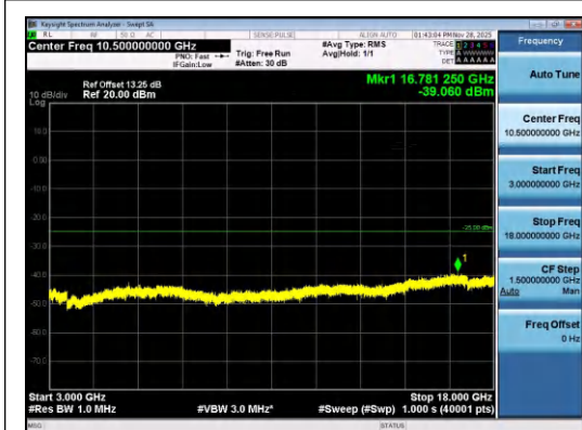
Band7-15MHz-16QAM-21100-1RB#74-3000~18000-PASS
