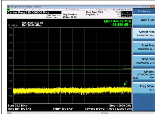
Band7-10MHz-16QAM-21100-1RB#49-30~1000- PASS
