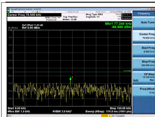
Band7-10MHz-16QAM-21100-1RB#49-0.009~0. 15-PASS
