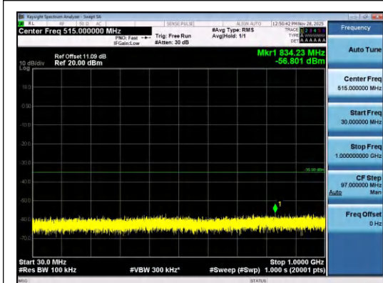
Band7-10MHz-16QAM-21400-1RB#49-30~1000-PASS
