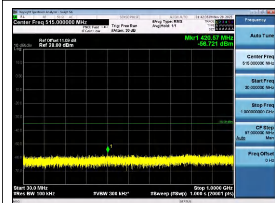
Band7-15MHz-16QAM-21100-1RB#74-30~1000-PASS
