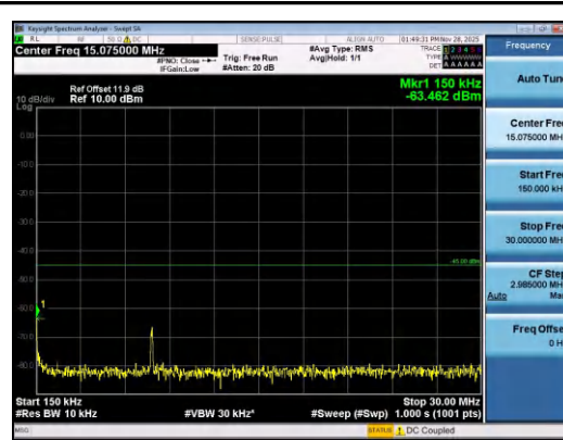
Band7-15MHz-16QAM-21375-1RB#74-0.15~30-PASS
