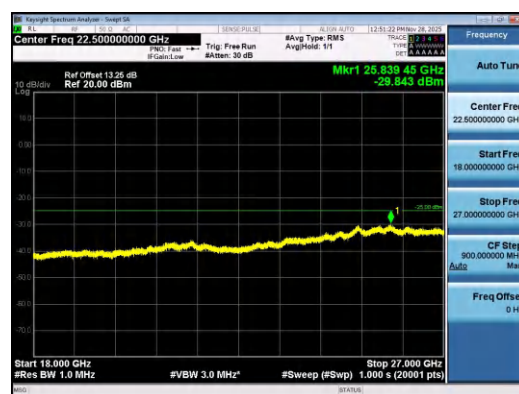
Band7-10MHz-16QAM-21400-1RB#49-18000~27000-PASS
