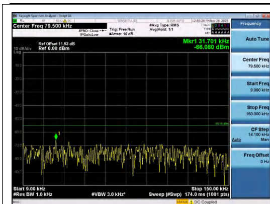
Band7-10MHz-16QAM-21400-1RB#49-0.009~0.15-PASS
