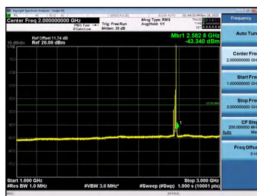
Band7-15MHz-16QAM-21375-1RB#74-1000~3000-PASS
