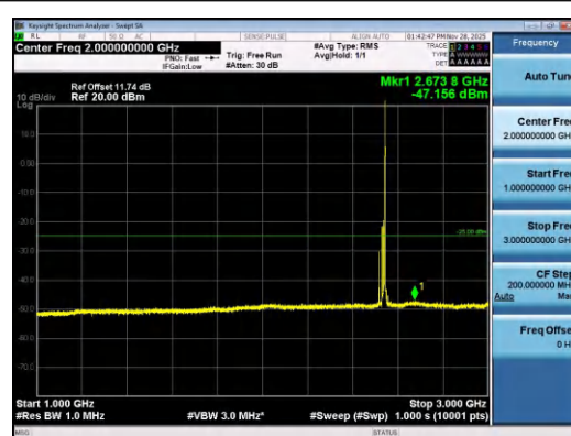
Band7-15MHz-16QAM-21100-1RB#74-1000~3000-PASS
