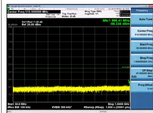
Band7-15MHz-16QAM-21375-1RB#74-30~1000-PASS
