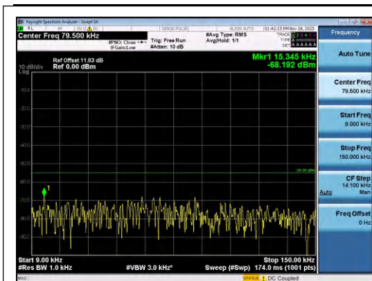
Band7-15MHz-16QAM-21100-1RB#74-0.009~0.15-PASS
