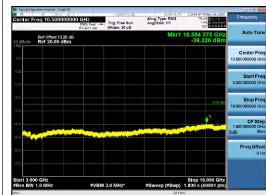
Band7-10MHz-16QAM-21100-1RB#49-3000~18 000-PASS
