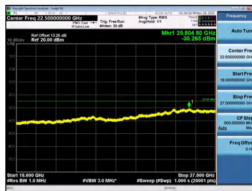
Band7-15MHz-16QAM-21375-1RB#74-18000~27000-PASS
