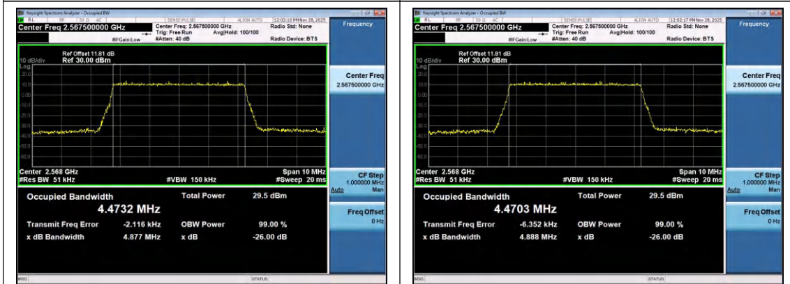
Band7-5MHz-16QAM-21425-25RB#0-PASS
