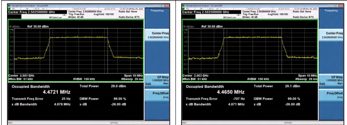
Band7-5MHz-16QAM-20775-25RB#0-PASS
