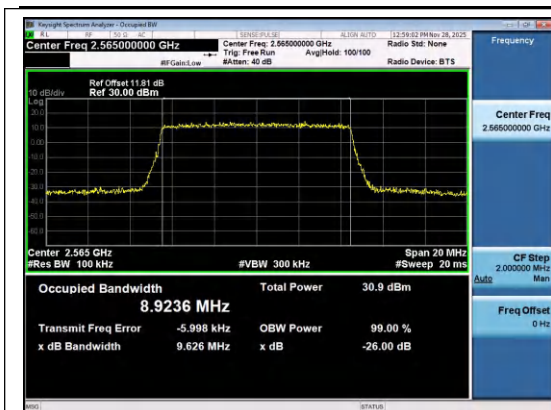
Band7-10MHz-QPSK-21400-50RB#0-PASS
