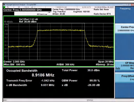
Band7-10MHz-16QAM-21400-50RB#0-PASS
