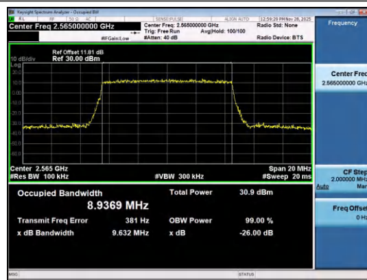
Band7-10MHz-QPSK-21400-50RB#0-PASS
