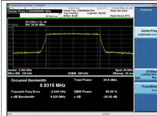
Band7-10MHz-QPSK-21400-50RB#0-PASS
