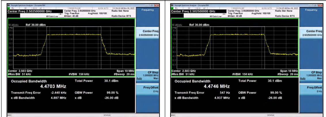
Band7-5MHz-QPSK-20775-25RB#0-PASS
