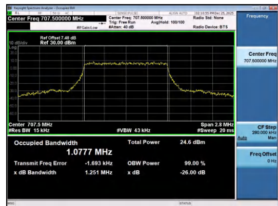
Band12-1.4MHz-QPSK-23095-6RB#0-PASS
