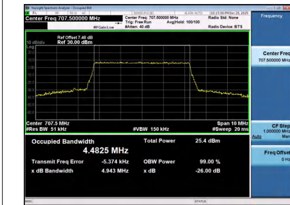
Band12-5MHz-QPSK-23095-25RB#0-PASS
