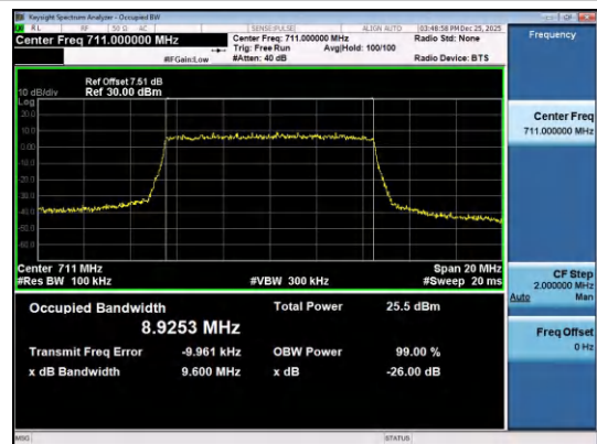
Band12-10MHz-QPSK-23130-50RB#0-PASS
