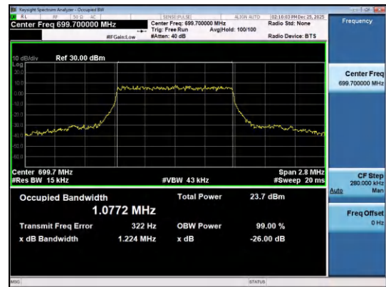
Band12-1.4MHz-16QAM-23017-6RB#0-PASS
