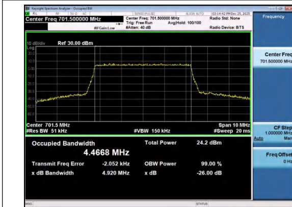
Band12-5MHz-16QAM-23035-25RB#0-PASS
