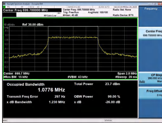
Band12-1.4MHz-16QAM-23017-6RB#0-PASS
