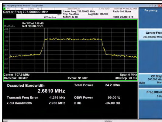
Band12-3MHz-16QAM-23095-15RB#0-PASS
