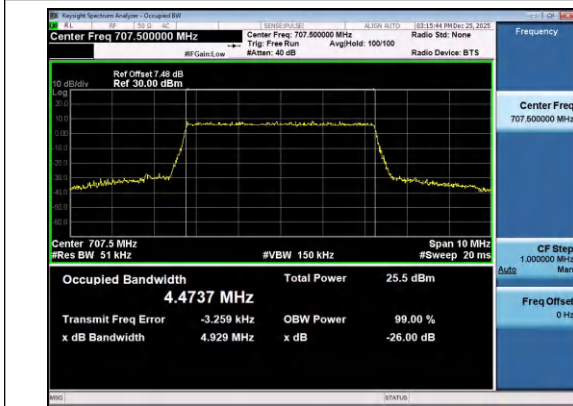
Band12-5MHz-QPSK-23095-25RB#0-PASS
