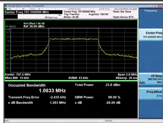
Band12-1.4MHz-16QAM-23095-6RB#0-PASS
