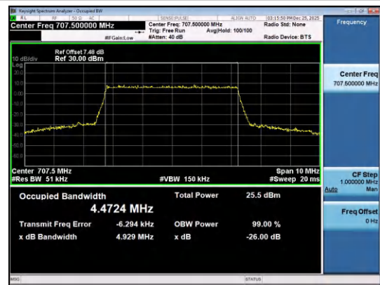
Band12-5MHz-QPSK-23095-25RB#0-PASS
