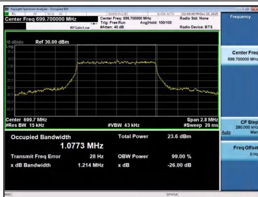
Band12-1.4MHz-16QAM-23017-6RB#0-PASS
