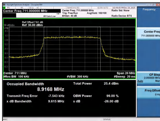
Band12-10MHz-QPSK-23130-50RB#0-PASS
