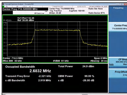
Band12-3MHz-QPSK-23165-15RB#0-PASS
