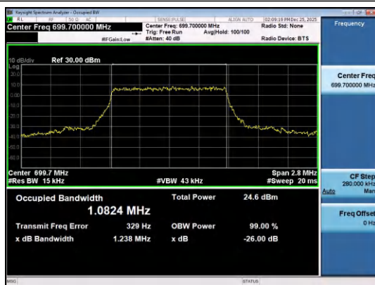
Band12-1.4MHz-QPSK-23017-6RB#0-PASS
