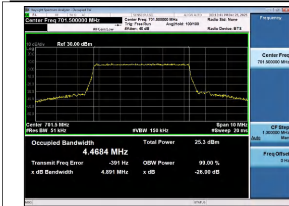
Band12-5MHz-QPSK-23035-25RB#0-PASS
