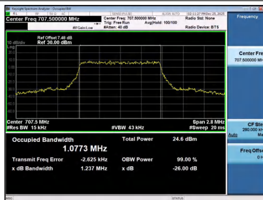
Band12-1.4MHz-QPSK-23095-6RB#0-PASS
