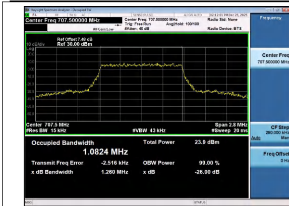
Band12-1.4MHz-16QAM-23095-6RB#0-PASS
