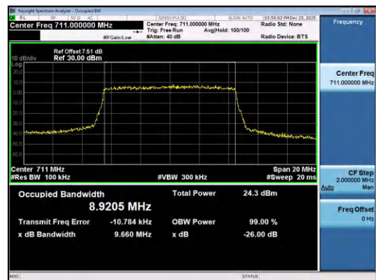
Band12-10MHz-16QAM-23130-50RB#0-PASS
