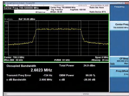
Band12-3MHz-QPSK-23025-15RB#0-PASS
