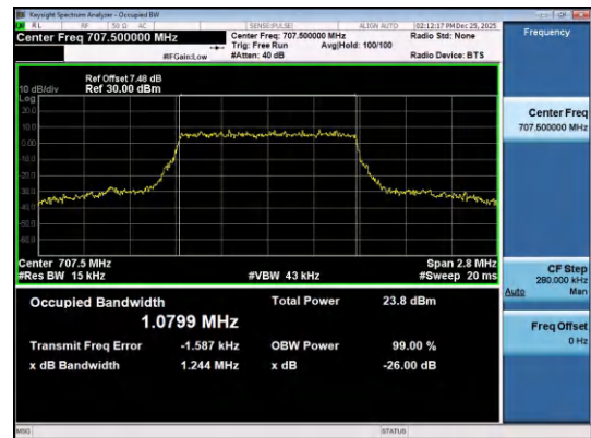
Band12-1.4MHz-16QAM-23095-6RB#0-PASS
