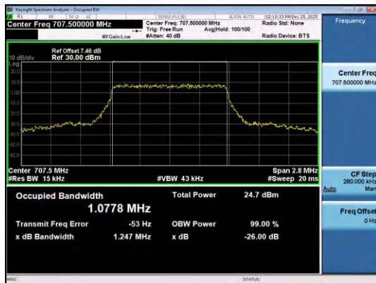
Band12-1.4MHz-QPSK-23095-6RB#0-PASS
