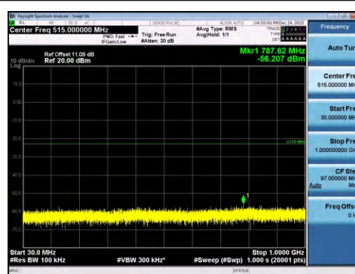
Band2-15MHz-16QAM-18675-75RB#0-30~1000- PASS
