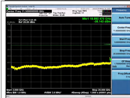
Band2-15MHz-16QAM-18675-1RB#74-3000~20 000-PASS
