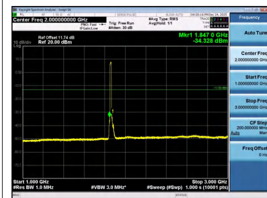
Band2-15MHz-16QAM-18675-75RB#0-1000~30 00-PASS
