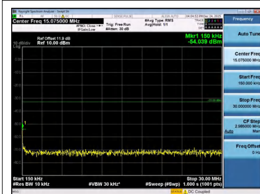
Band2-15MHz-16QAM-18675-75RB#0-0.15~30- PASS
