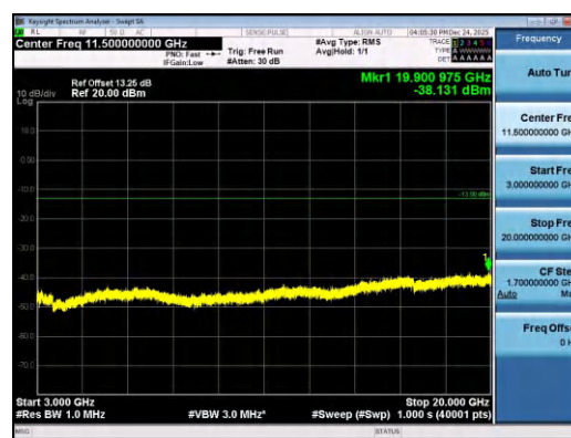
Band2-15MHz-16QAM-18675-75RB#0-3000~20 000-PASS
