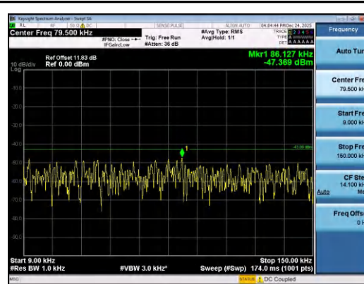
Band2-15MHz-16QAM-18675-75RB#0-0.009~0. 15-PASS
