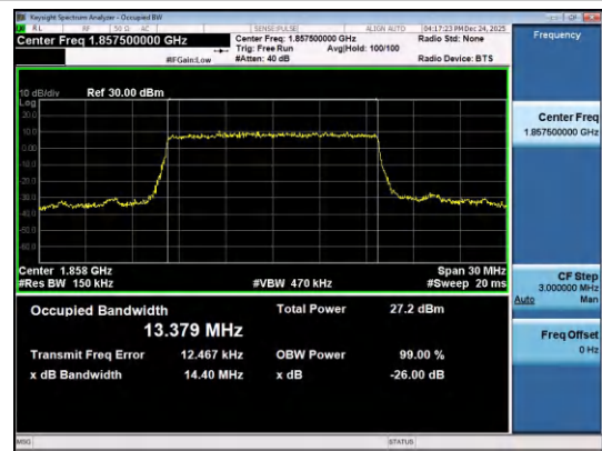
Band2-15MHz-QPSK-18675-75RB#0-PASS
