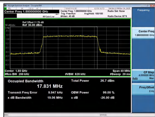
Band2-20MHz-16QAM-18900-100RB#0-PASS
