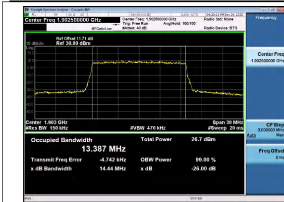
Band2-15MHz-16QAM-19125-75RB#0-PASS
