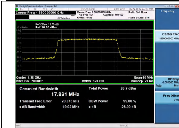
Band2-20MHz-16QAM-18900-100RB#0-PASS
