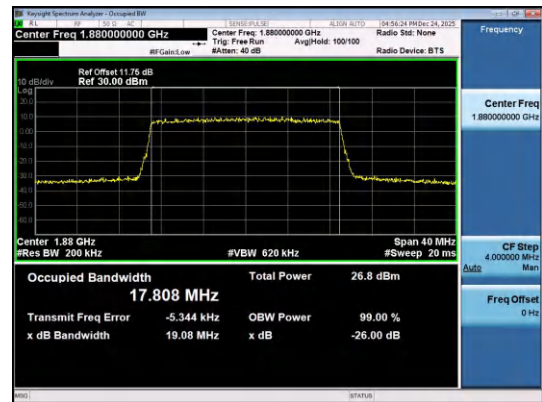
Band2-20MHz-16QAM-18900-100RB#0-PASS
