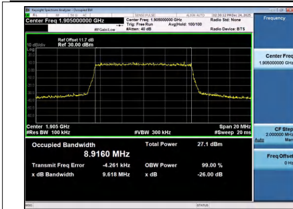
Band2-10MHz-16QAM-19150-50RB#0-PASS
