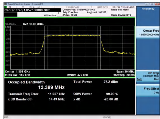
Band2-15MHz-QPSK-18675-75RB#0-PASS
