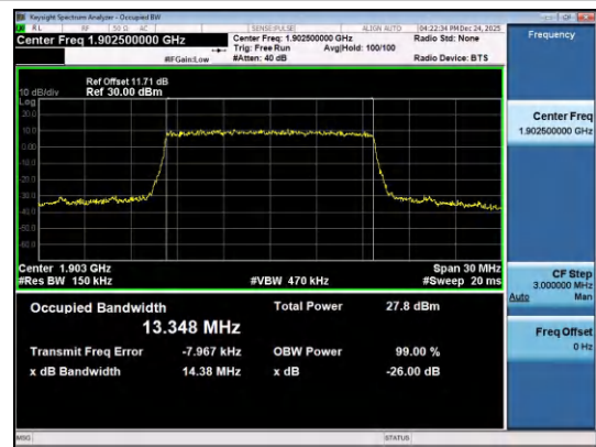
Band2-15MHz-QPSK-19125-75RB#0-PASS
