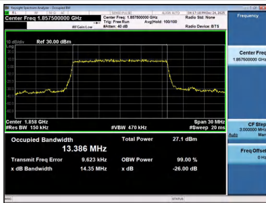
Band2-15MHz-QPSK-18675-75RB#0-PASS
