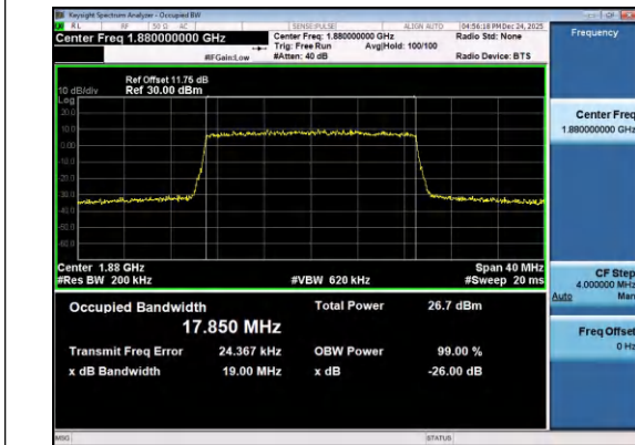
Band2-20MHz-16QAM-18900-100RB#0-PASS
