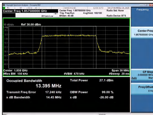
Band2-15MHz-QPSK-18675-75RB#0-PASS
