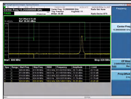
Band26(814-824)-10MHz-QPSK-26740-1RB#49-PASS
