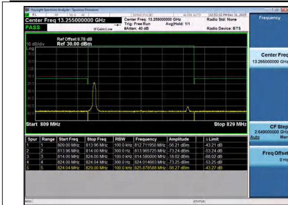
Band26(814-824)-10MHz-QPSK-26740-1RB#0-PASS
