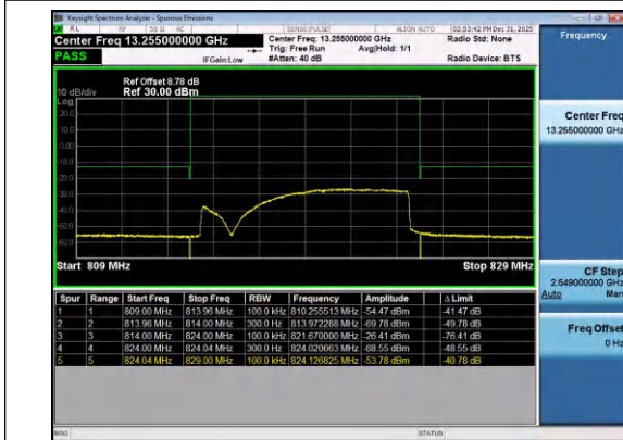
Band26(814-824)-10MHz-QPSK-26740-50RB#0-PASS
