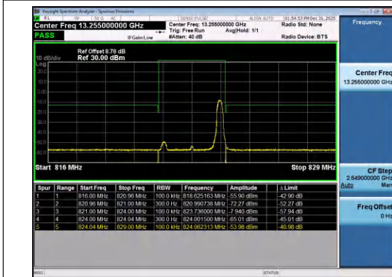
Band26(814-824)-3MHz-16QAM-26775-1RB#14-PASS
