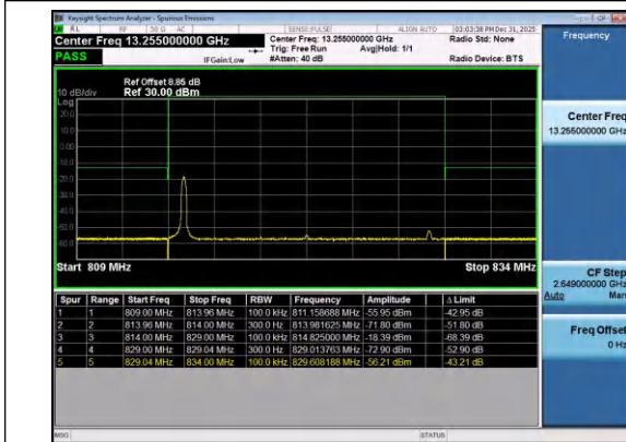
Band26(814-824)-10MHz-16QAM-26740-1RB#49-PAS
