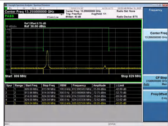
Band26(814-824)-10MHz-16QAM-26740-1RB#0-PASS
