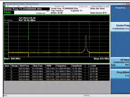
Band26(814-824)-10MHz-16QAM-26740-50RB#0-PAS
