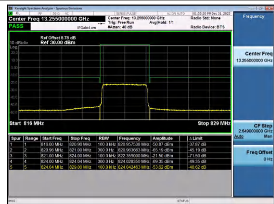
Band26(814-824)-3MHz-16QAM-26775-15RB#0-PASS
