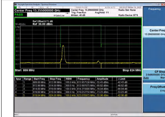
Band26(814-824)-5MHz-QPSK-26715-1RB#0-PASS
