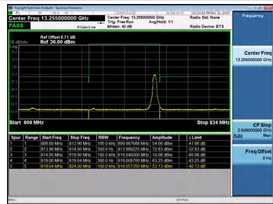
Band26(814-824)-5MHz-QPSK-26715-1RB#24-PASS
