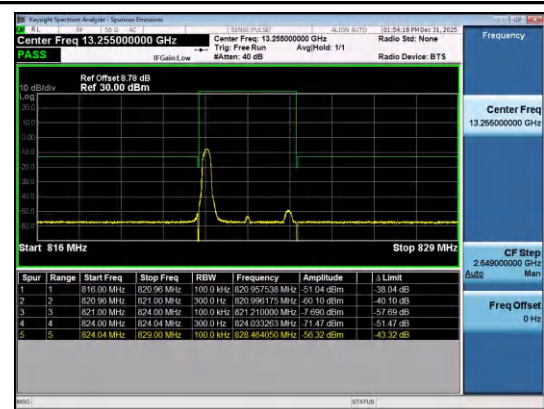
Band26(814-824)-3MHz-16QAM-26775-1RB#0-PASS
