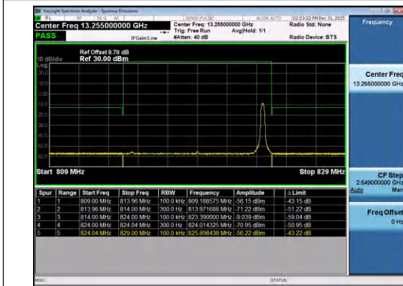
Band26(814-824)-10MHz-16QAM-26740-1RB#49-PAS
