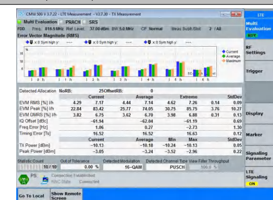
Band26(814-824)-5MHz-16QAM-26715-25RB#0-PASS
