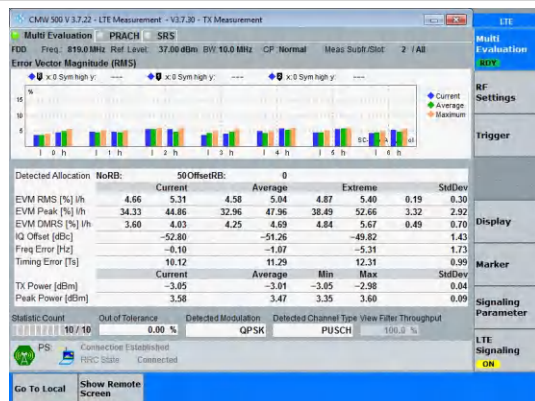
Band26(814-824)-10MHz-QPSK-26740-50RB#0-PASS
