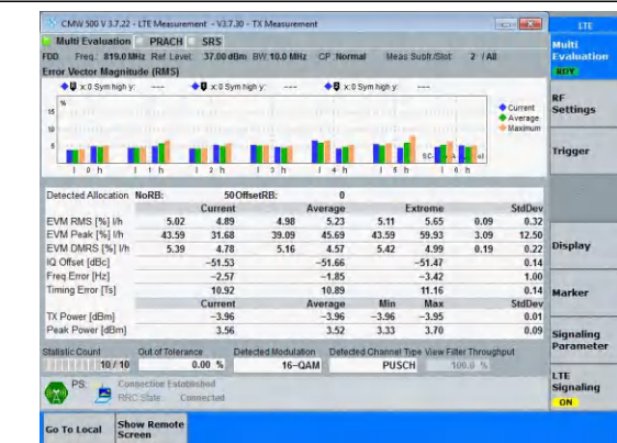
Band26(814-824)-10MHz-16QAM-26740-50RB#0-PASS
