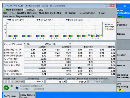
Band26(814-824)-1.4MHz-QPSK-26783-6RB#0-PASS
