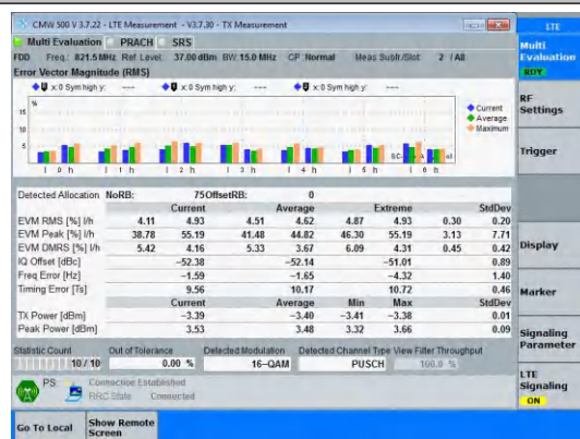
Band26(814-824)-15MHz-16QAM-26765-75RB#0-PASS
