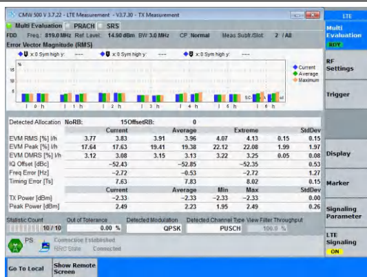
Band26(814-824)-3MHz-QPSK-26740-15RB#0-PASS
