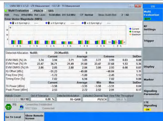
Band26(814-824)-5MHz-16QAM-26740-25RB#0-PASS
