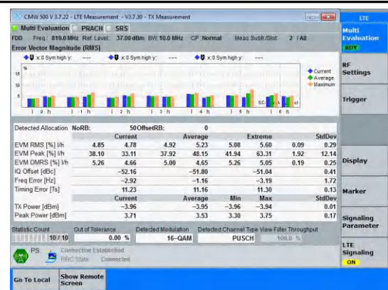
Band26(814-824)-10MHz-16QAM-26740-50RB#0-PAS
