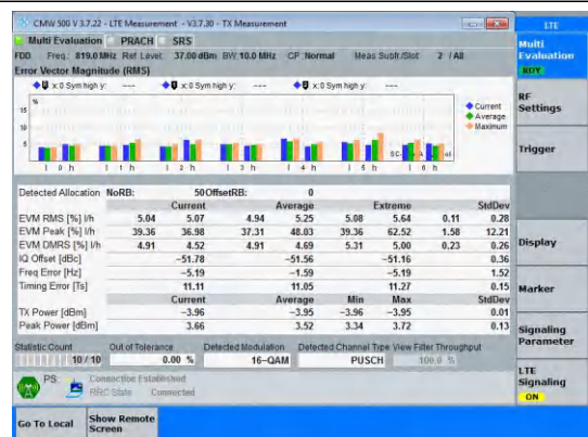
Band26(814-824)-10MHz-16QAM-26740-50RB#0-PASS
