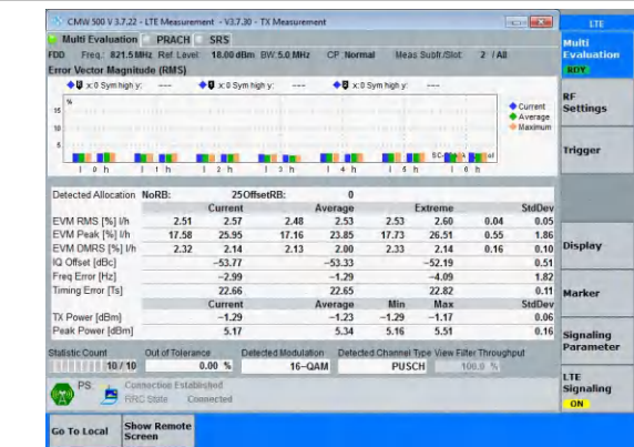
Band26(814-824)-5MHz-16QAM-26765-25RB#0-PASS
