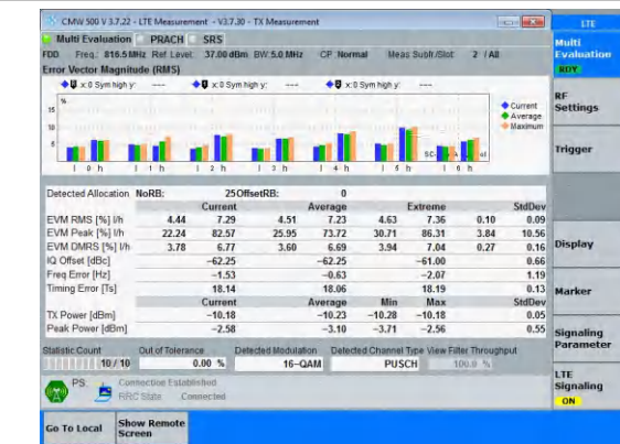
Band26(814-824)-5MHz-16QAM-26715-25RB#0-PASS
