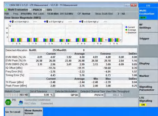
Band26(814-824)-5MHz-QPSK-26740-25RB#0-PASS
