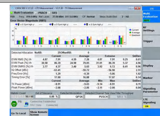
Band26(814-824)-5MHz-QPSK-26715-25RB#0-PASS
