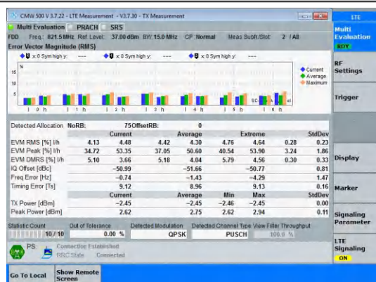
Band26(814-824)-15MHz-QPSK-26765-75RB#0-PASS
