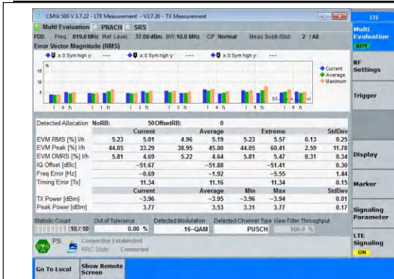
Band26(814-824)-10MHz-16QAM-26740-50RB#0-PAS
