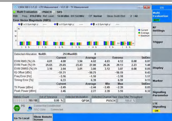
Band26(814-824)-5MHz-QPSK-26740-25RB#0-PASS
