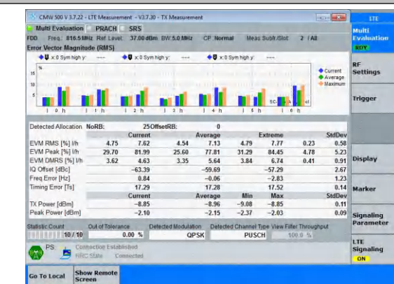
Band26(814-824)-5MHz-QPSK-26715-25RB#0-PASS
