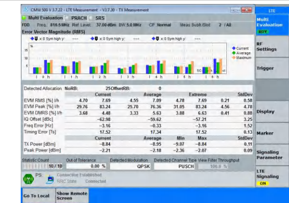
Band26(814-824)-5MHz-QPSK-26715-25RB#0-PASS
