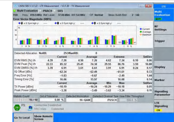
Band26(814-824)-5MHz-16QAM-26715-25RB#0-PASS
