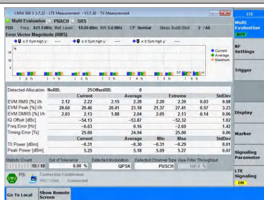
Band26(814-824)-5MHz-QPSK-26765-25RB#0-PASS
