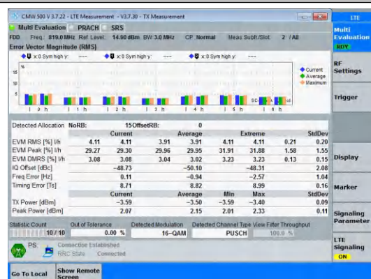
Band26(814-824)-3MHz-16QAM-26740-15RB#0-PASS
