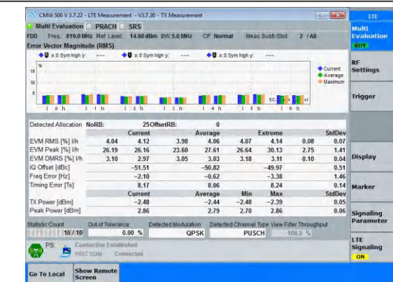
Band26(814-824)-5MHz-QPSK-26740-25RB#0-PASS
