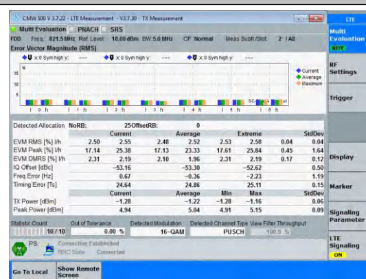
Band26(814-824)-5MHz-16QAM-26765-25RB#0-PASS
