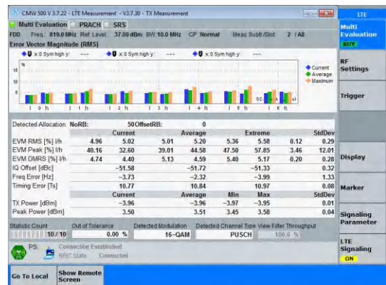
Band26(814-824)-10MHz-16QAM-26740-50RB#0-PASS
