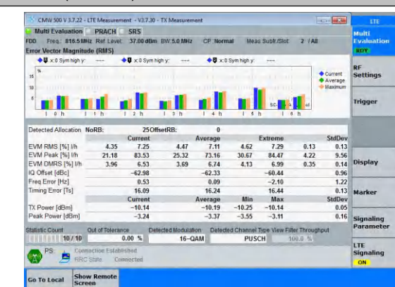
Band26(814-824)-5MHz-16QAM-26715-25RB#0-PASS
