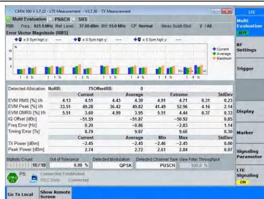
Band26(814-824)-15MHz-QPSK-26765-75RB#0-PASS
