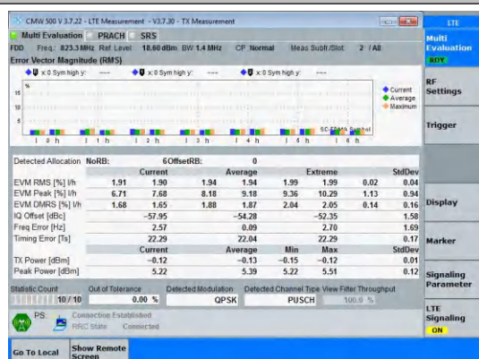
Band26(814-824)-1.4MHz-QPSK-26783-6RB#0-PASS
