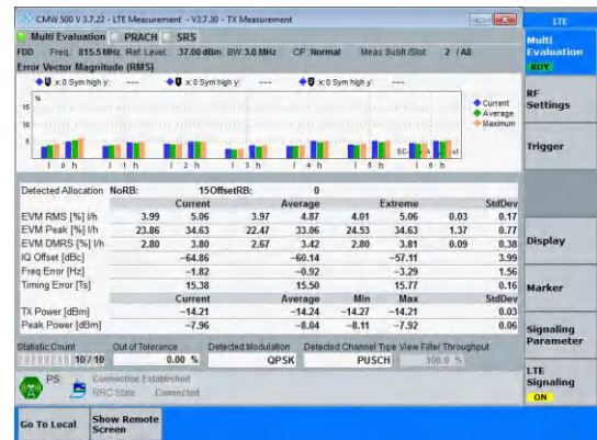
Band26(814-824)-3MHz-QPSK-26705-15RB#0-PASS
