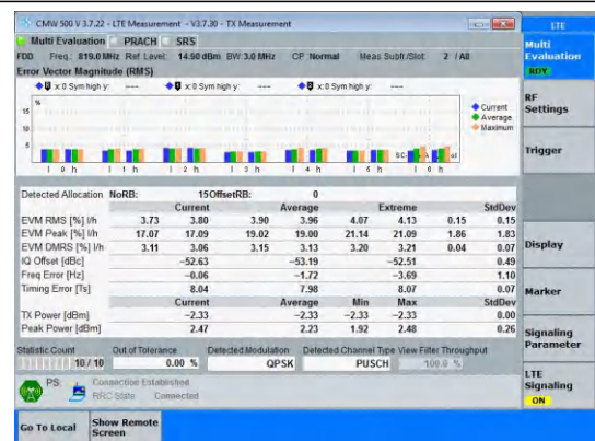
Band26(814-824)-3MHz-QPSK-26740-15RB#0-PASS
