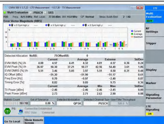
Band26(814-824)-15MHz-QPSK-26765-75RB#0-PASS
