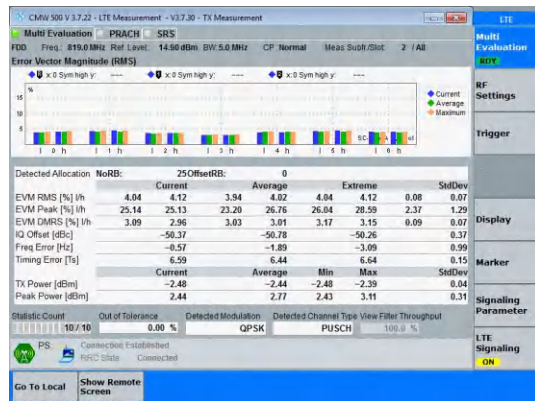
Band26(814-824)-5MHz-QPSK-26740-25RB#0-PASS
