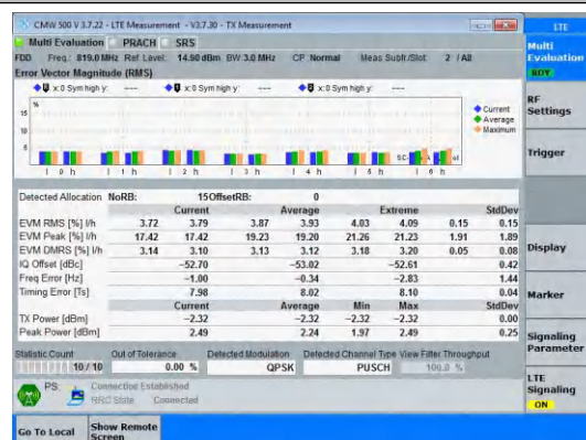
Band26(814-824)-3MHz-QPSK-26740-15RB#0-PASS
