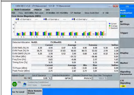
Band26(814-824)-15MHz-QPSK-26765-75RB#0-PASS
