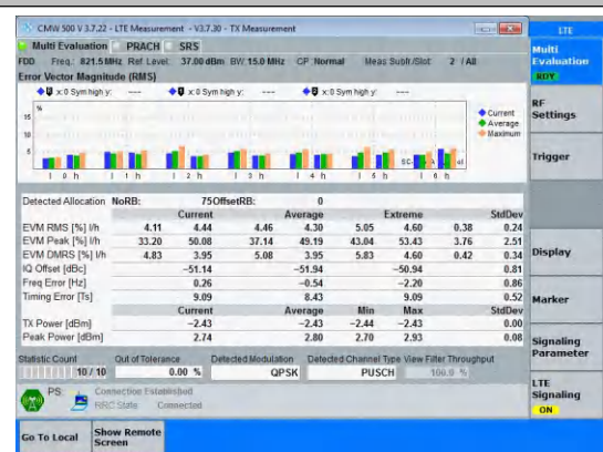
Band26(814-824)-15MHz-QPSK-26765-75RB#0-PASS
