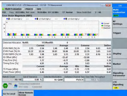
Band26(814-824)-3MHz-16QAM-26775-15RB#0-PASS
