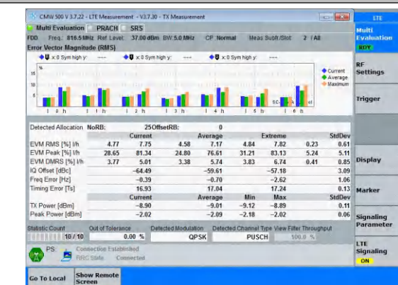
Band26(814-824)-5MHz-QPSK-26715-25RB#0-PASS
