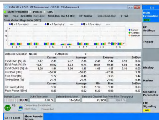
Band26(814-824)-1.4MHz-16QAM-26783-6RB#0-PAS
