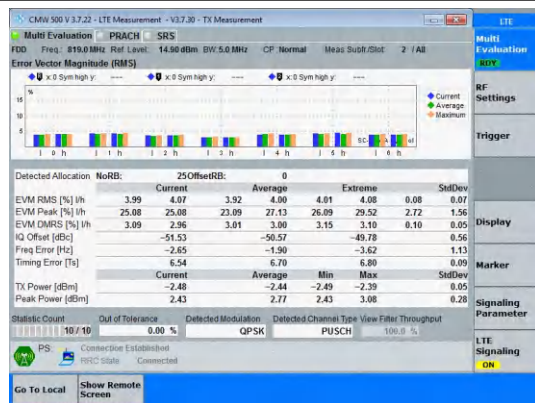
Band26(814-824)-5MHz-QPSK-26740-25RB#0-PASS
