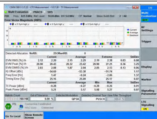
Band26(814-824)-5MHz-QPSK-26765-25RB#0-PASS
