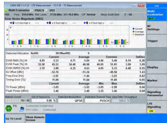
Band26(814-824)-10MHz-QPSK-26740-50RB#0-PASS
