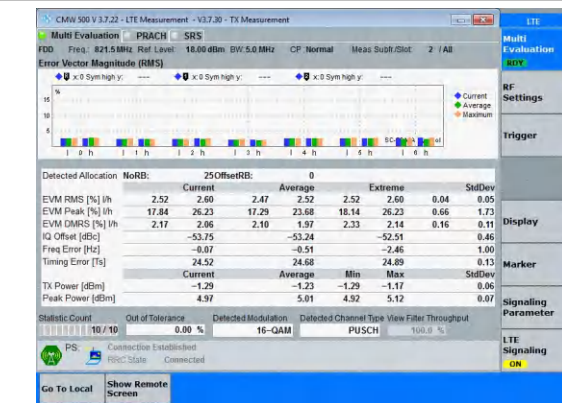
Band26(814-824)-5MHz-16QAM-26765-25RB#0-PASS
