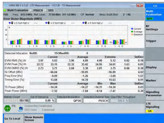
Band26(814-824)-3MHz-QPSK-26705-15RB#0-PASS
