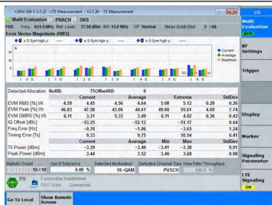
Band26(814-824)-15MHz-16QAM-26765-75RB#0-PASS
