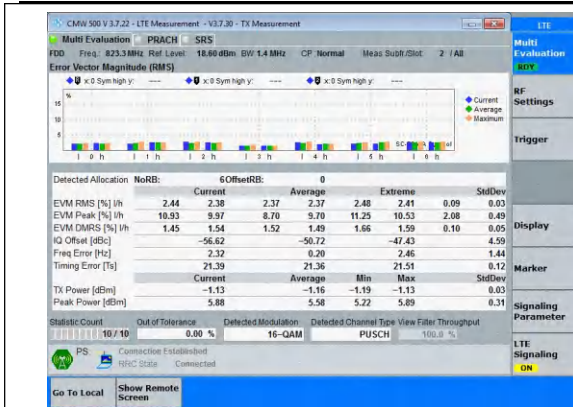
Band26(814-824)-1.4MHz-16QAM-26783-6RB#0-PAS
