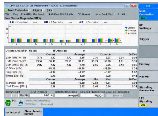
Band26(814-824)-5MHz-16QAM-26740-25RB#0-PASS
