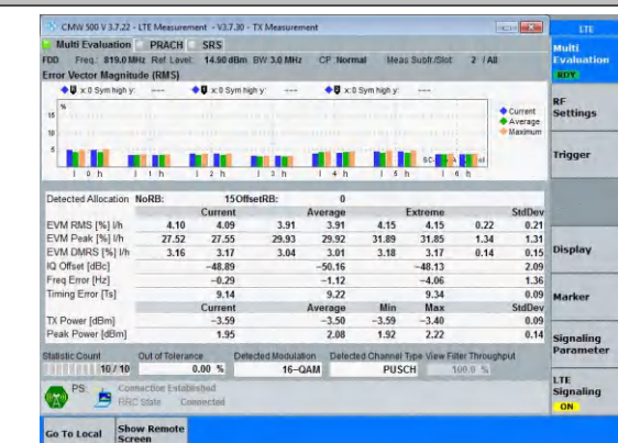
Band26(814-824)-3MHz-16QAM-26740-15RB#0-PASS
