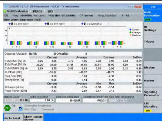
Band26(814-824)-5MHz-16QAM-26740-25RB#0-PASS
