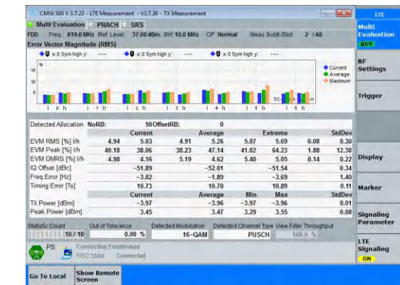
Band26(814-824)-10MHz-16QAM-26740-50RB#0-PASS
