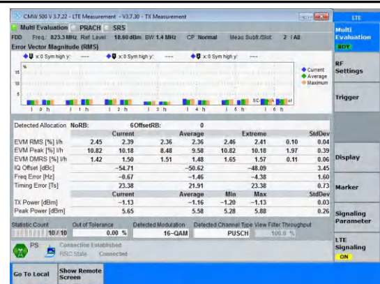
Band26(814-824)-1.4MHz-16QAM-26783-6RB#0-PAS
