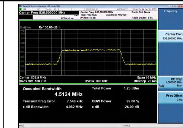
Band26(824-849)-5MHz-16QAM-26915-25RB#0-PASS
