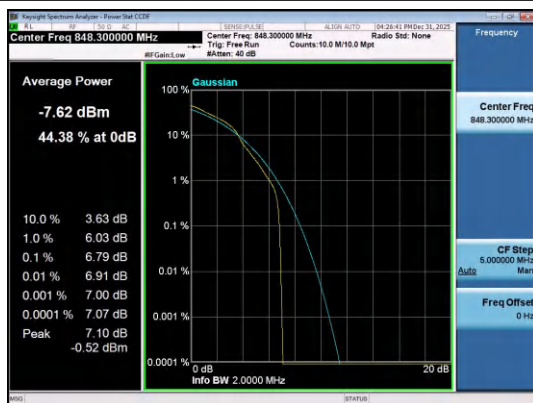
Band26(824-849)-1.4MHz-16QAM-27033-1RB#0-PAS
