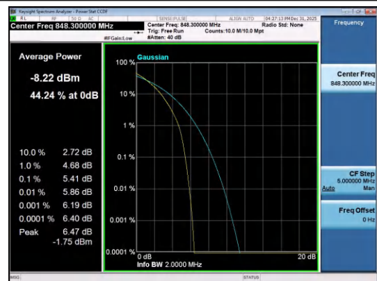
Band26(824-849)-1.4MHz-QPSK-27033-6RB#0-PASS
