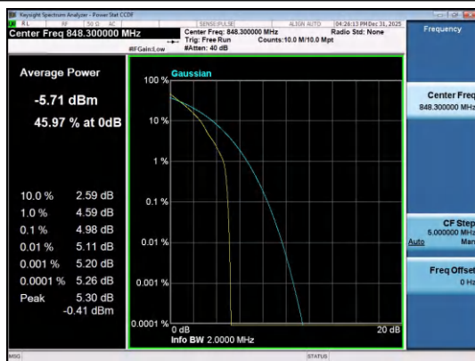
Band26(824-849)-1.4MHz-QPSK-27033-1RB#0-PASS
