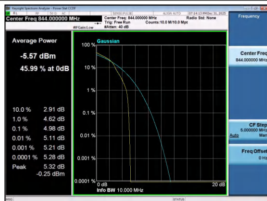
Band26(824-849)-10MHz-16QAM-26990-1RB#0-PASS
