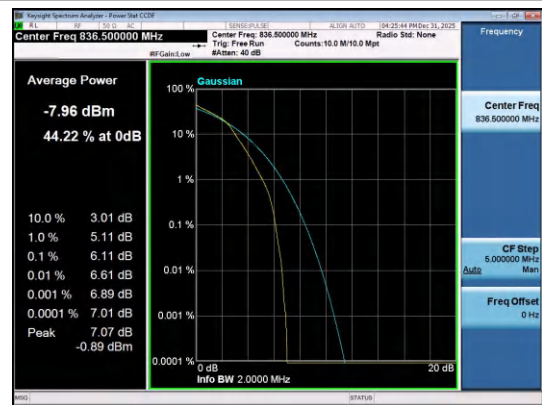
Band26(824-849)-1.4MHz-16QAM-26915-6RB#0-PAS
