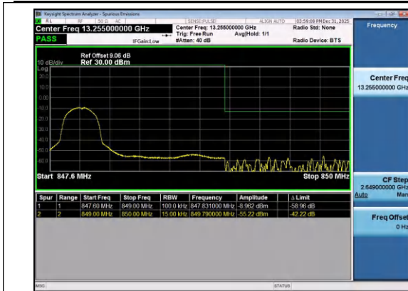
Band26(824-849)-1.4MHz-QPSK-27033-1RB#0-PASS
