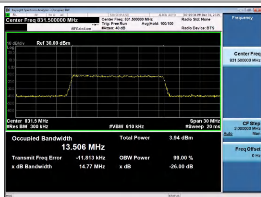
Band26(824-849)-15MHz-QPSK-26865-75RB#0-PAS
