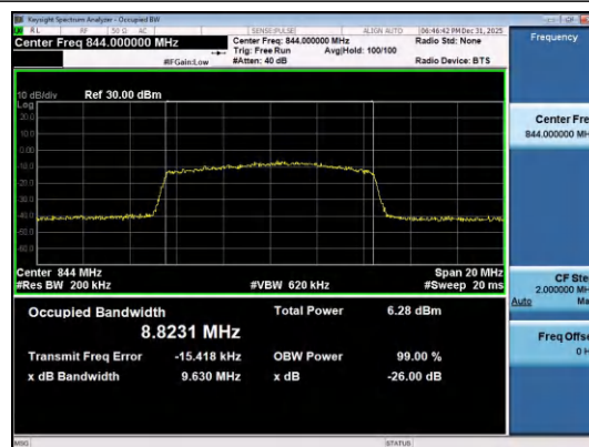
Band26(824-849)-10MHz-16QAM-26990-50RB#0-PAS
