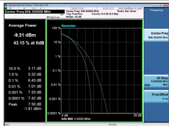
Band26(824-849)-1.4MHz-16QAM-27033-6RB#0-PAS
