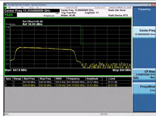
Band26(824-849)-1.4MHz-16QAM-27033-6RB#0-PAS S
