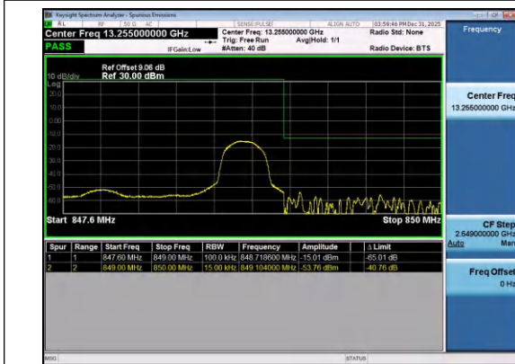
Band26(824-849)-1.4MHz-16QAM-27033-1RB#5-PAS S
