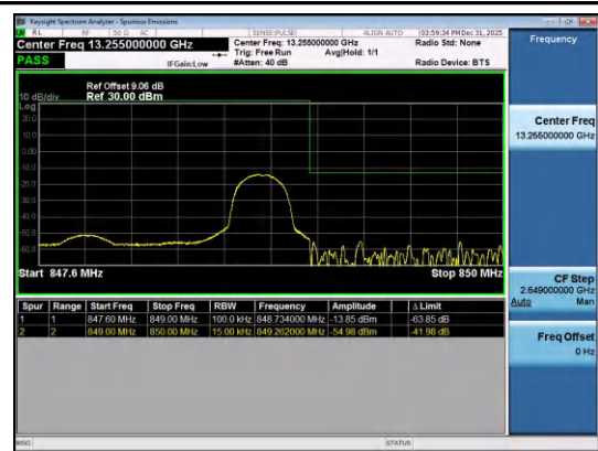
Band26(824-849)-1.4MHz-QPSK-27033-1RB#5-PASS
