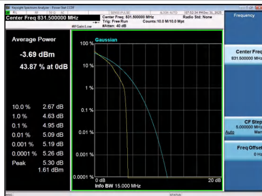
Band26(824-849)-15MHz-QPSK-26865-1RB#0-PASS
