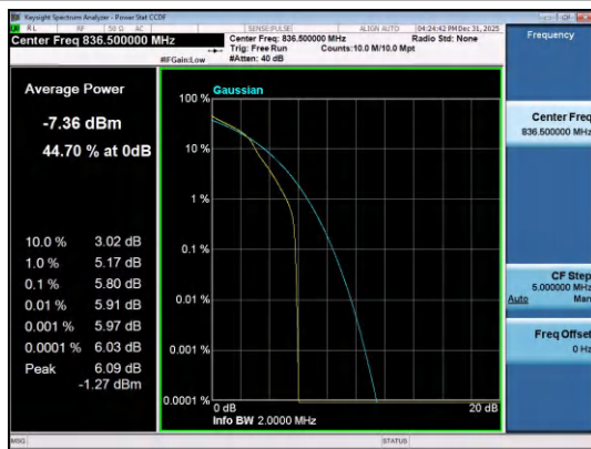
Band26(824-849)-1.4MHz-16QAM-26915-1RB#0-PAS
