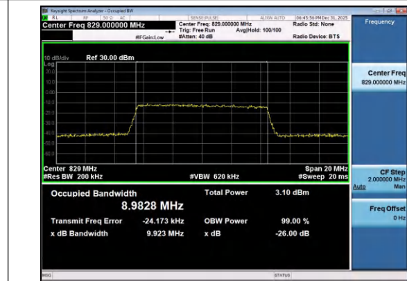
Band26(824-849)-10MHz-16QAM-26840-50RB#0-PAS
