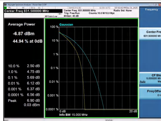
Band26(824-849)-15MHz-QPSK-26865-75RB#0-PASS
