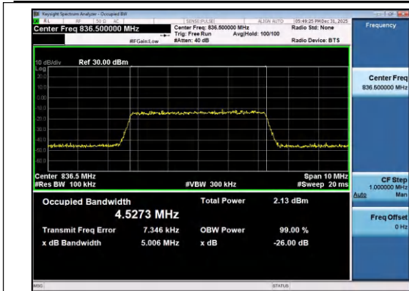
Band26(824-849)-5MHz-QPSK-26915-25RB#0-PASS
