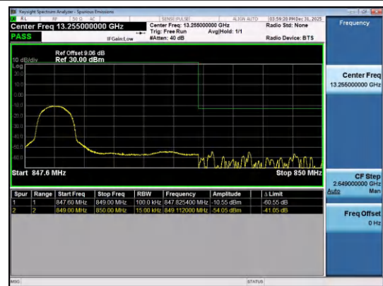
Band26(824-849)-1.4MHz-16QAM-27033-1RB#0-PAS S
