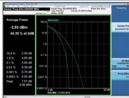
Band26(824-849)-10MHz-16QAM-26990-50RB#0-PASS
