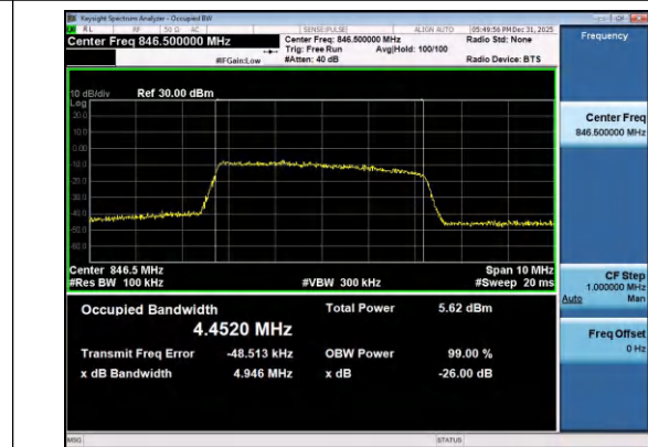
Band26(824-849)-5MHz-16QAM-27015-25RB#0-PASS
