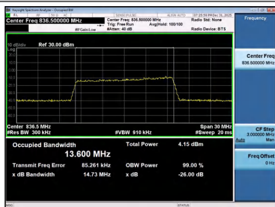
Band26(824-849)-15MHz-QPSK-26915-75RB#0-PAS
