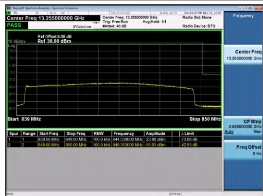
Band26(824-849)-10MHz-16QAM-26990-50RB#0-PAS
