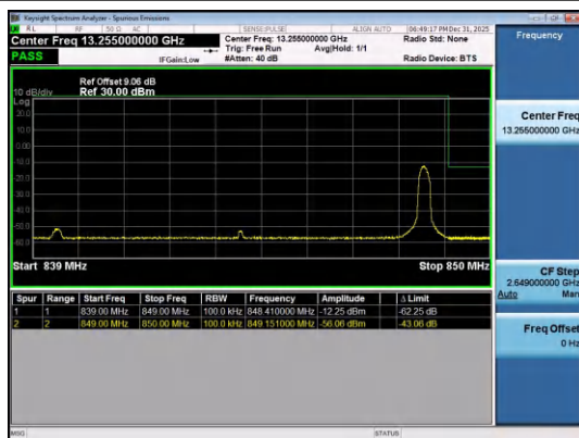
Band26(824-849)-10MHz-16QAM-26990-1RB#49-PAS
