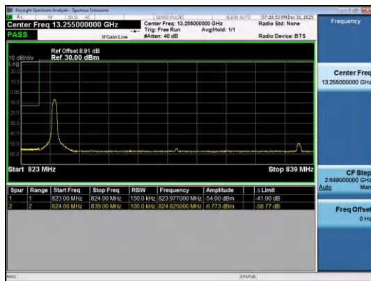
Band26(824-849)-15MHz-QPSK-26865-1RB#0-PASS
