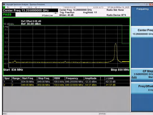
Band26(824-849)-15MHz-16QAM-26965-1RB#74-PAS
