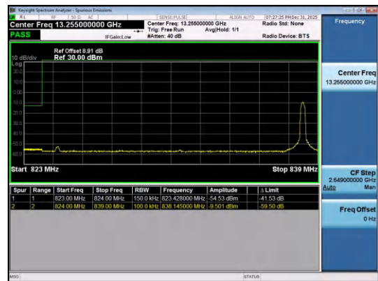
Band26(824-849)-15MHz-QPSK-26865-1RB#74-PASS
