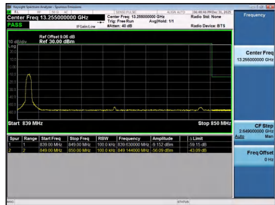
Band26(824-849)-10MHz-16QAM-26990-1RB#0-PASS
