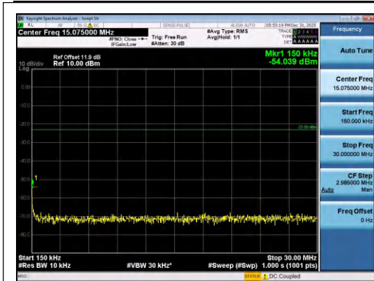
Band26(824-849)-5MHz-QPSK-26815-1RB#24-0 .15~30-PASS
