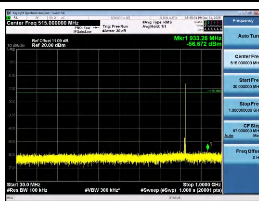
Band26(824-849)-5MHz-QPSK-26815-1RB#24-3 0~1000-PASS
