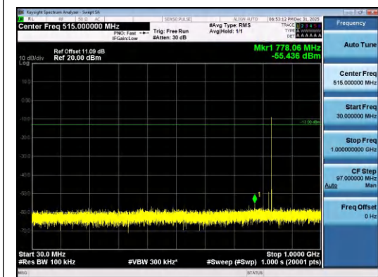
Band26(824-849)-10MHz-16QAM-26840-1RB#4 9-30~1000-PASS
