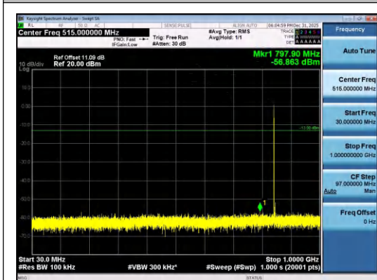
Band26(824-849)-5MHz-QPSK-27015-1RB#0-30 ~1000-PASS
