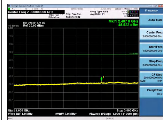
Band26(824-849)-5MHz-QPSK-26815-1RB#24-1 000~3000-PASS
