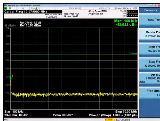
Band26(824-849)-5MHz-QPSK-27015-1RB#0-0. 15~30-PASS
