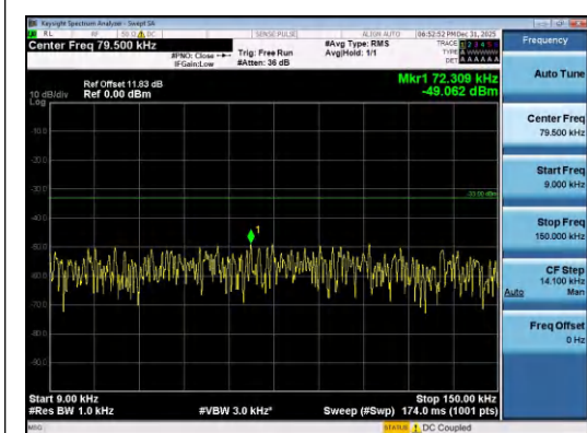
Band26(824-849)-10MHz-16QAM-26840-1RB#4 9-0.009~0.15-PASS
