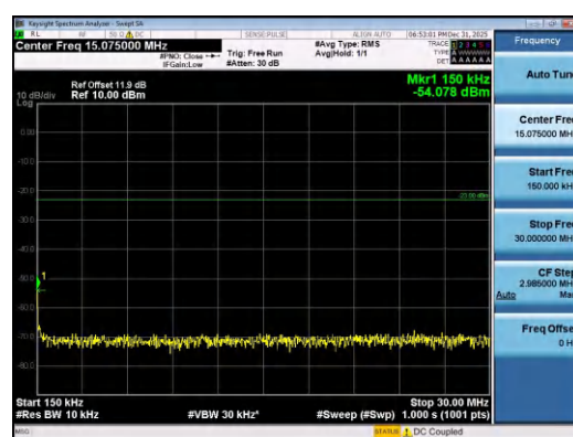
Band26(824-849)-10MHz-16QAM-26840-1RB#4 9-0.15~30-PASS
