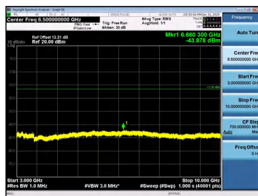
Band26(824-849)-5MHz-QPSK-26815-1RB#24-3 000~10000-PASS
