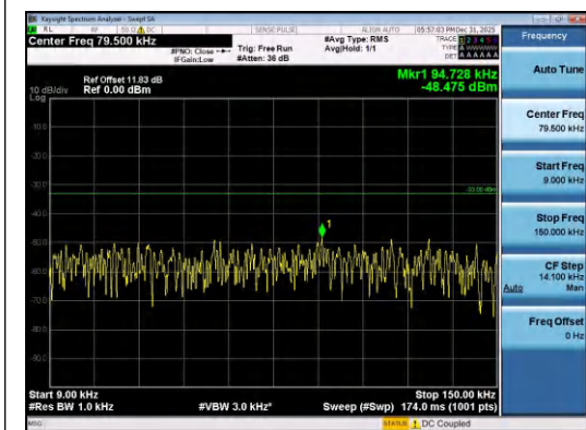
Band26(824-849)-5MHz-QPSK-26815-25RB#0-0 .009~0.15-PASS
