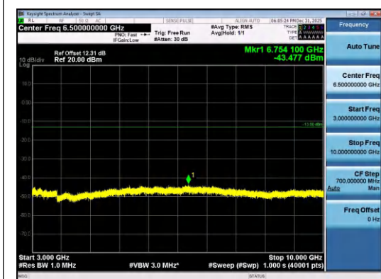
Band26(824-849)-5MHz-QPSK-27015-1RB#0-30 00~10000-PASS
