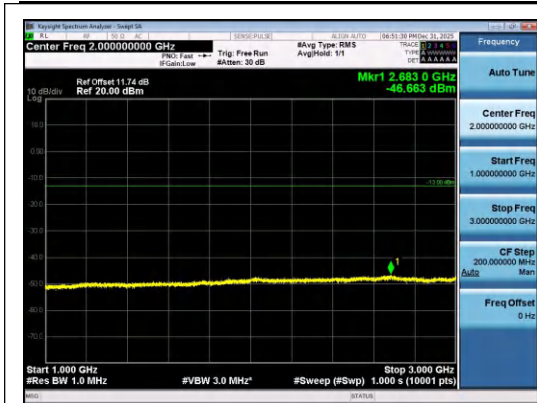
Band26(824-849)-10MHz-16QAM-26840-1RB#0 -1000~3000-PASS
