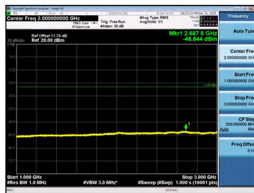
Band26(824-849)-10MHz-16QAM-26840-1RB#4 9-1000~3000-PASS
