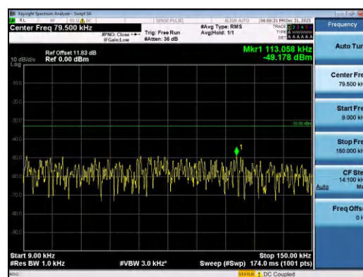
Band26(824-849)-5MHz-QPSK-27015-1RB#24-0 .009~0.15-PASS
