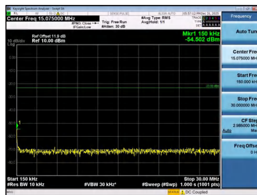
Band26(824-849)-5MHz-QPSK-26815-25RB#0-0 .15~30-PASS
