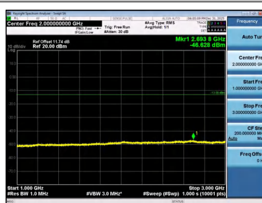
Band26(824-849)-5MHz-QPSK-27015-1RB#0-10 00~3000-PASS
