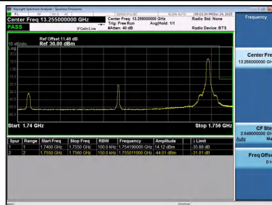
Band4-15MHz-QPSK-20325-1RB#74-PASS
