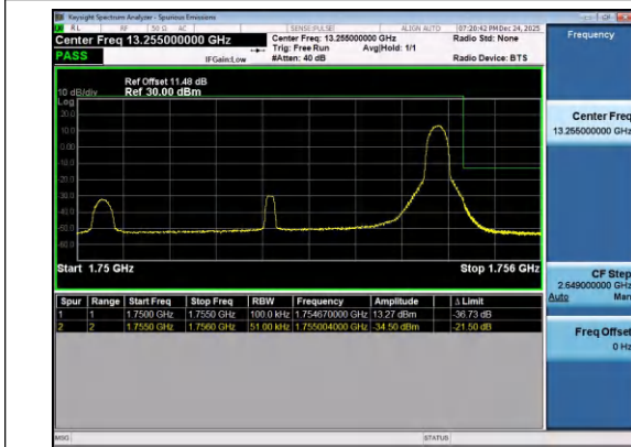
Band4-5MHz-16QAM-20375-1RB#24-PASS
