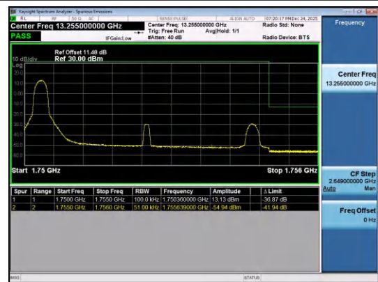
Band4-5MHz-16QAM-20375-1RB#0-PASS
