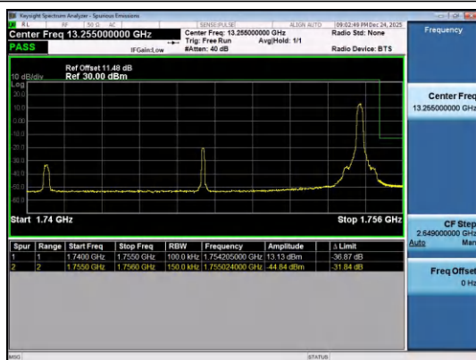
Band4-15MHz-16QAM-20325-1RB#74-PASS
