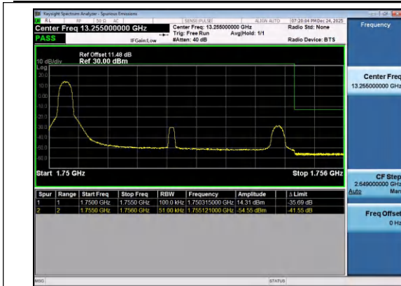
Band4-5MHz-QPSK-20375-1RB#0-PASS
