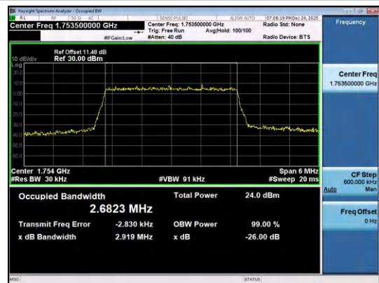
Band4-3MHz-16QAM-20385-15RB#0-PASS
