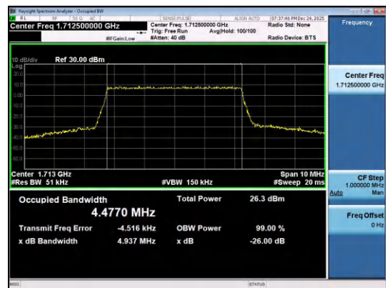
Band4-5MHz-QPSK-19975-25RB#0-PASS
