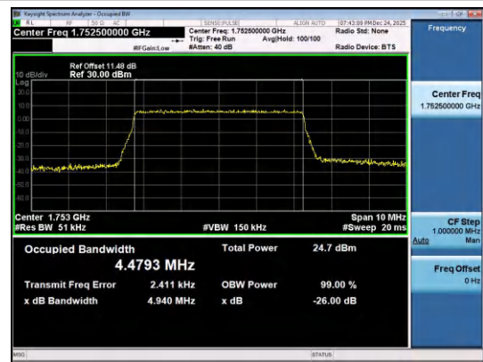
Band4-5MHz-16QAM-20375-25RB#0-PASS
