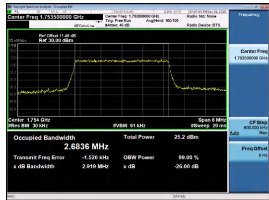
Band4-3MHz-QPSK-20385-15RB#0-PASS
