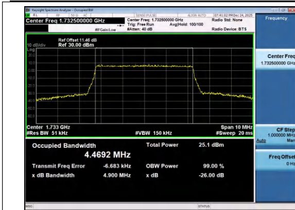
Band4-5MHz-16QAM-20175-25RB#0-PASS
