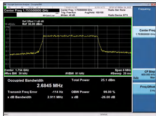
Band4-3MHz-QPSK-20385-15RB#0-PASS
