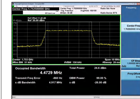
Band4-5MHz-16QAM-20375-25RB#0-PASS
