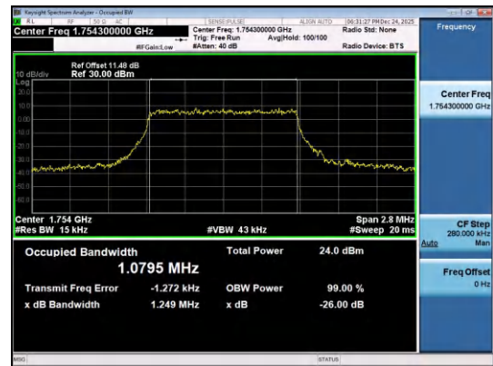
Band4-1.4MHz-16QAM-20393-6RB#0-PASS
