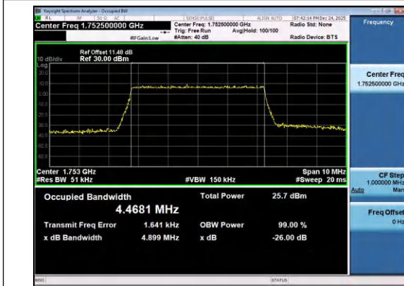
Band4-5MHz-QPSK-20375-25RB#0-PASS
