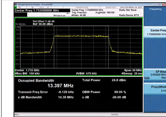
Band4-15MHz-16QAM-20175-75RB#0-PASS
