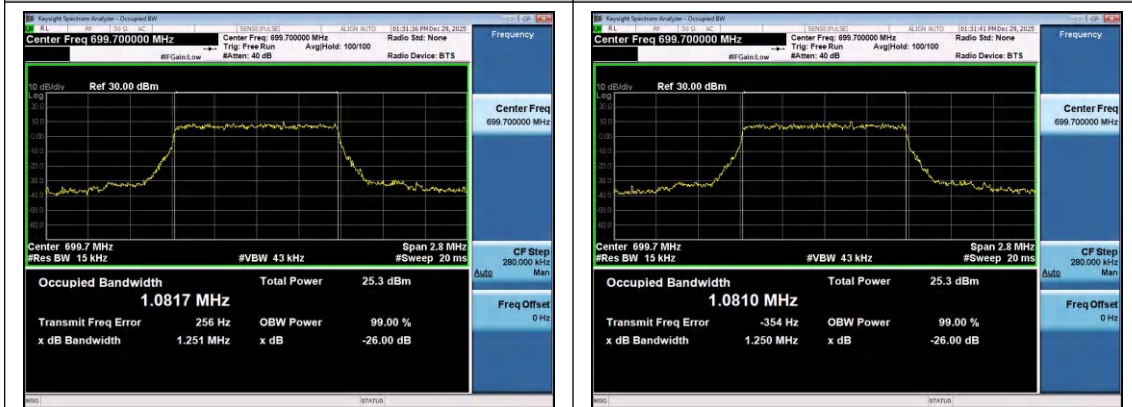
Band12-1.4MHz-QPSK-23017-6RB#0-PASS
