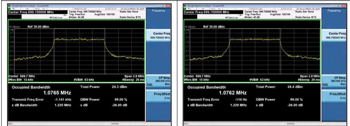
Band12-1.4MHz-16QAM-23017-6RB#0-PASS
