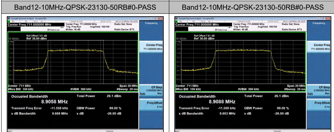
Band12-10MHz-QPSK-23130-50RB#0-PASS
