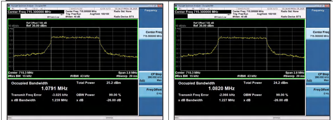
Band12-1.4MHz-QPSK-23173-6RB#0-PASS
