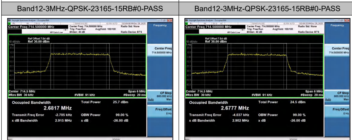
Band12-3MHz-QPSK-23165-15RB#0-PASS
