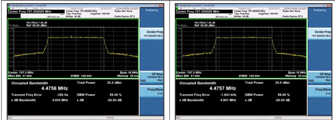
Band12-5MHz-16QAM-23095-25RB#0-PASS
