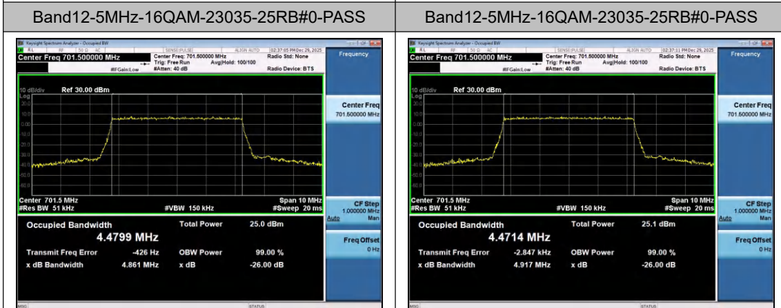
Band12-5MHz-16QAM-23035-25RB#0-PASS
