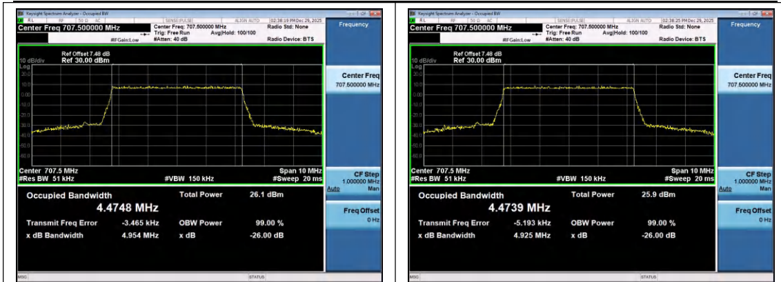
Band12-5MHz-QPSK-23095-25RB#0-PASS
