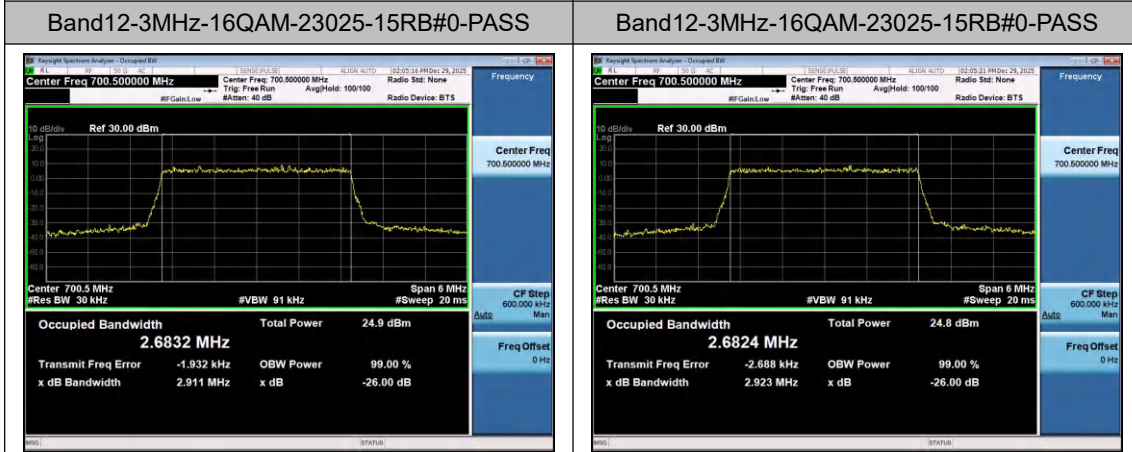
Band12-3MHz-16QAM-23025-15RB#0-PASS
