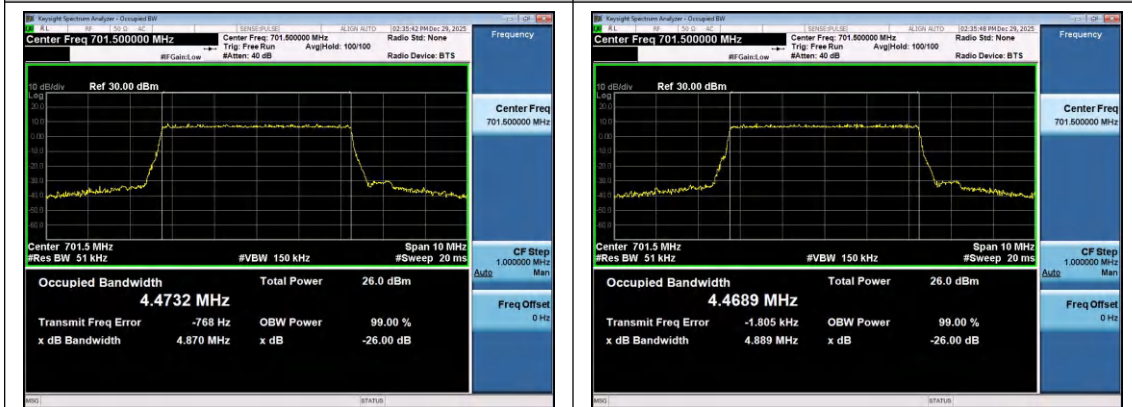
Band12-5MHz-QPSK-23035-25RB#0-PASS
