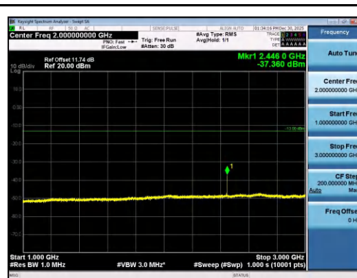
Band26(814-824)-1.4MHz-QPSK-26697-6RB#0- 1000~3000-PASS
