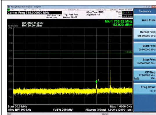
Band26(814-824)-3MHz-QPSK-26740-1RB#0-30 ~1000-PASS
