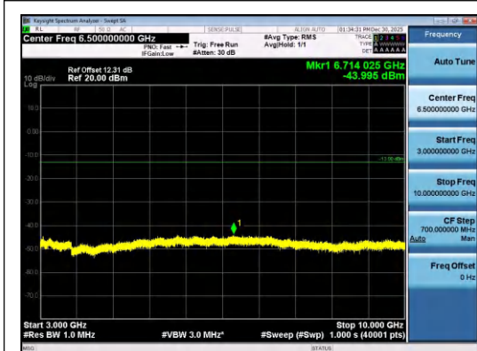
Band26(814-824)-1.4MHz-QPSK-26697-6RB#0- 3000~10000-PASS
