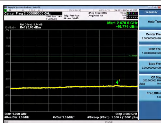
Band26(814-824)-3MHz-QPSK-26740-1RB#0-10 00~3000-PASS
