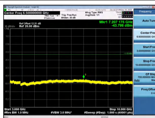
Band26(814-824)-1.4MHz-QPSK-26697-1RB#5- 3000~10000-PASS
