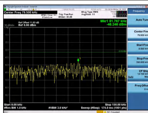
Band26(814-824)-1.4MHz-16QAM-26697-1RB#0 -0.009~0.15-PASS
