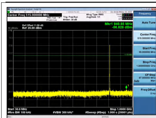
Band26(814-824)-1.4MHz-QPSK-26697-6RB#0- 30~1000-PASS
