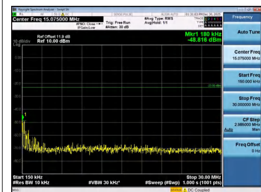
Band26(814-824)-1.4MHz-16QAM-26697-1RB#0 -0.15~30-PASS
