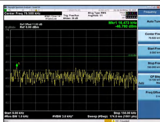
Band26(814-824)-1.4MHz-16QAM-26740-1RB#0 -0.009~0.15-PASS
