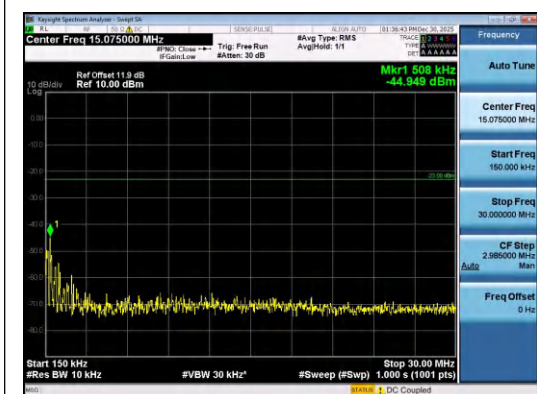
Band26(814-824)-1.4MHz-16QAM-26740-1RB#0 -0.15~30-PASS
