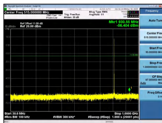
Band26(814-824)-1.4MHz-16QAM-26697-1RB#0 -30~1000-PASS
