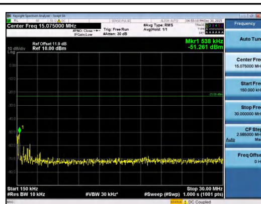
Band26(814-824)-3MHz-QPSK-26740-1RB#0-0. 15~30-PASS
