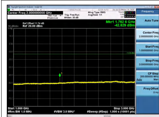
Band26(814-824)-1.4MHz-QPSK-26697-1RB#5- 1000~3000-PASS
