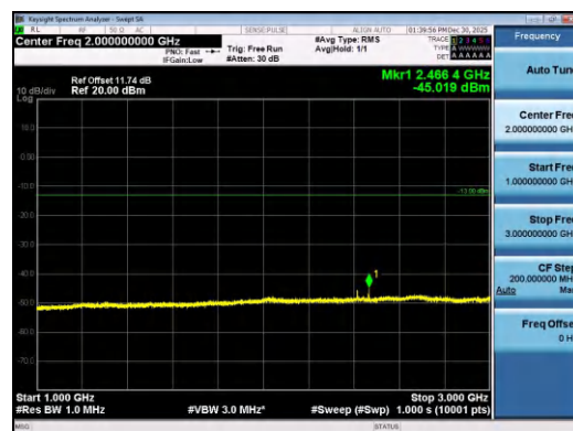
Band26(814-824)-1.4MHz-QPSK-26740-6RB#0- 1000~3000-PASS
