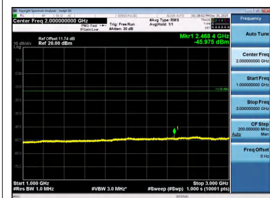
Band26(814-824)-1.4MHz-QPSK-26740-1RB#5-1000~3000-PASS
