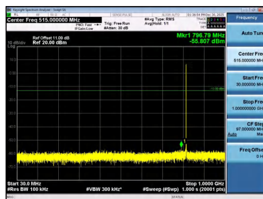
Band26(814-824)-1.4MHz-16QAM-26740-1RB#0 -30~1000-PASS
