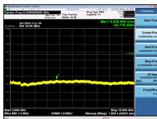
Band26(814-824)-1.4MHz-QPSK-26740-1RB#5-3000~10000-PASS
