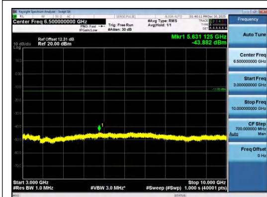
Band26(814-824)-1.4MHz-QPSK-26740-6RB#0- 3000~10000-PASS
