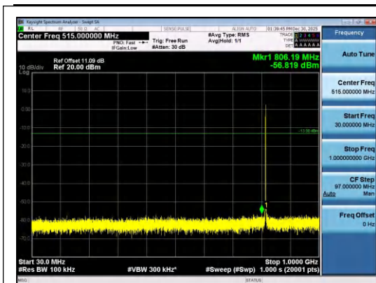
Band26(814-824)-1.4MHz-QPSK-26740-6RB#0- 30~1000-PASS
