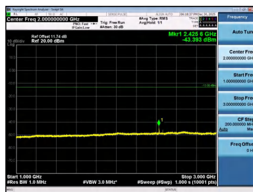
Band26(814-824)-10MHz-16QAM-26740-1RB#4 9-1000~3000-PASS
