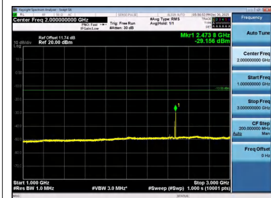
Band26(814-824)-5MHz-QPSK-26715-25RB#0-1 000~3000-PASS
