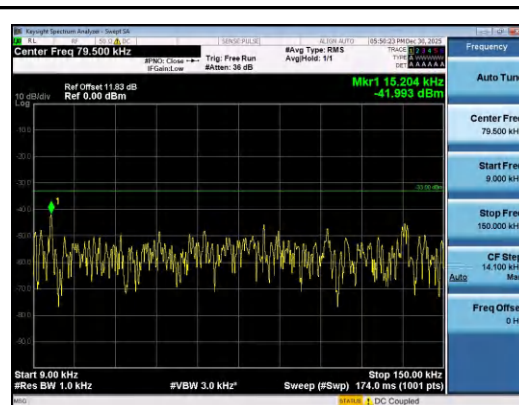
Band26(814-824)-5MHz-QPSK-26715-25RB#0-0 .009~0.15-PASS
