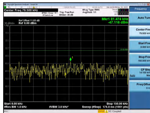
Band26(814-824)-10MHz-16QAM-26740-50RB# 0-0.009~0.15-PASS
