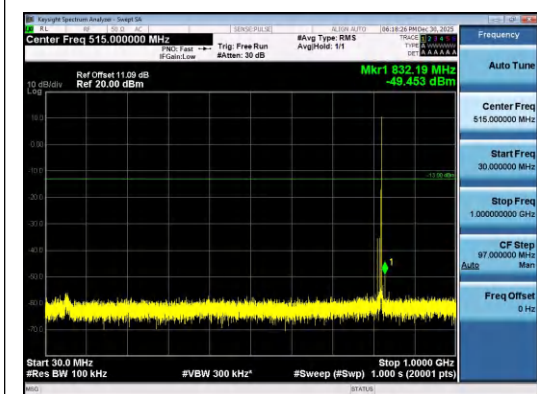
Band26(814-824)-10MHz-16QAM-26740-1RB#4 9-30~1000-PASS
