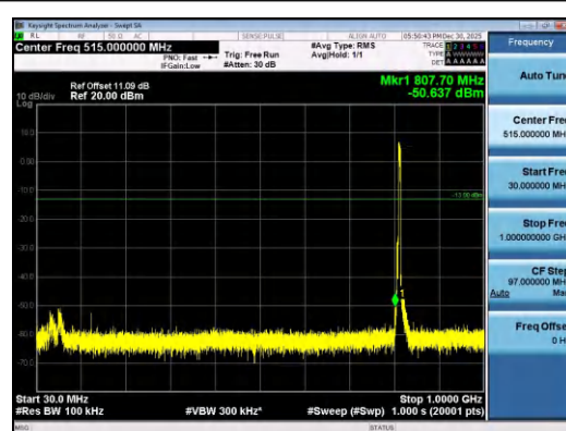
Band26(814-824)-5MHz-QPSK-26715-25RB#0-3 0~1000-PASS
