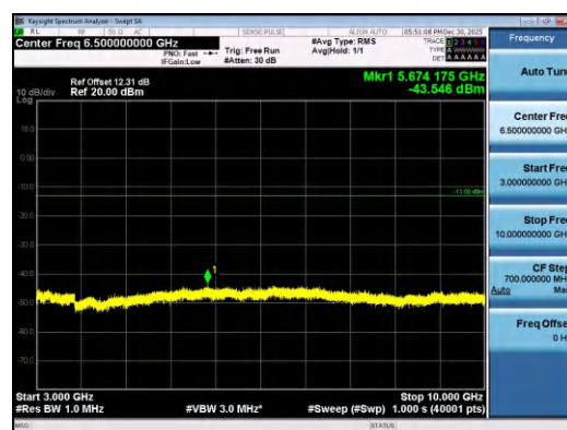
Band26(814-824)-5MHz-QPSK-26715-25RB#0-3 000~10000-PASS
