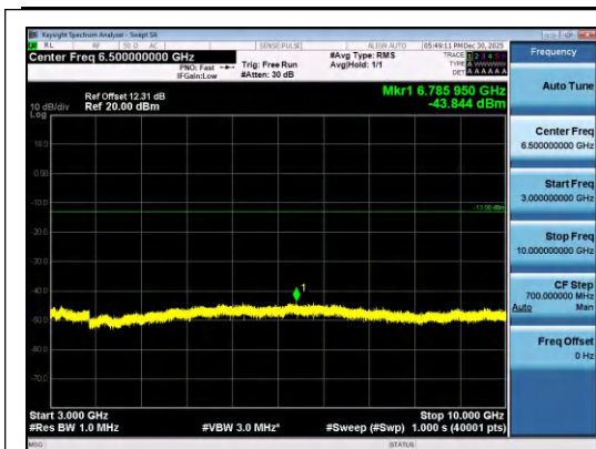
Band26(814-824)-5MHz-QPSK-26715-1RB#24-3 000~10000-PASS
