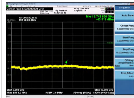
Band26(814-824)-10MHz-16QAM-26740-1RB#4 9-3000~10000-PASS
