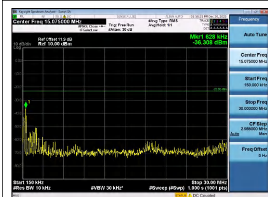
Band26(814-824)-5MHz-QPSK-26715-25RB#0-0 .15~30-PASS
