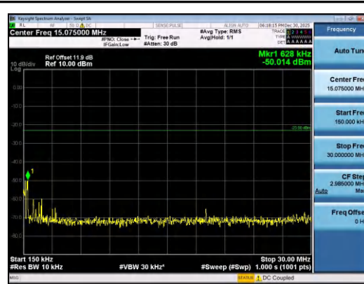
Band26(814-824)-10MHz-16QAM-26740-1RB#4 9-0.15~30-PASS
