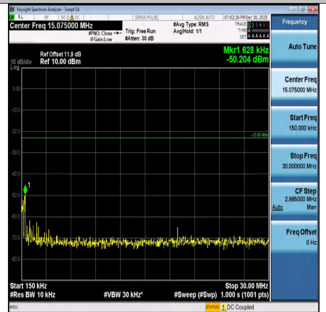
Band26(824-849)-1.4MHz-QPSK-27033-6RB#0-0.15~30-P ASS
