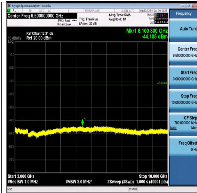
Band26(824-849)-1.4MHz-QPSK-26915-6RB#0-3000~100 00-PASS
