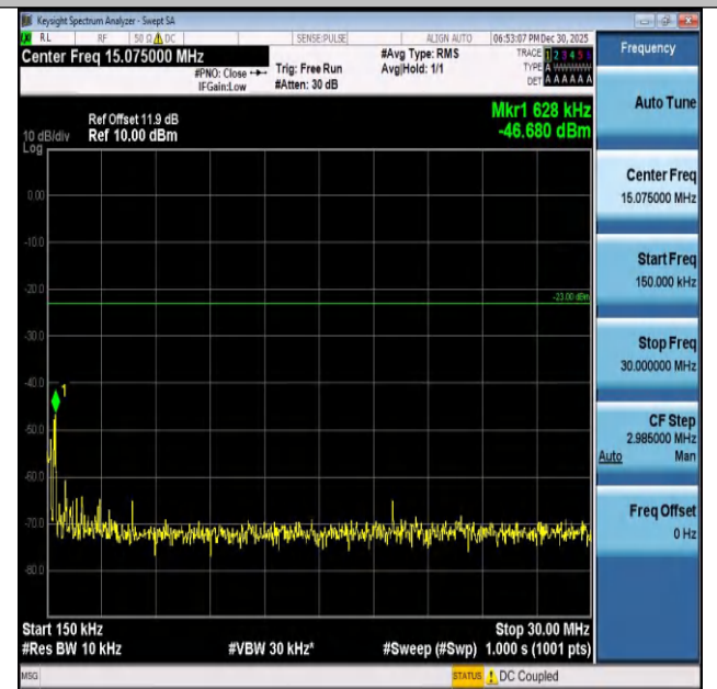
Band26(824-849)-1.4MHz-QPSK-26915-1RB#0-0.15~30-P ASS
