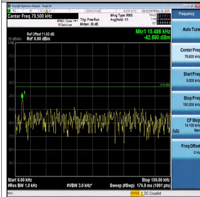
Band26(824-849)-1.4MHz-QPSK-26915-1RB#0-0.009~0.1 5-PASS
