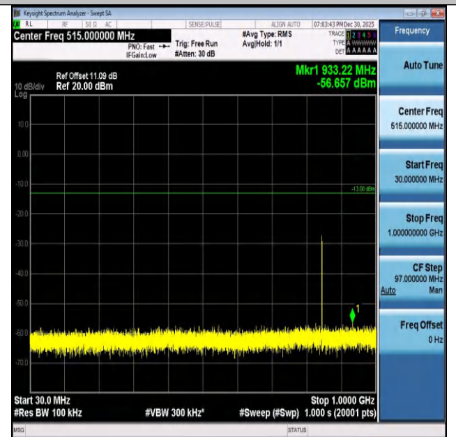
Band26(824-849)-1.4MHz-16QAM-27033-6RB#0-30~1000 -PASS
