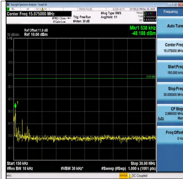
Band26(824-849)-3MHz-QPSK-26805-1RB#14-0.15~30-P
