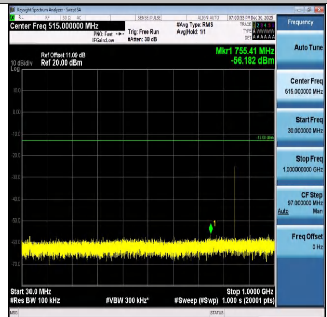
Band26(824-849)-1.4MHz-QPSK-27033-1RB#5-30~1000-PASS
