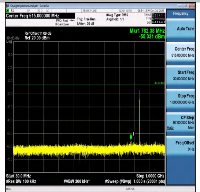
Band26(824-849)-1.4MHz-16QAM-26915-1RB#0-30~1000 -PASS
