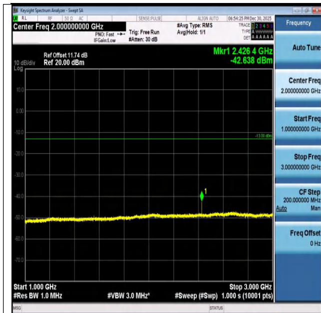
Band26(824-849)-1.4MHz-16QAM-26915-1RB#0-1000~30 00-PASS
