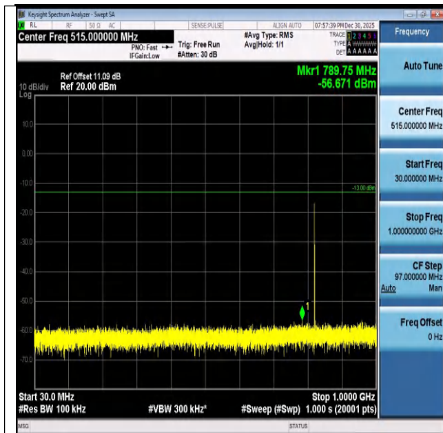
Band26(824-849)-3MHz-QPSK-26805-1RB#0-30~1000-PA SS
