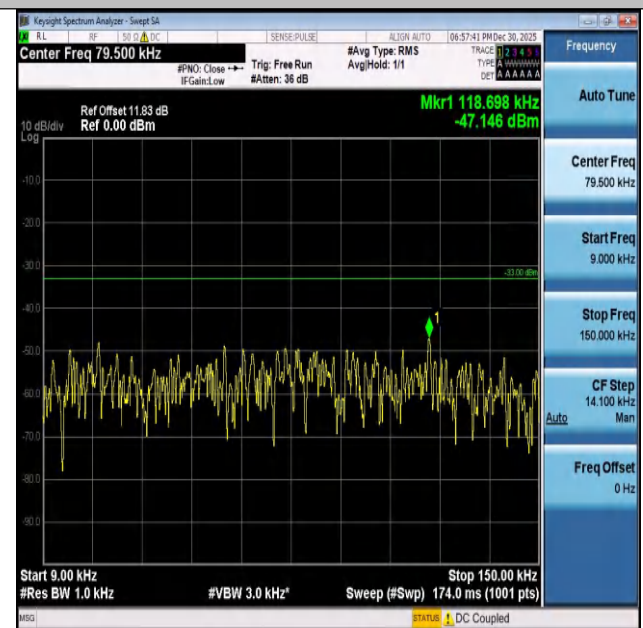
Band26(824-849)-1.4MHz-16QAM-26915-6RB#0-0.009~0. 15-PASS
