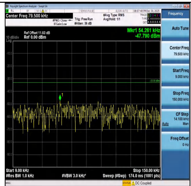
Band26(824-849)-3MHz-16QAM-26915-15RB#0-0.009~0.15-PASS
