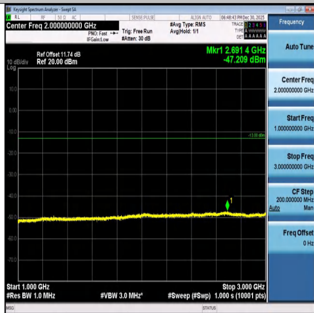
Band26(824-849)-1.4MHz-16QAM-26797-1RB#0-1000~30 00-PASS
