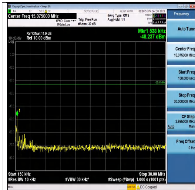
Band26(824-849)-3MHz-QPSK-27025-1RB#14-0.15~30-P
