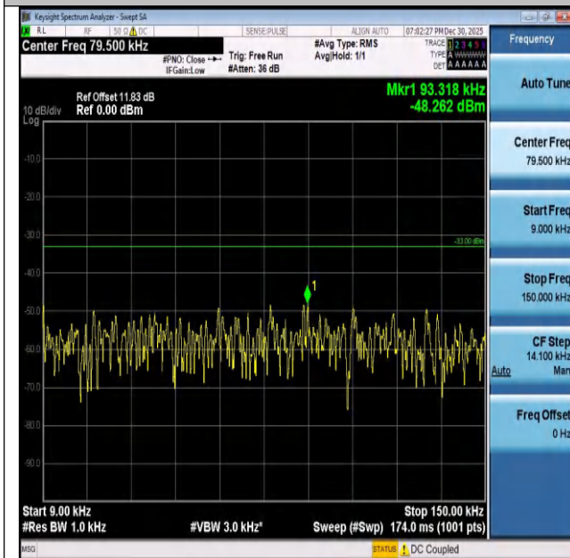
Band26(824-849)-1.4MHz-QPSK-27033-6RB#0-0.009~0.1 5-PASS
