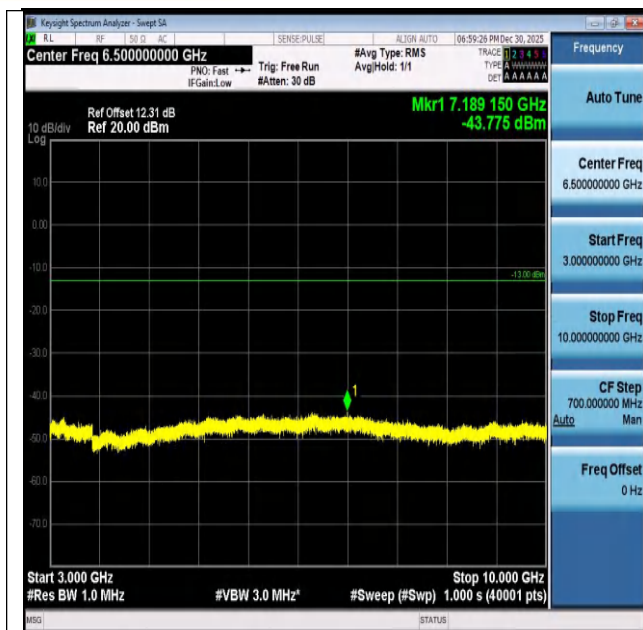
Band26(824-849)-1.4MHz-QPSK-27033-1RB#0-3000~100 00-PASS
