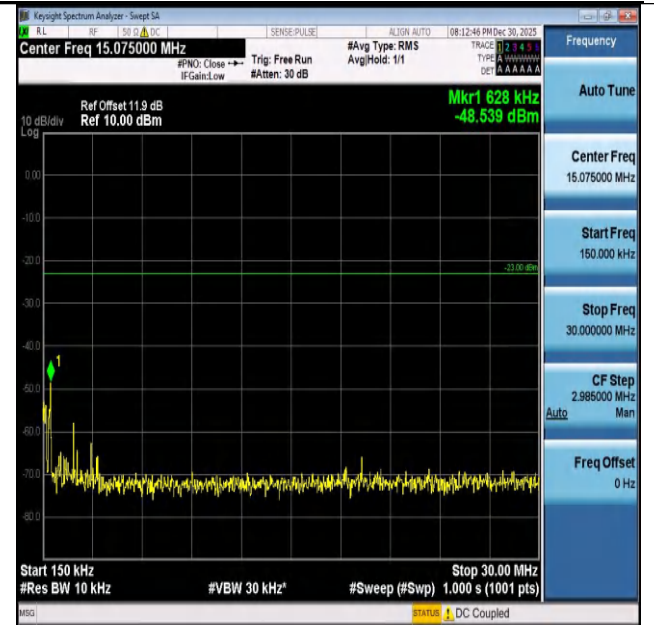
Band26(824-849)-3MHz-QPSK-27025-15RB#0-0.15~30-P ASS
