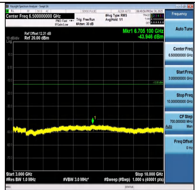
Band26(824-849)-1.4MHz-QPSK-26797-1RB#5-3000~100 00-PASS
