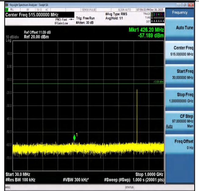
Band26(824-849)-3MHz-QPSK-26805-1RB#14-30~1000-P
