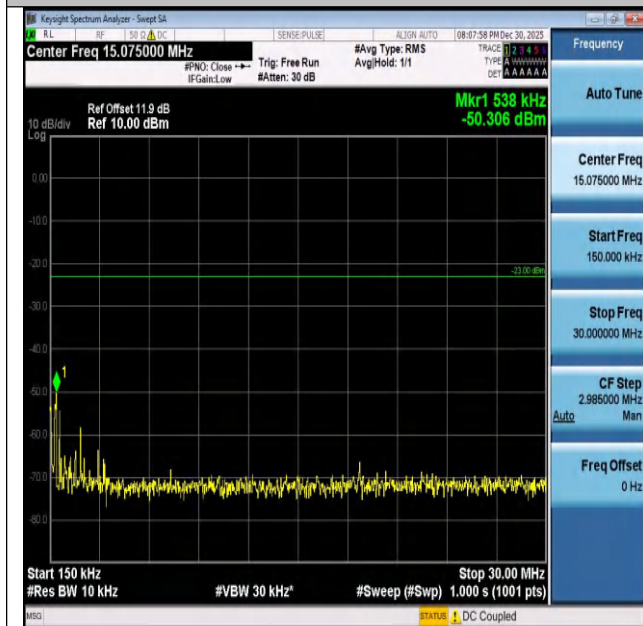
Band26(824-849)-3MHz-16QAM-26915-15RB#0-0.15~30-PASS
