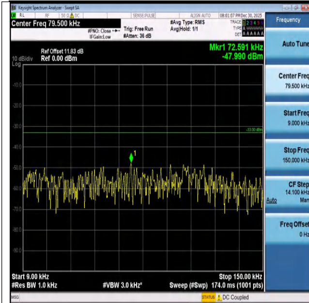
Band26(824-849)-3MHz-QPSK-26805-15RB#0-0.009~0.1 5-PASS
