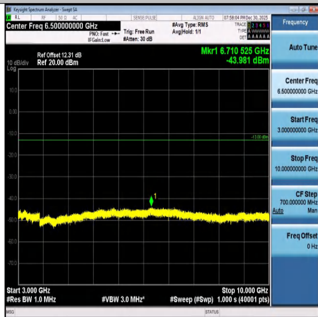
Band26(824-849)-3MHz-QPSK-26805-1RB#0-3000~1000 0-PASS
