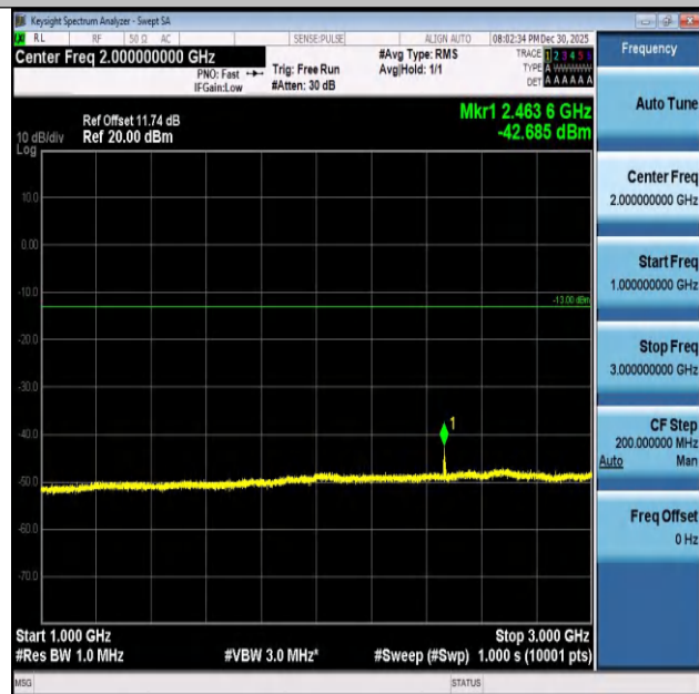
Band26(824-849)-3MHz-16QAM-26805-15RB#0-1000~3000- 00-PASS
