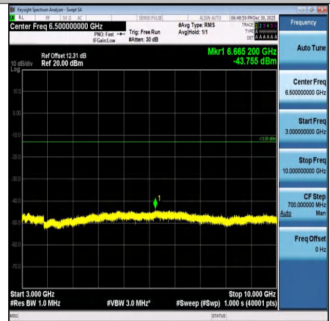
Band26(824-849)-1.4MHz-16QAM-26797-1RB#0-3000~10 000-PASS
