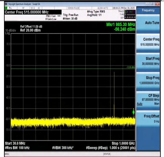
Band26(824-849)-3MHz-16QAM-26915-1RB#0-30~1000-P ASS
