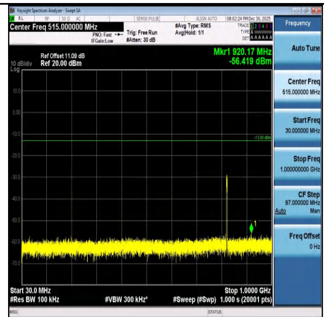
Band26(824-849)-3MHz-16QAM-26805-15RB#0-30~1000- PASS
