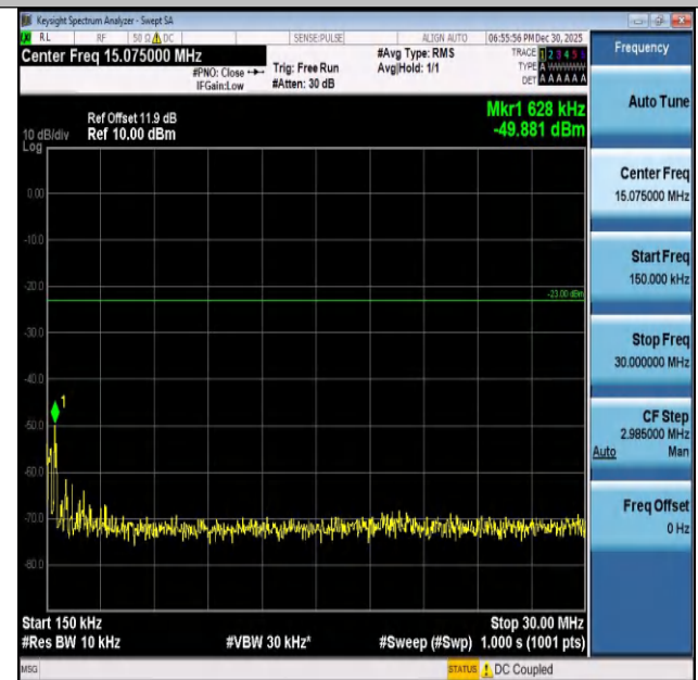
Band26(824-849)-1.4MHz-16QAM-26915-1RB#5-0.15~30- PASS
