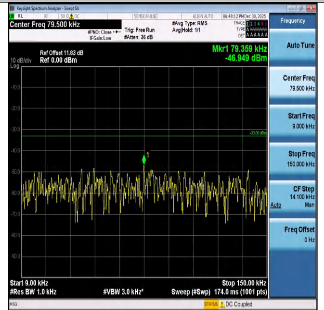
Band26(824-849)-1.4MHz-16QAM-26797-1RB#0-0.009~0- 15-PASS
