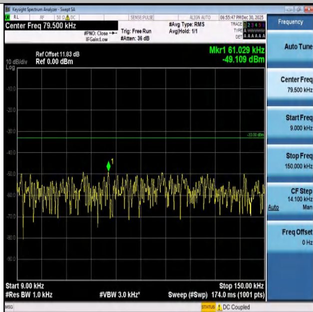
Band26(824-849)-1.4MHz-16QAM-26915-1RB#5-0.009~0. 15-PASS
