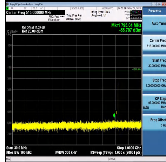
Band26(824-849)-1.4MHz-QPSK-26797-6RB#0-30~1000- PASS
