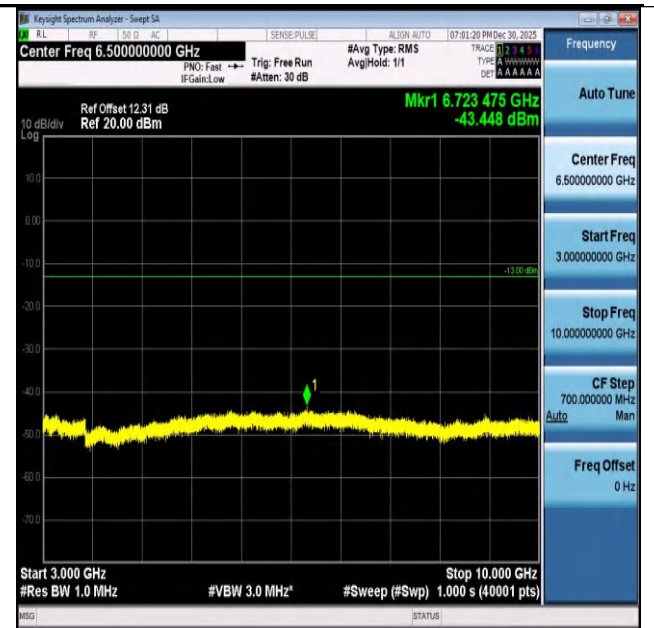
Band26(824-849)-1.4MHz-QPSK-27033-1RB#5-3000~100 00-PASS
