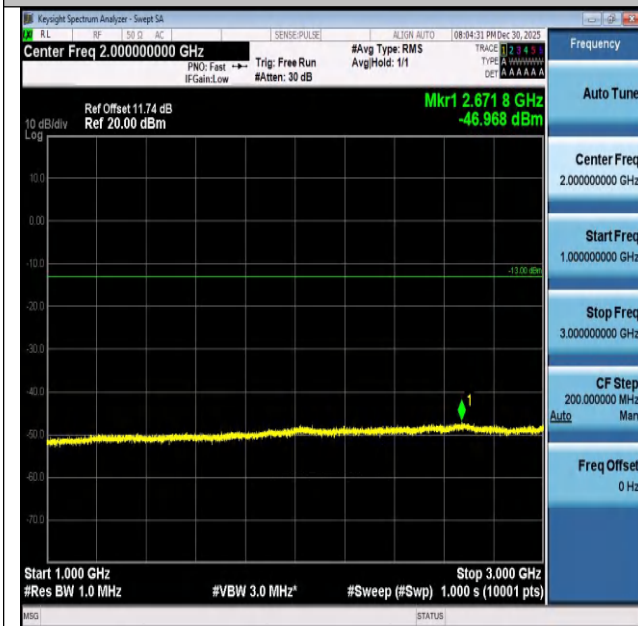
Band26(824-849)-3MHz-16QAM-26915-1RB#0-1000~300 0-PASS
