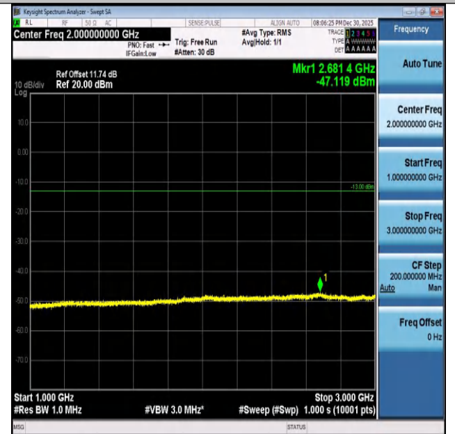
Band26(824-849)-3MHz-16QAM-26915-1RB#14-1000~30 00-PASS
