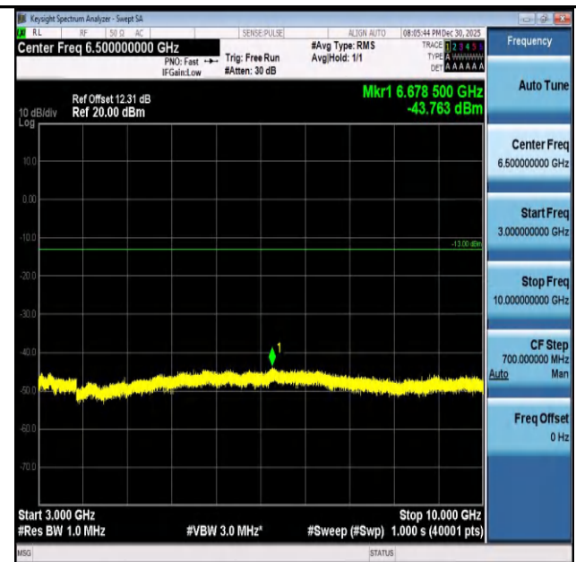
Band26(824-849)-3MHz-QPSK-26915-1RB#14-3000~100 00-PASS
