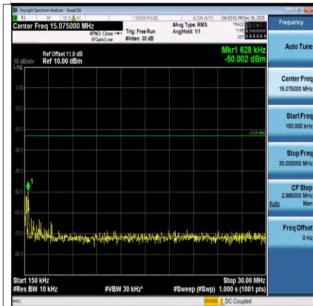
Band26(824-849)-1.4MHz-QPSK-26915-1RB#5-0.15~30-P ASS
