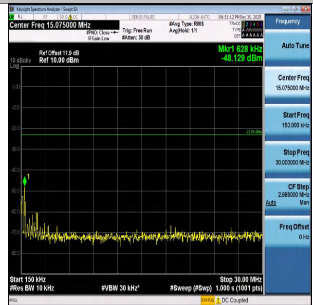
Band26(824-849)-1.4MHz-QPSK-26797-6RB#0-0.15~30-P ASS
