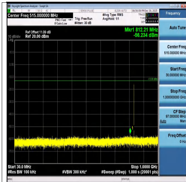
Band26(824-849)-1.4MHz-16QAM-26915-1RB#5-30~1000 -PASS
