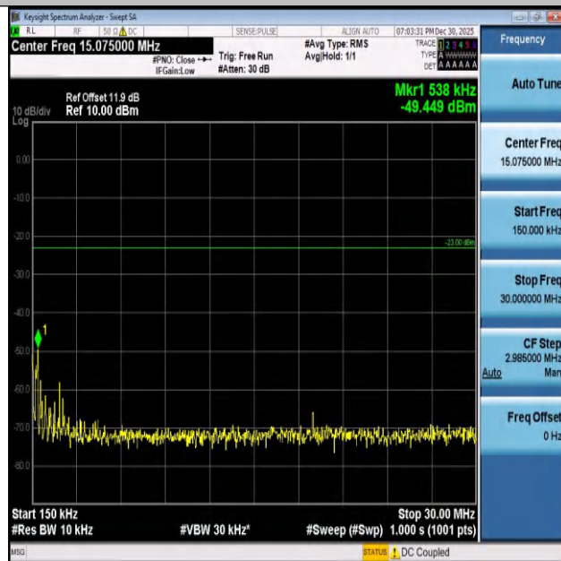
Band26(824-849)-1.4MHz-16QAM-27033-6RB#0-0.15~30- PASS
