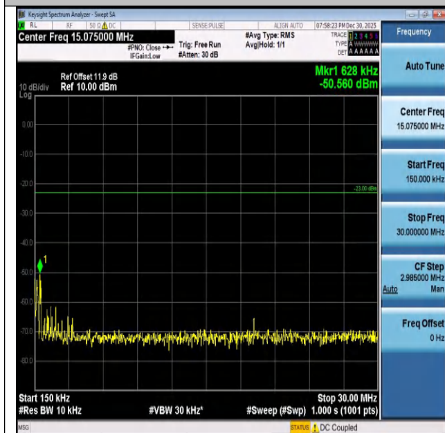
Band26(824-849)-3MHz-16QAM-26805-1RB#0-0.15~30-P ASS
