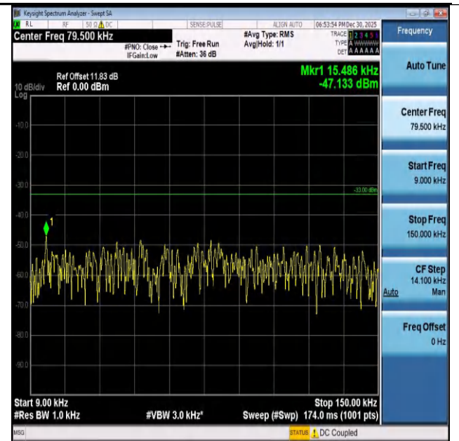
Band26(824-849)-1.4MHz-16QAM-26915-1RB#0-0.009~0. 15-PASS
