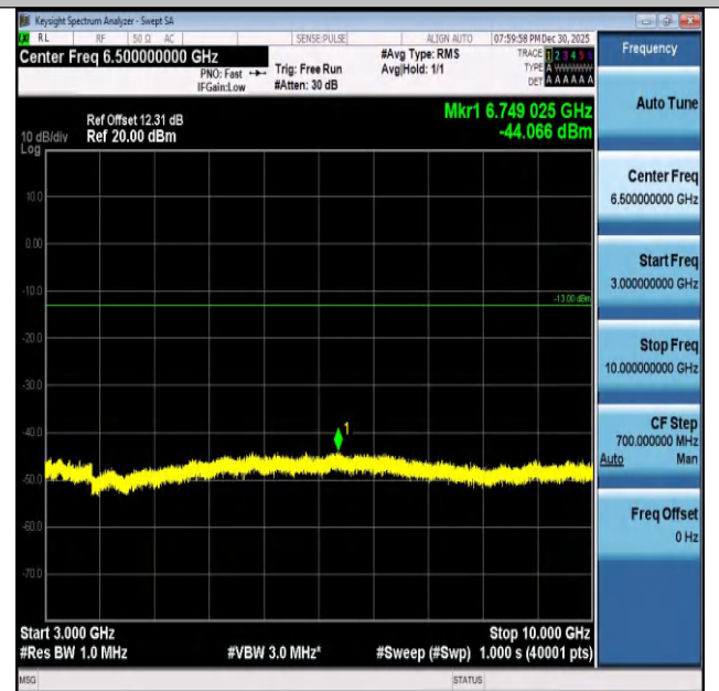
Band26(824-849)-3MHz-QPSK-26805-1RB#14-3000~100
