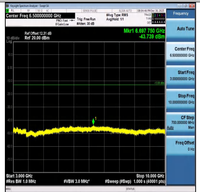
Band26(824-849)-3MHz-16QAM-26915-1RB#0-3000~100 00-PASS
