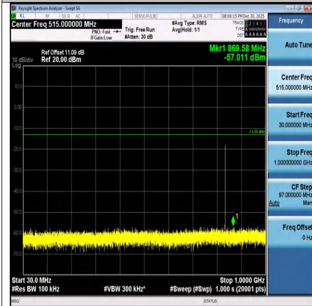
Band26(824-849)-3MHz-16QAM-26915-1RB#14-30~1000- PASS
