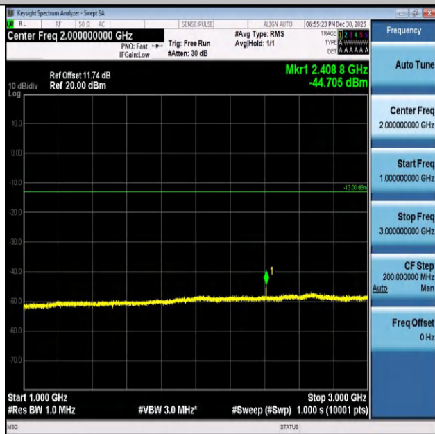
Band26(824-849)-1.4MHz-QPSK-26915-1RB#5-1000~300 0-PASS
