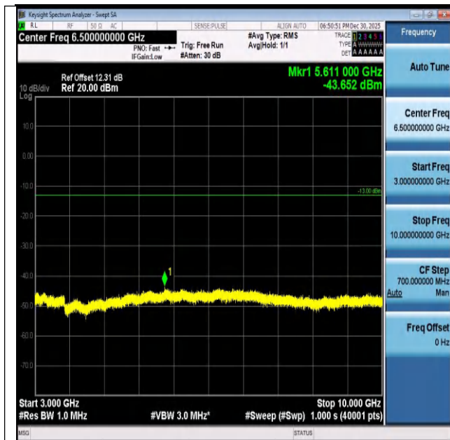
Band26(824-849)-1.4MHz-16QAM-26797-1RB#5-3000~10 000-PASS
