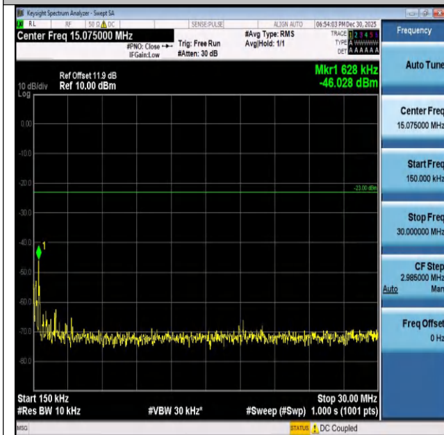
Band26(824-849)-1.4MHz-16QAM-26915-1RB#0-0.15~30- PASS
