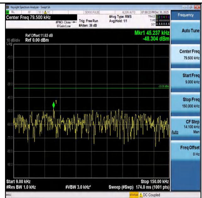
Band26(824-849)-1.4MHz-QPSK-27033-1RB#5-0.009~0.1 5-PASS
