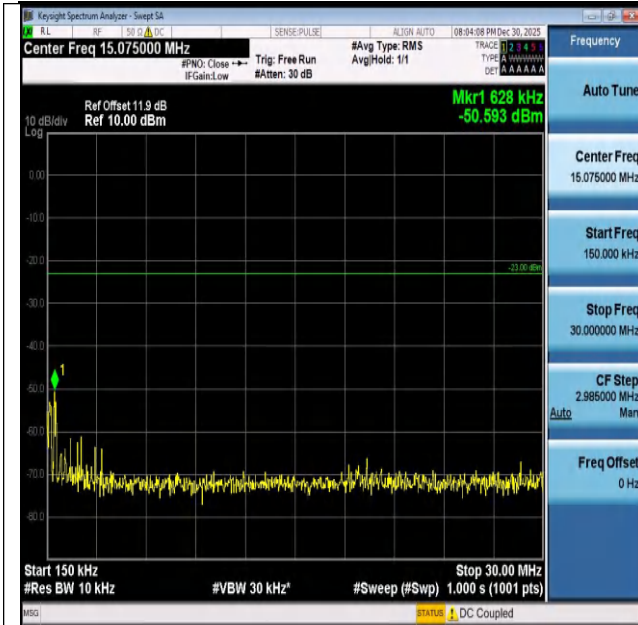
Band26(824-849)-3MHz-16QAM-26915-1RB#0-0.15~30-P ASS
