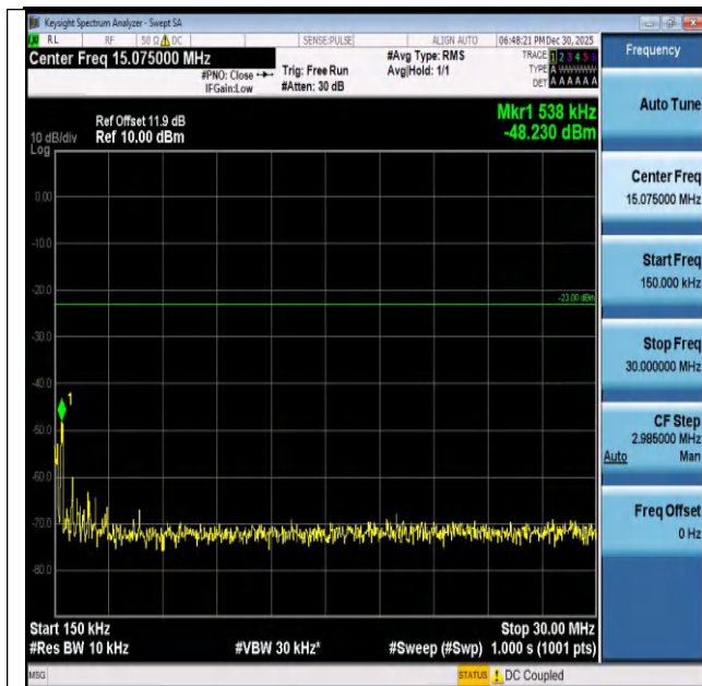
Band26(824-849)-1.4MHz-16QAM-26797-1RB#0-0.15~30- PASS
