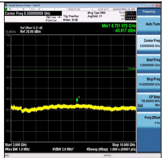
Band26(824-849)-1.4MHz-16QAM-26915-1RB#0-3000~10 000-PASS
