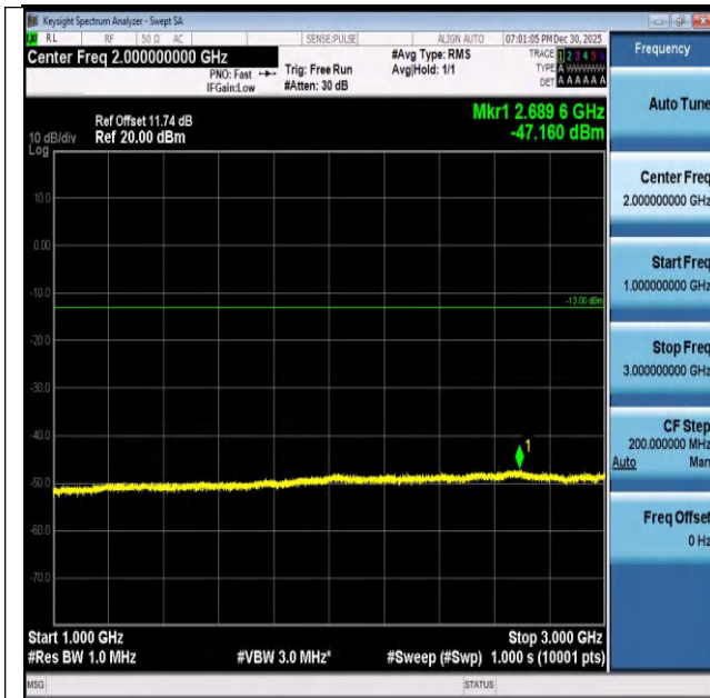
Band26(824-849)-1.4MHz-QPSK-27033-1RB#5-1000~300 0-PASS
