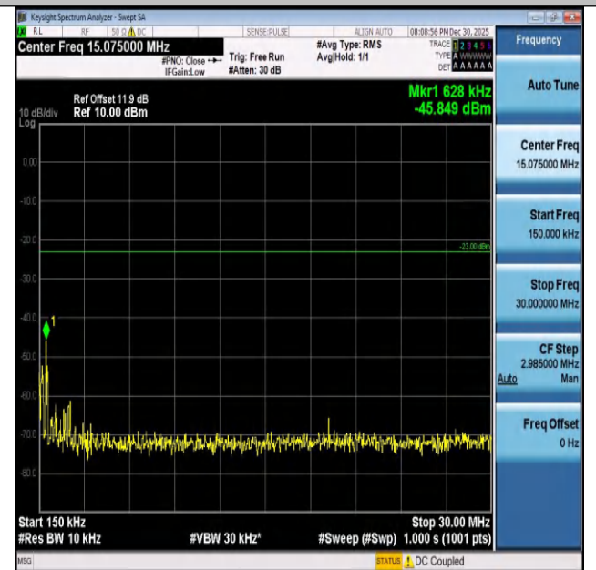
Band26(824-849)-3MHz-QPSK-27025-1RB#0-0.15~30-PA SS
