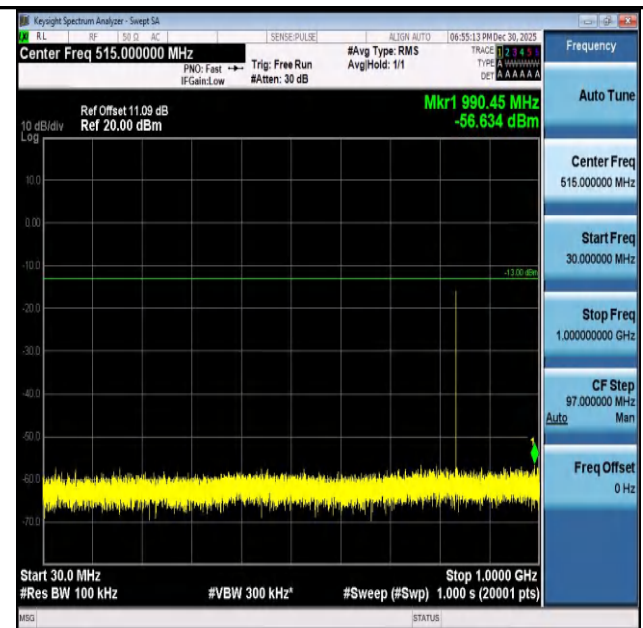
Band26(824-849)-1.4MHz-QPSK-26915-1RB#5-30~1000- PASS
