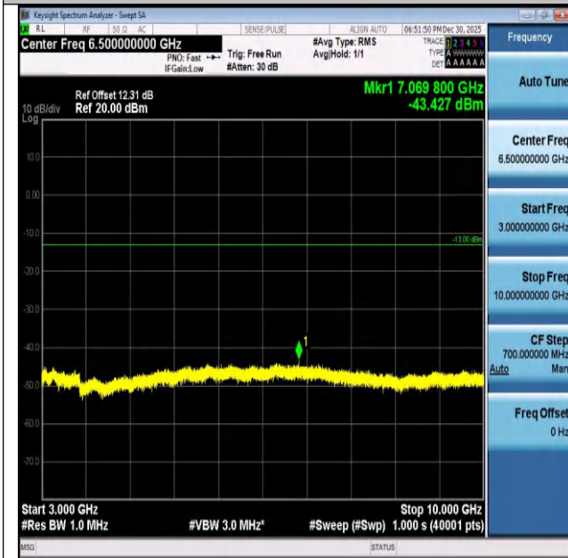
Band26(824-849)-1.4MHz-QPSK-26797-6RB#0-3000~100- 00-PASS
