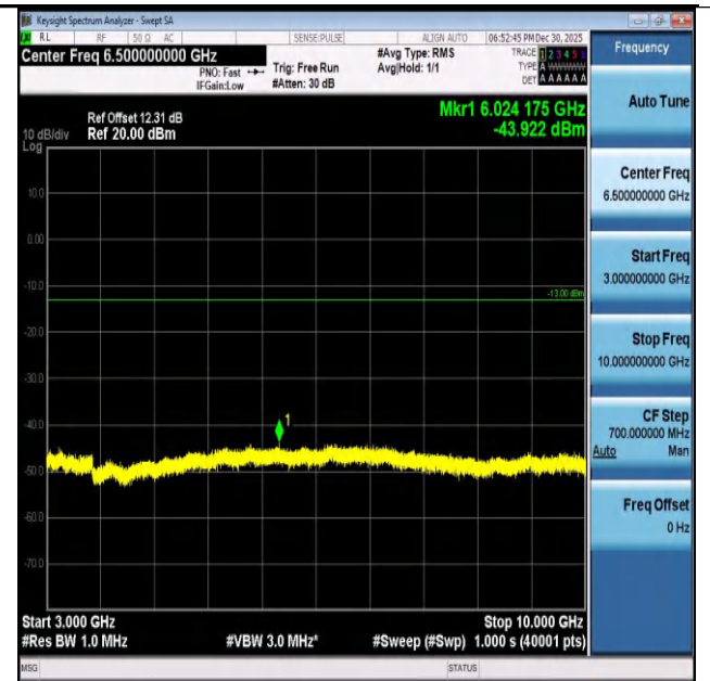
Band26(824-849)-1.4MHz-16QAM-26797-6RB#0-3000~10 000-PASS
