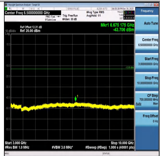
Band26(824-849)-1.4MHz-QPSK-26915-1RB#5-3000~100 00-PASS
