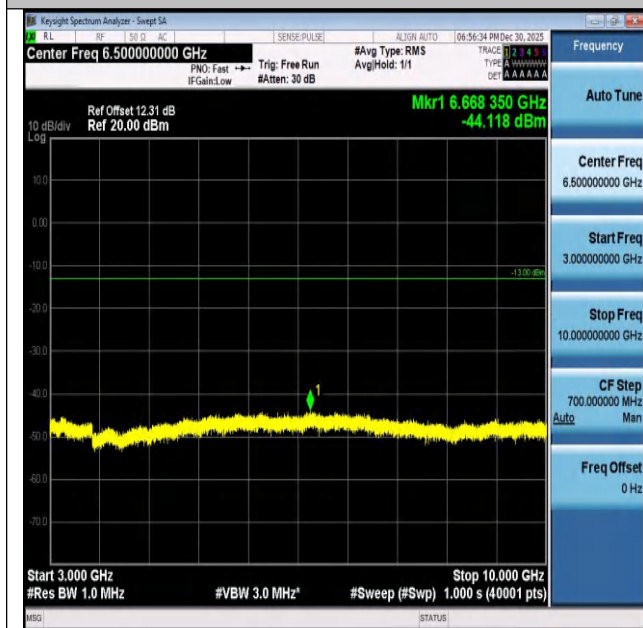
Band26(824-849)-1.4MHz-16QAM-26915-1RB#5-3000~10 000-PASS
