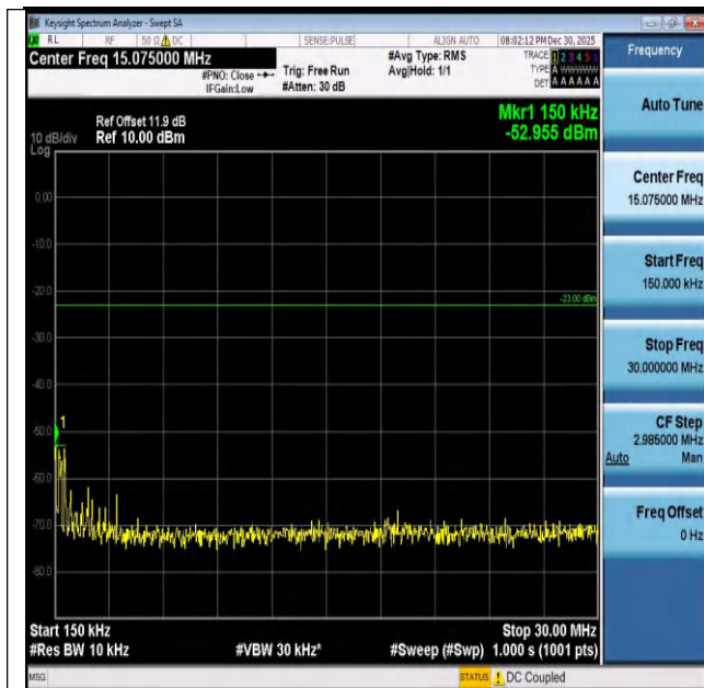
Band26(824-849)-3MHz-16QAM-26805-15RB#0-0.15~30- PASS
