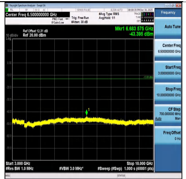
Band26(824-849)-3MHz-16QAM-26915-15RB#0-3000~10 000-PASS
