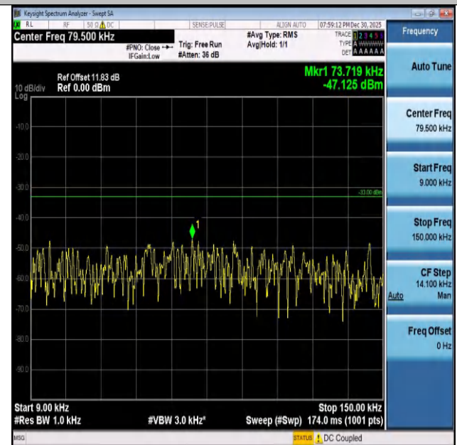
Band26(824-849)-3MHz-QPSK-26805-1RB#14-0.009~0.1 5-PASS
