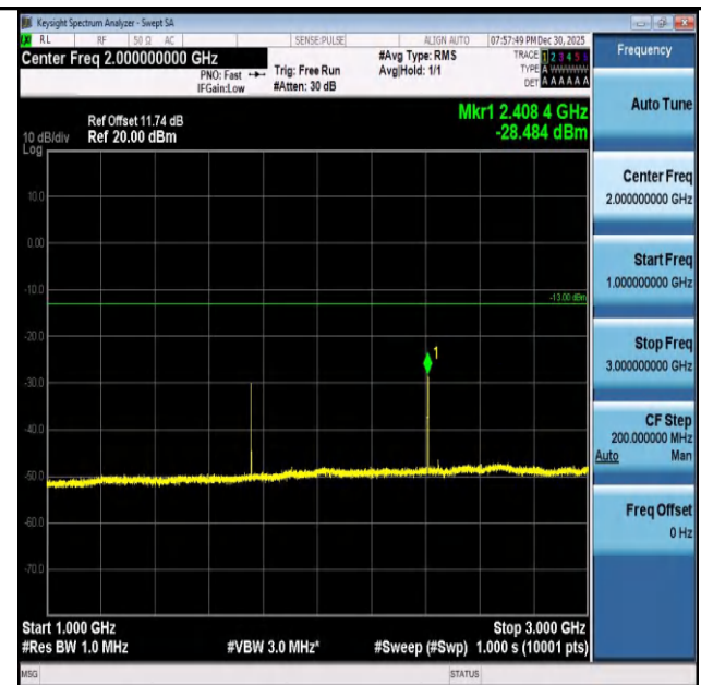
Band26(824-849)-3MHz-QPSK-26805-1RB#0-1000~3000- PASS
