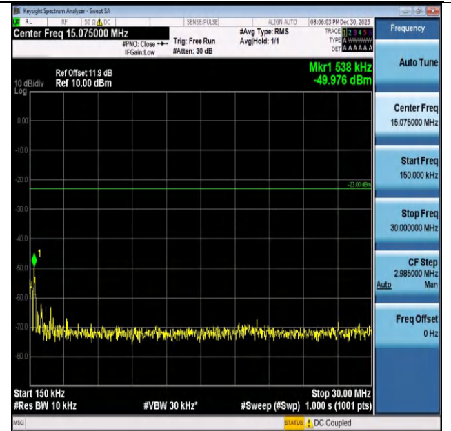
Band26(824-849)-3MHz-16QAM-26915-1RB#14-0.15~30- PASS
