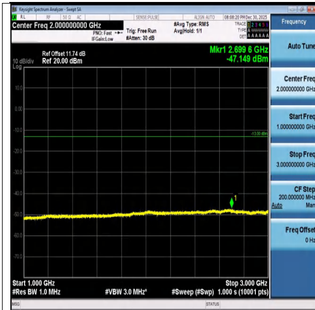
Band26(824-849)-3MHz-16QAM-26915-15RB#0-1000~30 00-PASS
