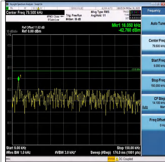
Band26(824-849)-3MHz-16QAM-26915-1RB#14-0.009~0. 15-PASS
