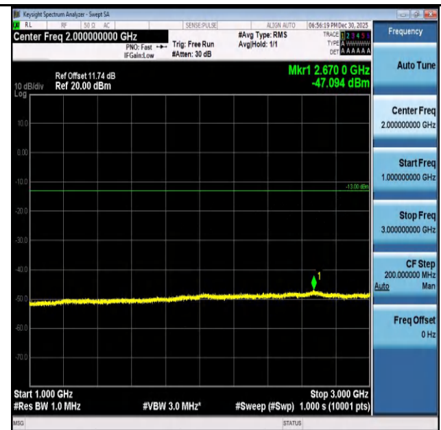
Band26(824-849)-1.4MHz-16QAM-26915-1RB#5-1000~30 00-PASS
