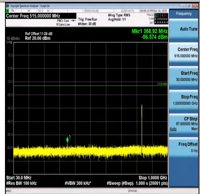
Band26(824-849)-3MHz-16QAM-26915-15RB#0-30~1000-PASS
