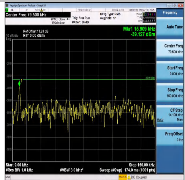
Band26(824-849)-3MHz-16QAM-26915-1RB#0-0.009~0.1 5-PASS
