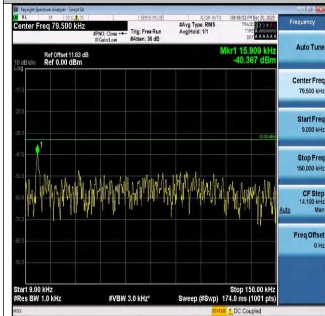
Band26(824-849)-3MHz-QPSK-26915-15RB#0-0.009~0.1 5-PASS
