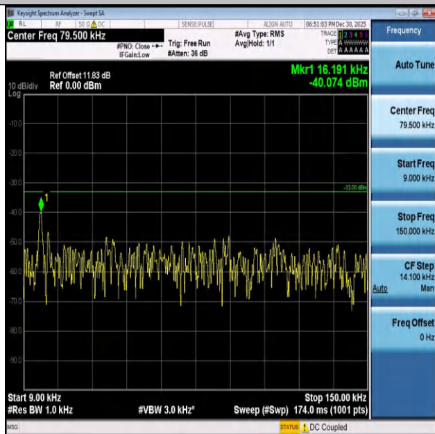
Band26(824-849)-1.4MHz-QPSK-26797-6RB#0-0.009~0.1 5-PASS
