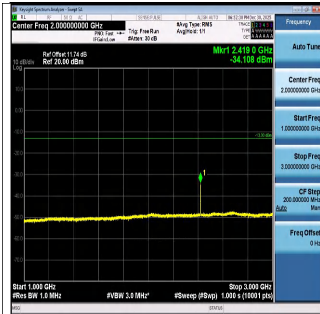
Band26(824-849)-1.4MHz-16QAM-26797-6RB#0-1000~30 00-PASS
