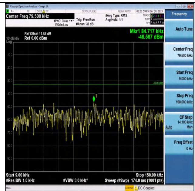
Band26(824-849)-1.4MHz-16QAM-26797-6RB#0-0.009~0. 15-PASS
