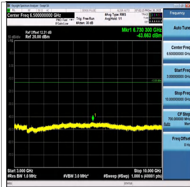
Band26(824-849)-1.4MHz-16QAM-27033-1RB#5-3000~10 000-PASS
