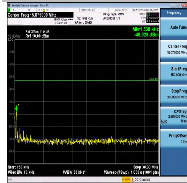
Band26(824-849)-1.4MHz-16QAM-26797-6RB#0-0.15~30- PASS
