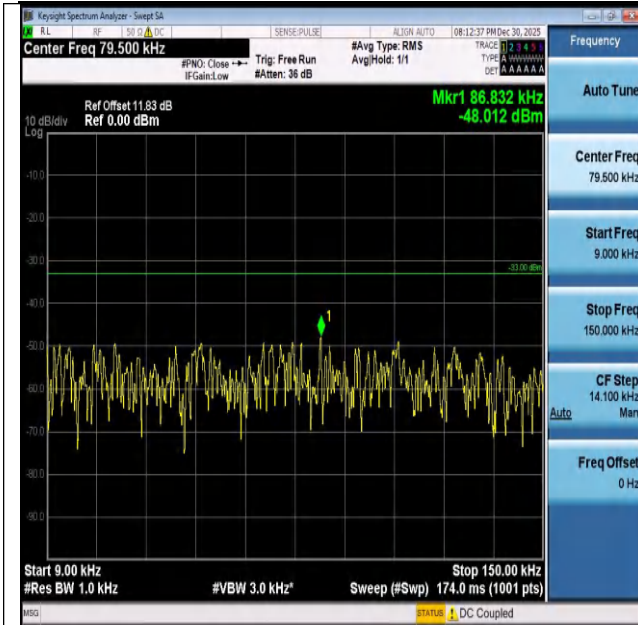
Band26(824-849)-3MHz-QPSK-27025-15RB#0-0.009~0.1 5-PASS
