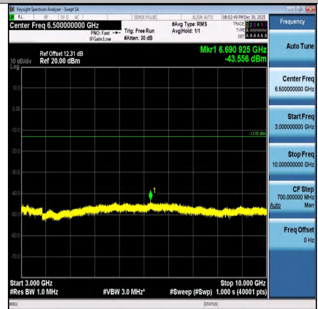
Band26(824-849)-3MHz-16QAM-26805-15RB#0-3000~10000- 000-PASS
