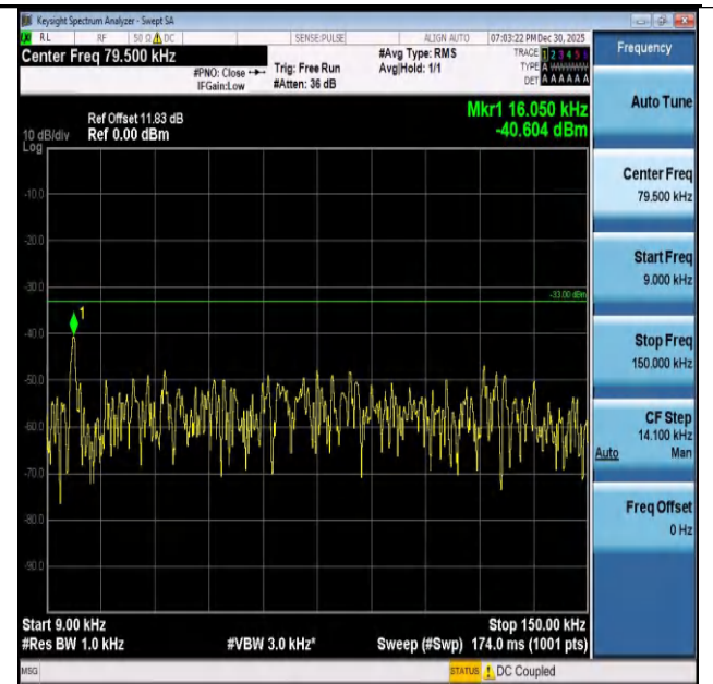
Band26(824-849)-1.4MHz-16QAM-27033-6RB#0-0.009~0. 15-PASS
