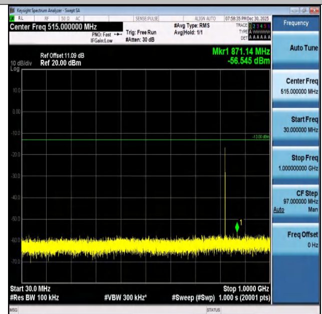
Band26(824-849)-3MHz-16QAM-26805-1RB#0-30~1000-P ASS
