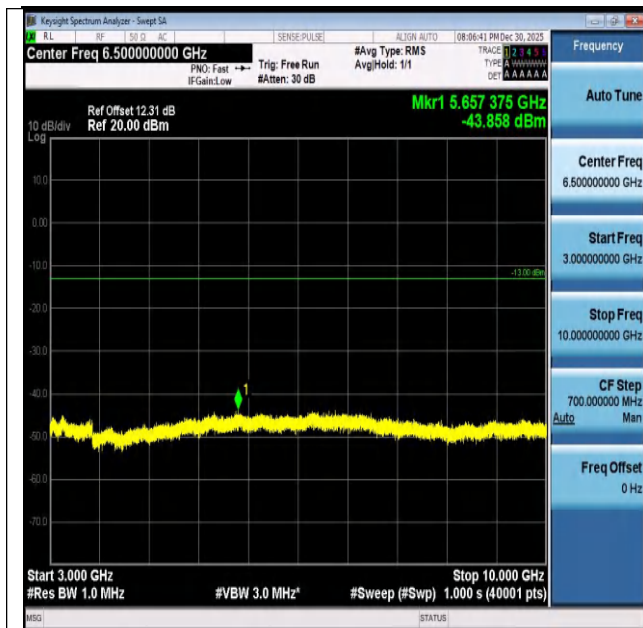
Band26(824-849)-3MHz-16QAM-26915-1RB#14-3000~10000-PASS
