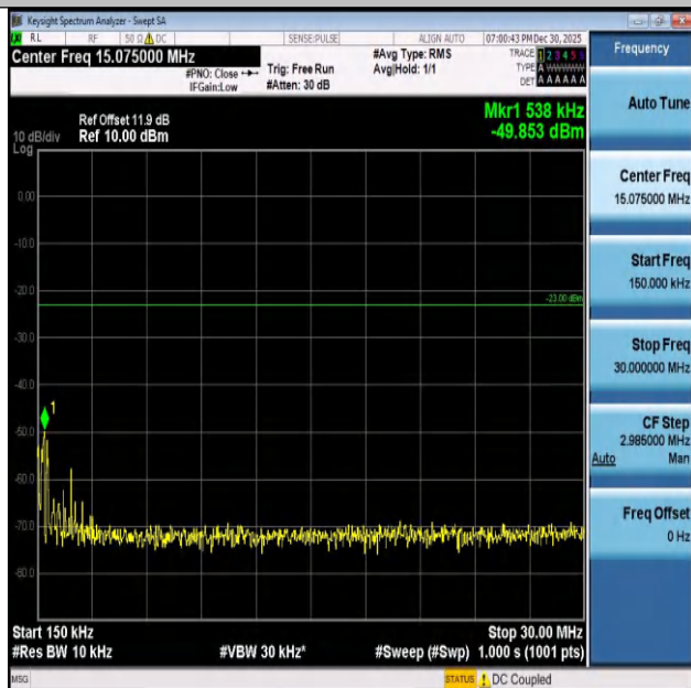
Band26(824-849)-1.4MHz-QPSK-27033-1RB#5-0.15~30-P ASS
