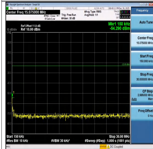
Band26(824-849)-5MHz-16QAM-26915-1RB#0-0.15~30-P ASS
