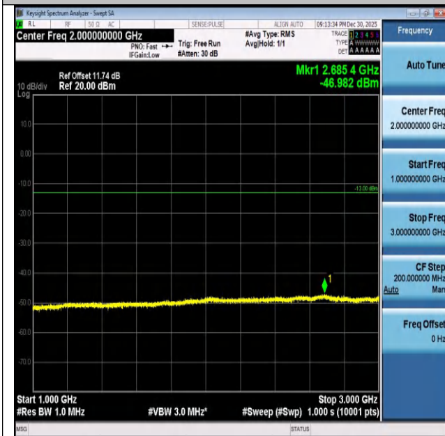
Band26(824-849)-10MHz-16QAM-26840-50RB#0-1000~3 000-PASS
