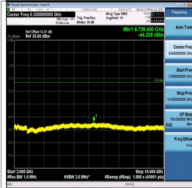
Band26(824-849)-5MHz-QPSK-26815-1RB#0-3000~1000 0-PASS
