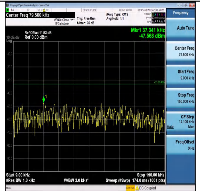
Band26(824-849)-5MHz-16QAM-27015-1RB#0-0.009~0.1 5-PASS
