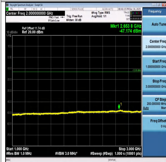
Band26(824-849)-5MHz-16QAM-27015-1RB#0-1000~300
