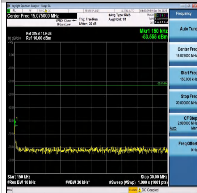
Band26(824-849)-5MHz-16QAM-27015-25RB#0-0.15~30-PASS
