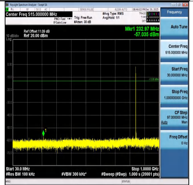
Band26(824-849)-5MHz-16QAM-27015-1RB#0-30~1000-P
