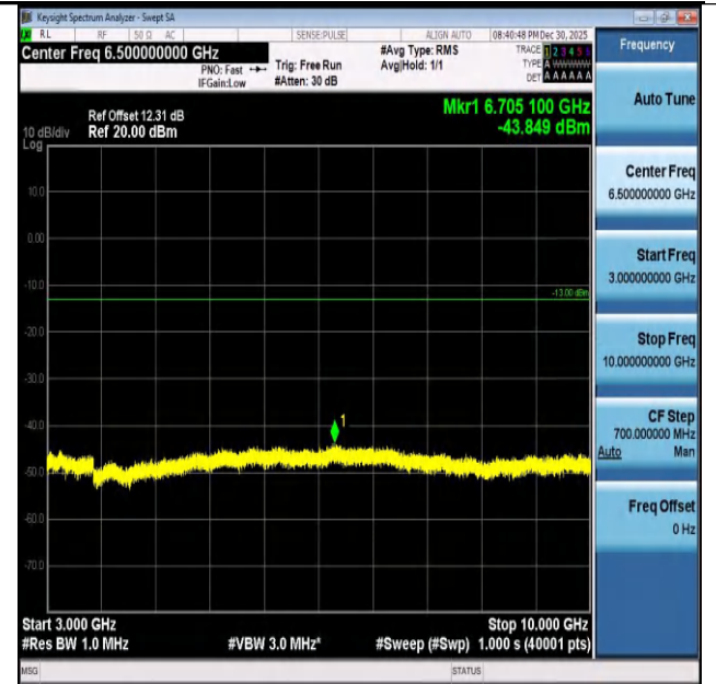
Band26(824-849)-5MHz-16QAM-26915-1RB#0-3000~100 00-PASS
