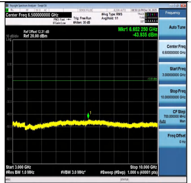
Band26(824-849)-5MHz-16QAM-27015-25RB#0-3000~10 000-PASS
