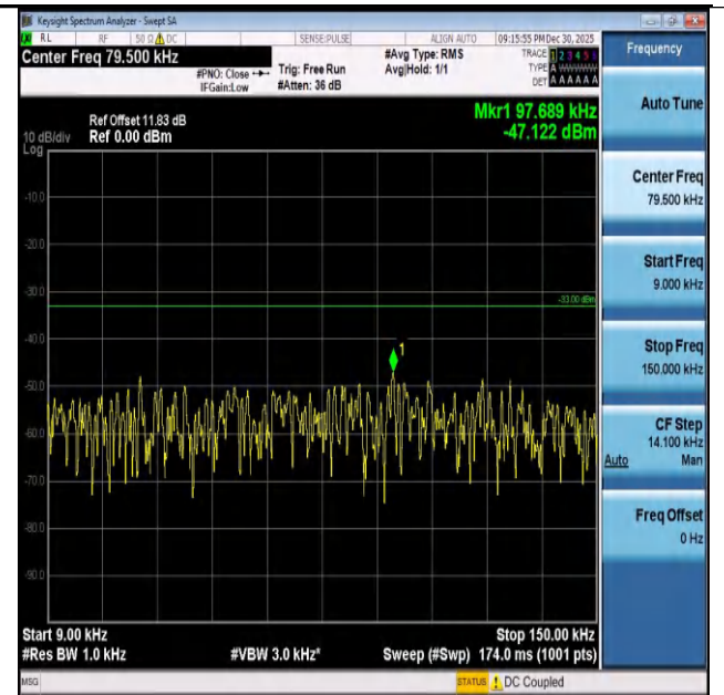
Band26(824-849)-10MHz-QPSK-26915-1RB#49-0.009~0.150-PASS
