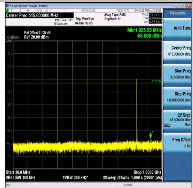
Band26(824-849)-5MHz-16QAM-26915-1RB#0-30~1000-P ASS
