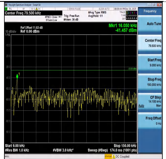
Band26(824-849)-3MHz-16QAM-27025-1RB#0-0.009~0.1 5-PASS
