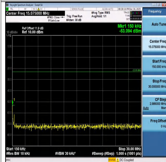
Band26(824-849)-5MHz-16QAM-26815-25RB#0-0.15~30- PASS
