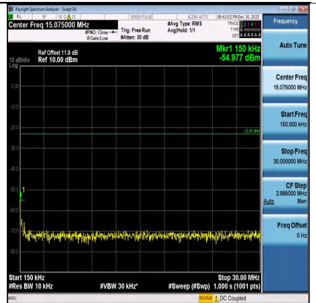
Band26(824-849)-5MHz-QPSK-26915-25RB#0-0.15~30-P
