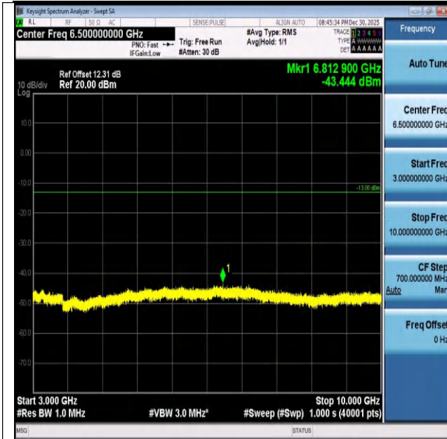
Band26(824-849)-5MHz-QPSK-27015-1RB#0-3000~1000 0-PASS
