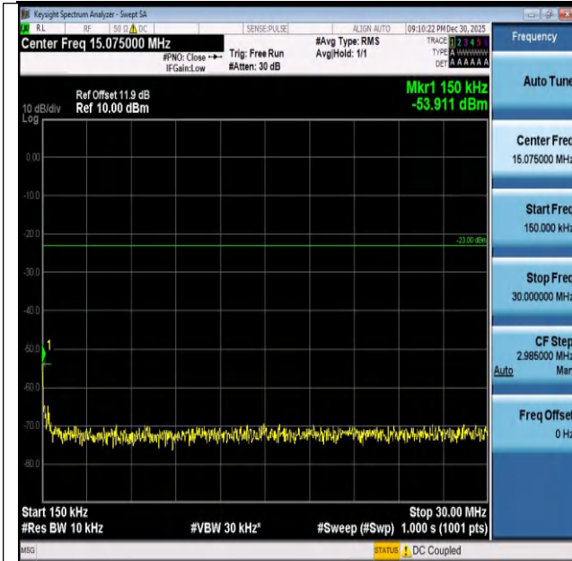
Band26(824-849)-10MHz-QPSK-26840-1RB#49-0.15~30- PASS
