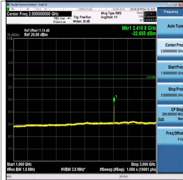
Band26(824-849)-5MHz-16QAM-26815-25RB#0-1000~30 00-PASS
