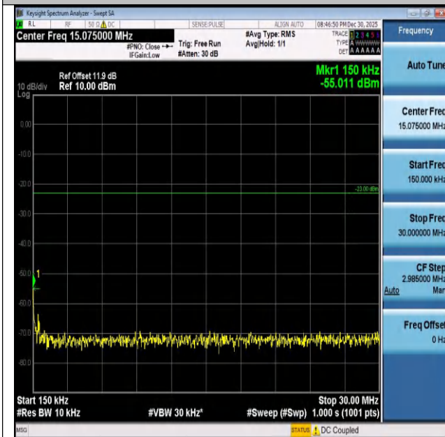
Band26(824-849)-5MHz-QPSK-27015-1RB#24-0.15~30-P ASS
