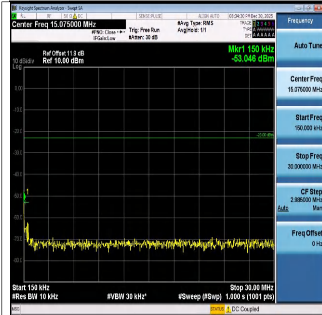
Band26(824-849)-5MHz-16QAM-26815-1RB#0-0.15~30-P ASS
