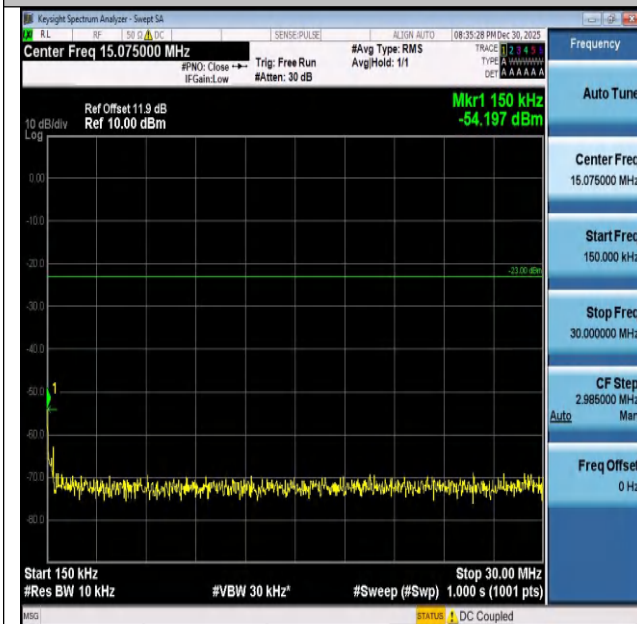
Band26(824-849)-5MHz-QPSK-26815-1RB#24-0.15~30-P ASS
