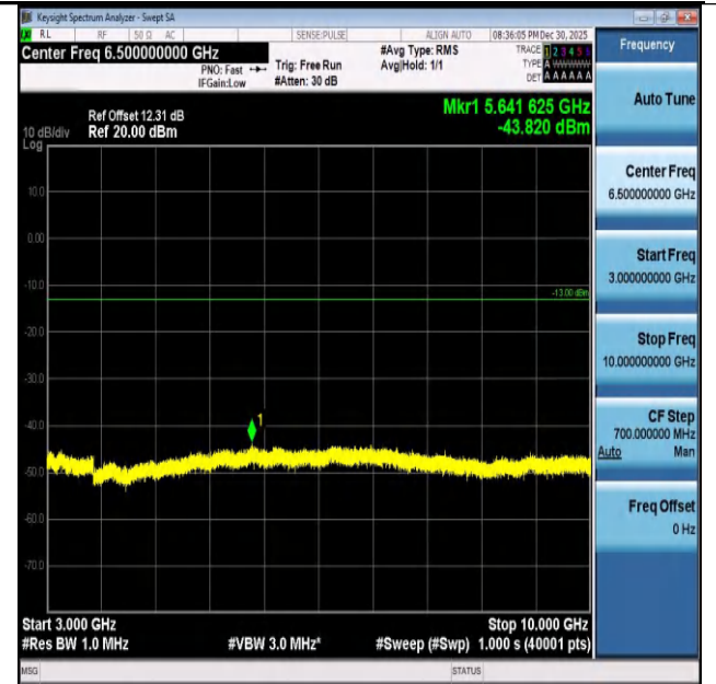
Band26(824-849)-5MHz-QPSK-26815-1RB#24-3000~100 00-PASS
