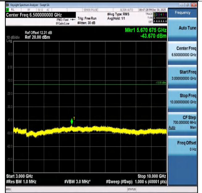
Band26(824-849)-5MHz-QPSK-27015-1RB#24-3000~100 00-PASS
