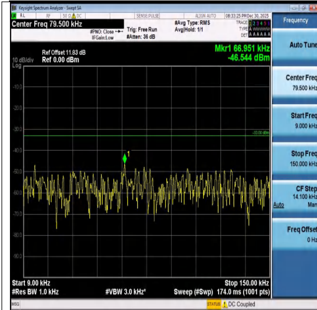
Band26(824-849)-5MHz-QPSK-26815-1RB#0-0.009~0.15-
