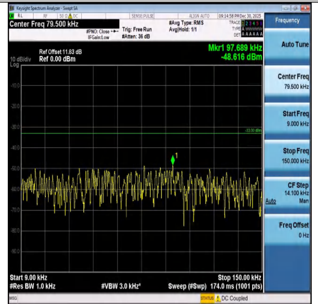
Band26(824-849)-10MHz-16QAM-26915-1RB#0-0.009~0.15-PASS
