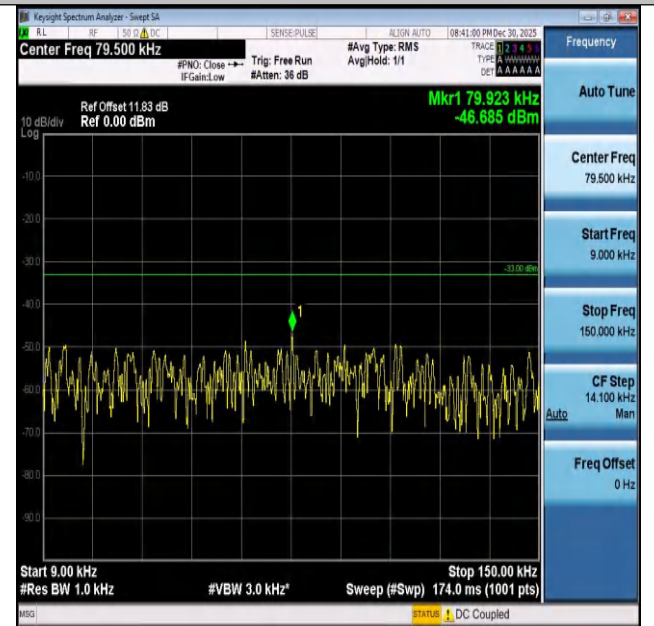
Band26(824-849)-5MHz-QPSK-26915-1RB#24-0.009~0.1 5-PASS
