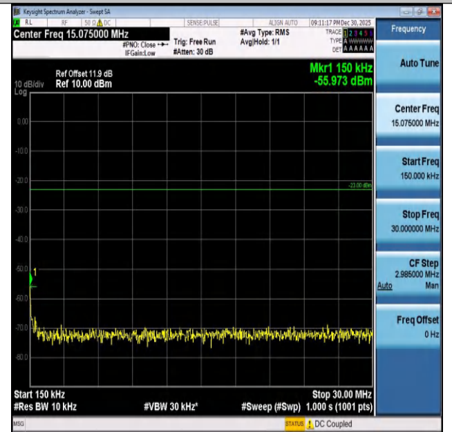
Band26(824-849)-10MHz-16QAM-26840-1RB#49-0.15~30 -PASS
