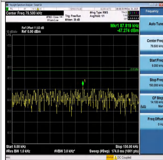
Band26(824-849)-5MHz-QPSK-27015-25RB#0-0.009~0.1 5-PASS
