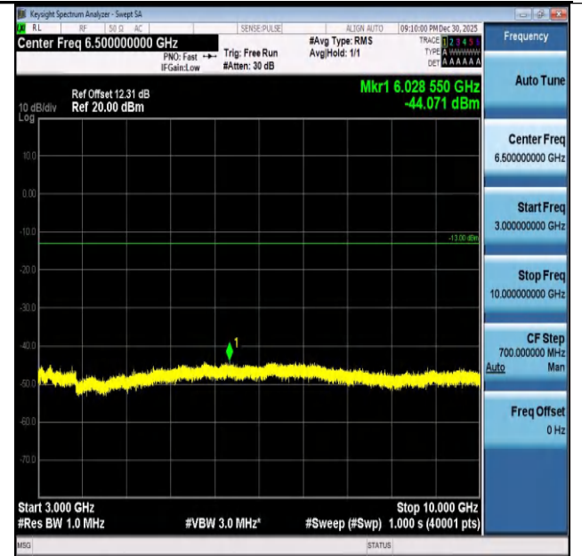
Band26(824-849)-10MHz-16QAM-26840-1RB#0-3000~10 000-PASS
