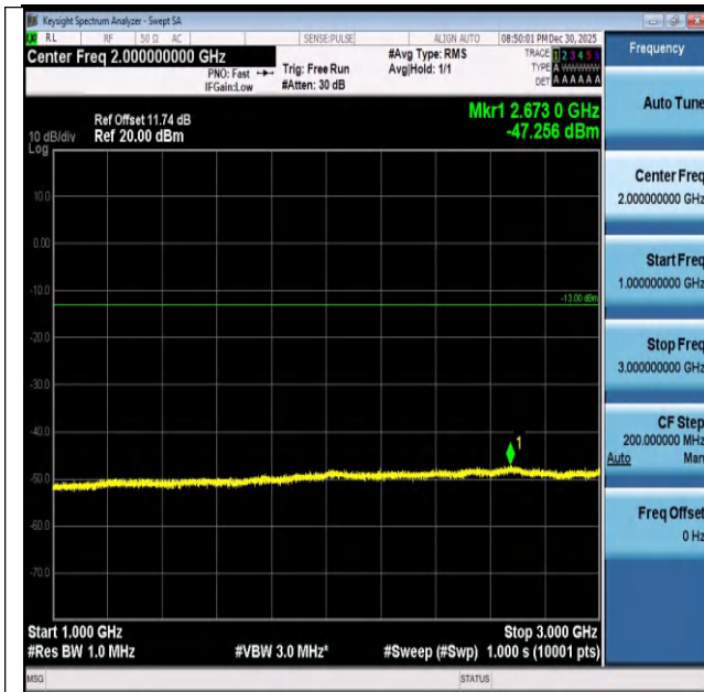
Band26(824-849)-5MHz-16QAM-27015-25RB#0-1000~30 00-PASS
