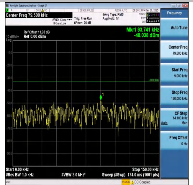
Band26(824-849)-10MHz-QPSK-26840-1RB#49-0.009~0. 15-PASS
