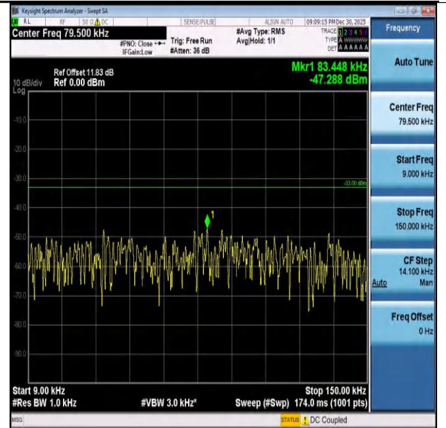
Band26(824-849)-10MHz-16QAM-26840-1RB#0-0.009~0.15-PASS
