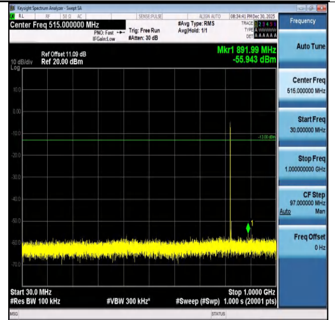
Band26(824-849)-5MHz-16QAM-26815-1RB#0-30~1000-P ASS
