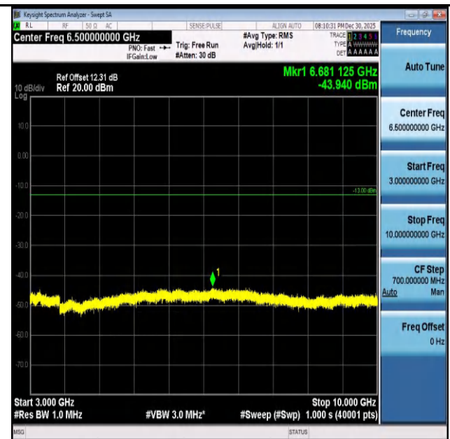
Band26(824-849)-3MHz-16QAM-27025-1RB#0-3000~100 00-PASS
