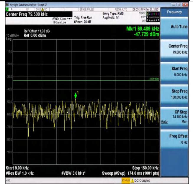
Band26(824-849)-5MHz-QPSK-26815-1RB#24-0.009~0.1 5-PASS
