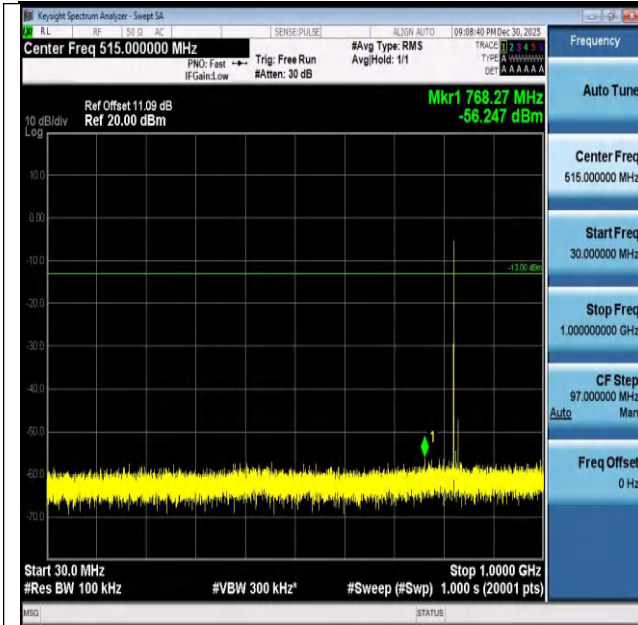
Band26(824-849)-10MHz-QPSK-26840-1RB#0-30~1000-P ASS
