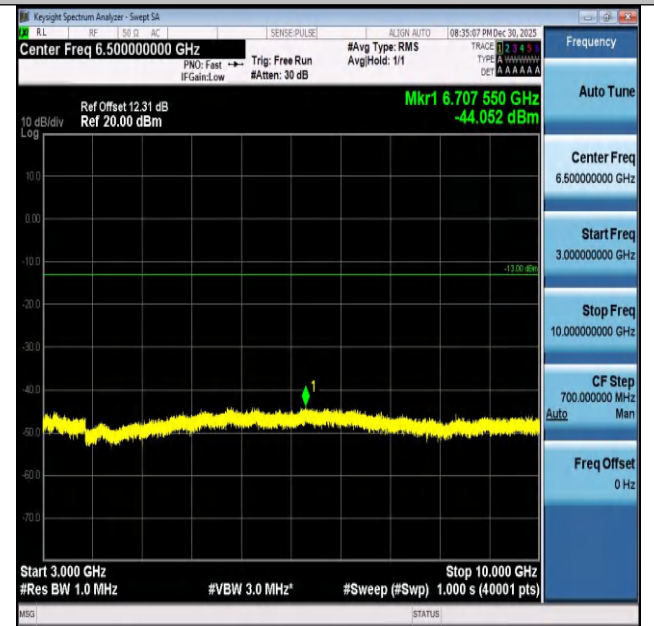
Band26(824-849)-5MHz-16QAM-26815-1RB#0-3000~100 00-PASS
