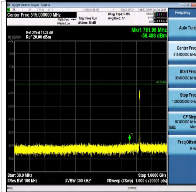
Band26(824-849)-5MHz-QPSK-26815-25RB#0-30~1000-P ASS
