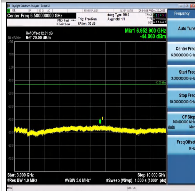
Band26(824-849)-10MHz-QPSK-26840-1RB#0-3000~100 00-PASS
