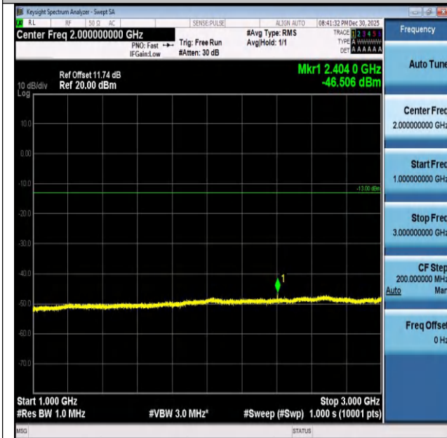
Band26(824-849)-5MHz-QPSK-26915-1RB#24-1000~300
