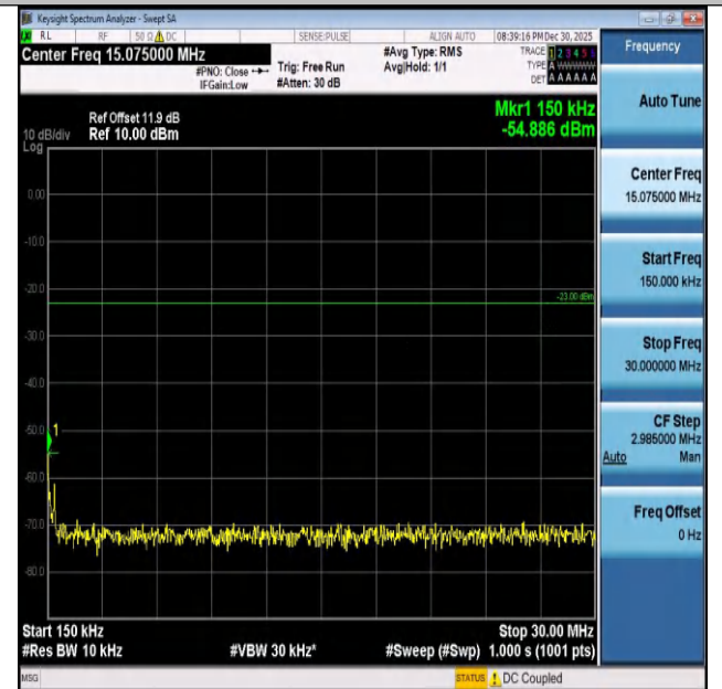
Band26(824-849)-5MHz-QPSK-26915-1RB#0-0.15~30-PA SS
