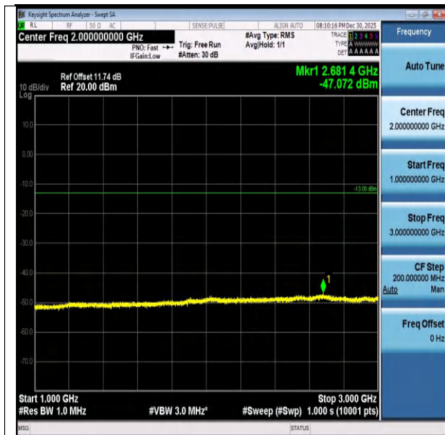
Band26(824-849)-3MHz-16QAM-27025-1RB#0-1000~300 0-PASS
