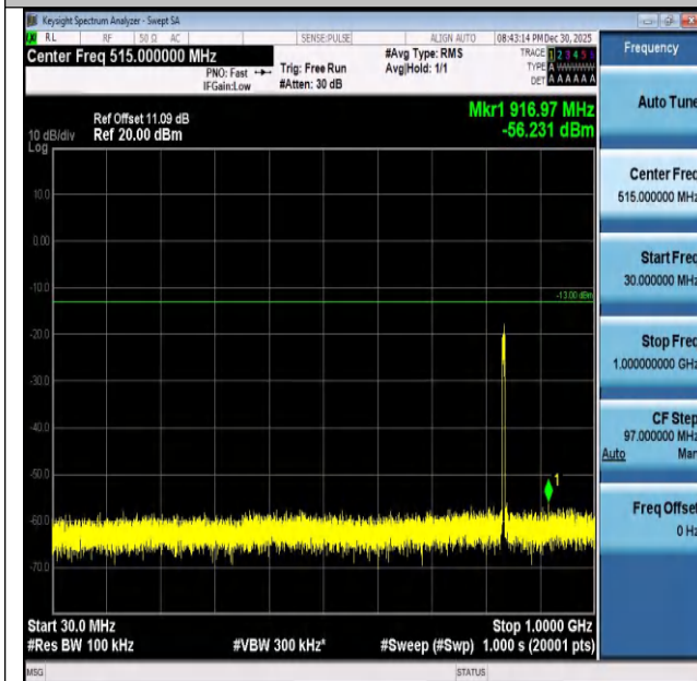
Band26(824-849)-5MHz-QPSK-26915-25RB#0-30~1000-P
