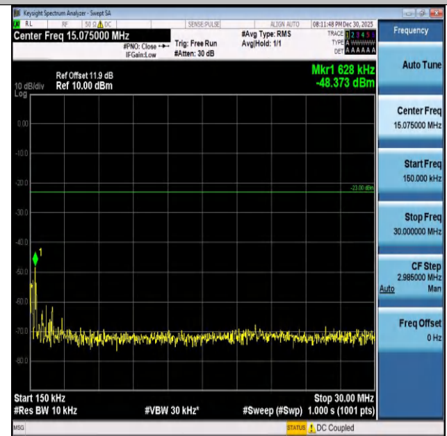
Band26(824-849)-3MHz-16QAM-27025-1RB#14-0.15~30- PASS
