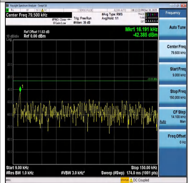
Band26(824-849)-3MHz-16QAM-27025-15RB#0-0.009~0.15-PASS
