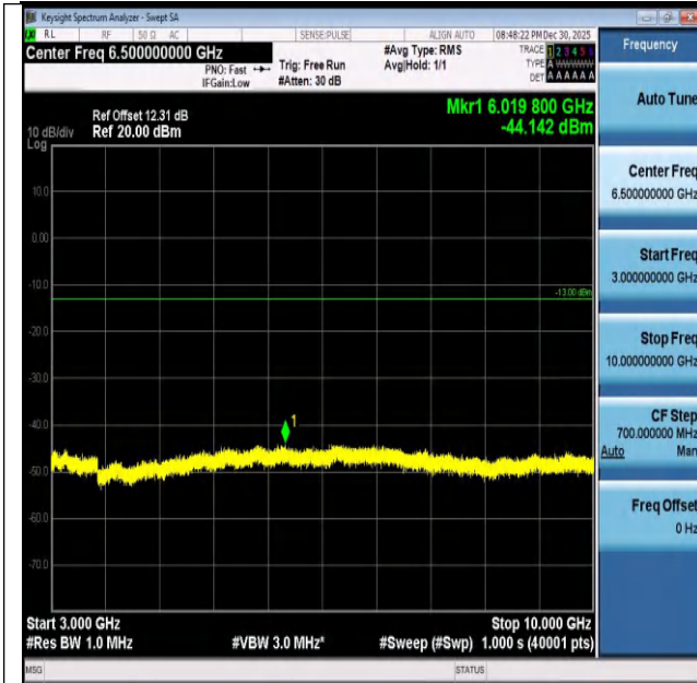
Band26(824-849)-5MHz-16QAM-27015-1RB#24-3000~10000-PASS
