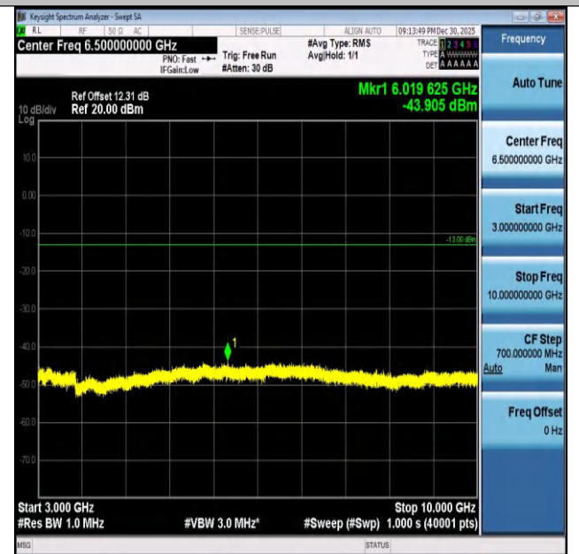
Band26(824-849)-10MHz-16QAM-26840-50RB#0-3000~1 0000-PASS
