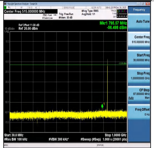
Band26(824-849)-5MHz-QPSK-26915-1RB#24-30~1000-P
