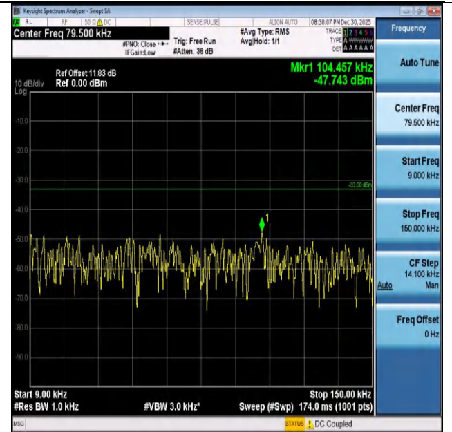
Band26(824-849)-5MHz-16QAM-26815-25RB#0-0.009~0. 15-PASS
