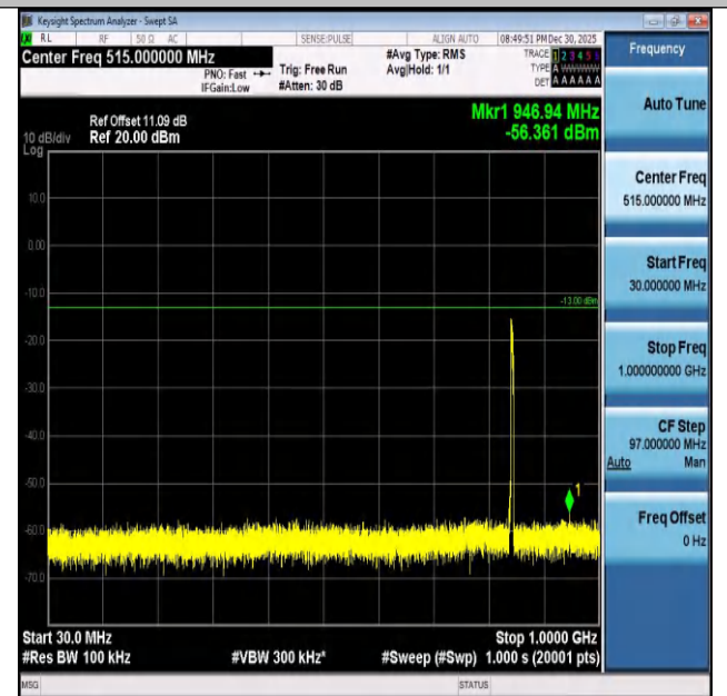
Band26(824-849)-5MHz-16QAM-27015-25RB#0-30~1000-PASS
