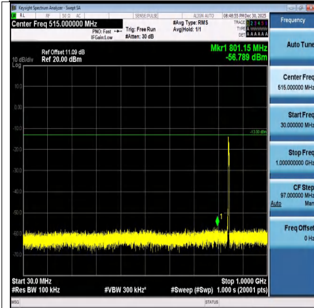
Band26(824-849)-5MHz-QPSK-27015-25RB#0-30~1000-P ASS
