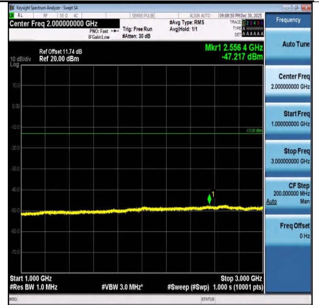
Band26(824-849)-10MHz-QPSK-26840-1RB#0-1000~300 0-PASS
