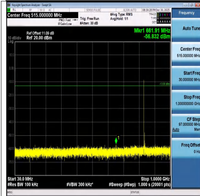
Band26(824-849)-5MHz-QPSK-26915-1RB#0-30~1000-PA SS
