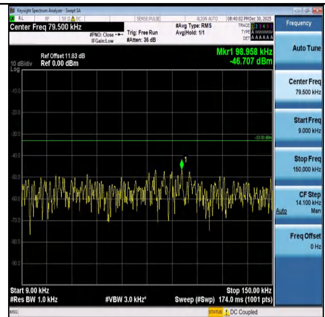
Band26(824-849)-5MHz-16QAM-26915-1RB#0-0.009~0.1 5-PASS
