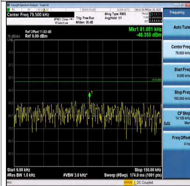
Band26(824-849)-5MHz-16QAM-26915-1RB#24-0.009~0. 15-PASS
