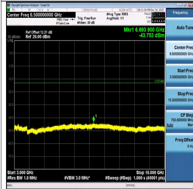
Band26(824-849)-10MHz-16QAM-26840-1RB#49-3000~1 0000-PASS
