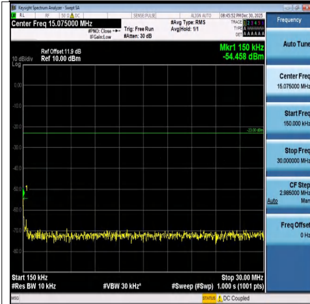
Band26(824-849)-5MHz-16QAM-27015-1RB#0-0.15~30-P
