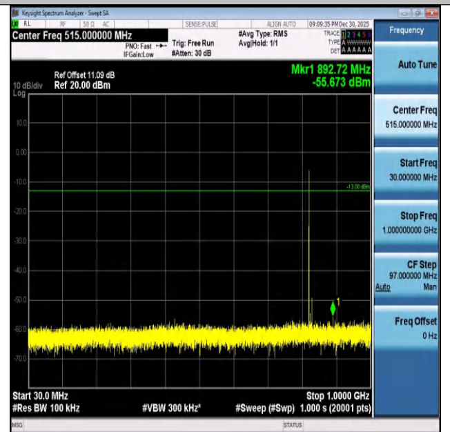
Band26(824-849)-10MHz-16QAM-26840-1RB#0-30~1000-PASS
