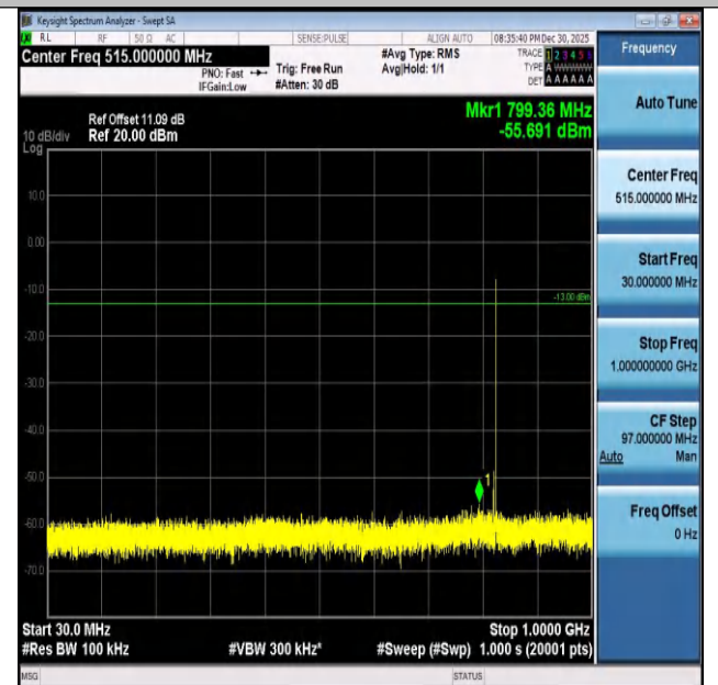
Band26(824-849)-5MHz-QPSK-26815-1RB#24-30~1000-P ASS
