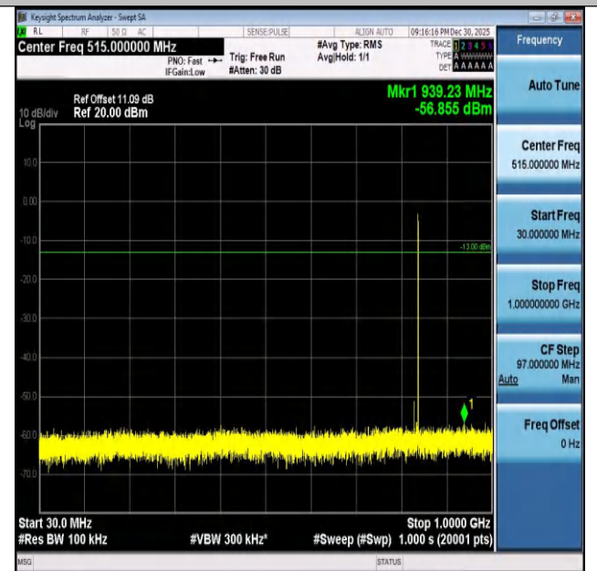
Band26(824-849)-10MHz-QPSK-26915-1RB#49-30~1000-PASS
