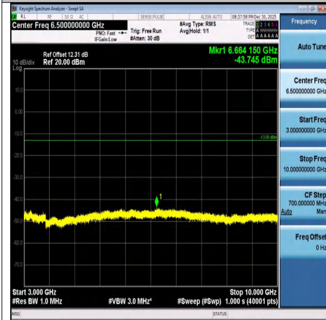
Band26(824-849)-5MHz-QPSK-26815-25RB#0-3000~100 00-PASS
