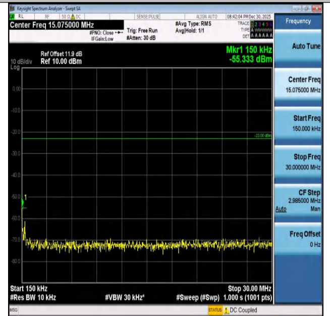
Band26(824-849)-5MHz-16QAM-26915-1RB#24-0.15~30- PASS
