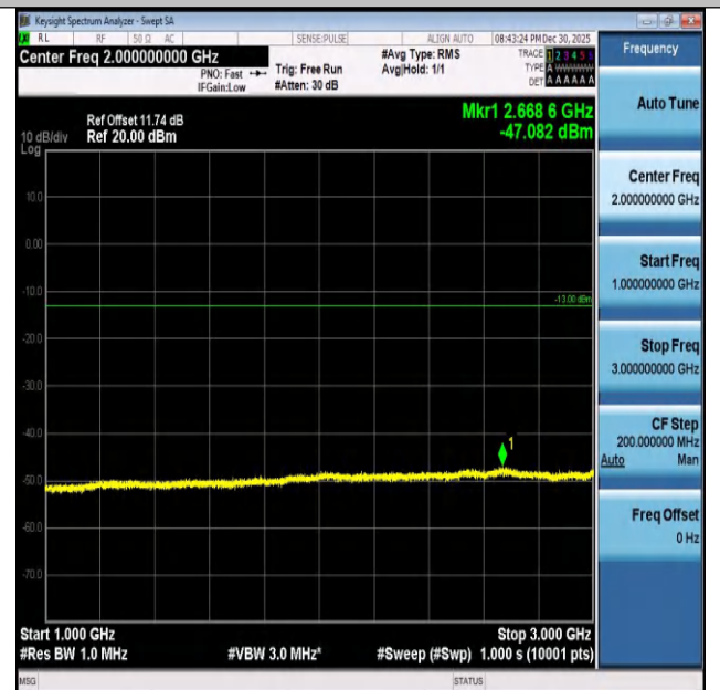
Band26(824-849)-5MHz-QPSK-26915-25RB#0-1000~300
