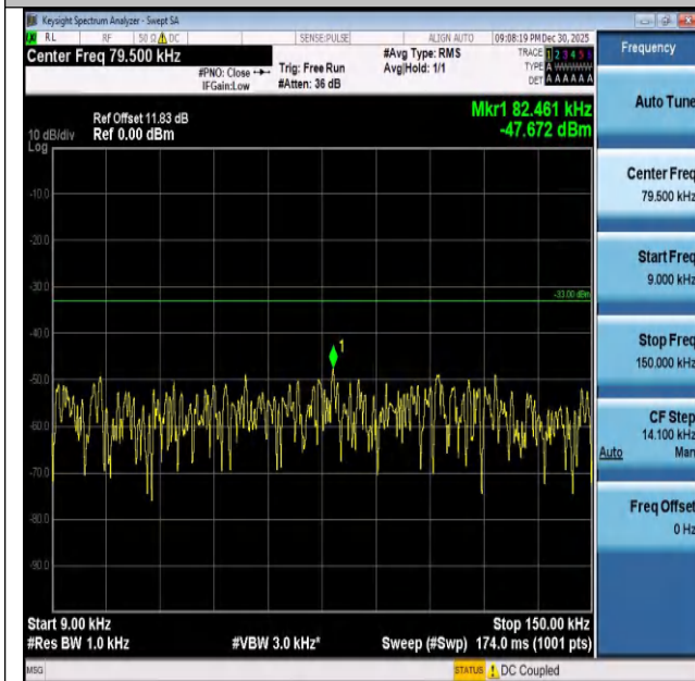
Band26(824-849)-10MHz-QPSK-26840-1RB#0-0.009~0.1 5-PASS
