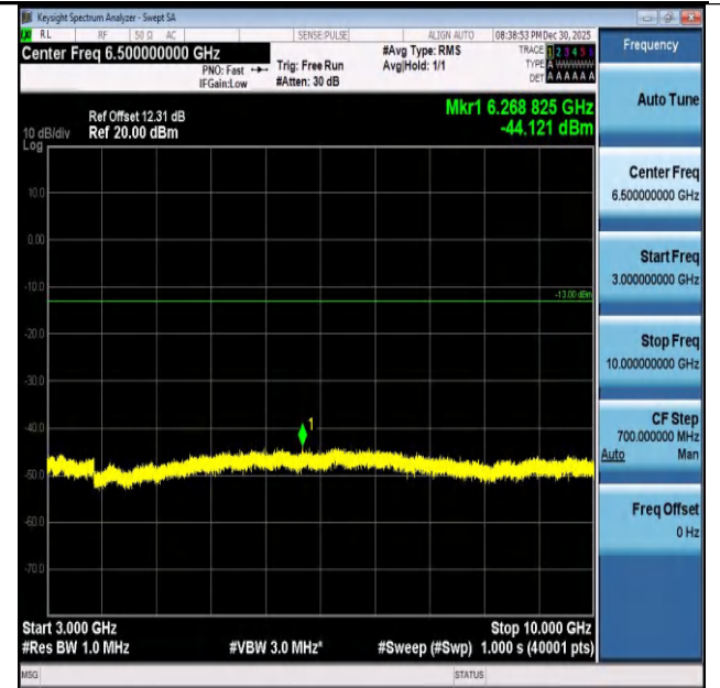
Band26(824-849)-5MHz-16QAM-26815-25RB#0-3000~10 000-PASS
