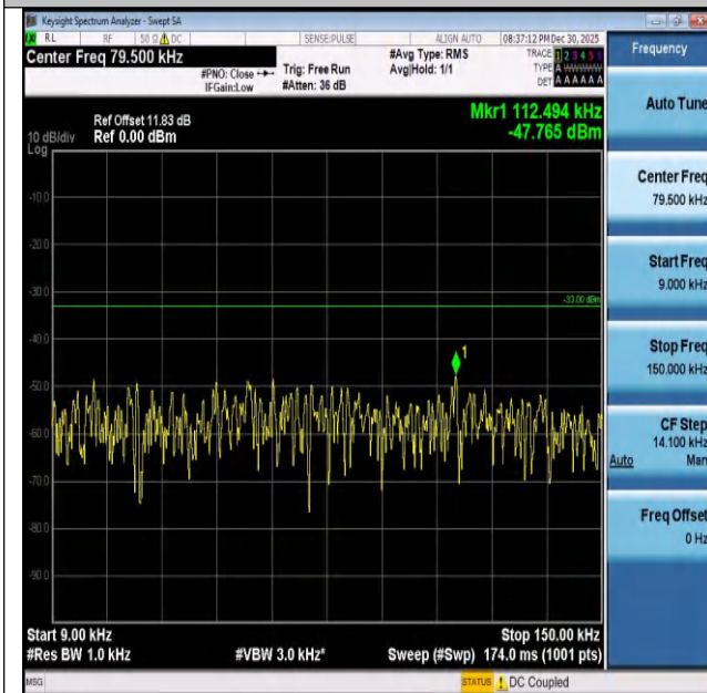
Band26(824-849)-5MHz-QPSK-26815-25RB#0-0.009~0.1 5-PASS
