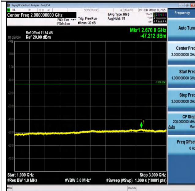
Band26(824-849)-10MHz-QPSK-26840-1RB#49-1000~3000- 00-PASS
