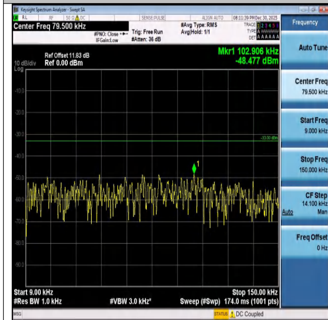
Band26(824-849)-3MHz-16QAM-27025-1RB#14-0.009~0. 15-PASS
