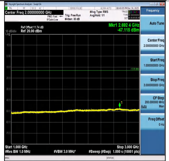
Band26(824-849)-5MHz-QPSK-27015-25RB#0-1000~300 0-PASS
