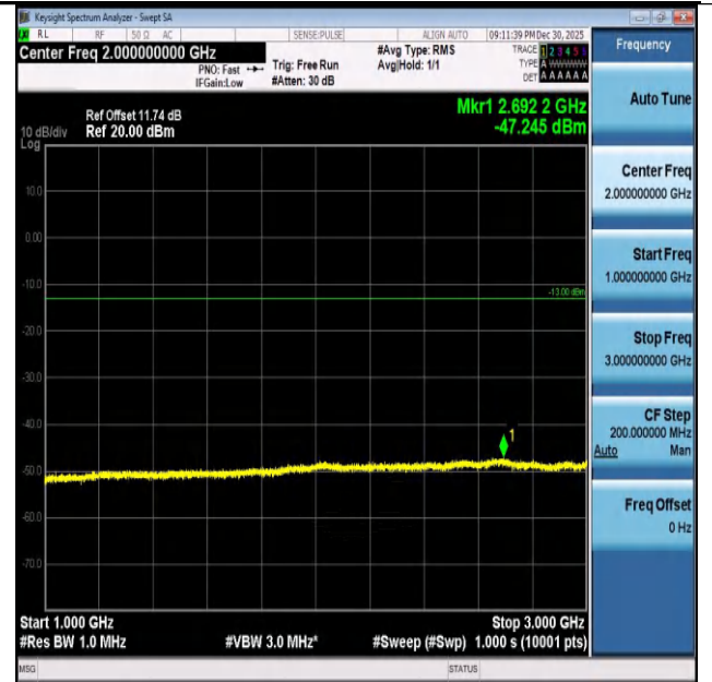
Band26(824-849)-10MHz-16QAM-26840-1RB#49-1000~3 000-PASS
