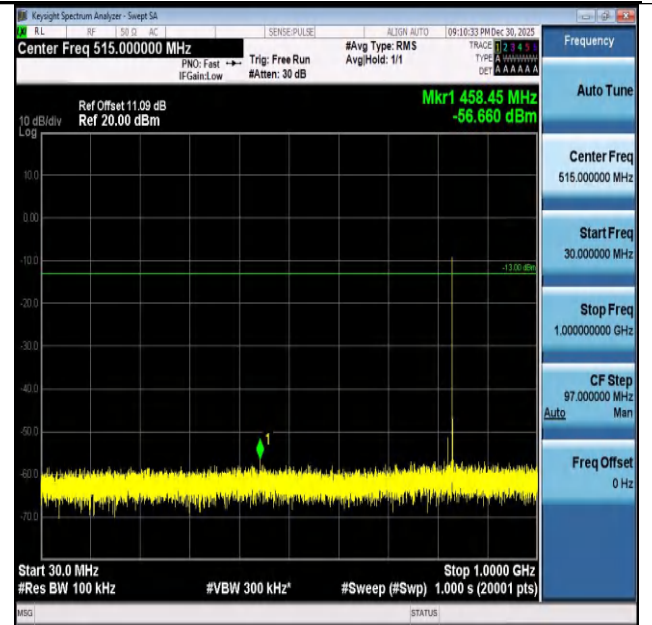
Band26(824-849)-10MHz-QPSK-26840-1RB#49-30~1000- PASS
