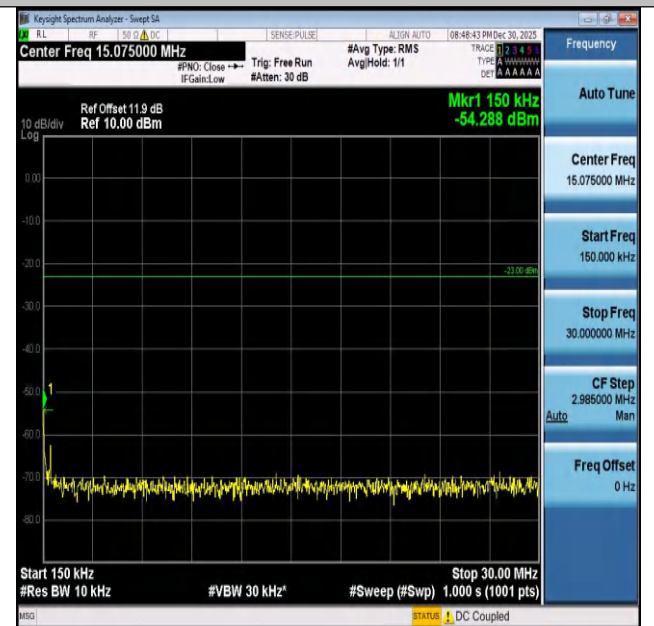
Band26(824-849)-5MHz-QPSK-27015-25RB#0-0.15~30-P ASS
