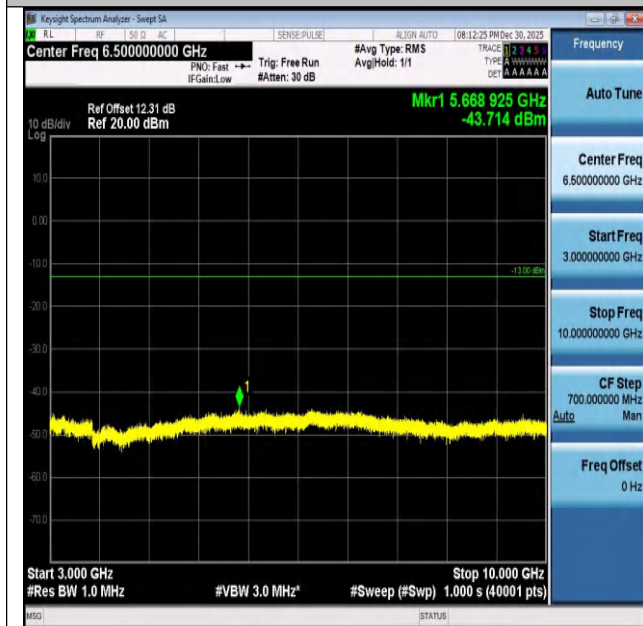
Band26(824-849)-3MHz-16QAM-27025-1RB#14-3000~10000-PASS
