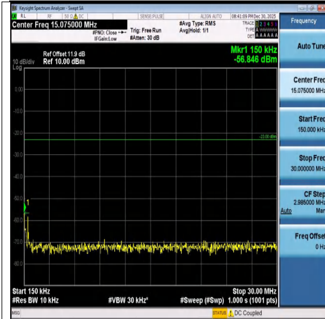
Band26(824-849)-5MHz-QPSK-26915-1RB#24-0.15~30-P
