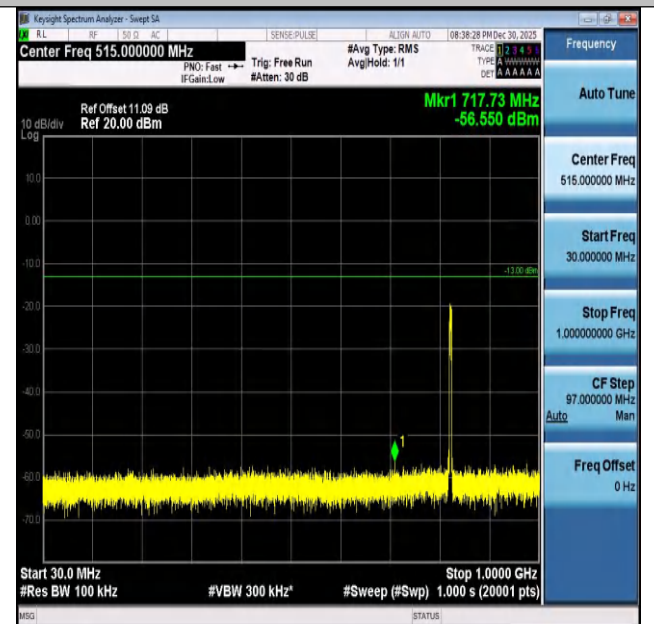
Band26(824-849)-5MHz-16QAM-26815-25RB#0-30~1000- PASS
