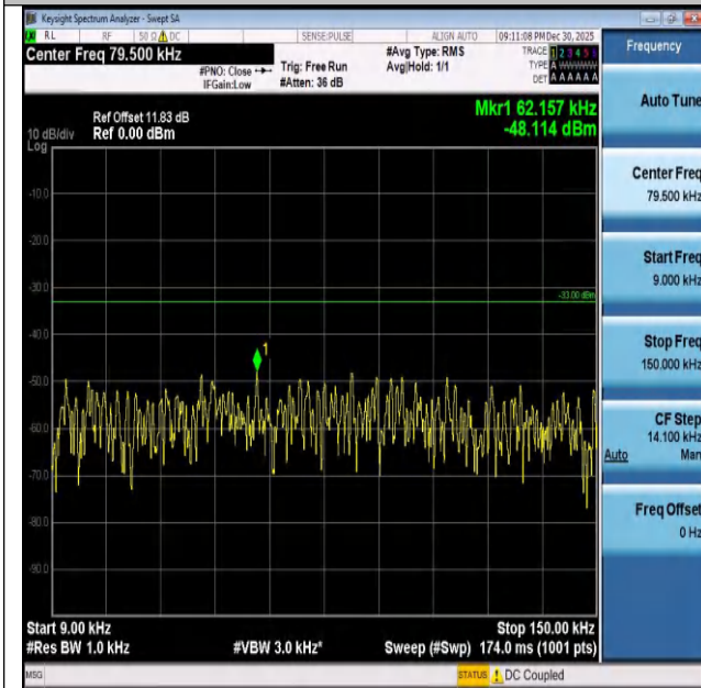
Band26(824-849)-10MHz-16QAM-26840-1RB#49-0.009~0 .15-PASS
