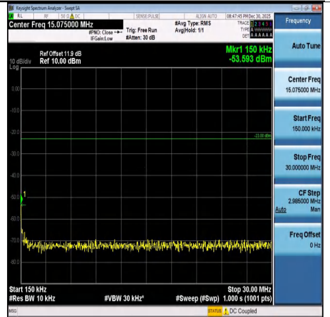
Band26(824-849)-5MHz-16QAM-27015-1RB#24-0.15~30- PASS
