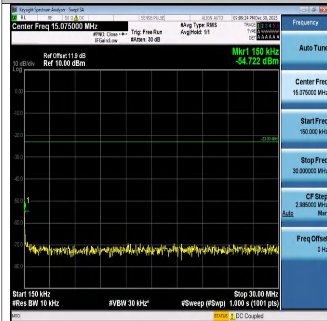
Band26(824-849)-10MHz-16QAM-26840-1RB#0-0.15~30-PASS
