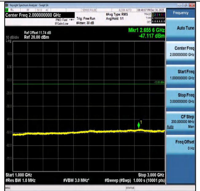
Band26(824-849)-5MHz-16QAM-27015-1RB#24-1000~30 00-PASS
