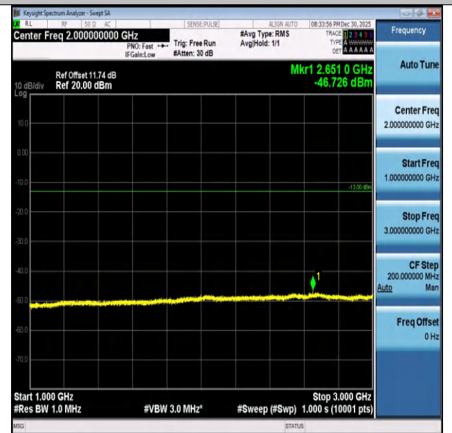
Band26(824-849)-5MHz-QPSK-26815-1RB#0-1000~3000-
