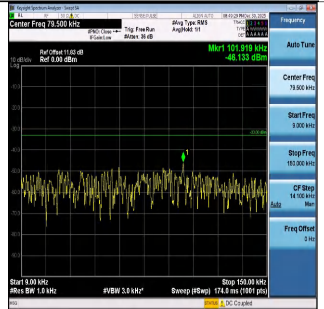
Band26(824-849)-5MHz-16QAM-27015-25RB#0-0.009~0.15-PASS
