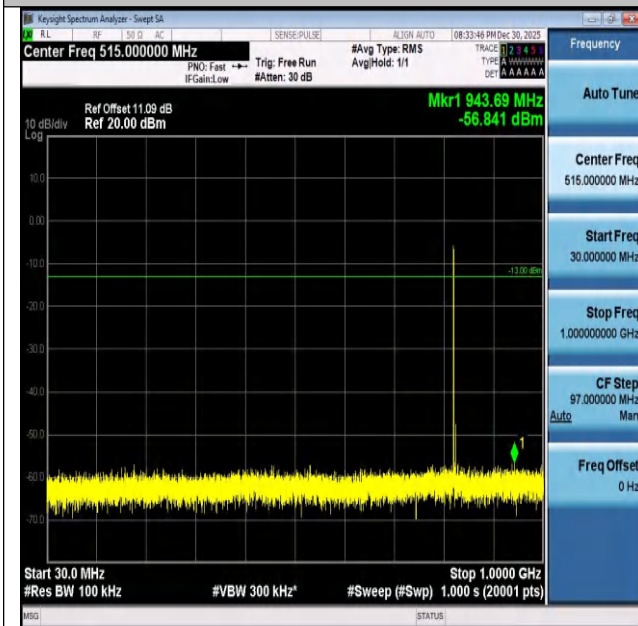
Band26(824-849)-5MHz-QPSK-26815-1RB#0-30~1000-PA
