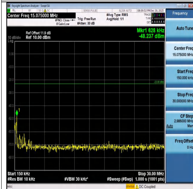
Band26(824-849)-3MHz-16QAM-27025-1RB#0-0.15~30-P ASS
