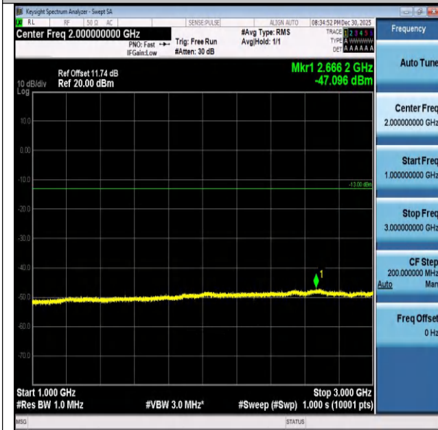
Band26(824-849)-5MHz-16QAM-26815-1RB#0-1000~300 0-PASS
