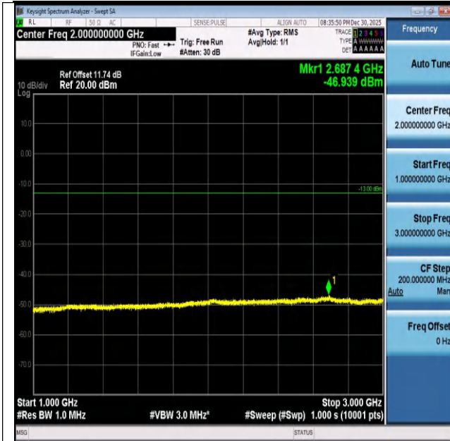
Band26(824-849)-5MHz-QPSK-26815-1RB#24-1000~300 0-PASS
