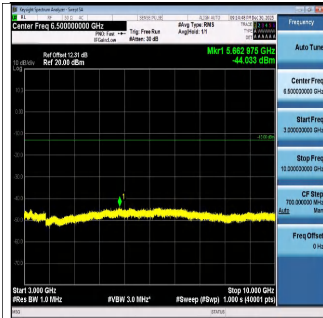
Band26(824-849)-10MHz-QPSK-26915-1RB#0-3000~10000-PASS
