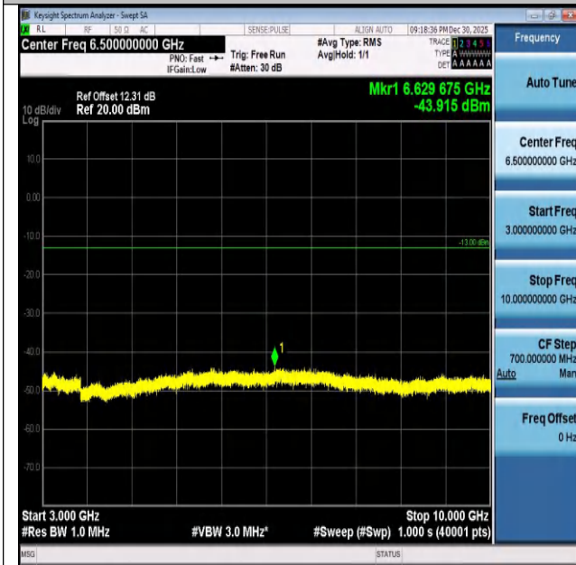
Band26(824-849)-10MHz-QPSK-26915-50RB#0-3000~10000-PASS
