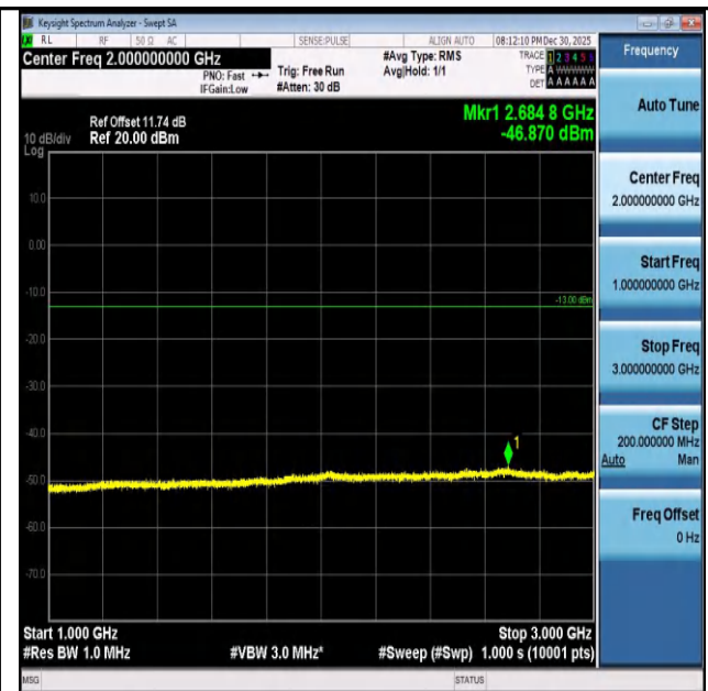
Band26(824-849)-3MHz-16QAM-27025-1RB#14-1000~3000-PASS
