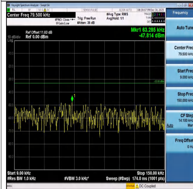
Band26(824-849)-5MHz-QPSK-26915-1RB#0-0.009~0.15- PASS
