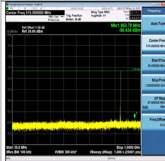
Band26(824-849)-5MHz-16QAM-27015-1RB#24-30~1000- PASS
