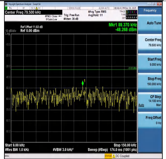
Band26(824-849)-5MHz-QPSK-27015-1RB#24-0.009~0.1 5-PASS
