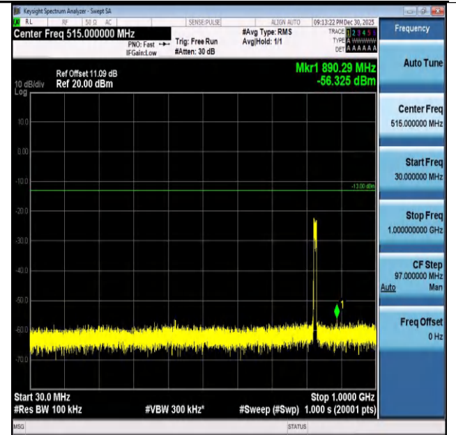
Band26(824-849)-10MHz-16QAM-26840-50RB#0-30~100 0-PASS
