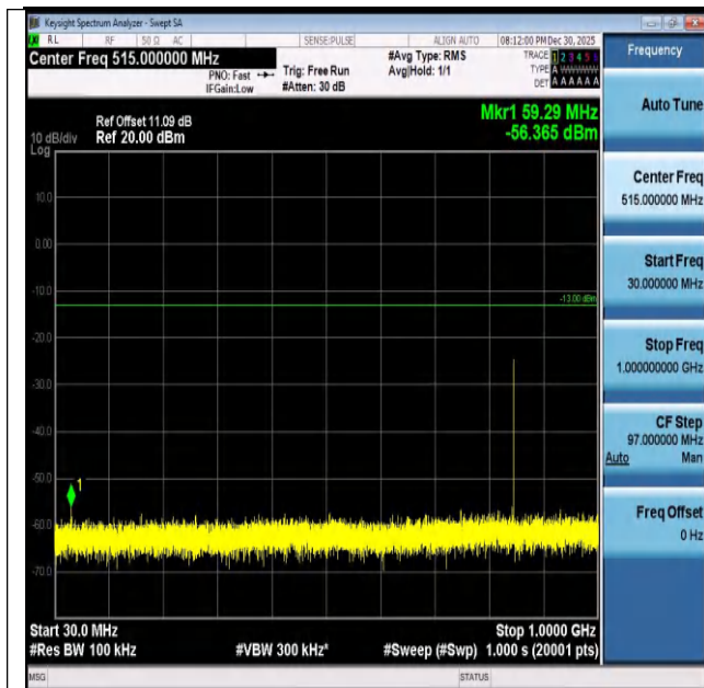
Band26(824-849)-3MHz-16QAM-27025-1RB#14-30~1000-PASS
