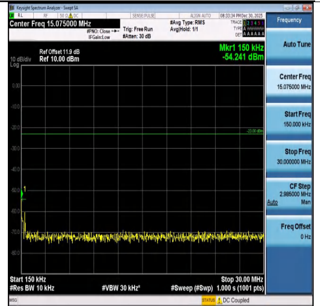
Band26(824-849)-5MHz-QPSK-26815-1RB#0-0.15~30-PA
