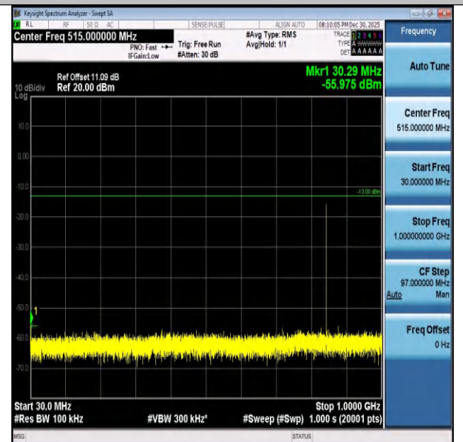
Band26(824-849)-3MHz-16QAM-27025-1RB#0-30~1000-P ASS
