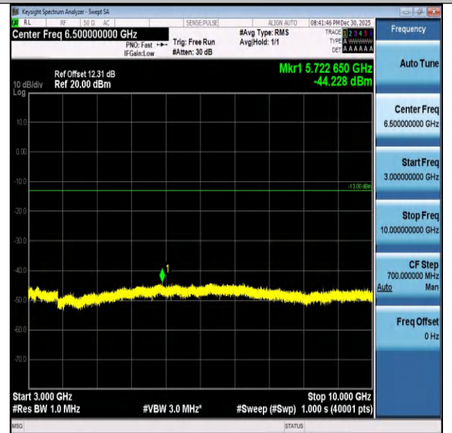
Band26(824-849)-5MHz-QPSK-26915-1RB#24-3000~100
