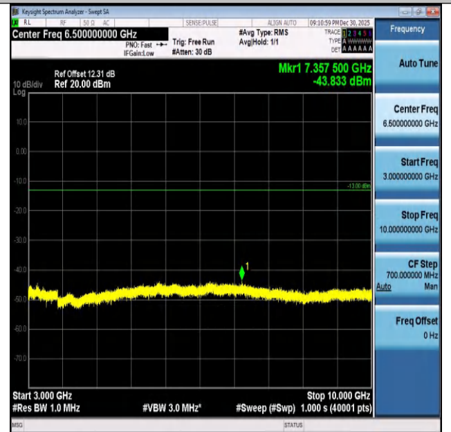
Band26(824-849)-10MHz-QPSK-26840-1RB#49-3000~10000- 000-PASS
