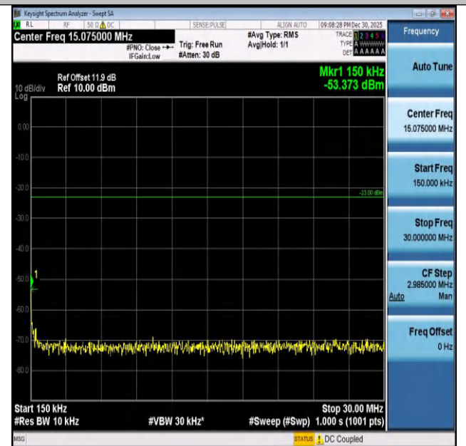
Band26(824-849)-10MHz-QPSK-26840-1RB#0-0.15~30-P ASS
