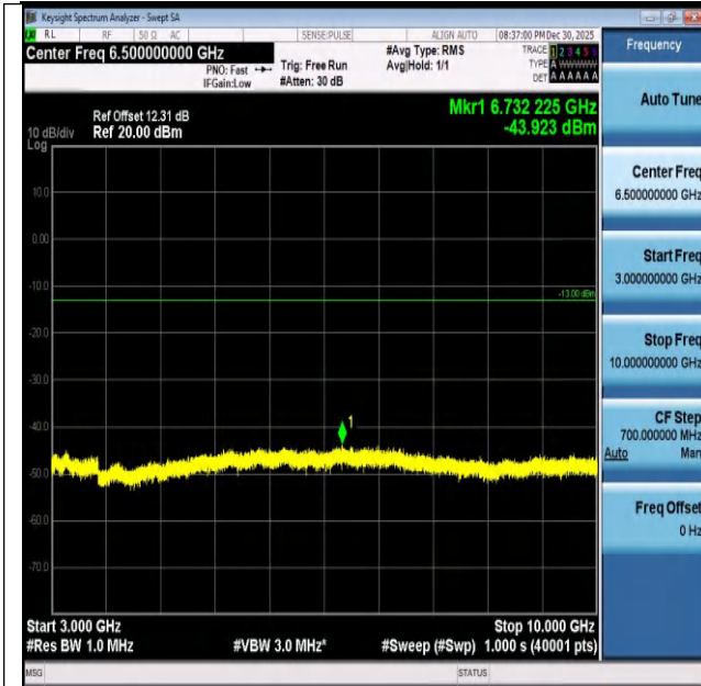
Band26(824-849)-5MHz-16QAM-26815-1RB#24-3000~10 000-PASS
