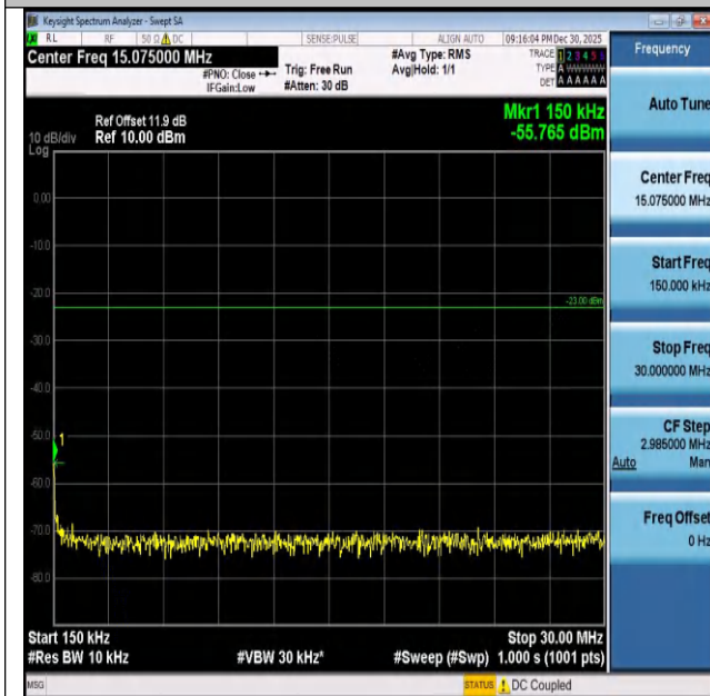
Band26(824-849)-10MHz-QPSK-26915-1RB#49-0.15~30-PASS
