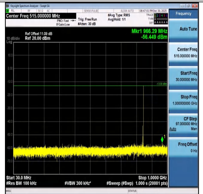
Band26(824-849)-5MHz-QPSK-27015-1RB#24-30~1000-P ASS
