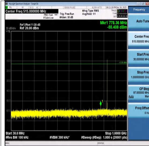
Band26(824-849)-10MHz-16QAM-26840-1RB#49-30~100 0-PASS
