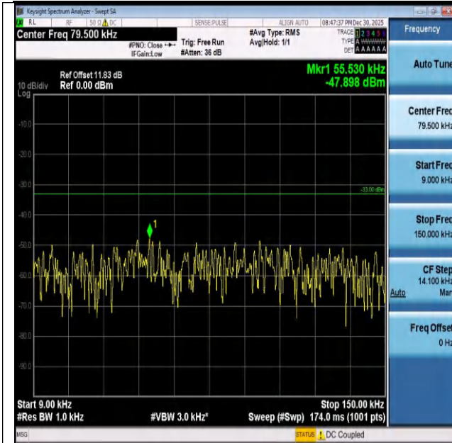
Band26(824-849)-5MHz-16QAM-27015-1RB#24-0.009~0. 15-PASS
