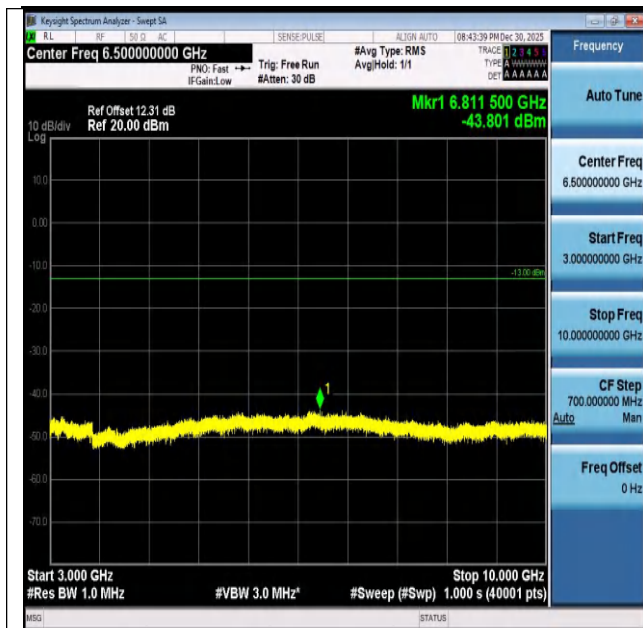
Band26(824-849)-5MHz-QPSK-26915-25RB#0-3000~100 00-PASS
