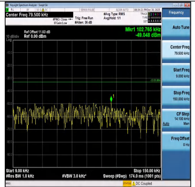
Band26(824-849)-5MHz-16QAM-26815-1RB#0-0.009~0.1 5-PASS
