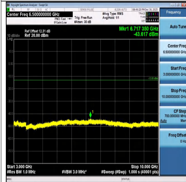
Band26(824-849)-5MHz-QPSK-27015-25RB#0-3000~100 00-PASS
