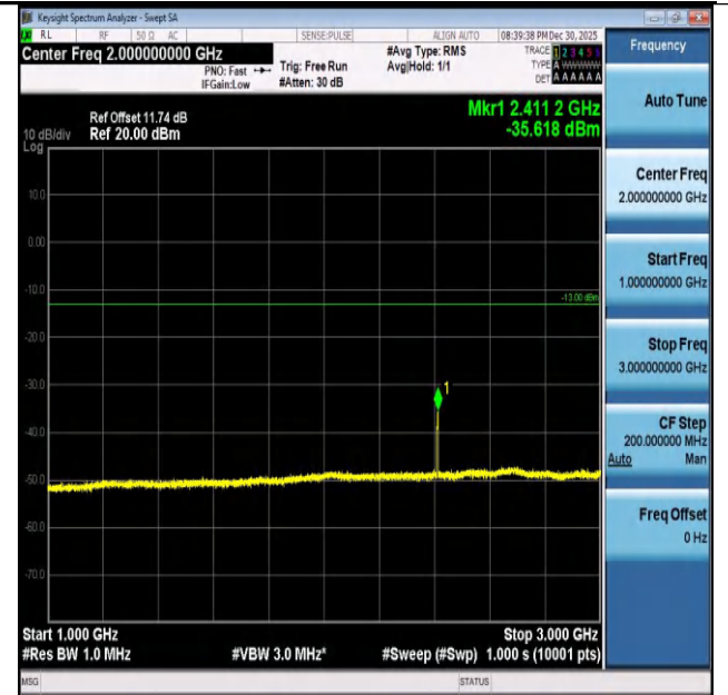
Band26(824-849)-5MHz-QPSK-26915-1RB#0-1000~3000- PASS
