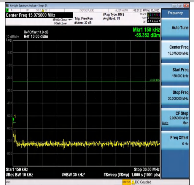
Band26(824-849)-5MHz-QPSK-26815-25RB#0-0.15~30-P ASS
