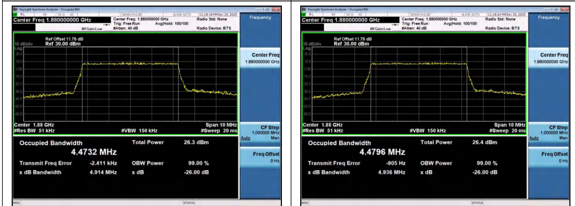
Band2-5MHz-16QAM-18900-25RB#0-PASS
