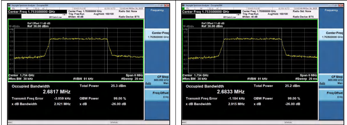
Band4-3MHz-16QAM-20385-15RB#0-PASS
