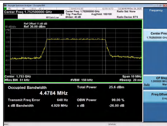
Band4-5MHz-16QAM-20375-25RB#0-PASS
