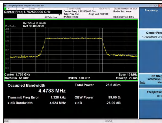
Band4-5MHz-16QAM-20375-25RB#0-PASS
