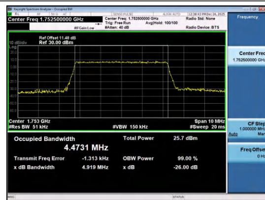
Band4-5MHz-16QAM-20375-25RB#0-PASS
