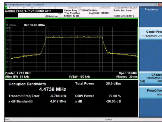
Band4-5MHz-QPSK-19975-25RB#0-PASS
