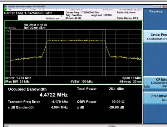
Band4-5MHz-16QAM-20175-25RB#0-PASS
