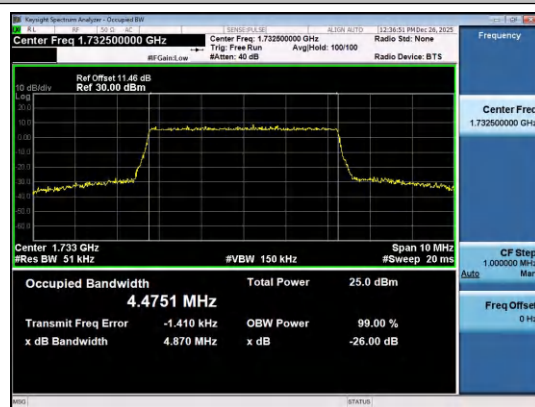
Band4-5MHz-16QAM-20175-25RB#0-PASS
