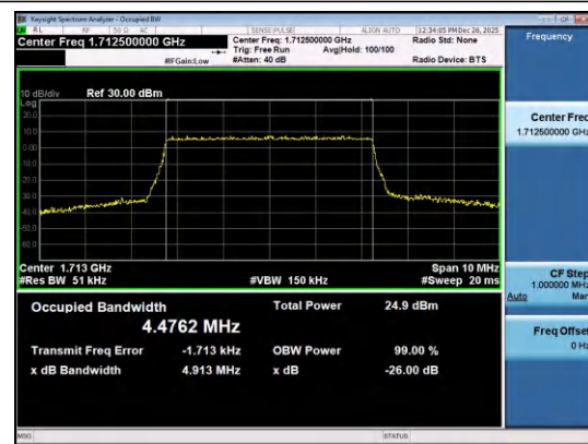
Band4-5MHz-16QAM-19975-25RB#0-PASS
