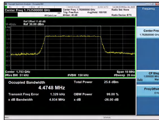
Band4-5MHz-16QAM-20375-25RB#0-PASS
