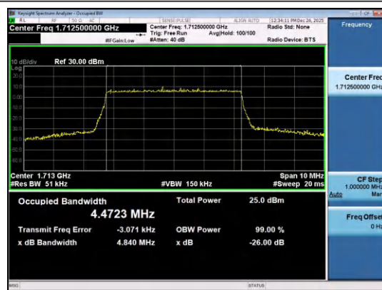
Band4-5MHz-QPSK-19975-25RB#0-PASS
