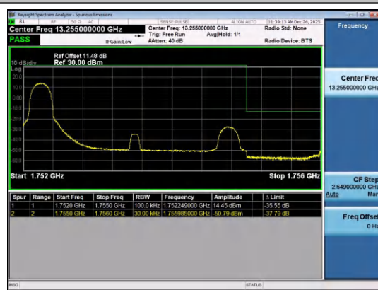
Band4-3MHz-16QAM-20385-1RB#0-PASS
