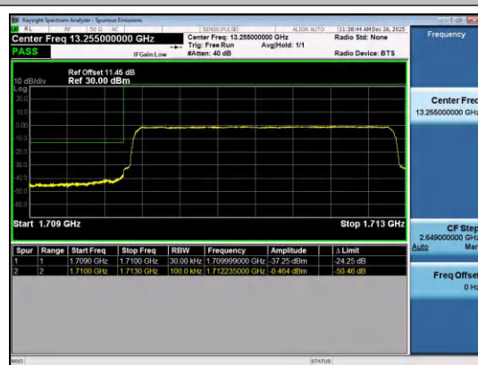
Band4-3MHz-16QAM-19965-15RB#0-PASS
