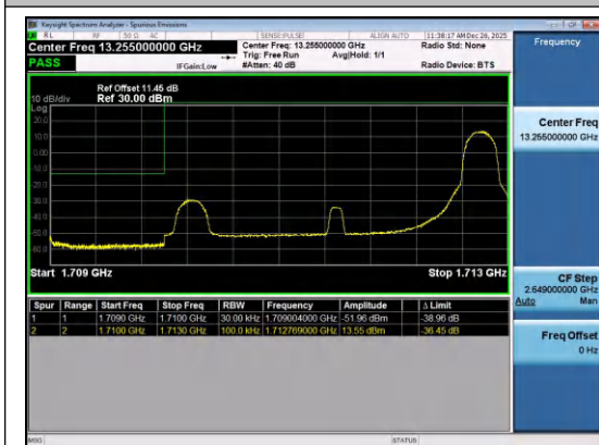
Band4-3MHz-16QAM-19965-1RB#14-PASS
