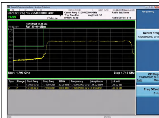
Band4-3MHz-QPSK-19965-15RB#0-PASS
