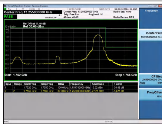
Band4-3MHz-QPSK-20385-1RB#14-PASS
