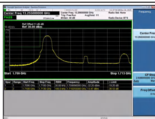
Band4-3MHz-16QAM-19965-1RB#0-PASS
