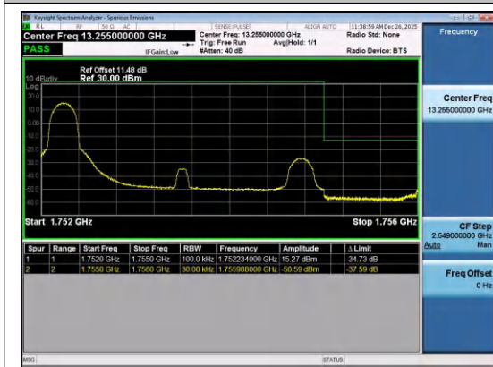
Band4-3MHz-QPSK-20385-1RB#0-PASS
