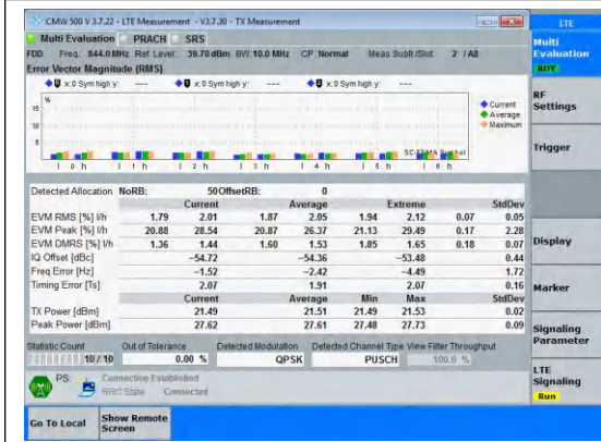
Band5-10MHz-QPSK-20600-50RB#0-PASS
