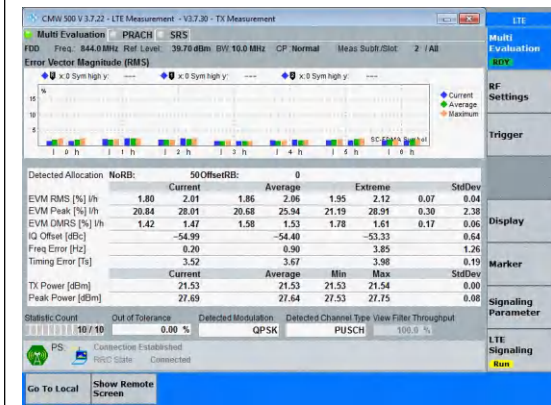
Band5-10MHz-QPSK-20600-50RB#0-PASS
