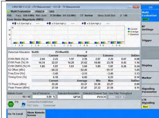
Band5-5MHz-QPSK-20425-25RB#0-PASS
