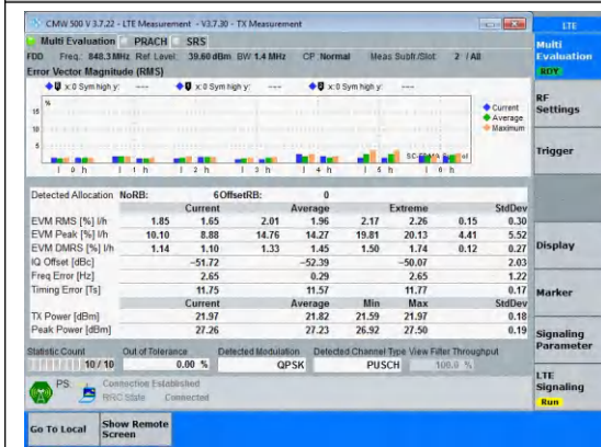
Band5-1.4MHz-QPSK-20643-6RB#0-PASS
