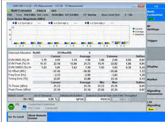
Band5-5MHz-QPSK-20525-25RB#0-PASS
