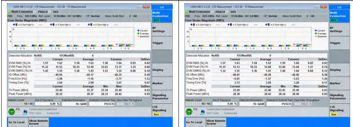
Band5-3MHz-16QAM-20415-15RB#0-PASS
