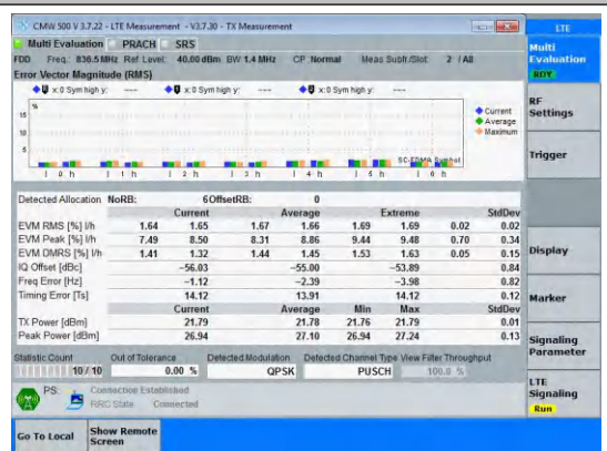
Band5-1.4MHz-QPSK-20525-6RB#0-PASS
