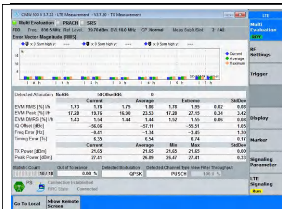
Band5-10MHz-QPSK-20525-50RB#0-PASS
