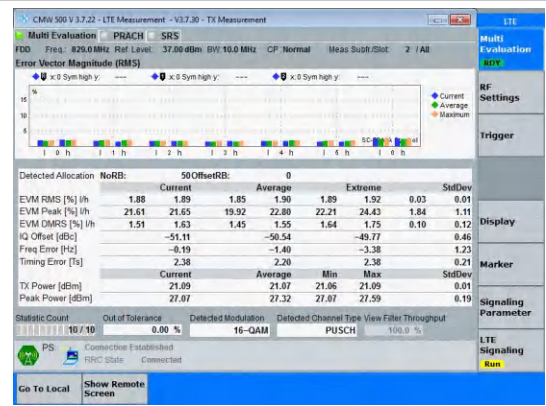
Band5-10MHz-16QAM-20450-50RB#0-PASS
