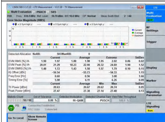
Band5-10MHz-16QAM-20525-50RB#0-PASS
