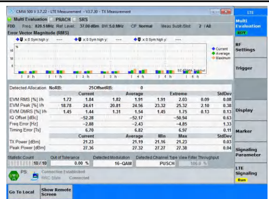
Band5-5MHz-16QAM-20425-25RB#0-PASS
