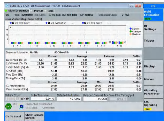
Band5-10MHz-16QAM-20450-50RB#0-PASS
