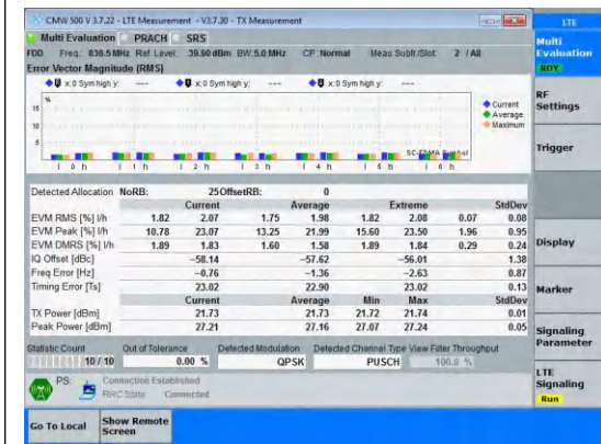
Band5-5MHz-QPSK-20525-25RB#0-PASS
