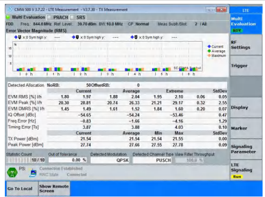
Band5-10MHz-QPSK-20600-50RB#0-PASS
