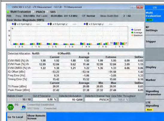
Band5-1.4MHz-16QAM-20525-6RB#0-PASS
