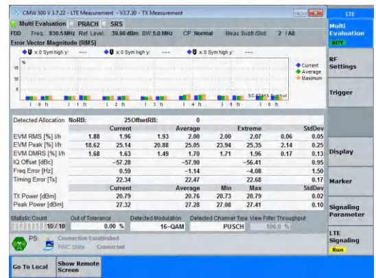
Band5-5MHz-16QAM-20525-25RB#0-PASS
