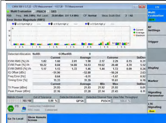
Band5-1.4MHz-QPSK-20643-6RB#0-PASS
