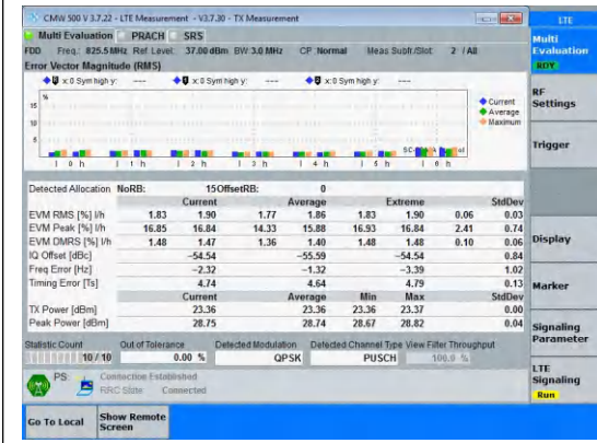
Band5-3MHz-QPSK-20415-15RB#0-PASS
