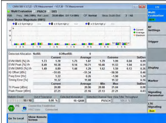
Band5-1.4MHz-16QAM-20643-6RB#0-PASS
