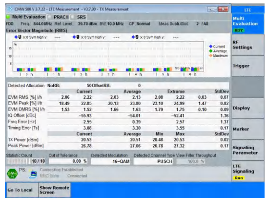
Band5-10MHz-16QAM-20600-50RB#0-PASS
