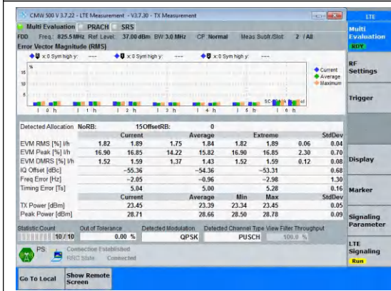
Band5-3MHz-QPSK-20415-15RB#0-PASS
