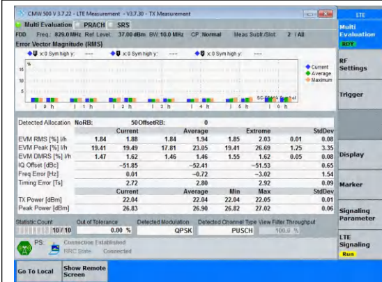
Band5-10MHz-QPSK-20450-50RB#0-PASS
