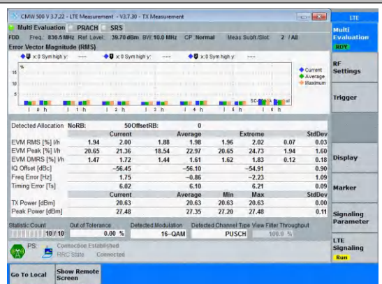
Band5-10MHz-16QAM-20525-50RB#0-PASS
