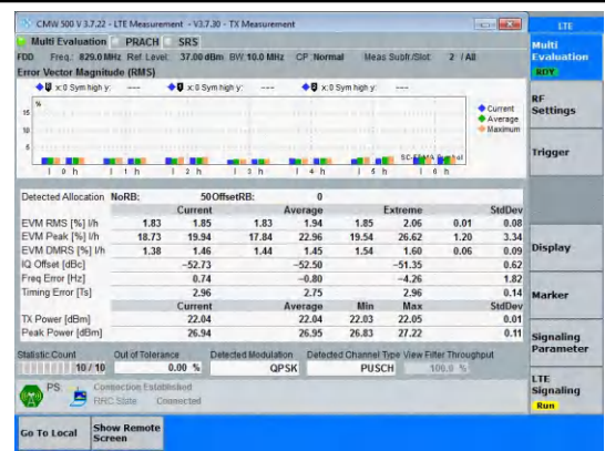
Band5-10MHz-QPSK-20450-50RB#0-PASS
