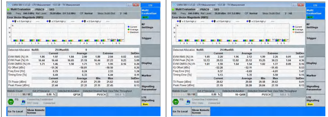
Band5-5MHz-QPSK-20625-25RB#0-PASS
