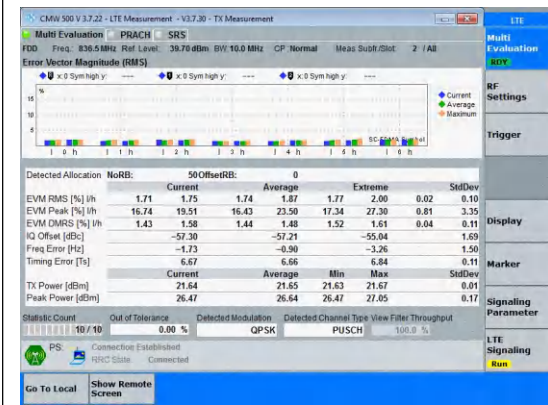
Band5-10MHz-QPSK-20525-50RB#0-PASS
