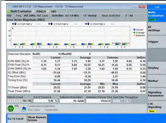
Band5-1.4MHz-16QAM-20643-6RB#0-PASS
