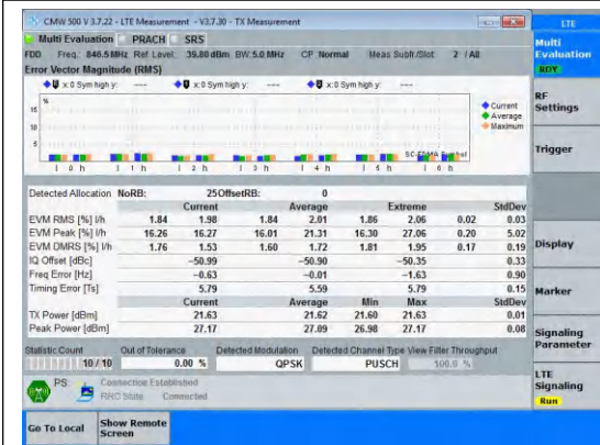
Band5-5MHz-QPSK-20625-25RB#0-PASS
