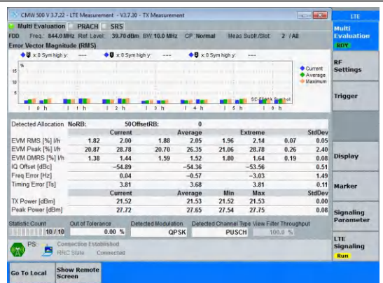
Band5-10MHz-QPSK-20600-50RB#0-PASS
