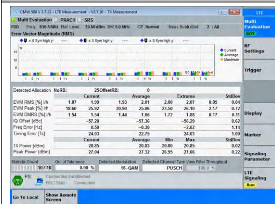
Band5-5MHz-16QAM-20525-25RB#0-PASS
