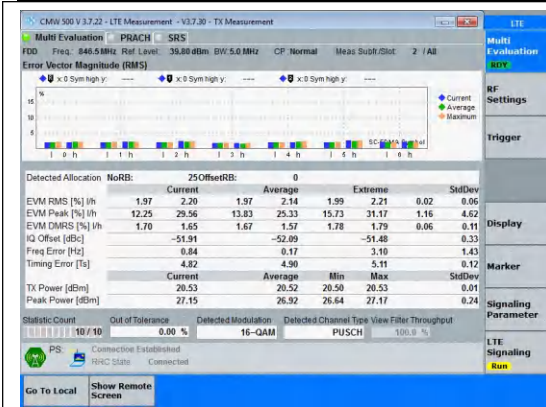
Band5-5MHz-16QAM-20625-25RB#0-PASS
