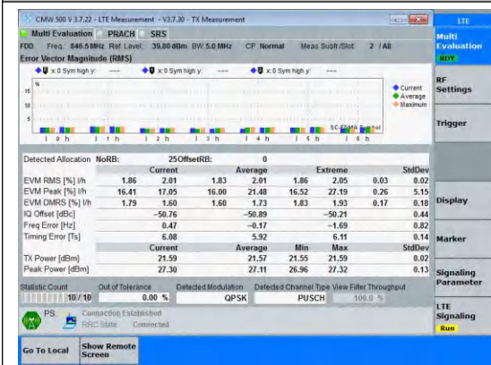
Band5-5MHz-QPSK-20625-25RB#0-PASS
