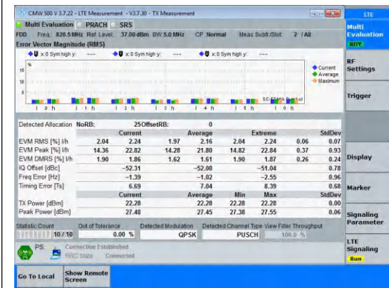
Band5-5MHz-QPSK-20425-25RB#0-PASS
