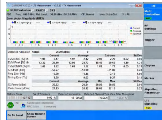
Band5-5MHz-16QAM-20625-25RB#0-PASS
