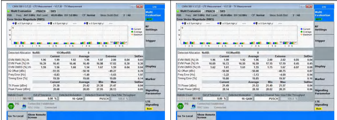
Band5-3MHz-16QAM-20635-15RB#0-PASS
