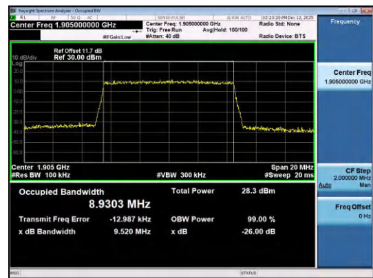
Band2-10MHz-16QAM-19150-50RB#0-PASS
