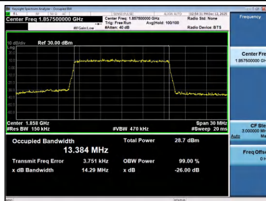
Band2-15MHz-16QAM-18675-75RB#0-PASS
