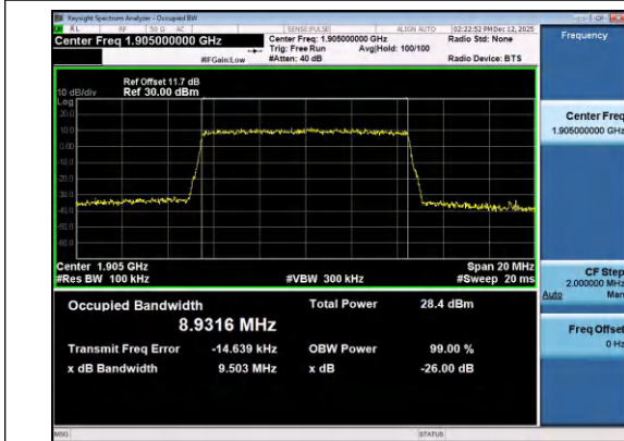
Band2-10MHz-16QAM-19150-50RB#0-PASS
