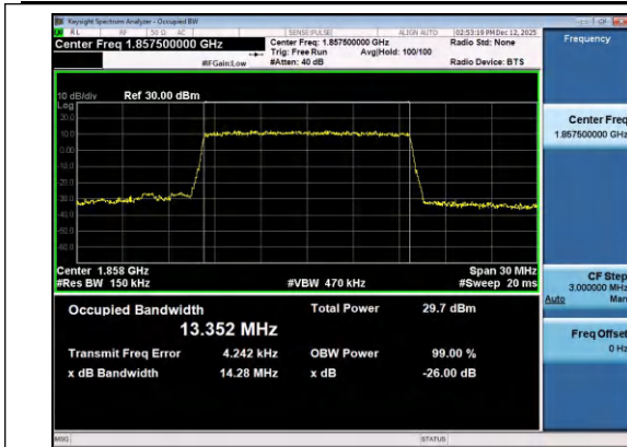
Band2-15MHz-QPSK-18675-75RB#0-PASS
