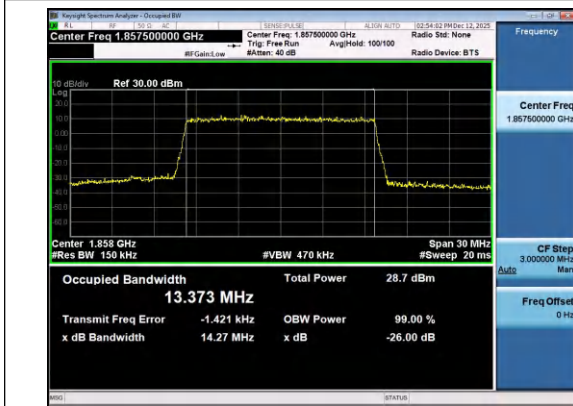
Band2-15MHz-16QAM-18675-75RB#0-PASS
