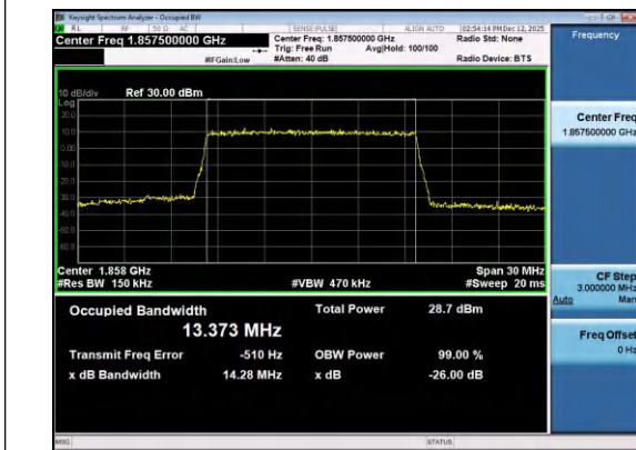
Band2-15MHz-16QAM-18675-75RB#0-PASS
