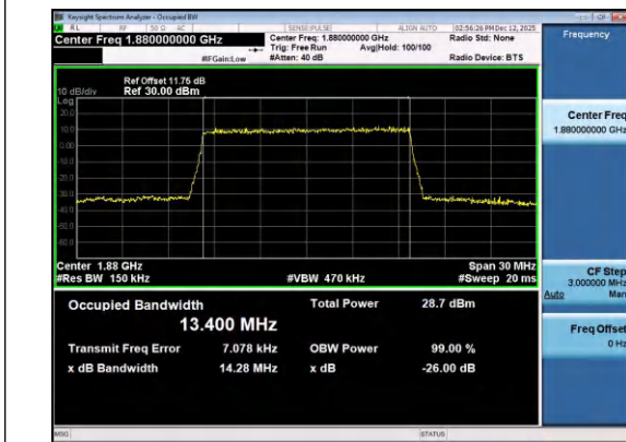
Band2-15MHz-16QAM-18900-75RB#0-PASS
