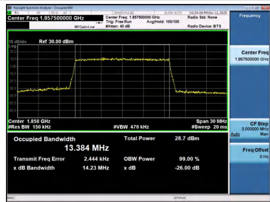
Band2-15MHz-16QAM-18675-75RB#0-PASS
