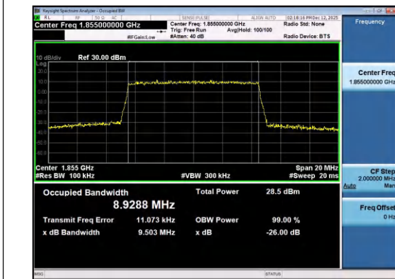
Band2-10MHz-16QAM-18650-50RB#0-PASS
