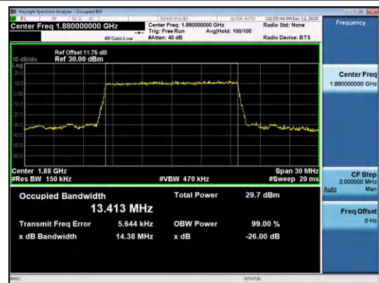
Band2-15MHz-QPSK-18900-75RB#0-PASS
