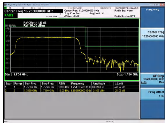
Band4-1.4MHz-16QAM-20393-6RB#0-PASS
