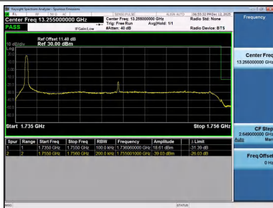
Band4-20MHz-QPSK-20300-1RB#0-PASS
