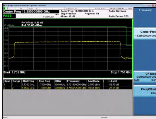
Band4-20MHz-QPSK-20300-100RB#0-PASS
