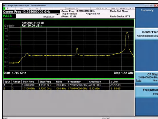
Band4-10MHz-16QAM-20000-1RB#49-PASS
