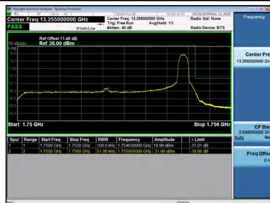
Band4-5MHz-QPSK-20375-1RB#24-PASS
