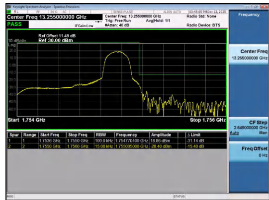
Band4-1.4MHz-QPSK-20393-1RB#5-PASS
