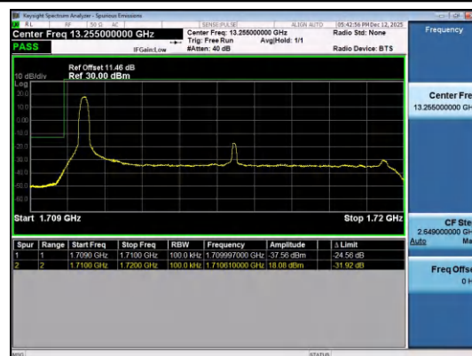
Band4-10MHz-16QAM-20000-1RB#0-PASS
