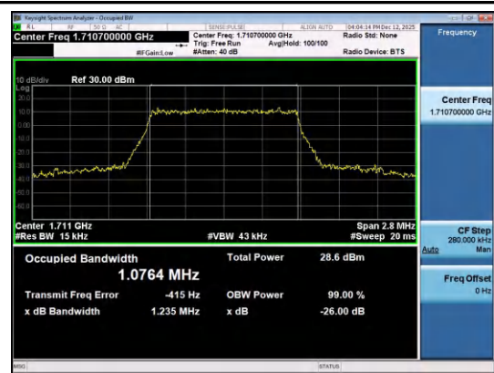
Band4-1.4MHz-16QAM-19957-6RB#0-PASS
