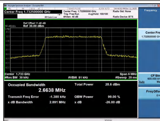
Band4-3MHz-16QAM-20175-15RB#0-PASS
