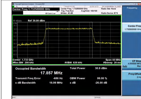
Band4-20MHz-QPSK-20175-100RB#0-PASS
