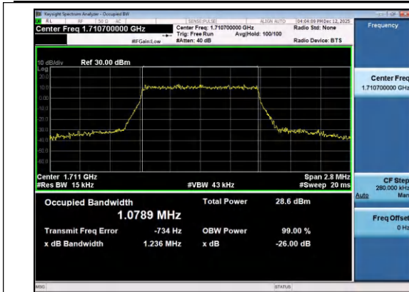
Band4-1.4MHz-16QAM-19957-6RB#0-PASS
