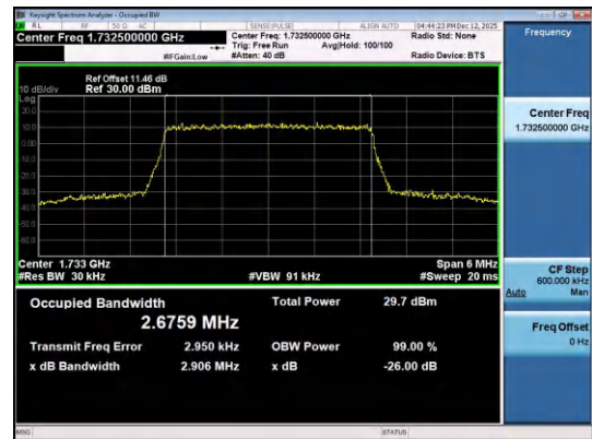
Band4-3MHz-QPSK-20175-15RB#0-PASS
