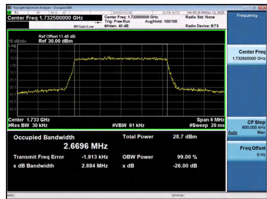
Band4-3MHz-16QAM-20175-15RB#0-PASS
