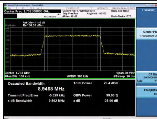
Band4-10MHz-16QAM-20175-50RB#0-PASS
