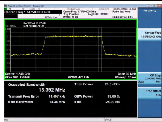
Band4-15MHz-16QAM-20325-75RB#0-PASS
