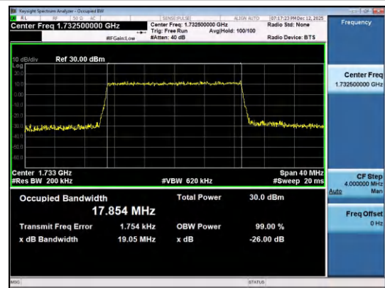
Band4-20MHz-16QAM-20175-100RB#0-PASS
