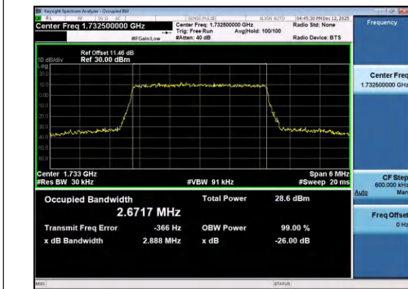
Band4-3MHz-16QAM-20175-15RB#0-PASS
