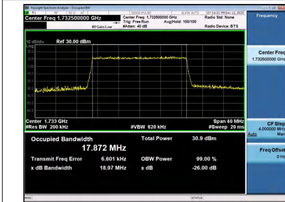
Band4-20MHz-QPSK-20175-100RB#0-PASS
