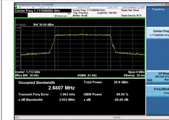
Band4-3MHz-QPSK-19965-15RB#0-PASS
