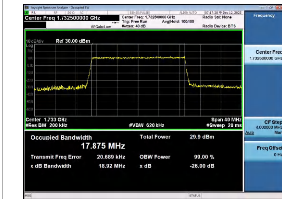
Band4-20MHz-16QAM-20175-100RB#0-PASS
