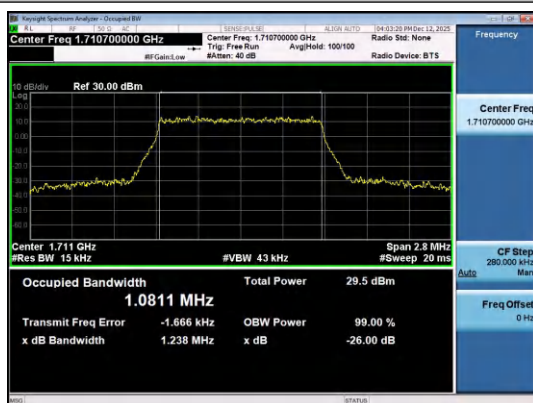
Band4-1.4MHz-QPSK-19957-6RB#0-PASS
