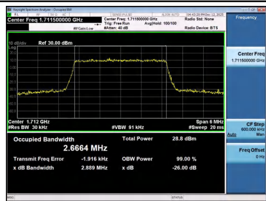
Band4-3MHz-16QAM-19965-15RB#0-PASS
