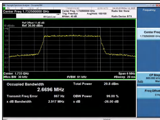
Band4-3MHz-QPSK-20175-15RB#0-PASS
