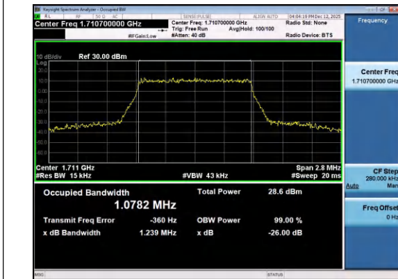
Band4-1.4MHz-16QAM-19957-6RB#0-PASS
