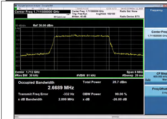
Band4-3MHz-16QAM-19965-15RB#0-PASS
