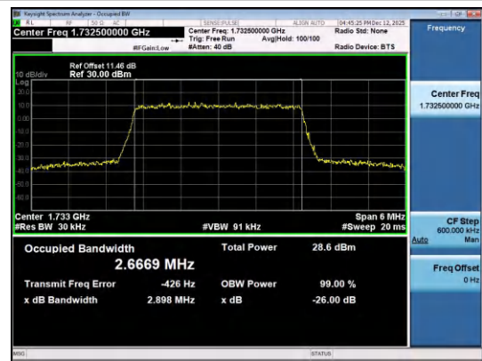
Band4-3MHz-16QAM-20175-15RB#0-PASS
