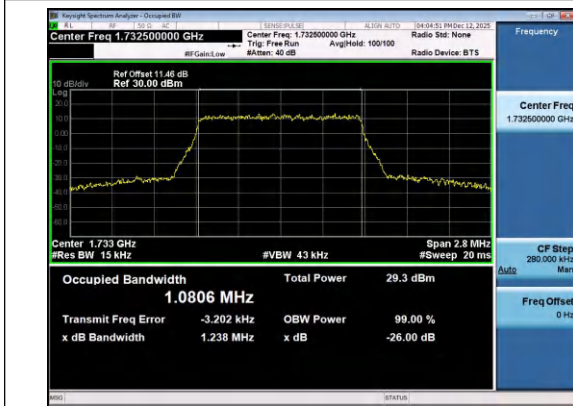
Band4-1.4MHz-QPSK-20175-6RB#0-PASS
