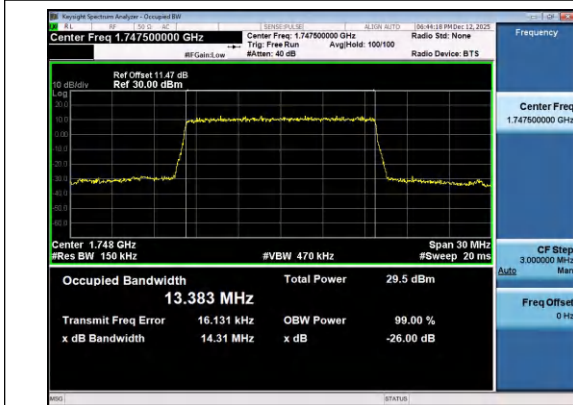
Band4-15MHz-16QAM-20325-75RB#0-PASS
