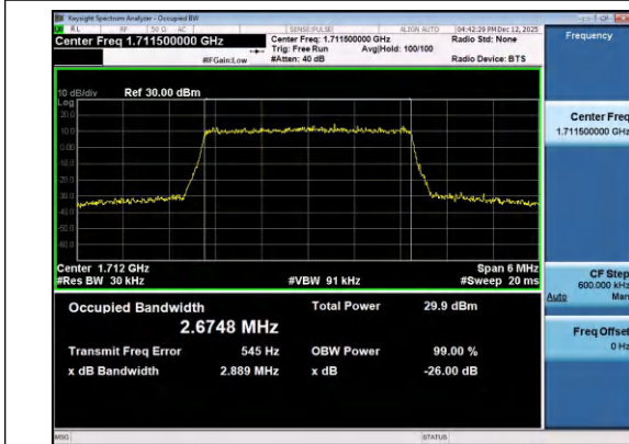
Band4-3MHz-QPSK-19965-15RB#0-PASS
