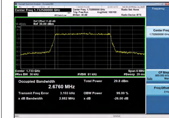
Band4-3MHz-QPSK-20175-15RB#0-PASS
