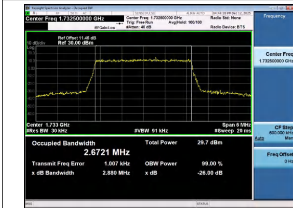
Band4-3MHz-QPSK-20175-15RB#0-PASS
