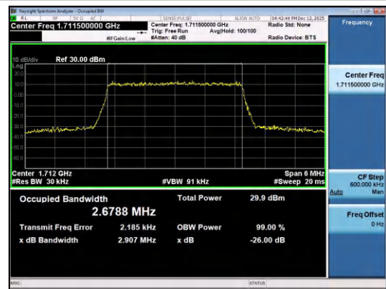
Band4-3MHz-QPSK-19965-15RB#0-PASS
