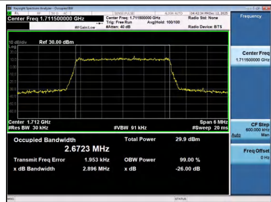
Band4-3MHz-QPSK-19965-15RB#0-PASS
