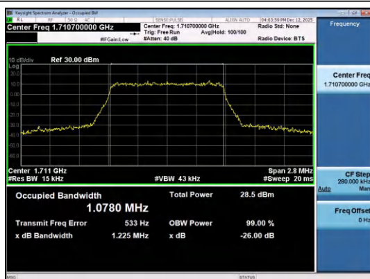
Band4-1.4MHz-16QAM-19957-6RB#0-PASS
