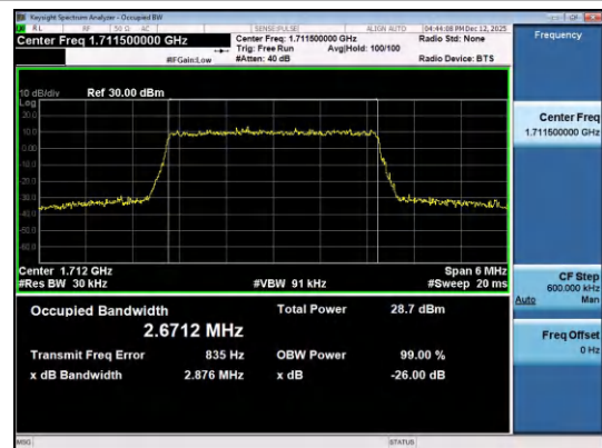
Band4-3MHz-16QAM-19965-15RB#0-PASS
