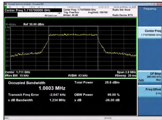
Band4-1.4MHz-16QAM-19957-6RB#0-PASS
