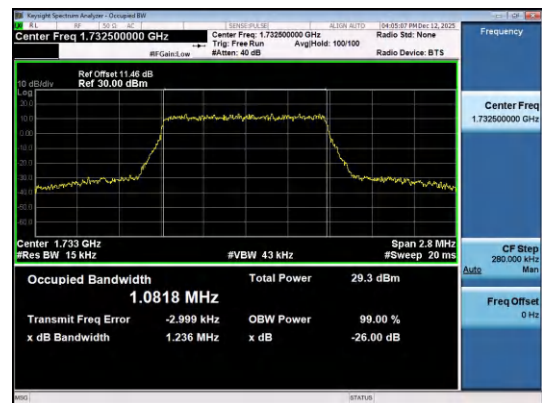
Band4-1.4MHz-QPSK-20175-6RB#0-PASS
