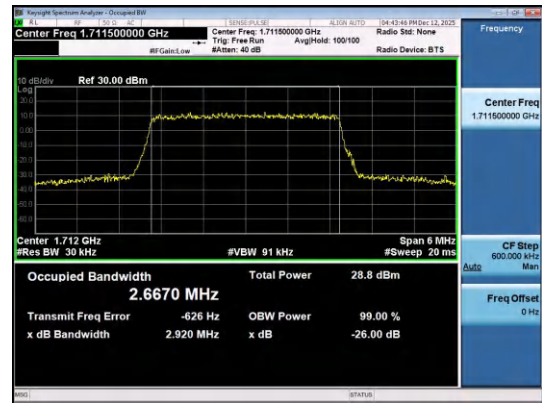
Band4-3MHz-16QAM-19965-15RB#0-PASS
