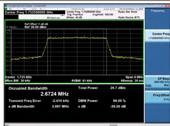
Band4-3MHz-QPSK-20175-15RB#0-PASS
