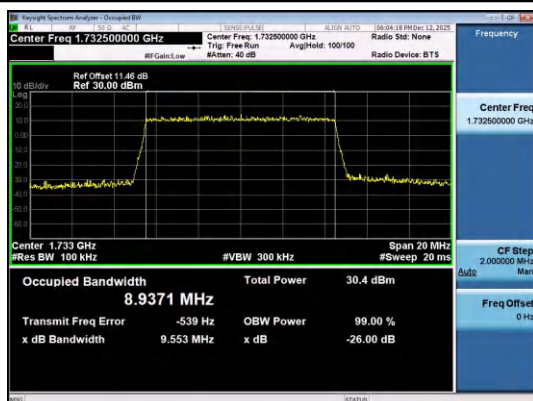
Band4-10MHz-QPSK-20175-50RB#0-PASS
