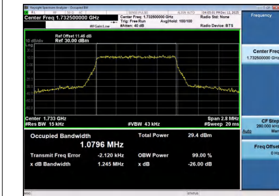
Band4-1.4MHz-QPSK-20175-6RB#0-PASS
