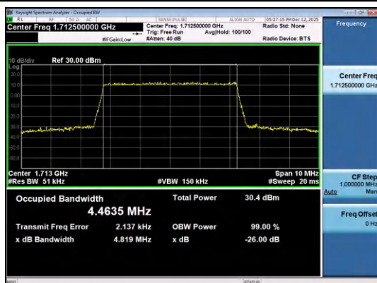
Band4-5MHz-QPSK-19975-25RB#0-PASS
