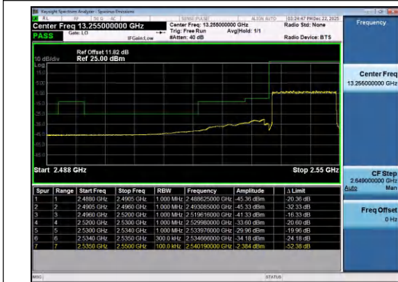
Band41(2535-2655)-15MHz-QPSK-40115-75RB#0-PA
