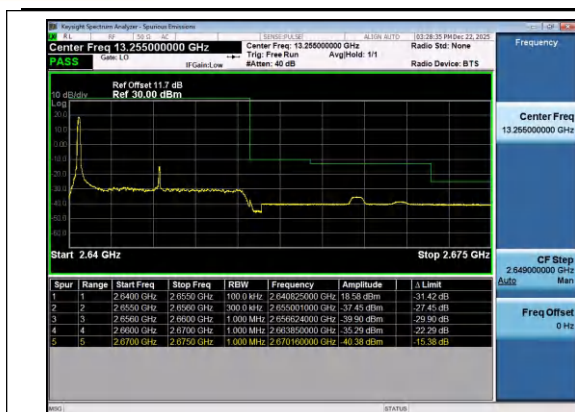
Band41(2535-2655)-15MHz-QPSK-41165-1RB#0-PAS
