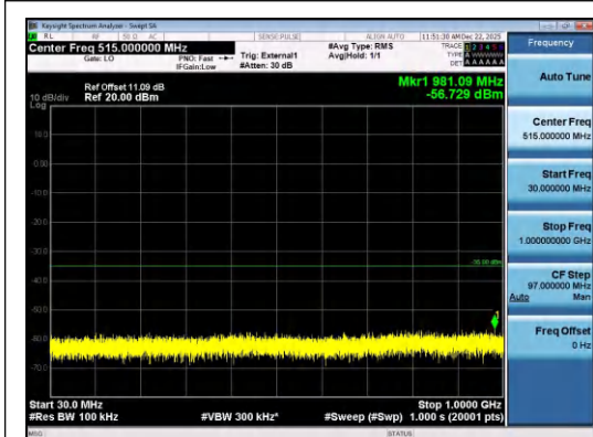
Band41(2535-2655)-5MHz-QPSK-40065-1RB#2 4-30~1000-PASS
