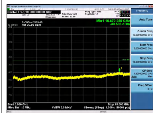
Band41(2535-2655)-5MHz-QPSK-40065-1RB#2 4-3000~18000-PASS
