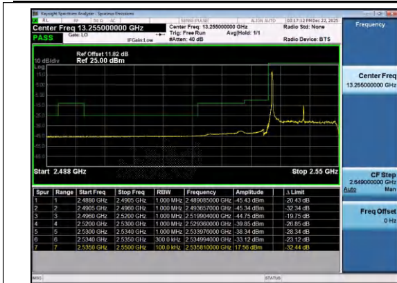
Band41(2535-2655)-15MHz-QPSK-40115-1RB#0-PAS
