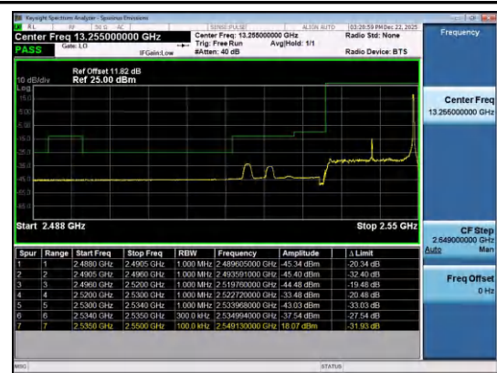
Band41(2535-2655)-15MHz-QPSK-40115-1RB#74-PAS
