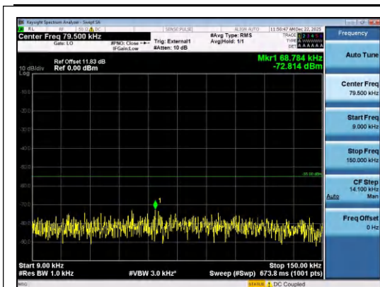
Band41(2535-2655)-5MHz-QPSK-40065-1RB#2 4-0.009~0.15-PASS
