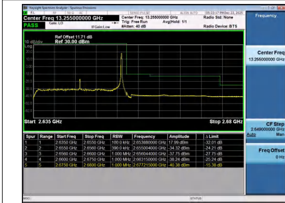
Band41(2535-2655)-20MHz-16QAM-41140-1RB#99-P
