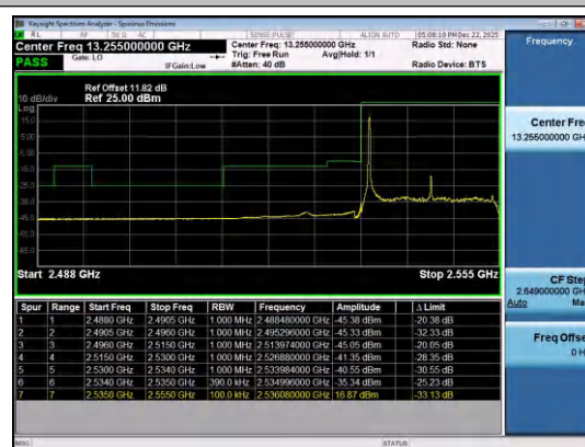
Band41(2535-2655)-20MHz-16QAM-40140-1RB#0-PA
