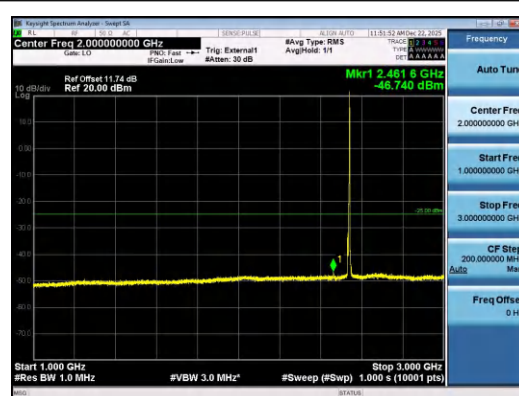
Band41(2535-2655)-5MHz-QPSK-40065-1RB#2 4-1000~3000-PASS
