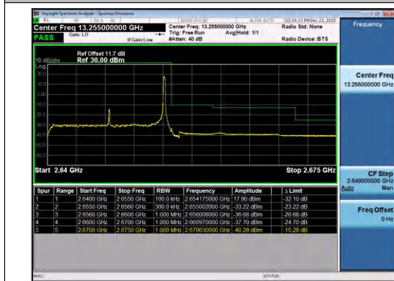
Band41(2535-2655)-15MHz-16QAM-41165-1RB#74-P
