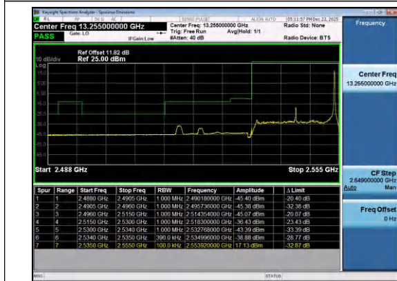
Band41(2535-2655)-20MHz-16QAM-40140-1RB#99-P
