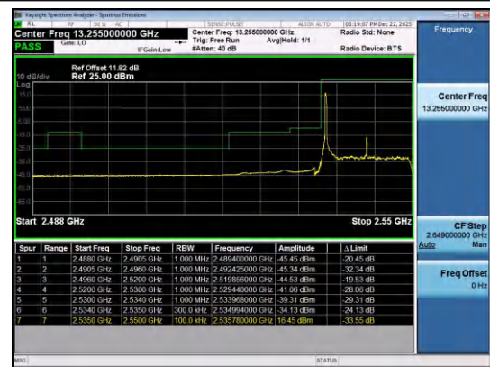
Band41(2535-2655)-15MHz-16QAM-40115-1RB#0-PA
