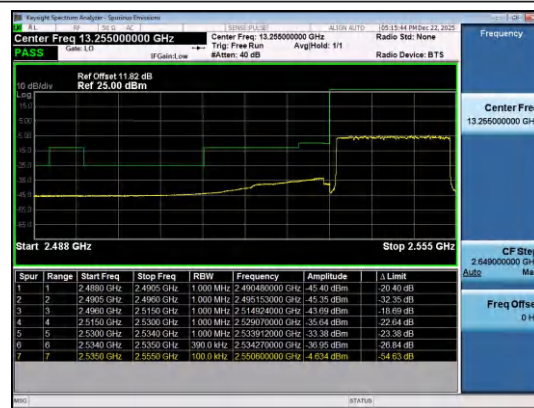
Band41(2535-2655)-20MHz-16QAM-40140-100RB#0-P
