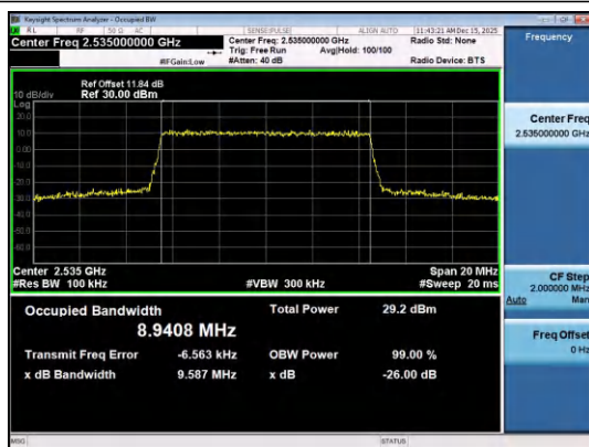
Band7-10MHz-QPSK-21100-50RB#0-PASS
