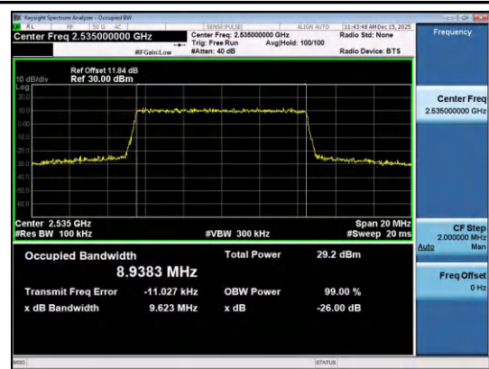
Band7-10MHz-QPSK-21100-50RB#0-PASS
