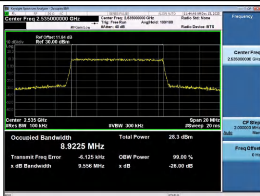
Band7-10MHz-16QAM-21100-50RB#0-PASS
