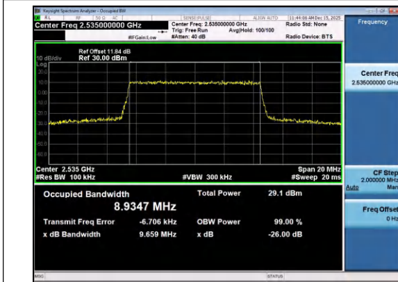
Band7-10MHz-QPSK-21100-50RB#0-PASS
