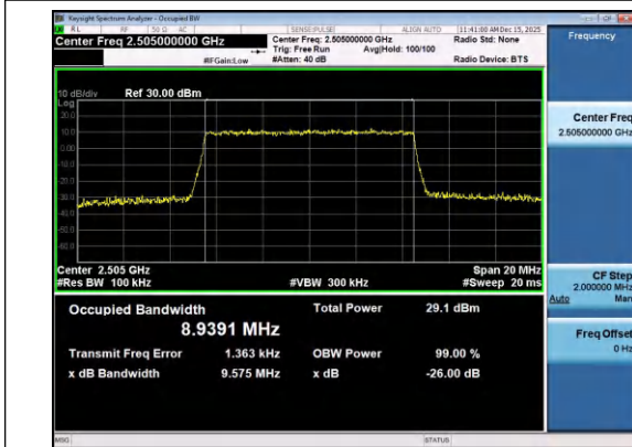
Band7-10MHz-QPSK-20800-50RB#0-PASS
