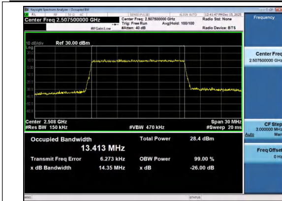
Band7-15MHz-16QAM-20825-75RB#0-PASS
