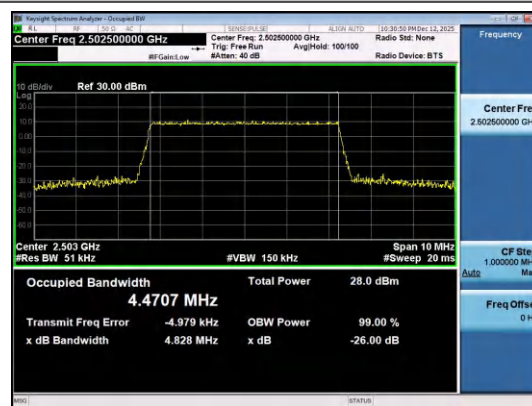
Band7-5MHz-16QAM-20775-25RB#0-PASS
