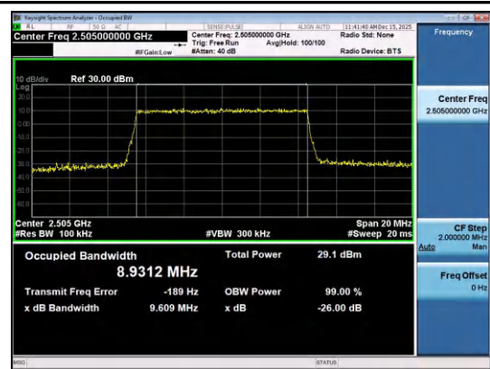
Band7-10MHz-QPSK-20800-50RB#0-PASS
