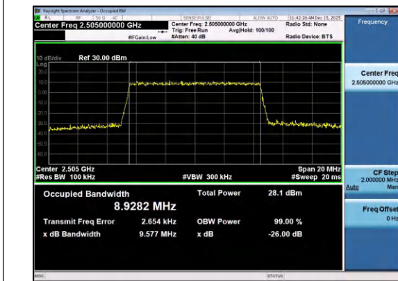
Band7-10MHz-16QAM-20800-50RB#0-PASS
