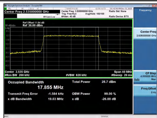
Band7-20MHz-16QAM-21100-100RB#0-PASS
