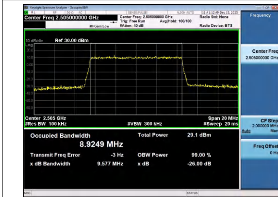
Band7-10MHz-QPSK-20800-50RB#0-PASS
