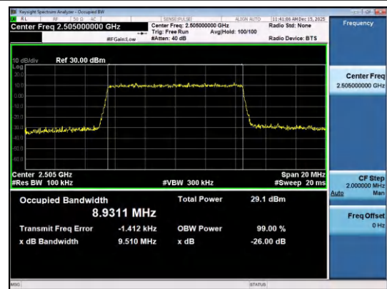
Band7-10MHz-QPSK-20800-50RB#0-PASS
