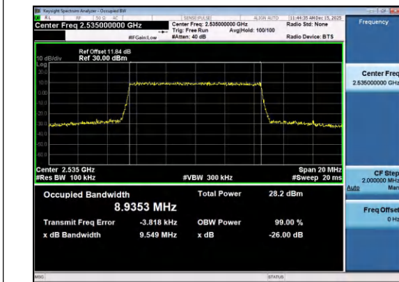
Band7-10MHz-16QAM-21100-50RB#0-PASS
