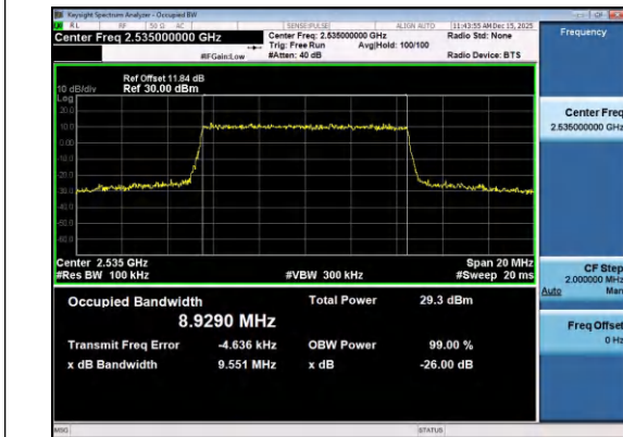
Band7-10MHz-QPSK-21100-50RB#0-PASS
