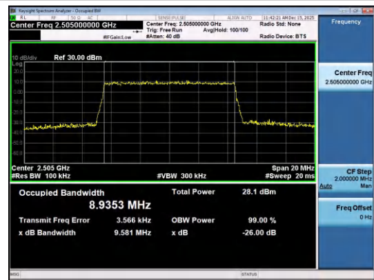
Band7-10MHz-16QAM-20800-50RB#0-PASS
