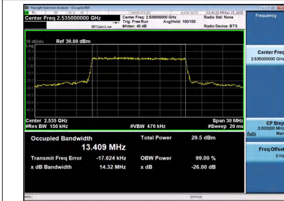
Band7-15MHz-QPSK-21100-75RB#0-PASS
