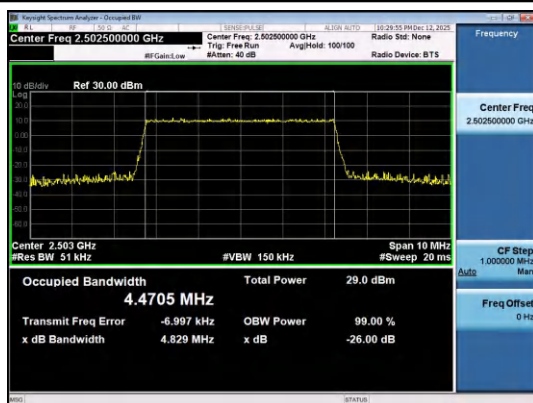
Band7-5MHz-QPSK-20775-25RB#0-PASS
