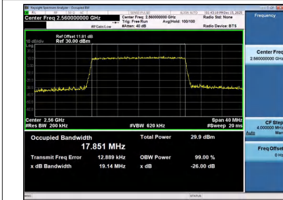
Band7-20MHz-QPSK-21350-100RB#0-PASS
