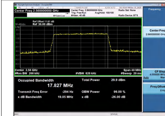
Band7-20MHz-QPSK-21350-100RB#0-PASS
