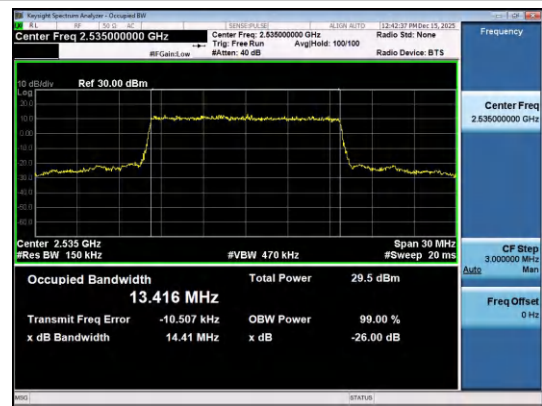
Band7-15MHz-QPSK-21100-75RB#0-PASS
