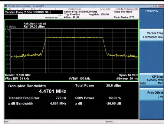
Band7-5MHz-16QAM-21425-25RB#0-PASS
