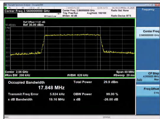
Band7-20MHz-QPSK-21350-100RB#0-PASS
