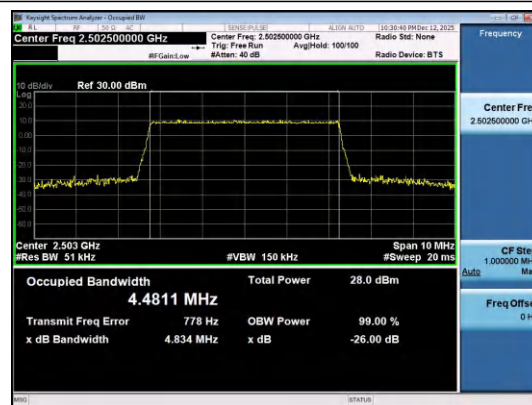
Band7-5MHz-16QAM-20775-25RB#0-PASS
