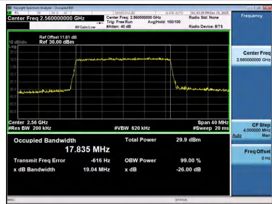
Band7-20MHz-QPSK-21350-100RB#0-PASS
