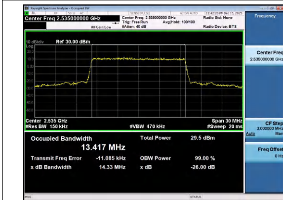
Band7-15MHz-QPSK-21100-75RB#0-PASS
