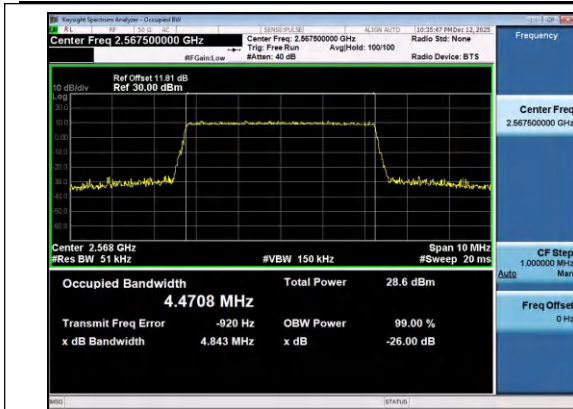
Band7-5MHz-16QAM-21425-25RB#0-PASS
