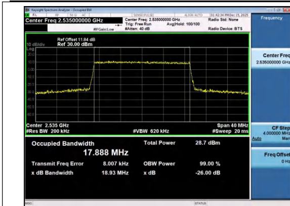
Band7-20MHz-16QAM-21100-100RB#0-PASS
