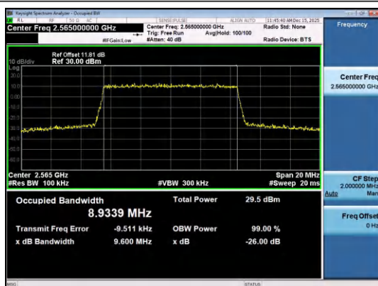
Band7-10MHz-QPSK-21400-50RB#0-PASS
