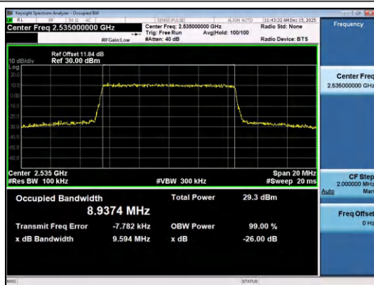
Band7-10MHz-QPSK-21100-50RB#0-PASS
