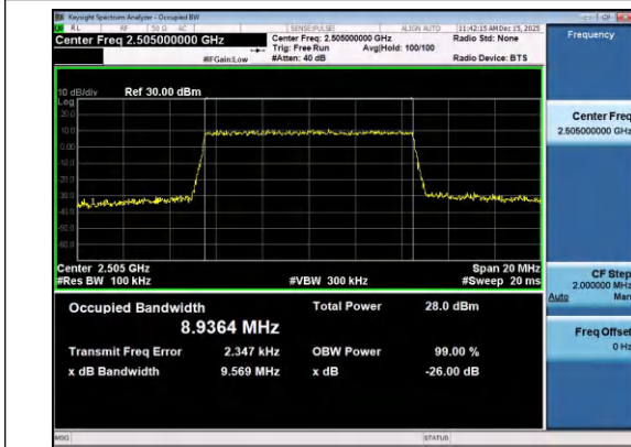
Band7-10MHz-16QAM-20800-50RB#0-PASS
