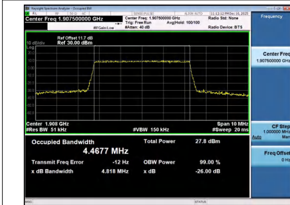
Band2-5MHz-QPSK-19175-25RB#0-PASS
