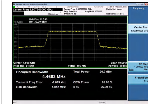
Band2-5MHz-16QAM-19175-25RB#0-PASS
