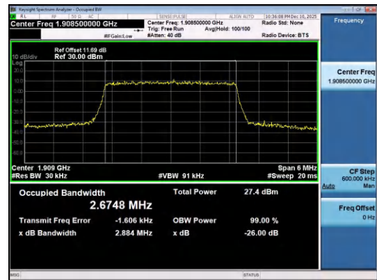
Band2-3MHz-QPSK-19185-15RB#0-PASS
