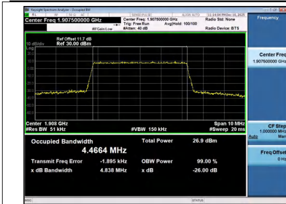
Band2-5MHz-16QAM-19175-25RB#0-PASS
