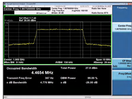
Band2-5MHz-QPSK-19175-25RB#0-PASS
