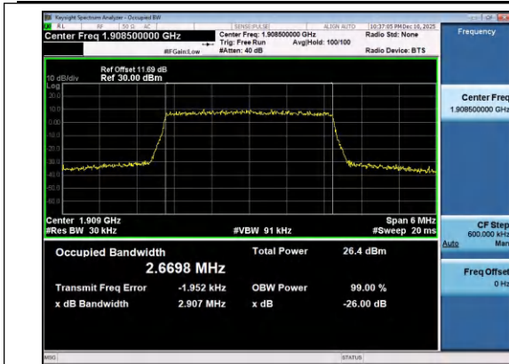
Band2-3MHz-16QAM-19185-15RB#0-PASS
