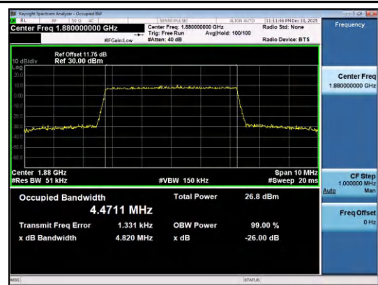
Band2-5MHz-16QAM-18900-25RB#0-PASS
