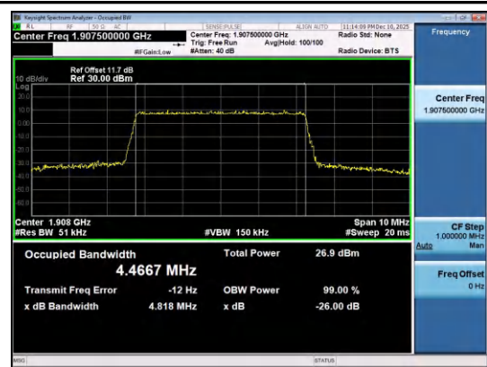
Band2-5MHz-16QAM-19175-25RB#0-PASS
