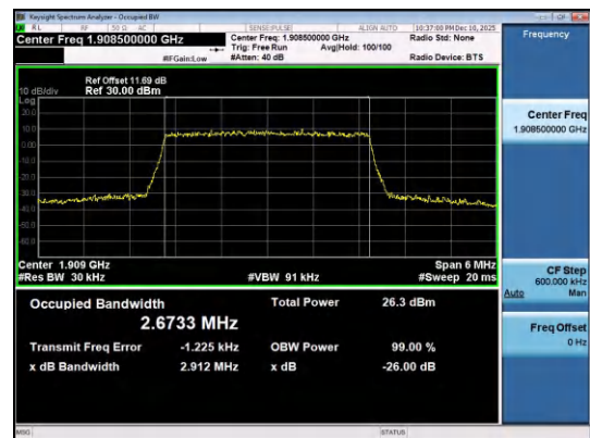
Band2-3MHz-16QAM-19185-15RB#0-PASS
