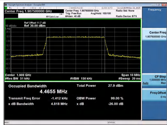
Band2-5MHz-QPSK-19175-25RB#0-PASS
