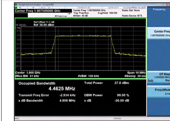
Band2-5MHz-QPSK-19175-25RB#0-PASS
