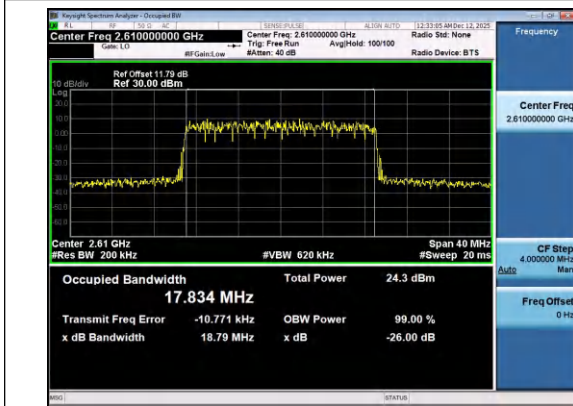
Band38-20MHz-16QAM-38150-100RB#0-PASS
