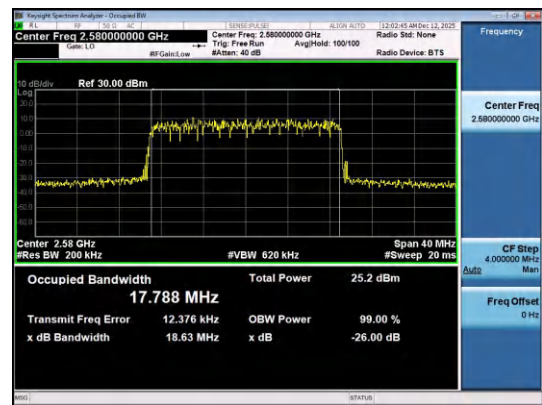
Band38-20MHz-QPSK-37850-100RB#0-PASS
