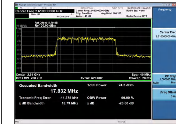
Band38-20MHz-16QAM-38150-100RB#0-PASS
