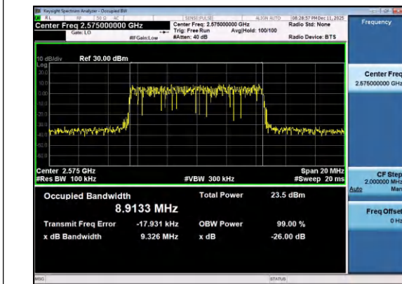
Band38-10MHz-16QAM-37800-50RB#0-PASS
