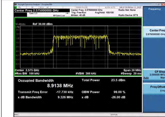
Band38-10MHz-16QAM-37800-50RB#0-PASS
