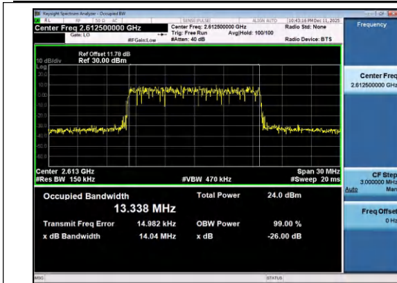
Band38-15MHz-16QAM-38175-75RB#0-PASS
