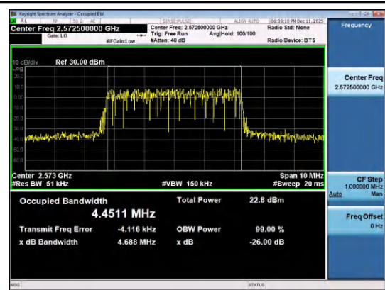
Band38-5MHz-16QAM-37775-25RB#0-PASS
