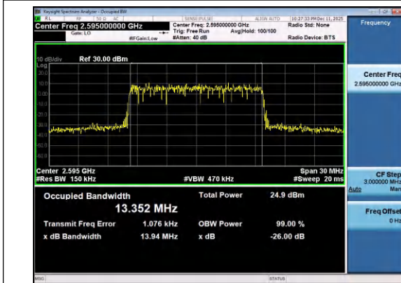
Band38-15MHz-QPSK-38000-75RB#0-PASS
