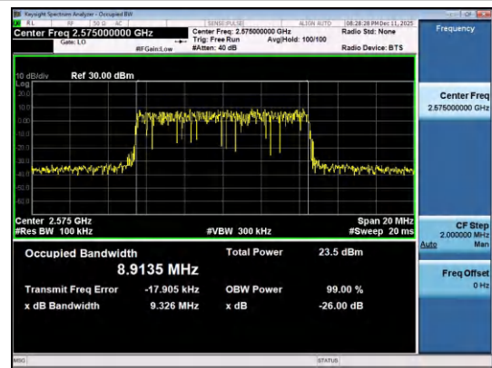
Band38-10MHz-16QAM-37800-50RB#0-PASS
