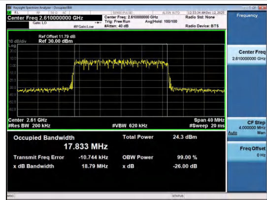
Band38-20MHz-16QAM-38150-100RB#0-PASS
