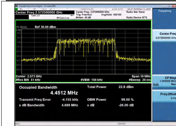
Band38-5MHz-16QAM-37775-25RB#0-PASS
