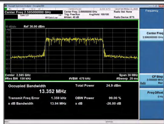
Band38-15MHz-QPSK-38000-75RB#0-PASS
