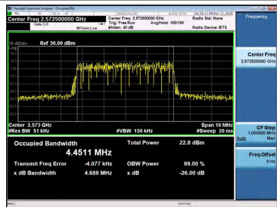
Band38-5MHz-16QAM-37775-25RB#0-PASS
