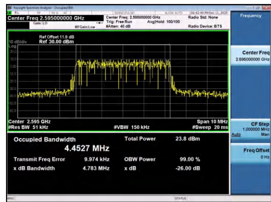
Band38-5MHz-QPSK-38000-25RB#0-PASS
