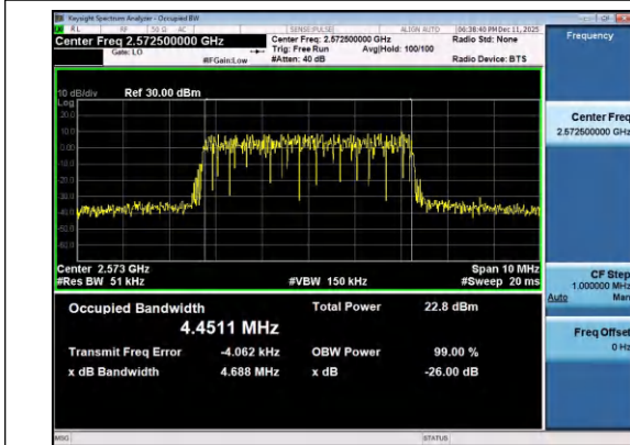
Band38-5MHz-16QAM-37775-25RB#0-PASS
