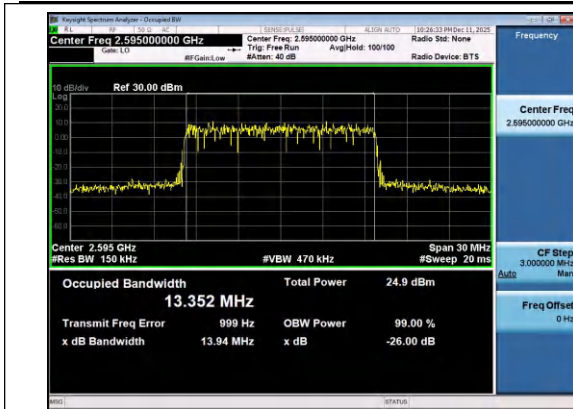
Band38-15MHz-QPSK-38000-75RB#0-PASS
