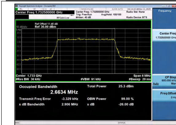
Band4-3MHz-16QAM-20175-15RB#0-PASS
