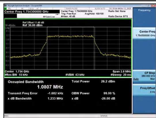
Band4-1.4MHz-QPSK-20393-6RB#0-PASS
