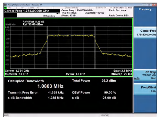
Band4-1.4MHz-QPSK-20393-6RB#0-PASS
