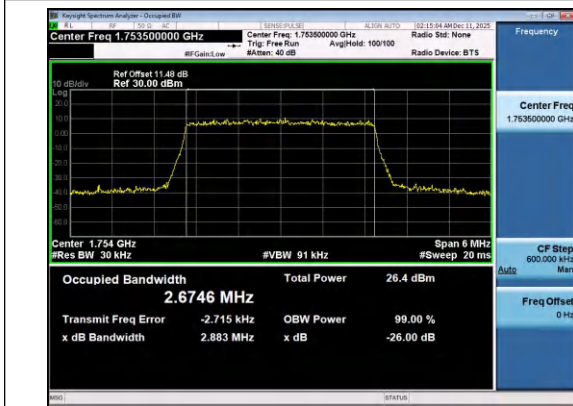
Band4-3MHz-QPSK-20385-15RB#0-PASS
