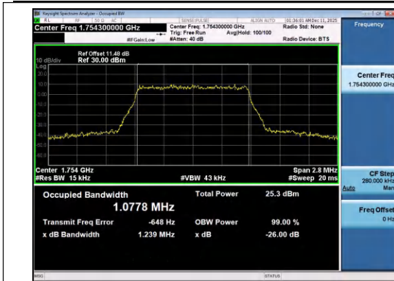
Band4-1.4MHz-16QAM-20393-6RB#0-PASS
