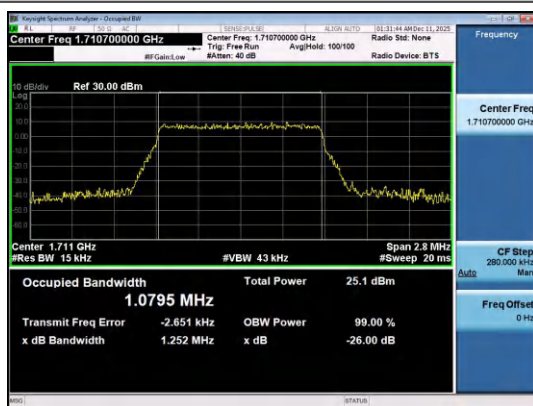
Band4-1.4MHz-16QAM-19957-6RB#0-PASS
