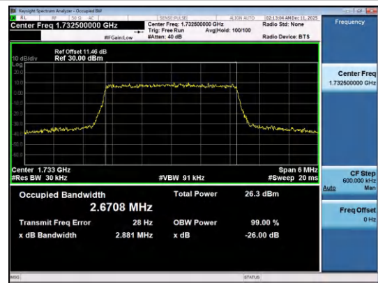
Band4-3MHz-QPSK-20175-15RB#0-PASS
