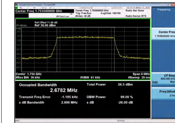
Band4-3MHz-QPSK-20385-15RB#0-PASS
