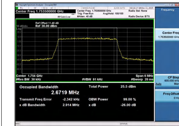
Band4-3MHz-16QAM-20385-15RB#0-PASS
