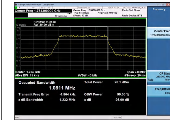
Band4-1.4MHz-QPSK-20393-6RB#0-PASS
