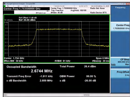
Band4-3MHz-QPSK-20385-15RB#0-PASS
