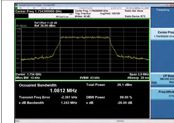
Band4-1.4MHz-QPSK-20393-6RB#0-PASS
