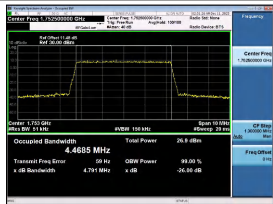
Band4-5MHz-QPSK-20375-25RB#0-PASS
