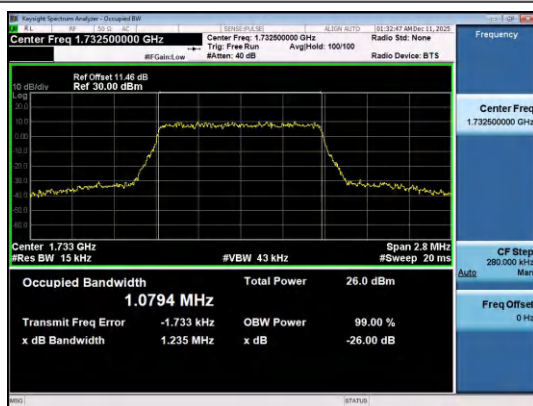
Band4-1.4MHz-QPSK-20175-6RB#0-PASS
