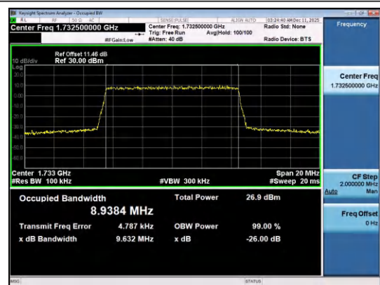
Band4-10MHz-QPSK-20175-50RB#0-PASS
