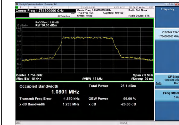
Band4-1.4MHz-16QAM-20393-6RB#0-PASS
