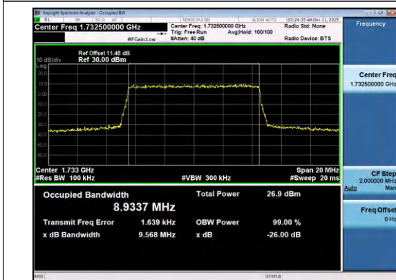
Band4-10MHz-QPSK-20175-50RB#0-PASS
